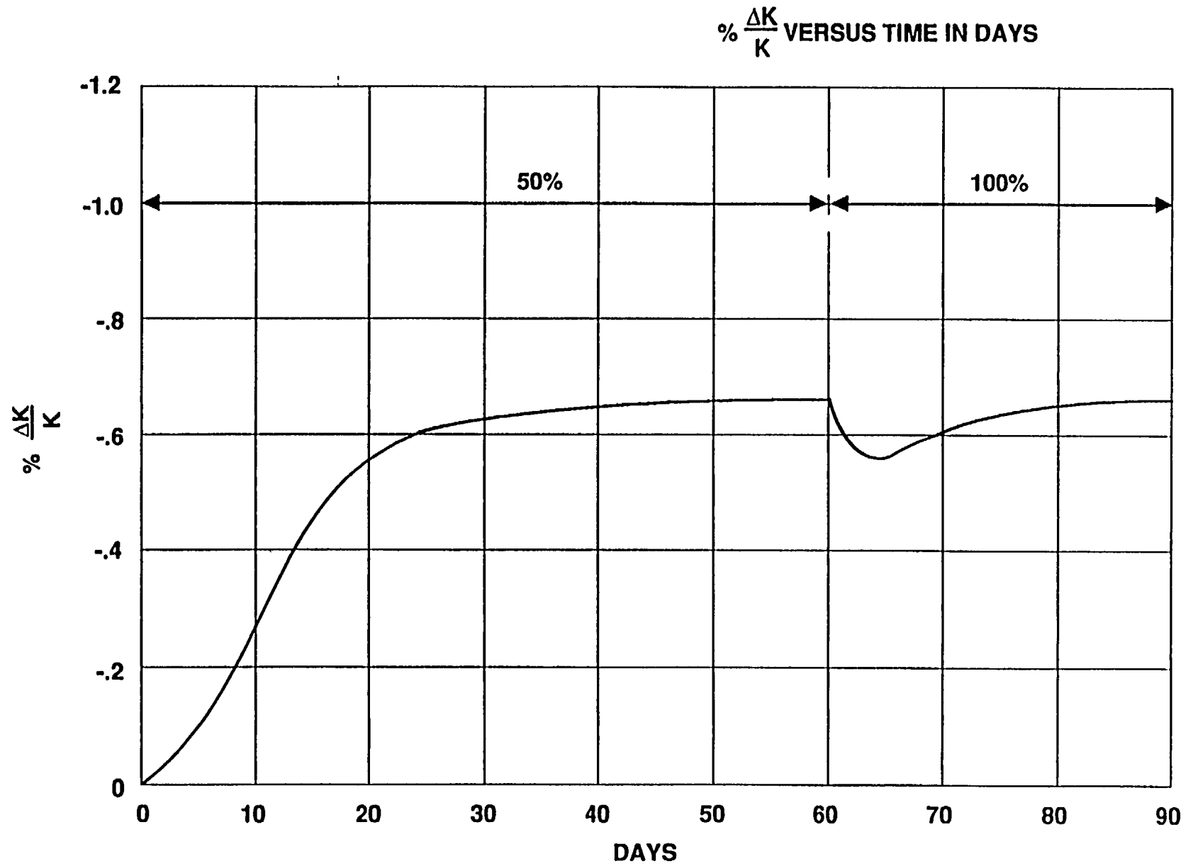
Figure 2 - 18. Samarium Buildup
