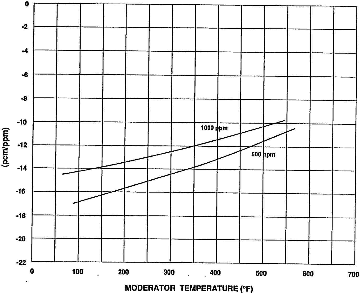
Figure 2-14. Boron Worth Vs. Moderator Temperature
