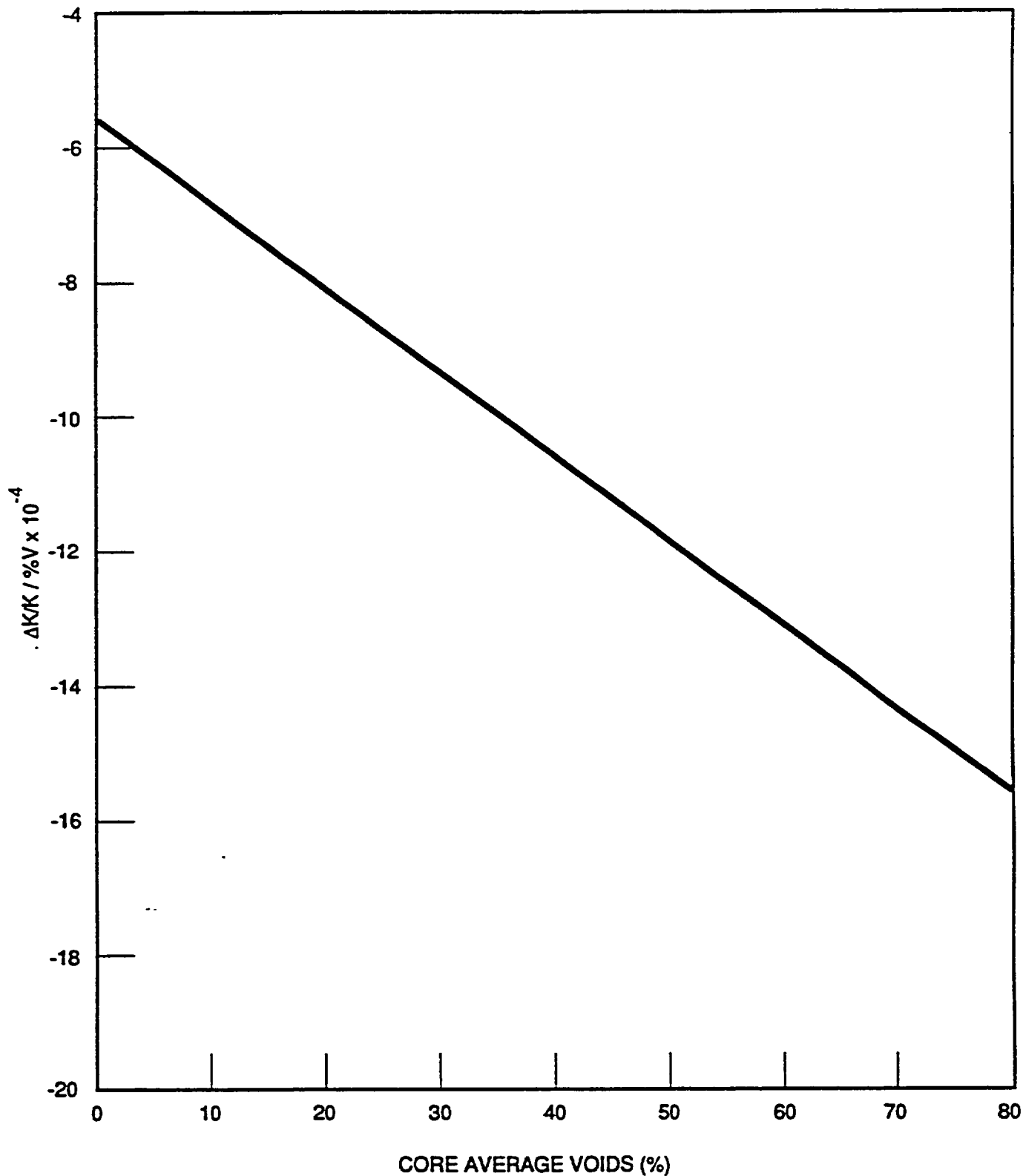
Figure 2-5. Void Coefficient
