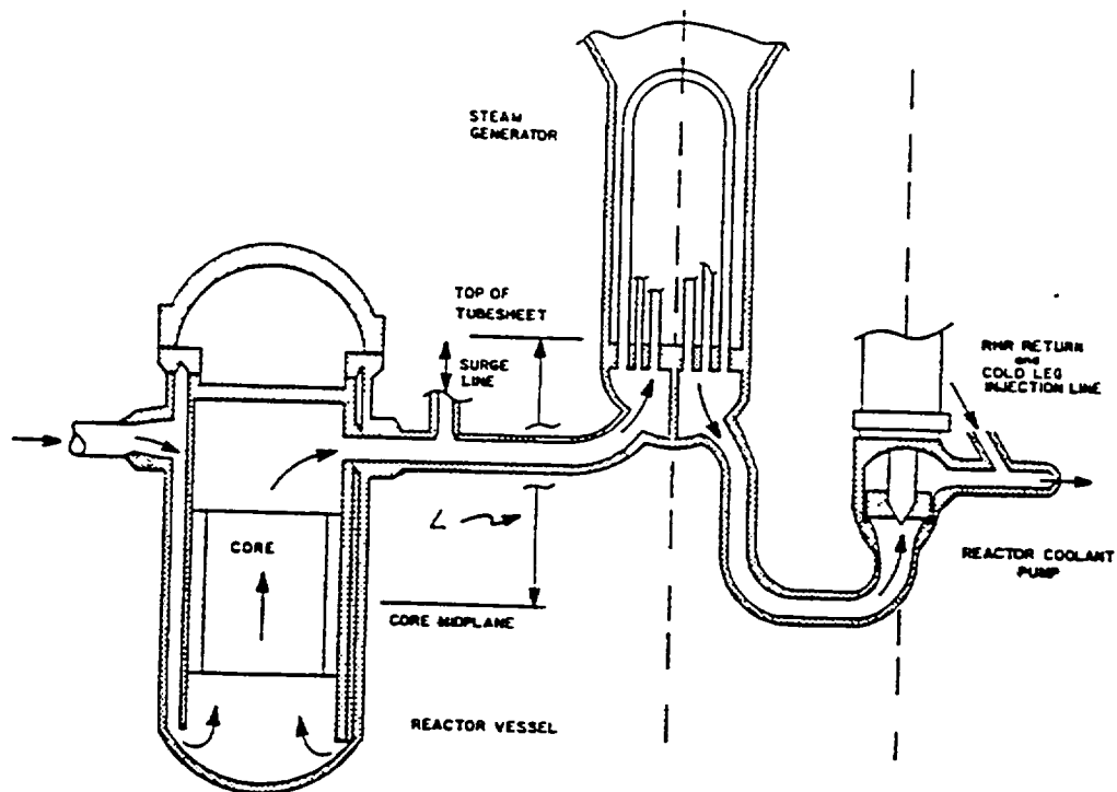
A. Typical Natural Circulation Geometry
