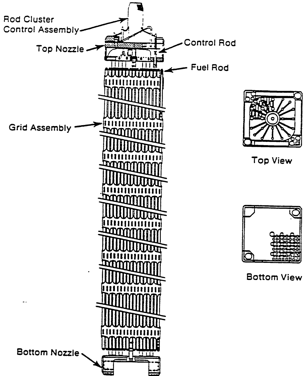
Figure 1-11. Typical PWR Fuel Assembly
