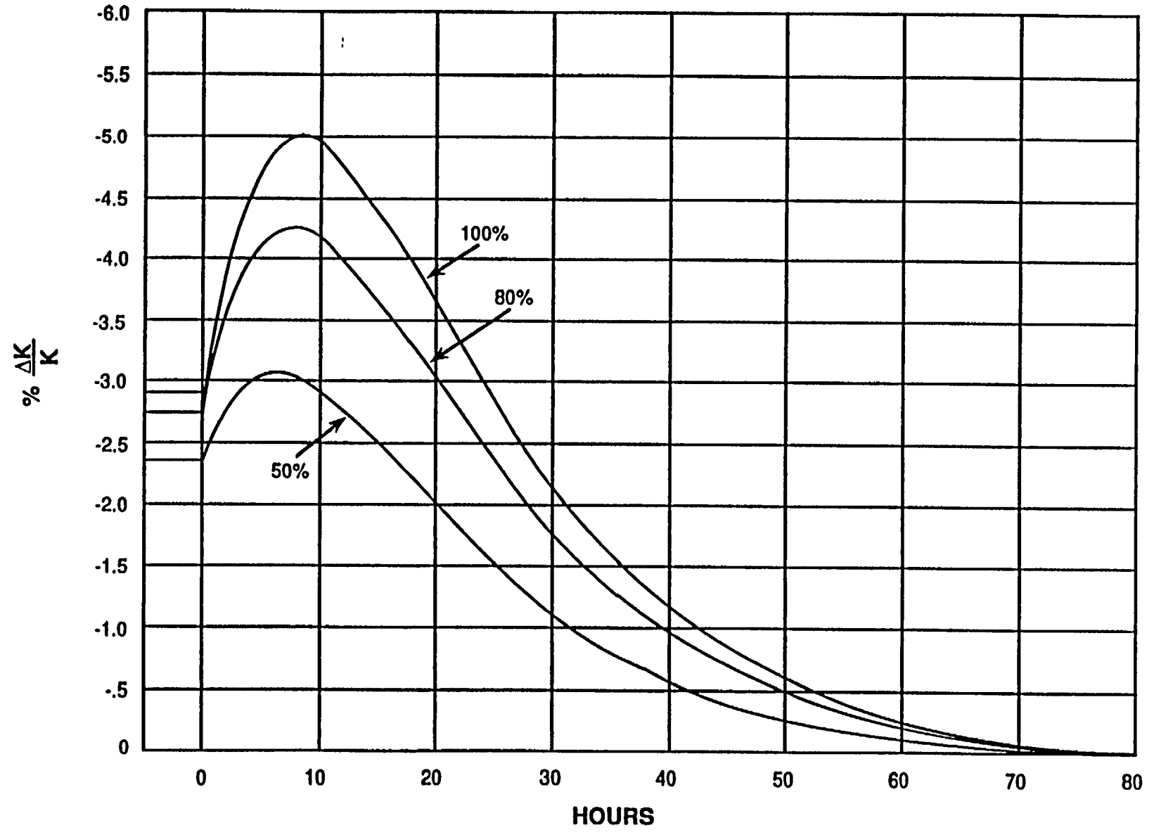
Figure 2-17. Xenon Peaking
