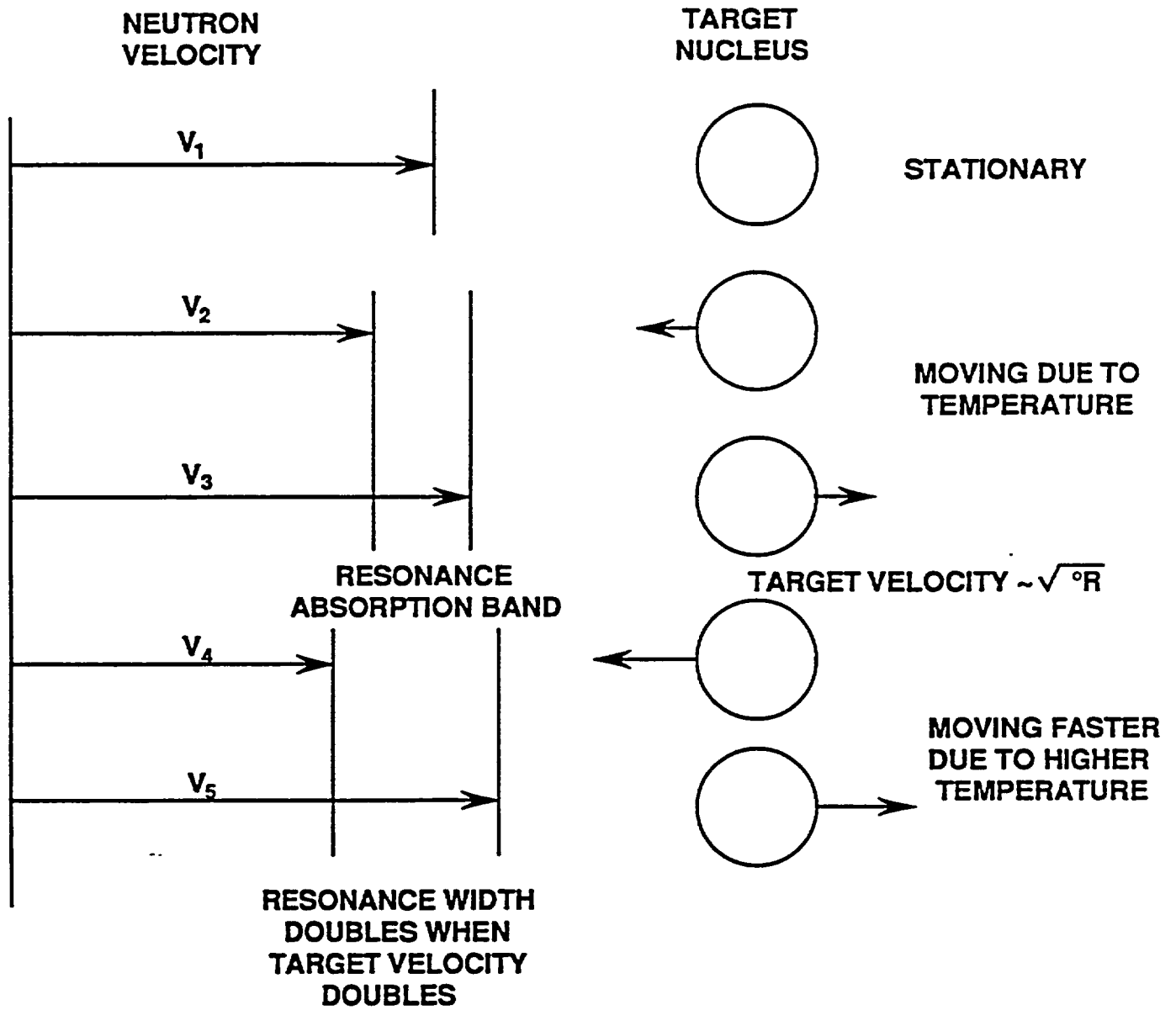
Figure 2-7. Resonance Capture
