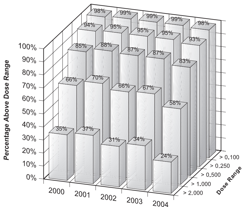
FIGURE 3.3. Collective TEDE Distribution by Dose Range Industrial Radiographer—Multiple Location Licensees 2000 - 2004
