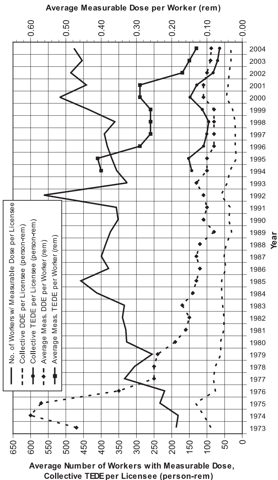
FIGURE 3.10. Average Annual Values at Fuel Cycle Licensees 1973-2004
