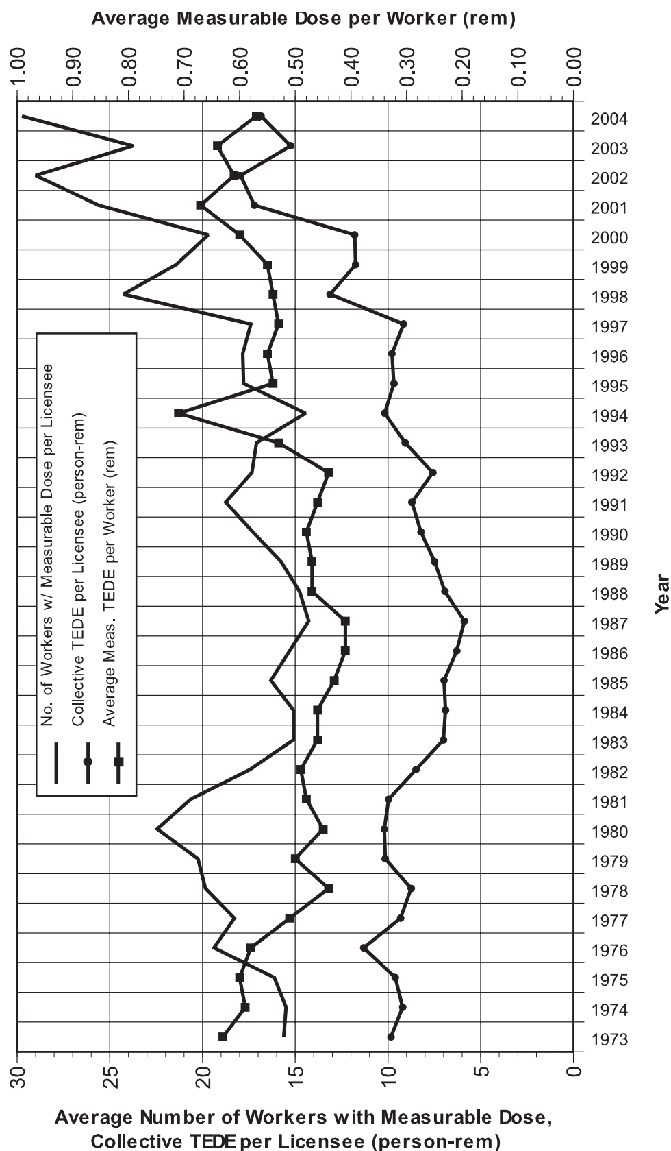
FIGURE 3.1. Average Annual Values at Industrial Radiography Facilities 1973 - 2004
