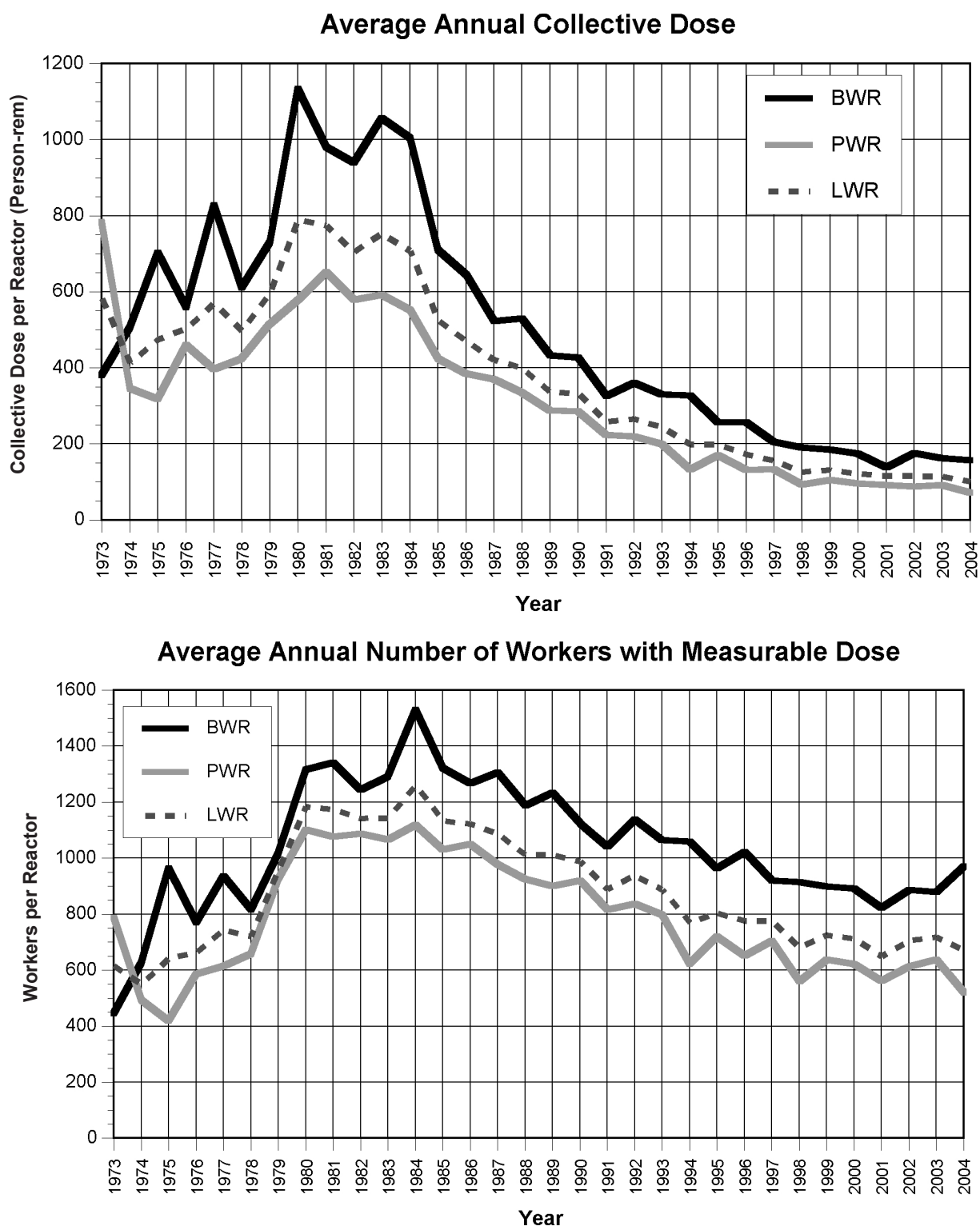
FIGURE 4.1. Average Collective Dose and Number of Workers with Measurable Dose per Reactor 1973-2004
