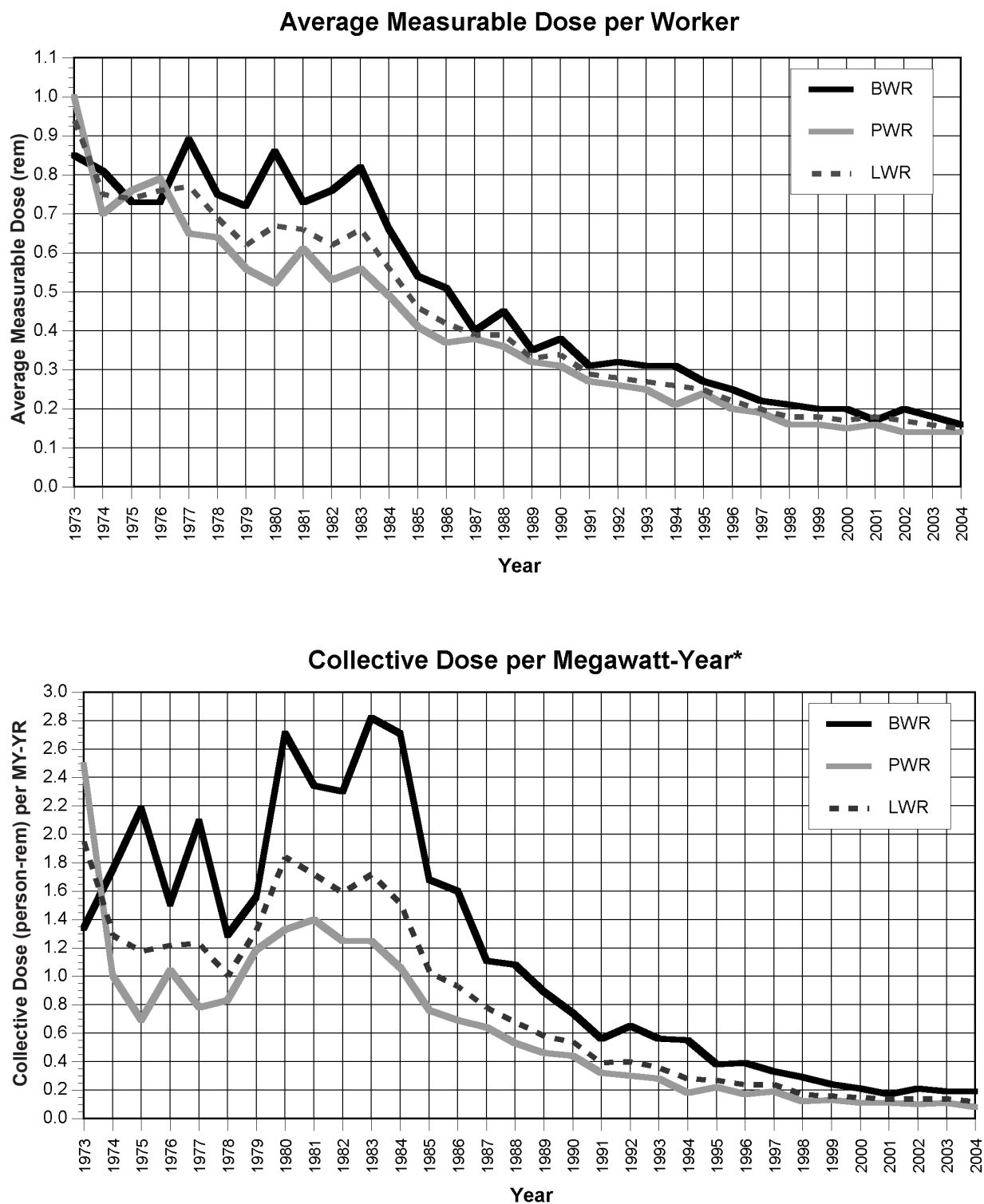
FIGURE 4.3. Average Measurable Dose per Worker and Collective Dose per Megawatt-Year 1973-2004
