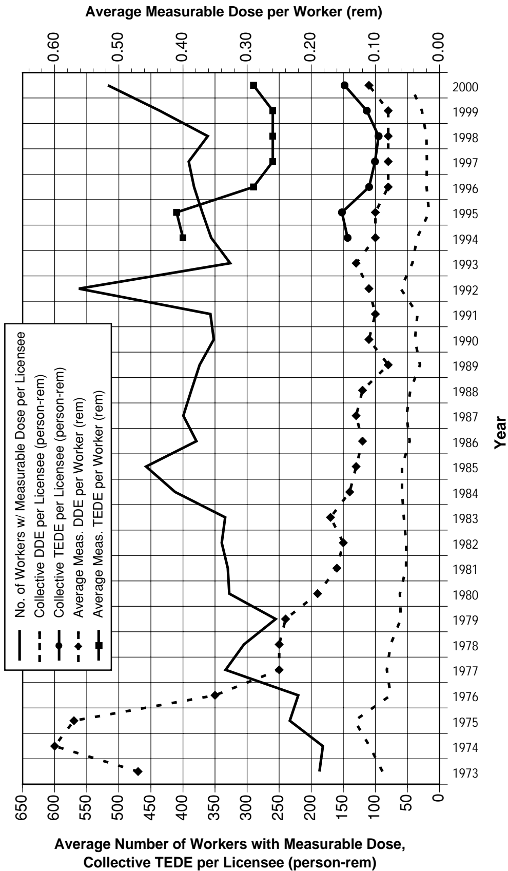
FIGURE 3.11. Average Annual Values at Fuel Cycle Licensees 1973 - 2000
