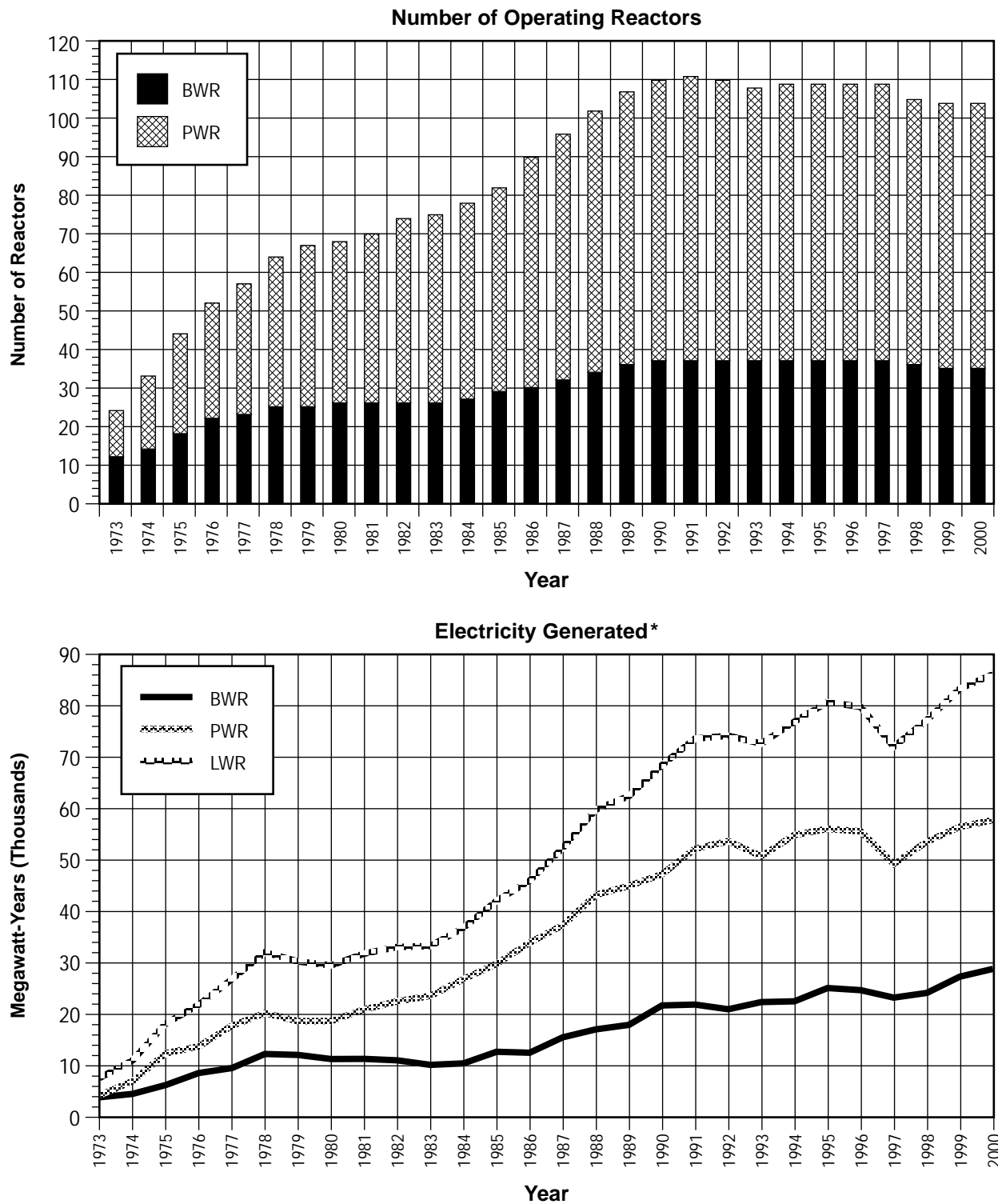
FIGURE 4.2. Number of Operating Reactors and Gross Electricity Generated 1973 - 2000
