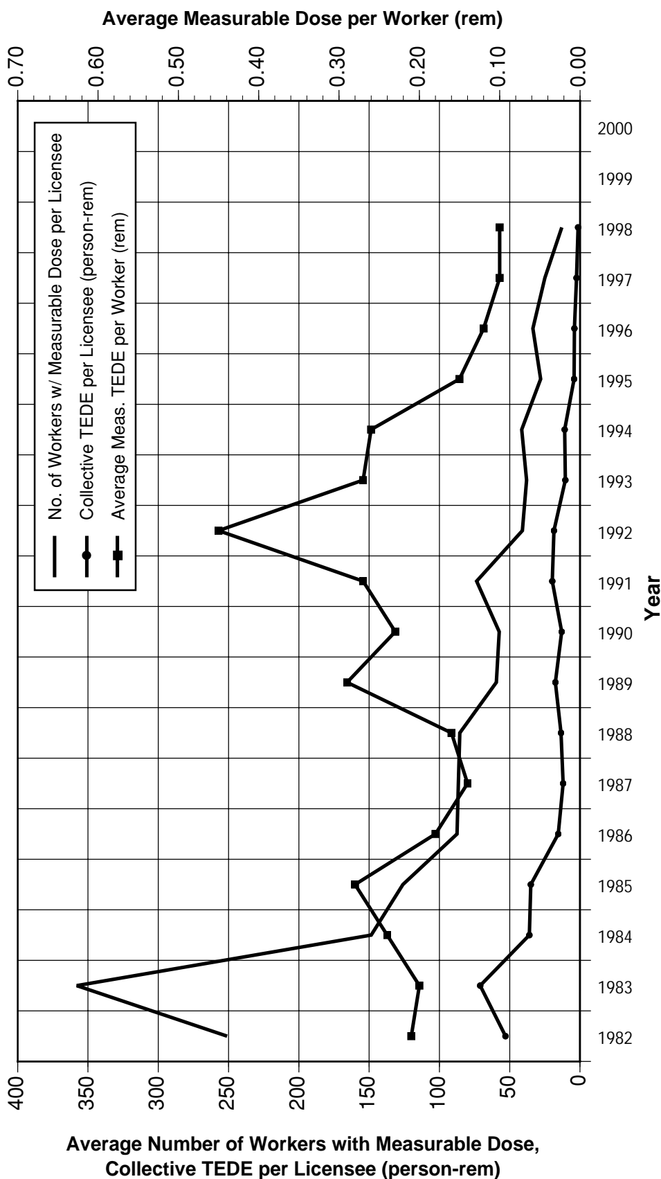
FIGURE 3.7. Average Annual Values at Low-Level Waste Disposal Facilities 1982 - 2000
