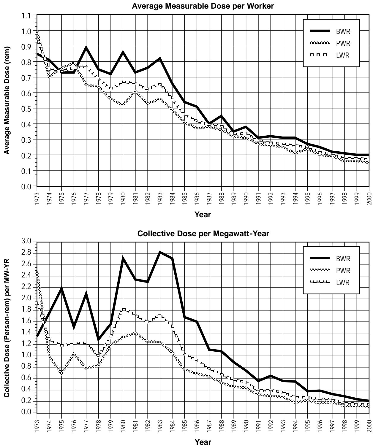
FIGURE 4.3. Average Measurable Dose per Worker and Collective Dose per Megawatt-Year 1973 - 2000
