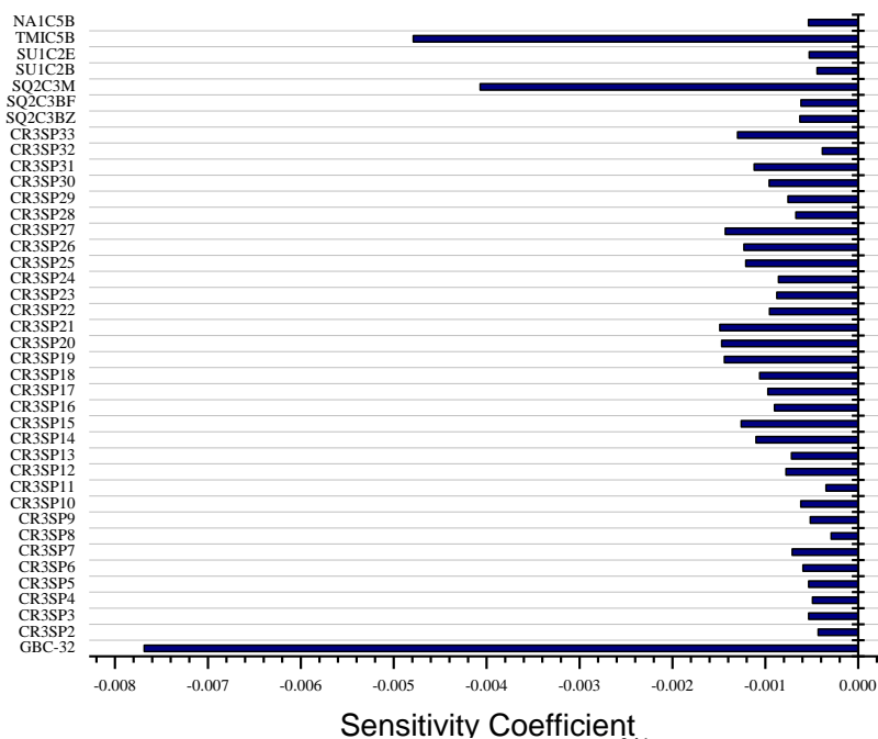
Fig. A.12 Energy- and region-integrated k_{eff} sensitivities to ^{241}\text{Am} total cross section.
