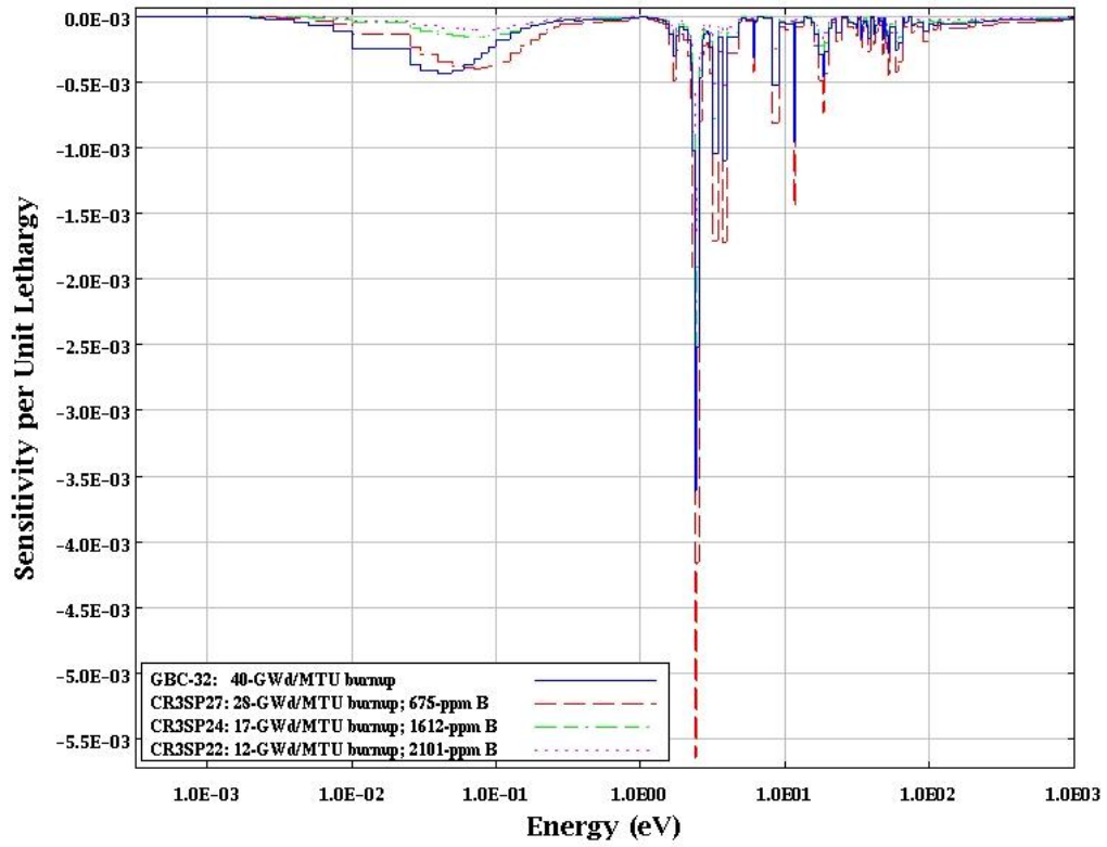
Fig. B.9 Comparison of ^{153}\text{Eu} sensitivity profiles for GBC40, CR3SP27, CR3SP24, and CR3SP22.
