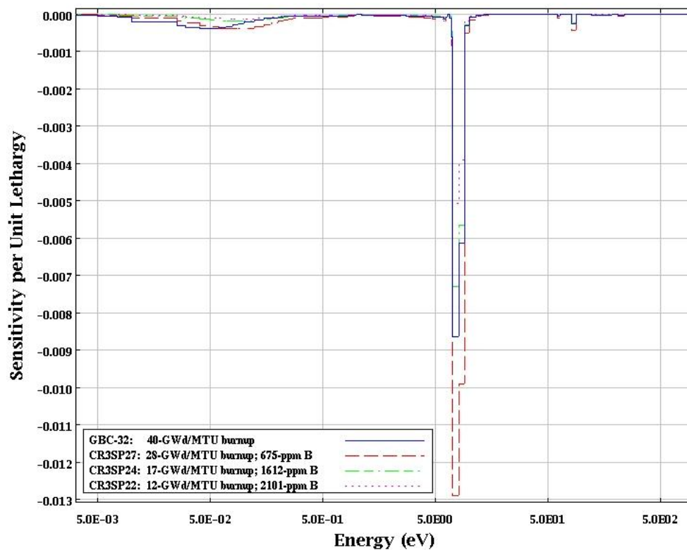
Fig. B.8 Comparison of 152 Sm sensitivity profiles for GBC40, CR3SP27, CR3SP24, and CR3SP22.
