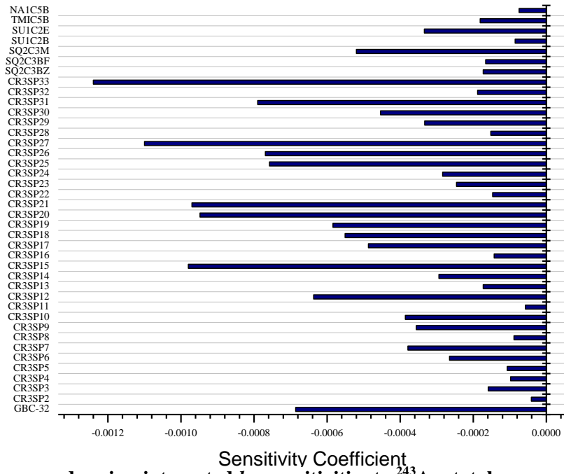
Fig. A.29 Energy- and region-integrated k_{eff} sensitivities to ^{243}\text{Am} total cross section.
