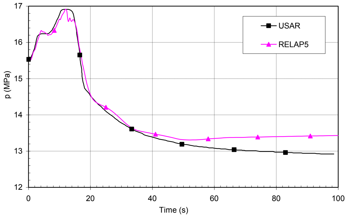
Figure 3 Pressurizer pressure - base case comparison between RELAP5 and USAR
