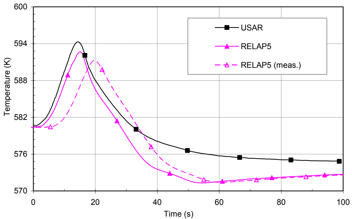
Figure 5 RCS average temperature and measured RCS average temperature - base case comparison between RELAP5 and USAR
