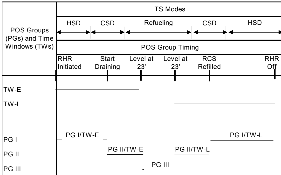
Figure 1B.2 POS and Time Windows for PWRs at Shutdown
