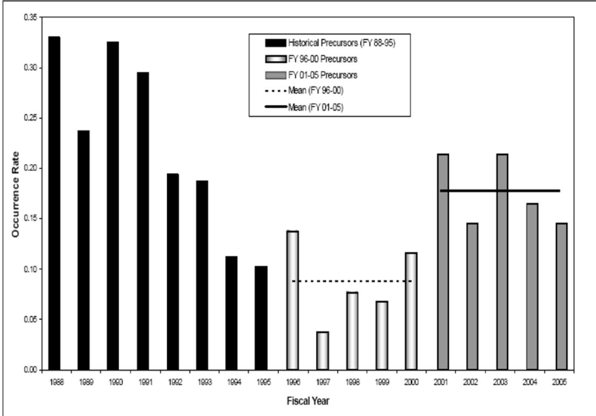
Figure 1: Total Precursors — occurrence rate, by fiscal year. Data for FY 1988 through FY 1995 are shown for historical perspective. Data from FY 2001 through FY 2005 represent the period with an increased ASP scope. No statistically significant trend (p-value = 0.8608) is detected during the FY 2001–2005 period. Data from FY 1996 through 2000 are charted separately since it is part of the data from within the last 10 years without the increase in ASP scope. No statistically significant trend (p-value = 0.3735) is detected during the FY 1996–2000 period.
