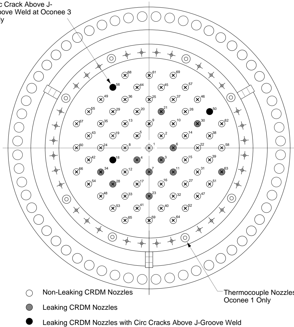
Figure 1 Locations of Leaking CRDM Nozzles at Ocone and ANO-1
