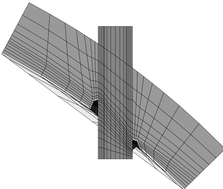
Figure 5 Typical FEA Model of Peripheral Row CRDM Nozzle
