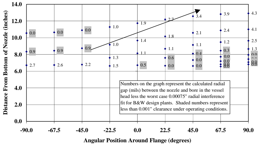
Figure 6 Effect of Nozzle Ovalization on Fit
