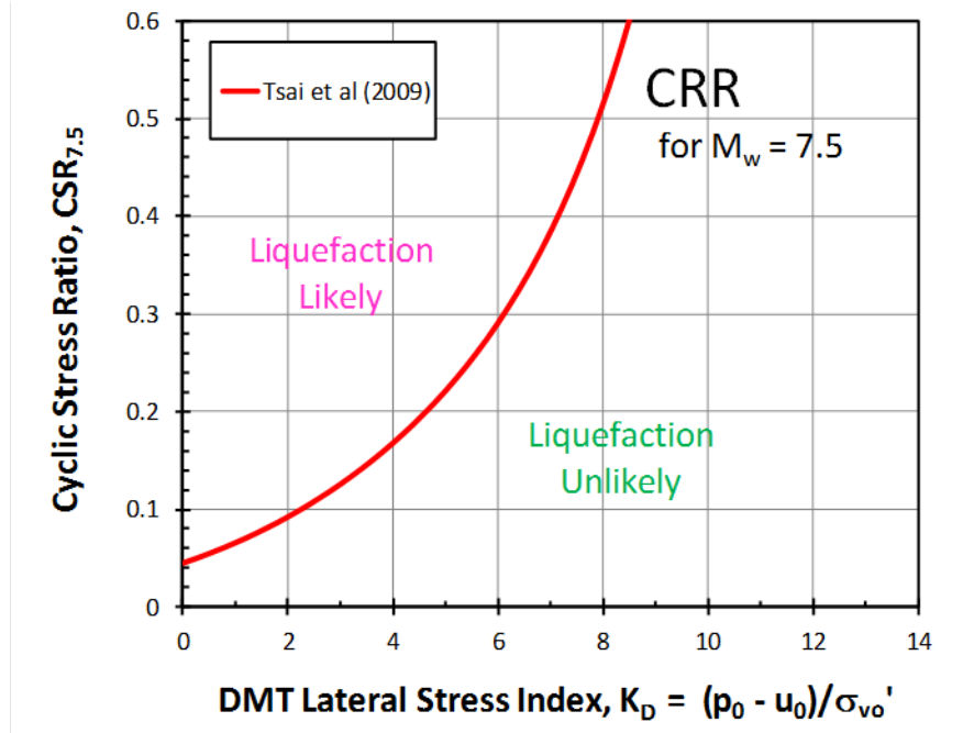
Figure B-6 Recommended CRR_{7.5} for liquefaction evaluation using DMT in clean sands (after Tsai et al., 2009)
