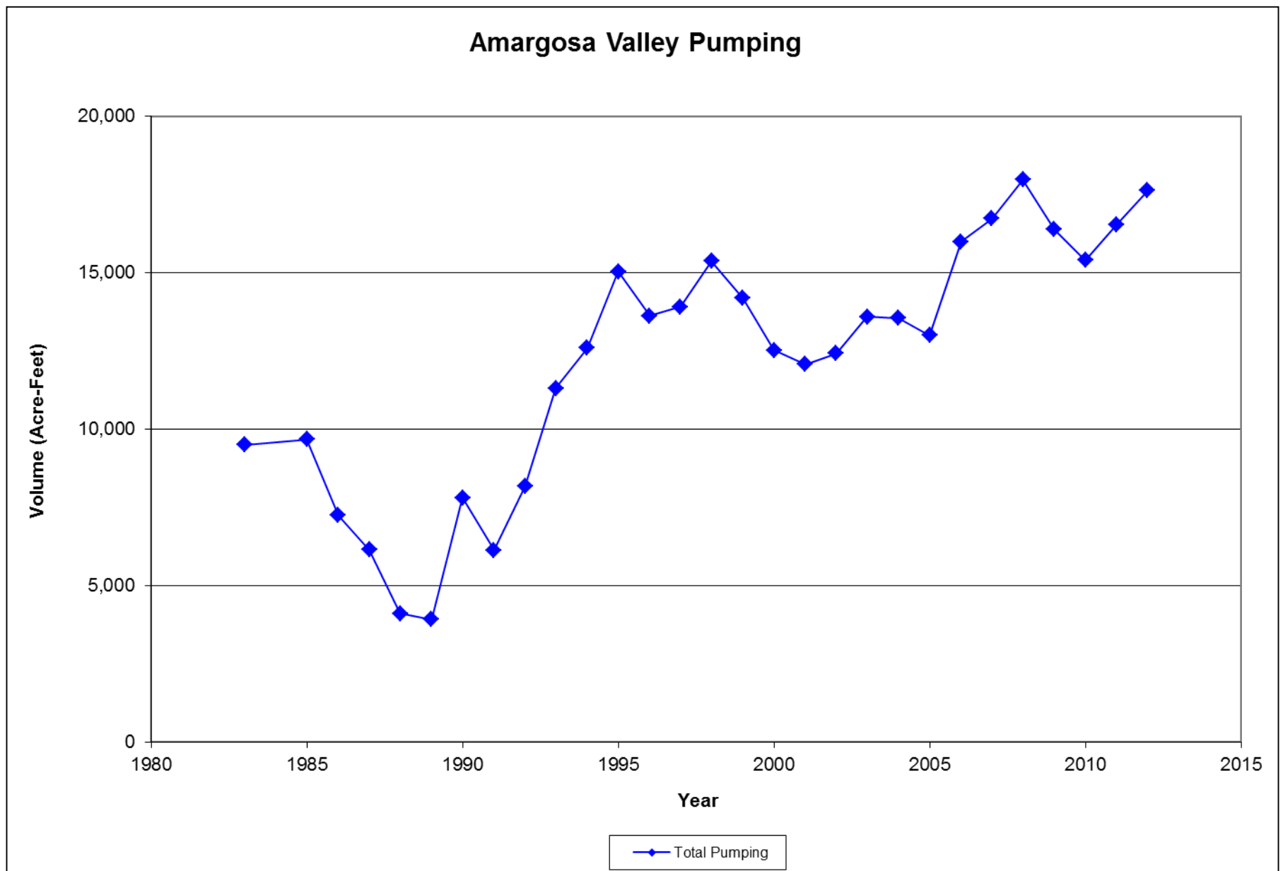
Figure 3-9. Pumping vs. Time, Amargosa Desert Area, Nevada
