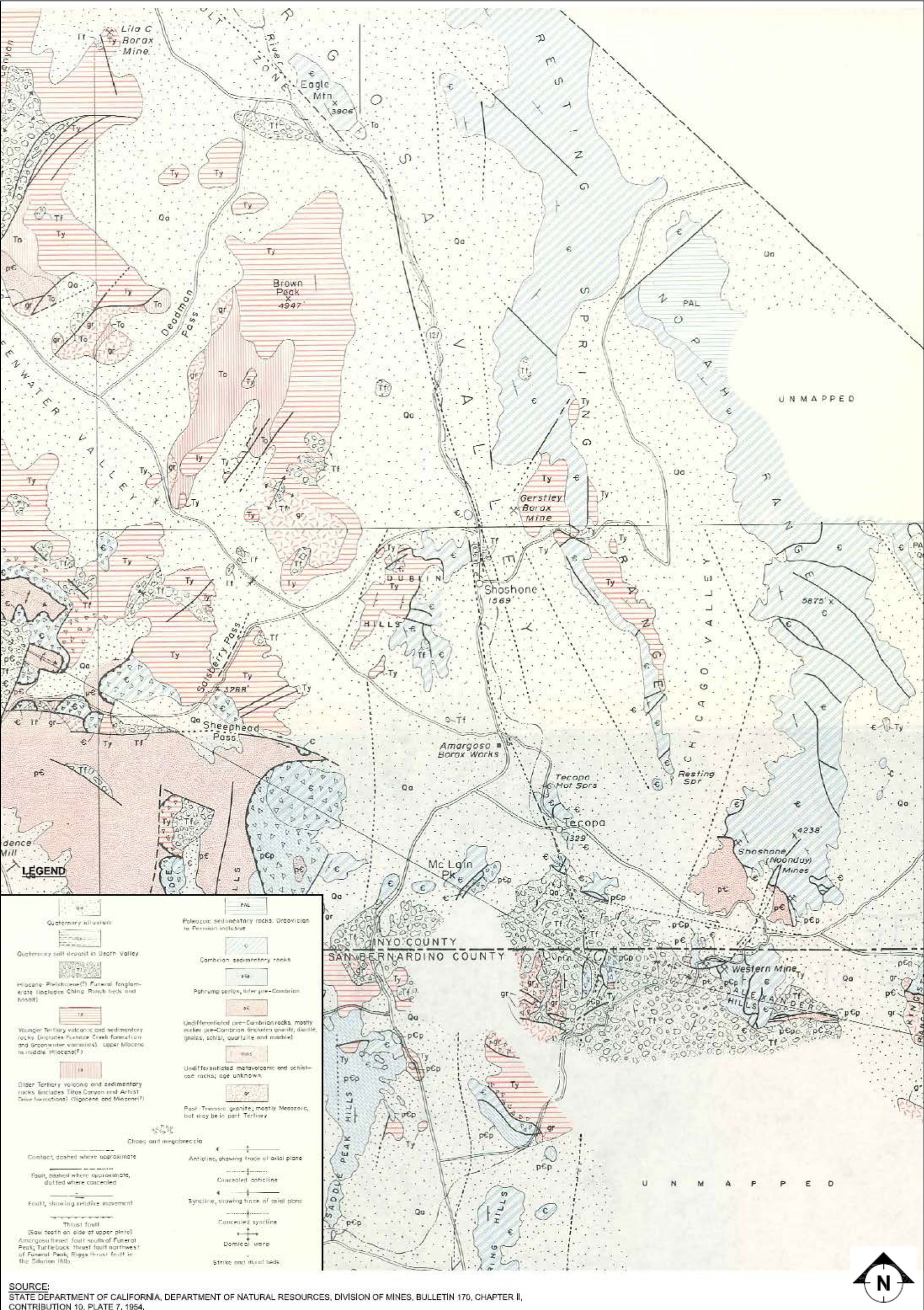
Figure 3-2. Geology of the Shoshone-Tecopa Area
