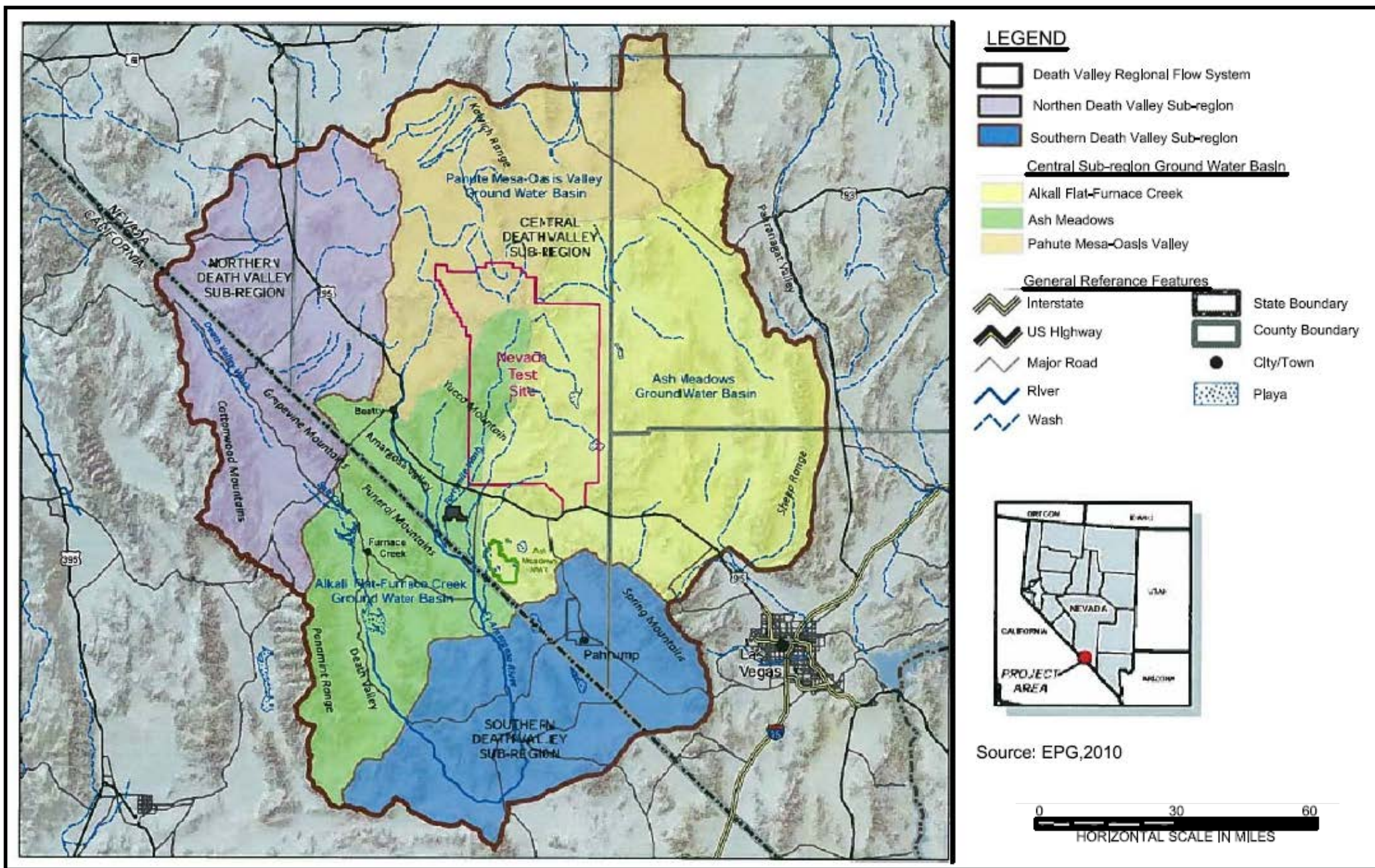
Figure 3-3. Extent of the Death Valley Regional Flow System
