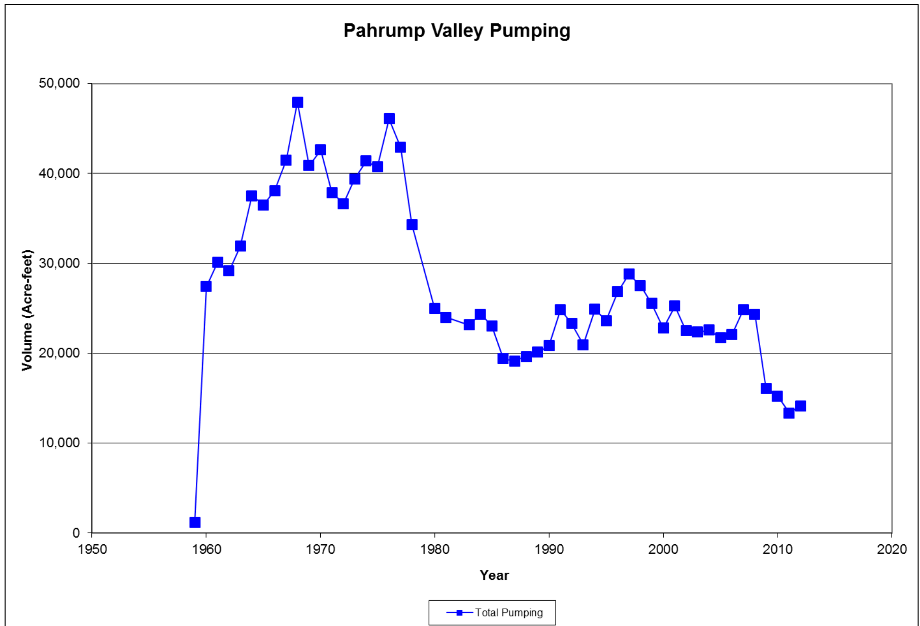
Figure 3-10. Pumping vs. Time, Pahrump Valley, Nevada
