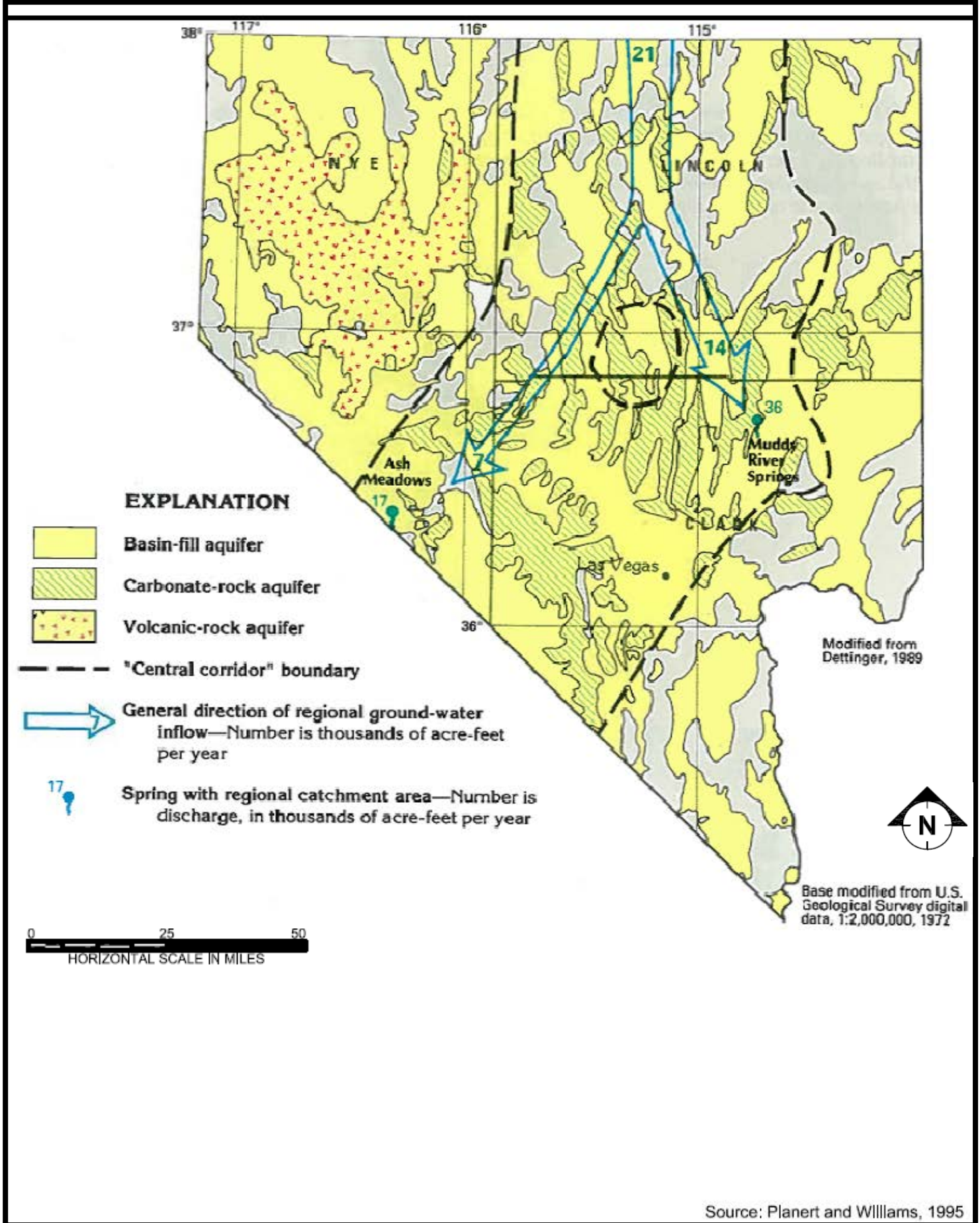
Figure 3-4. Paths for Regional Groundwater Flow – Nevada Portion of Basin
