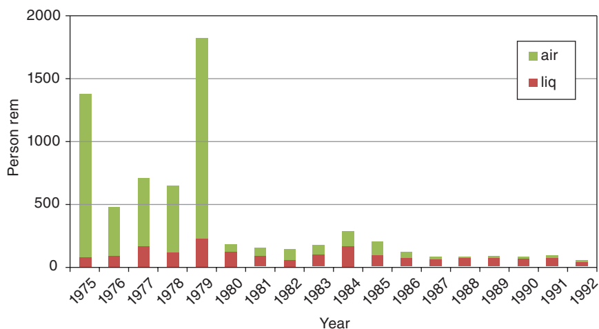
FIGURE 3.4 Collective doses from air and liquid effluents at all operating nuclear plants from 1975 to 1992. SOURCE: NUREG/CR-2850 (PNL-4221), vol. 14.
