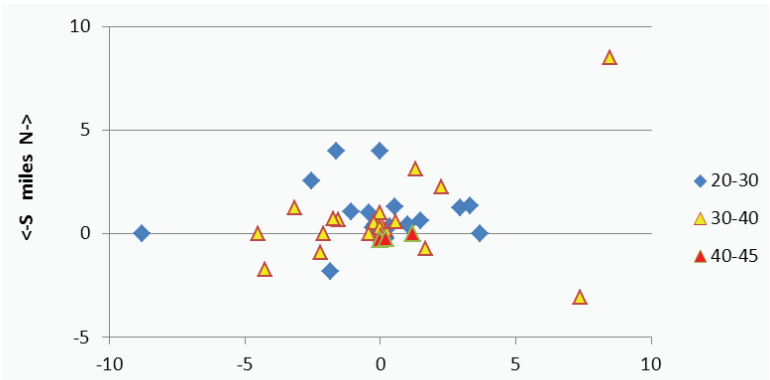
FIGURE 3.9 Variations in background radiation around the Millstone plant for 2009 based on TLD data. Note the relatively higher values near the fence line and variations with distance and direction. SOURCE: Dominion Nuclear Connecticut, Inc. (2009).
