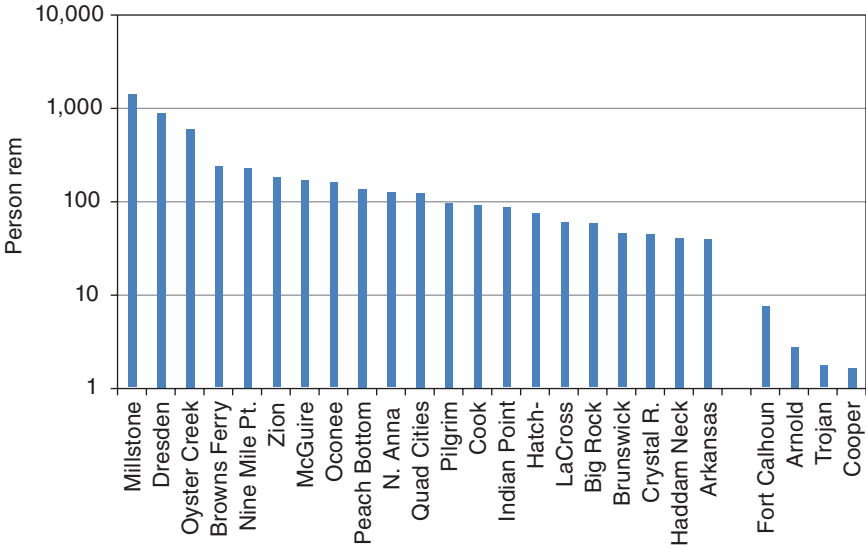
FIGURE 3.2 Collective doses to populations living between 2 and 80 km from selected nuclear plants. SOURCE: NUREG/CR-2850 (PNL-4221), vol. 14.
