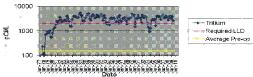
FIGURE 2.13 Variations in tritium concentrations at a surface water monitoring station in the vicinity of the North Anna plant from 1977 to 2010. SOURCE: Dominion (2010b).
