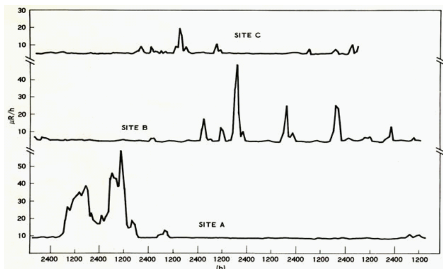
FIGURE 2.16 Mean hourly exposures over a 1-week period at three sites near at the Millstone plant. Site A is located inside the fence line; Site B is located approximately 2 km from the stack; and Site C is located several kilometers away from the stack. SOURCE: Beck et al. (1972).
