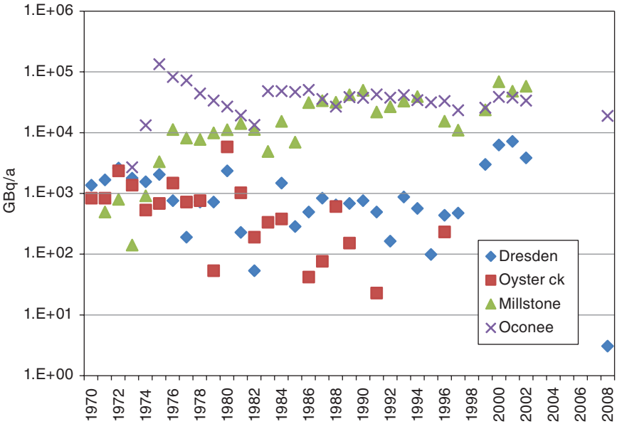
FIGURE 2.11 Variation of annual tritium releases in liquid effluents from selected nuclear plants. SOURCE: Data from UNSCEAR.
