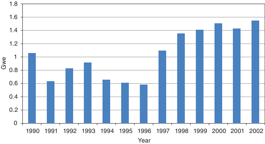
FIGURE 2.7 Variation with time of the electricity generated by the Dresden plant. SOURCE: UNSCEAR (2008).
