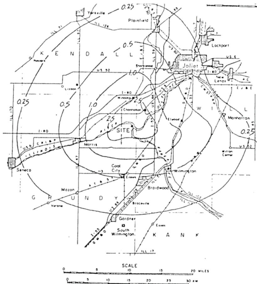
FIGURE 3.6 Calculated annual dose contours (rem) for 1975 at the Dresden plant from airborne effluent releases for comparison with the average wind rose (Figure 3.4). SOURCE: Commonwealth Edison (1976).
