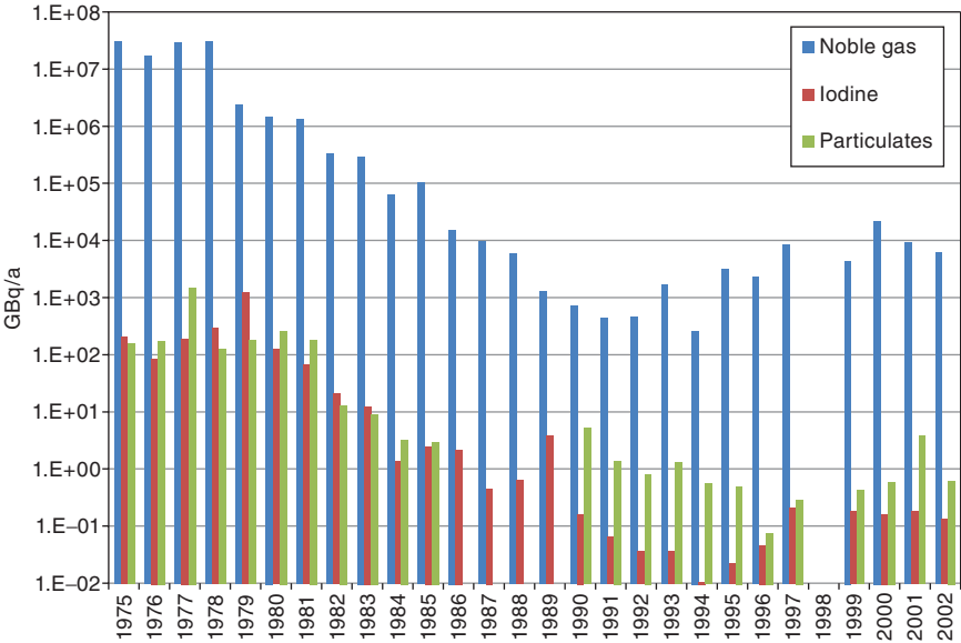
FIGURE 2.6 Comparison of annual atmospheric releases of noble gases (blue bars), iodine-131 (red bars), and radioactive particulates (green bars) for the Dresden plant from 1975 to 2002. The units on the vertical scale are in GBq (=0.03 Ci). SOURCE: Data from UNSCEAR.
