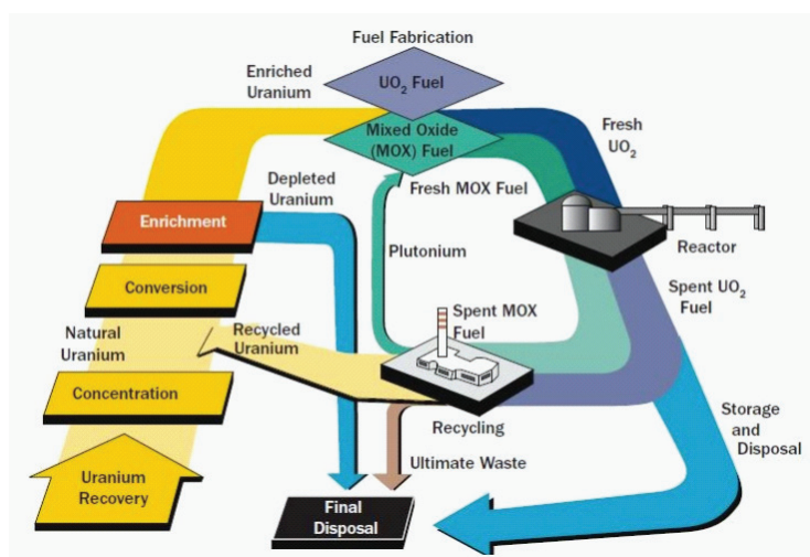
FIGURE S.1 Schematic depiction of the nuclear fuel cycle. SOURCE: USNRC.
