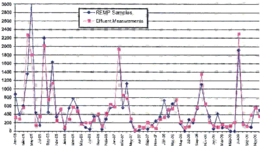
FIGURE 2.14 Five-year comparison between liquid effluent monitoring data and environmental monitoring data for tritium at location 32-I at the Millstone Plant. SOURCE: Dominion Nuclear Connecticut, Inc. (2010).
