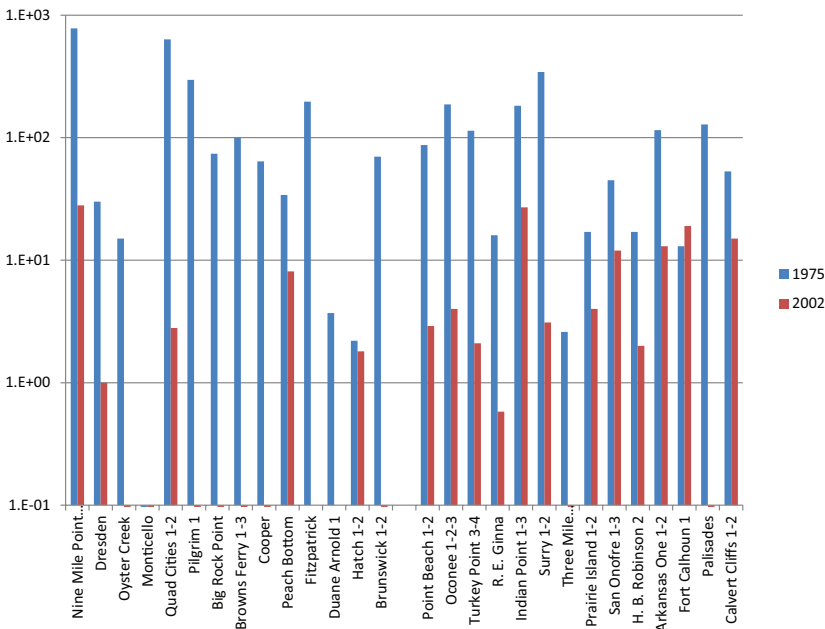
FIGURE 2.9 Comparison of liquid radioactive effluent releases, excluding tritium, for selected BWRs (left) and PWRs (right) in 1975 and 2002. SOURCE: Data from UNSCEAR.
