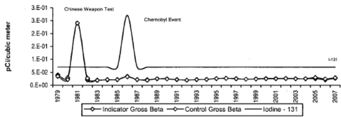
FIGURE 2.12 Measurements of gross beta and iodine-131 activity in air samples at the Fermi plant (located in Michigan) from 1979 to 2007. The measurements are sensitive enough to detect air emissions from Chinese nuclear weapons testing in the early 1980s and the Chernobyl accident in 1986. SOURCE: Detroit Edison (2007).
