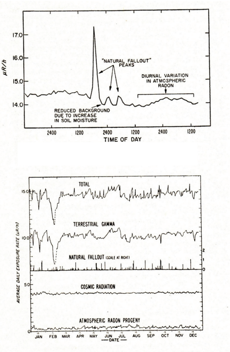
FIGURE 3.7 Daily variations in background radiation for a site in New Jersey. SOURCE: Beck and Miller (1982).
