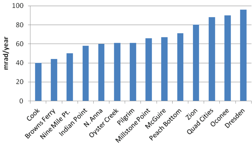
FIGURE 3.8 Variation in annual terrestrial free-in-air terrestrial and cosmic-ray natural background doses for selected facilities. SOURCE: TLD data from 2008-2009 radiological environmental monitoring reports for the plants shown in the figure.
