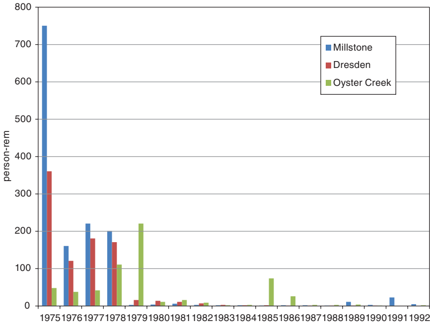
FIGURE 3.3 Collective doses to populations living between 2 and 80 km from the Millstone, Dresden, and Oyster Creek plants, 1975-1992. SOURCE: NUREG/CR-2850 (PNL-4221), vol. 1-14.
