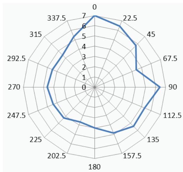
FIGURE 3.5 Annual wind rose for the Dresden plant for all stability classes and speeds combined at the height of the plant stack. The concentric lines indicate the percent time (from 0 to 7 percent) the wind was blowing. The radial lines show the compass direction that the wind was blowing. SOURCE: Commonwealth Edison (1976).
