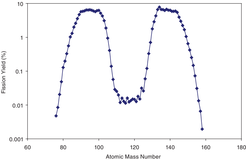
FIGURE D.1 Mass distributions resulting from fission of uranium-235 by thermal neutrons. SOURCE: Data from Joint Evaluated Fission and Fusion File, Incident-neutron data, http://www-nds.iaea.org/exfor/endf00.htm , October 2, 2006; see http://www-nds.iaea.org/sgnucdat/c1.htm .
