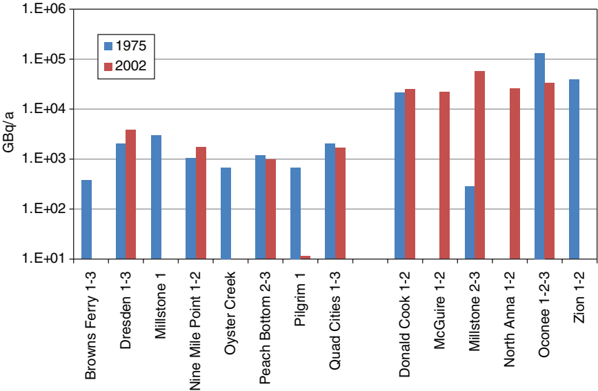
FIGURE 2.10 Tritium released in liquid effluents for selected nuclear plants (left, BWRs; right, PWRs) in 1975 and 2002. NOTE: The North Anna and McGuire plants were not operational in 1975. SOURCE: Data from UNSCEAR.
