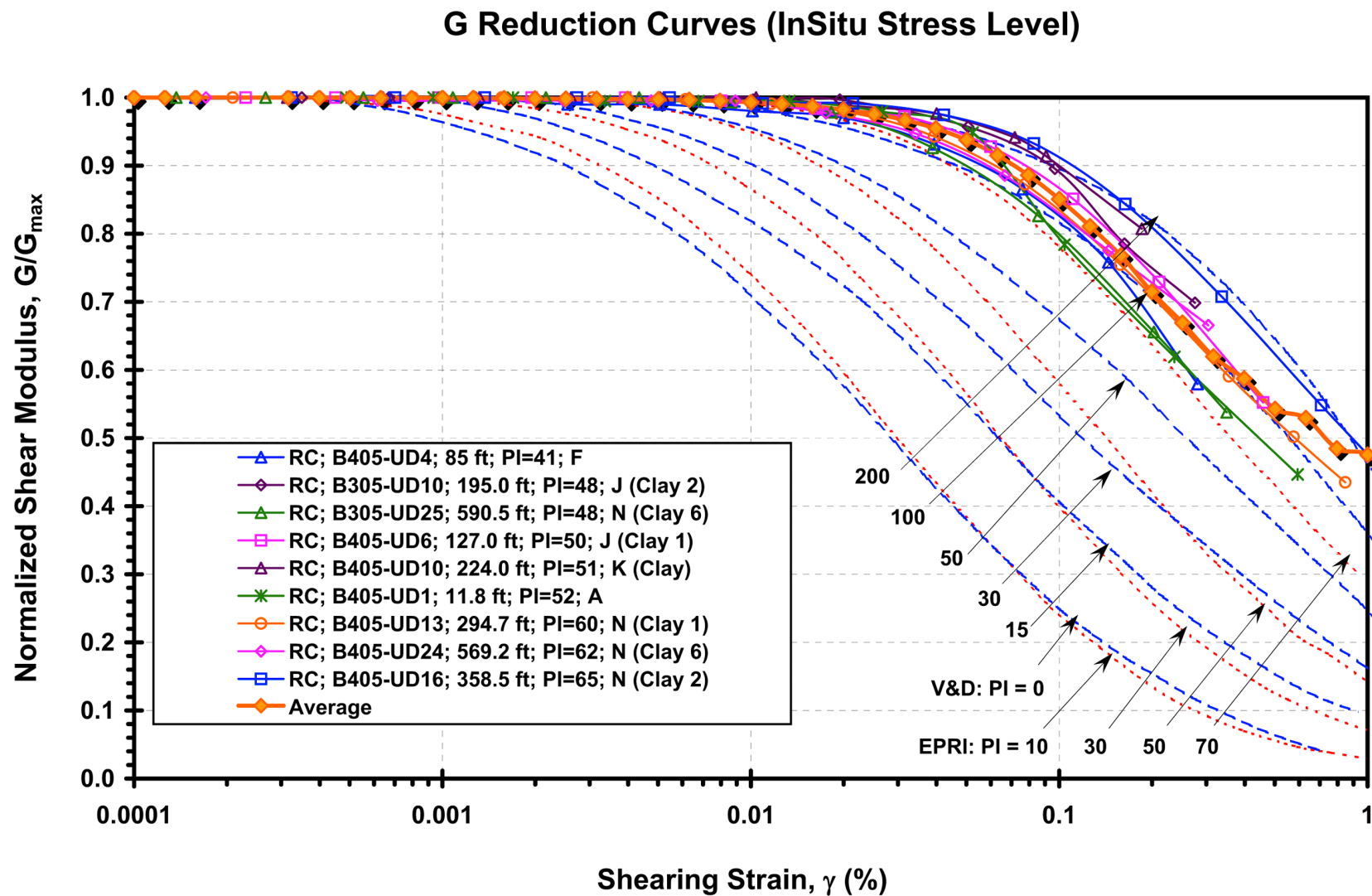
Figure 2.5S.4-64 Shear Modulus Degradation Based on RCTS Testing - High PI Clay Sample
