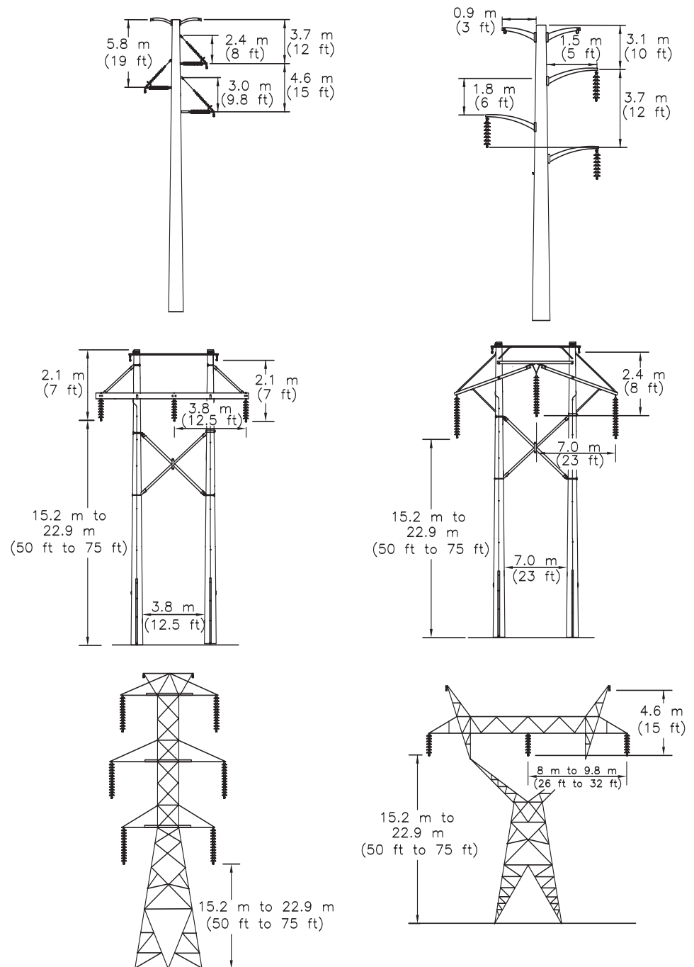
FIGURE 5.4: Examples of transmission structures.
