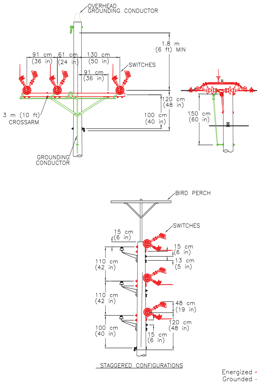
FIGURE 5.49: Pole-mounted switches.
