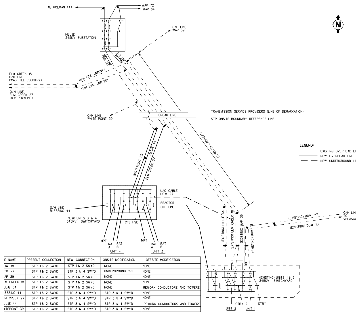
Figure 3.7-5 345kV Transmission Configuration for STP 1 &amp; 2 and STP 3 &amp; 4
