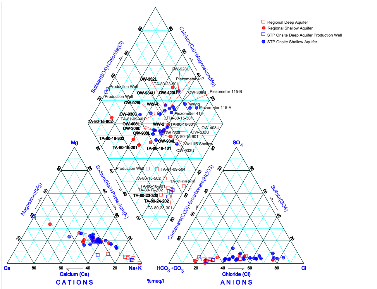
Figure 2.3.1-34 Trilinear Diagram of Hydrogeochemical Data
