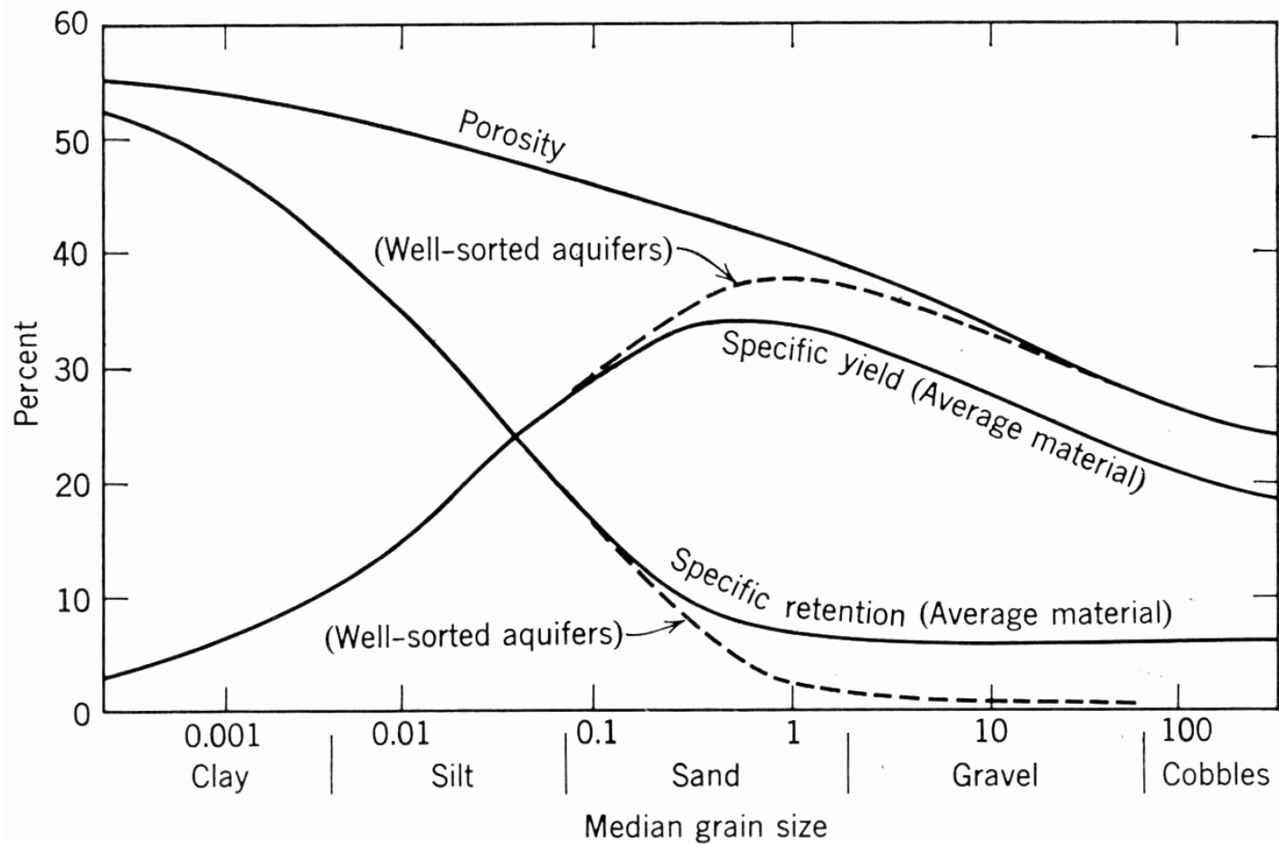
Figure 2.3.1-33 Relationship of Porosity, Specific Yield, and Specific Retention (Reference 2.3.1-28)
