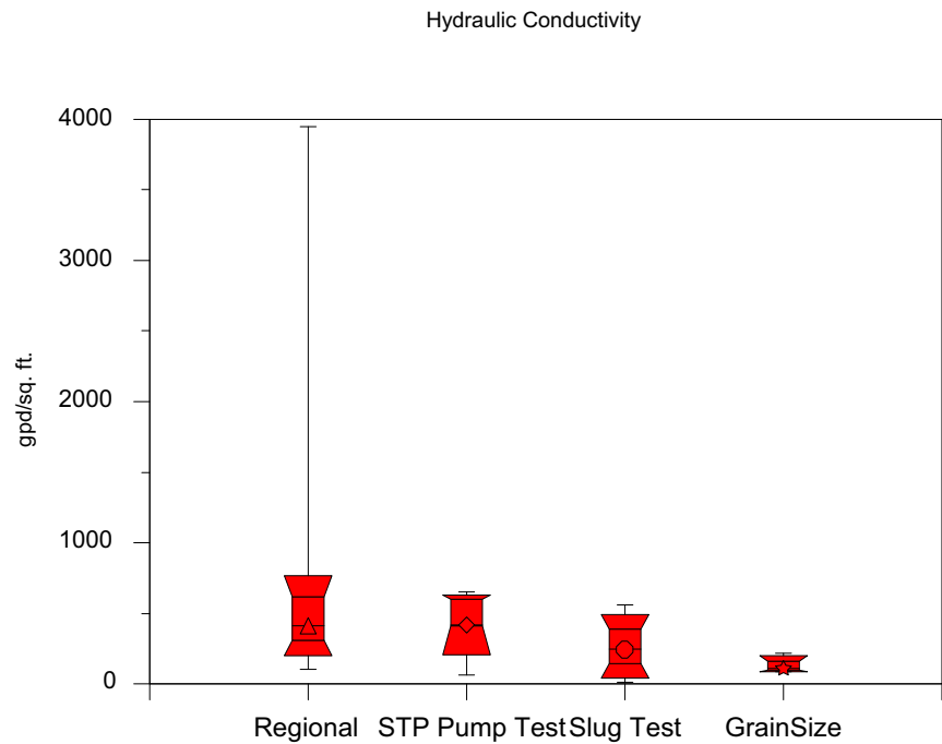
Figure 2.3.1-32 Summary of Hydraulic Conductivity from Aquifer Pumping Tests, Slug Tests, and Grain Size
