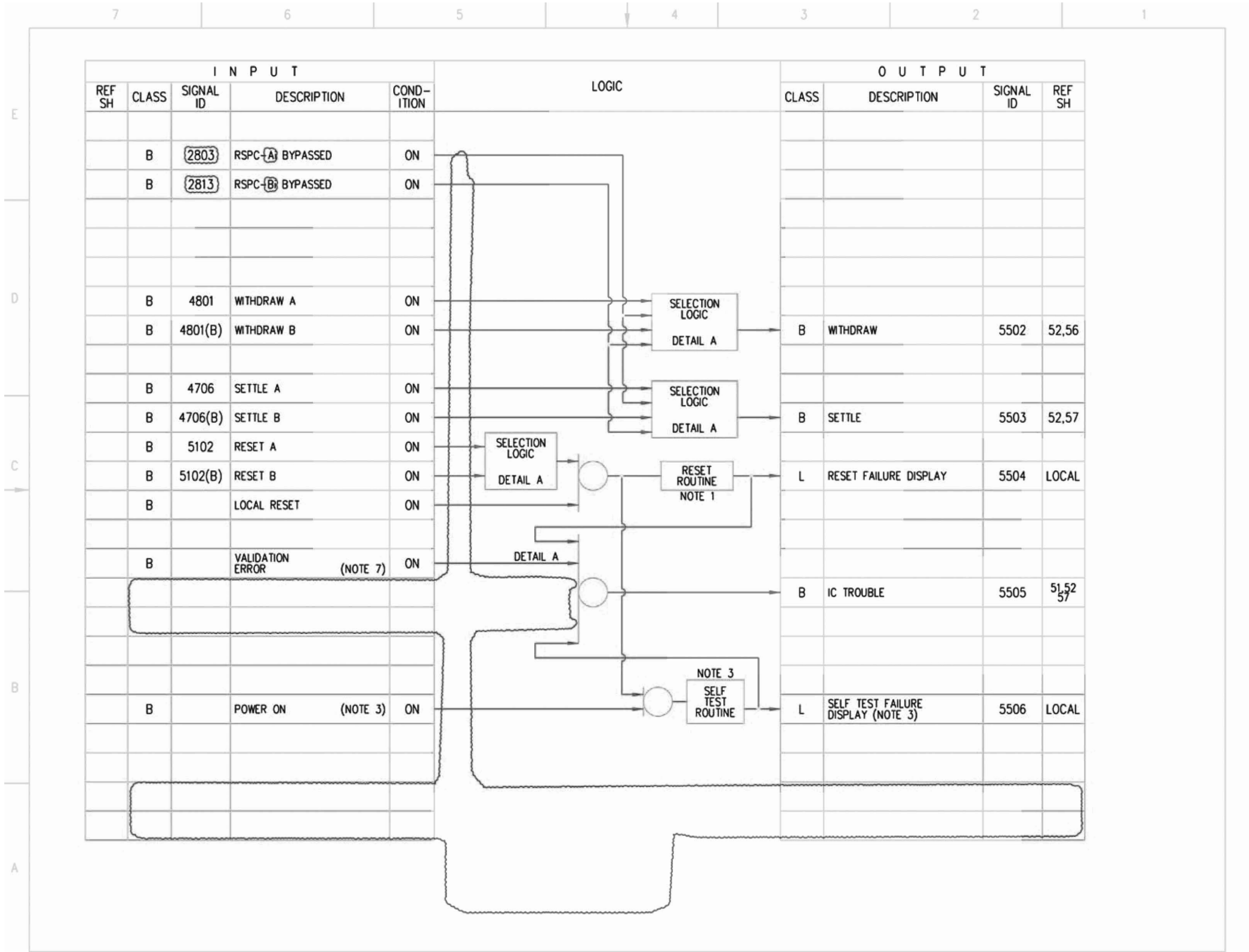
Figure 7.7-3 – Rod Control and Information System IBD (Sheet 55 of 87)
