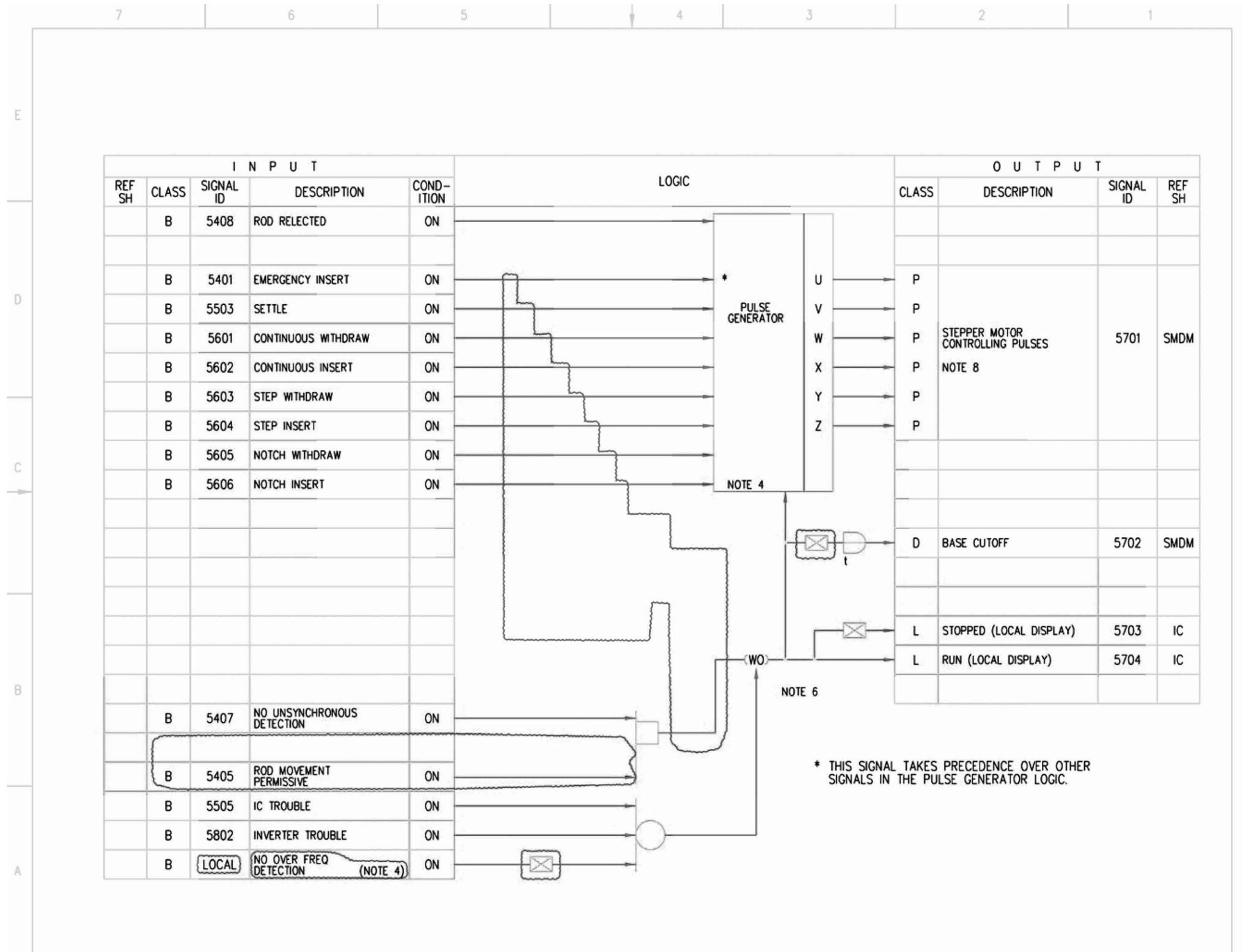
Figure 7.7-3 – Rod Control and Information System IBD (Sheet 57 of 87)
