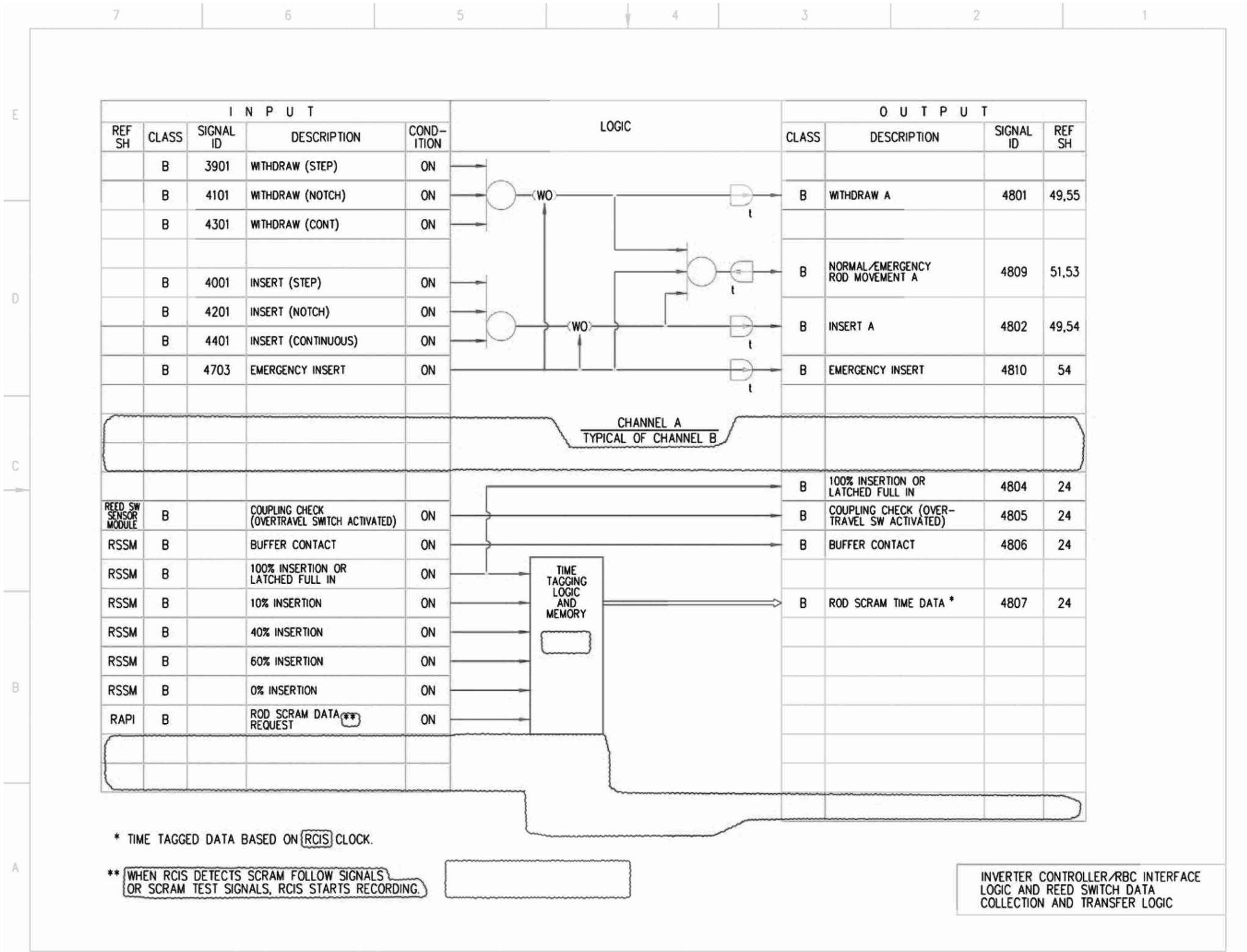
Figure 7.7-3 – Rod Control and Information System IBD (Sheet 48 of 87)
