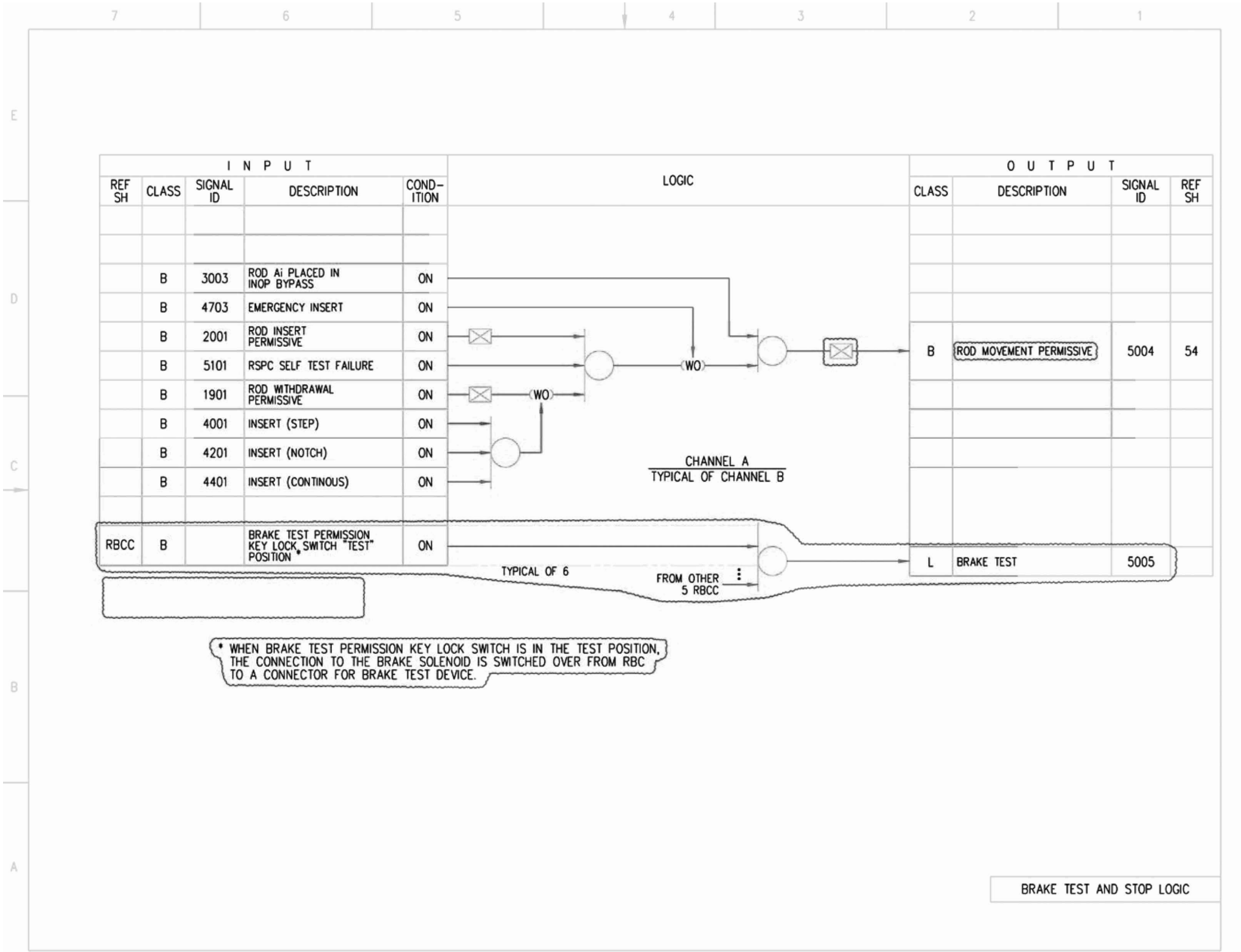
Figure 7.7-3 – Rod Control and Information System IBD (Sheet 50 of 87)
