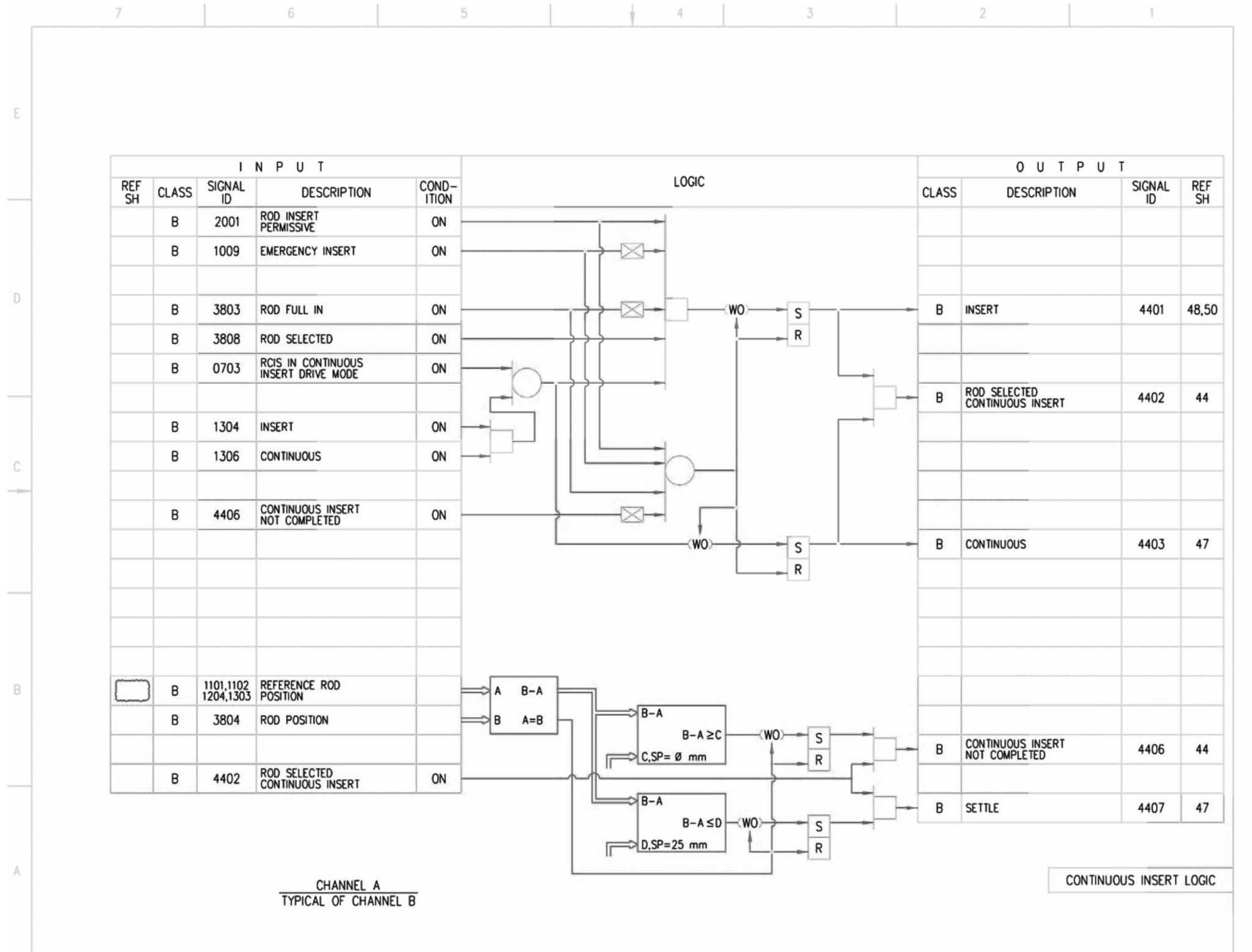
Figure 7.7-3 – Rod Control and Information System IBD (Sheet 44 of 87)
