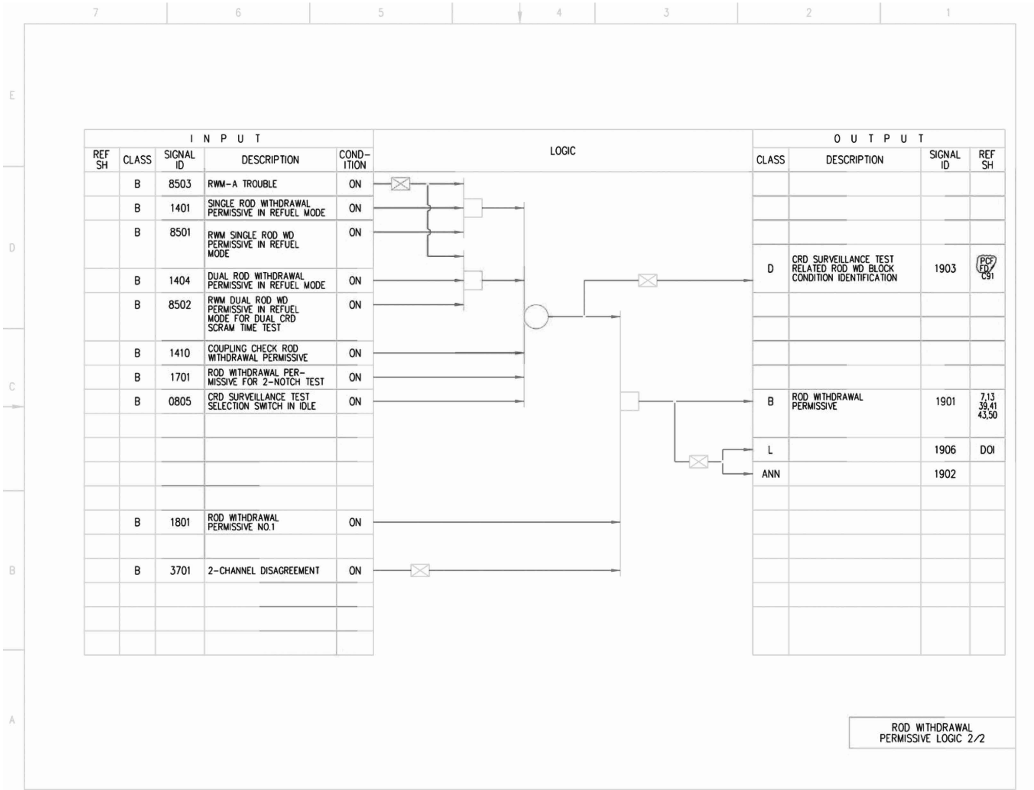
Figure 7.7-3 – Rod Control and Information System IBD (Sheet 19 of 87)
