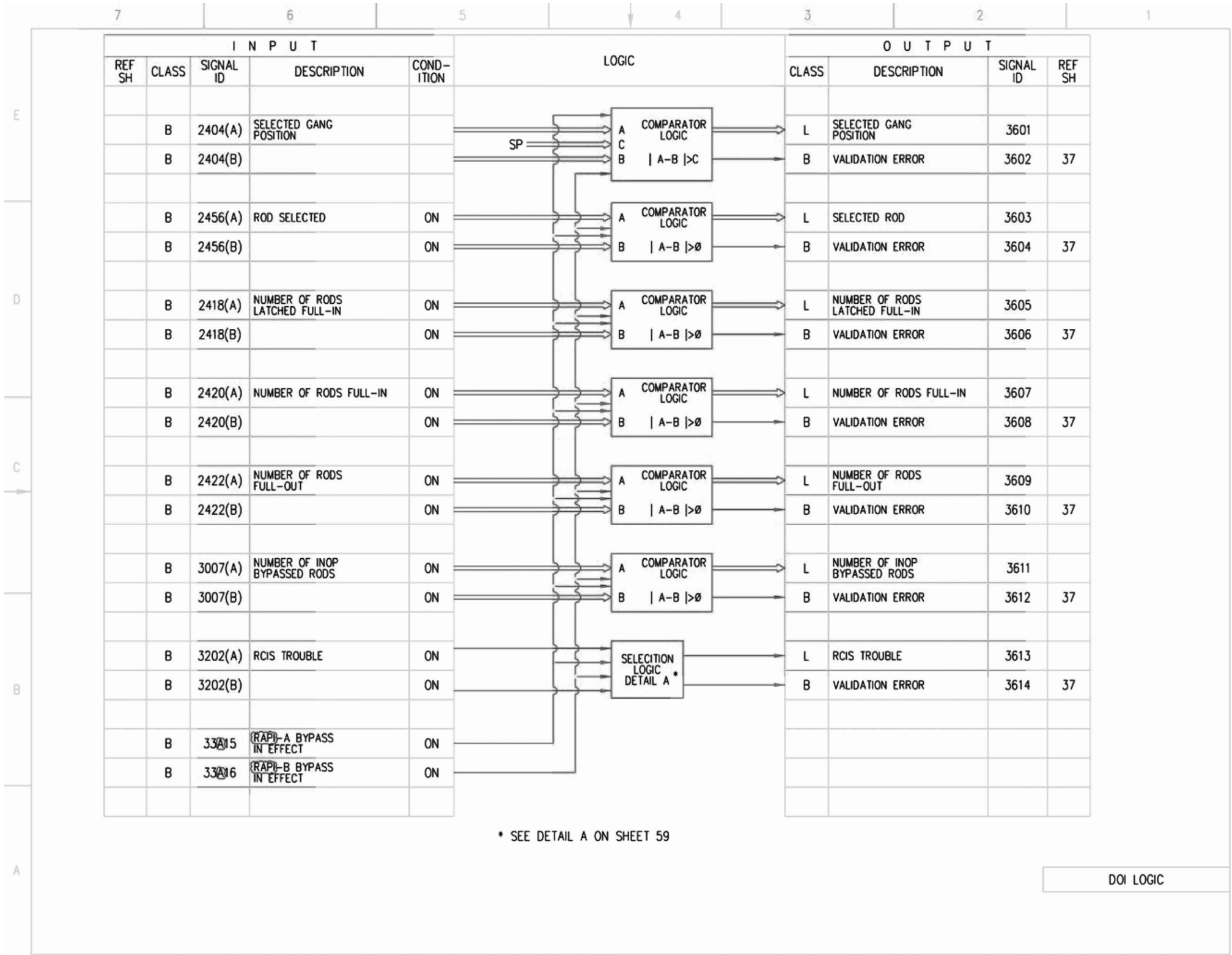
Figure 7.7-3 – Rod Control and Information System IBD (Sheet 36 of 87)
