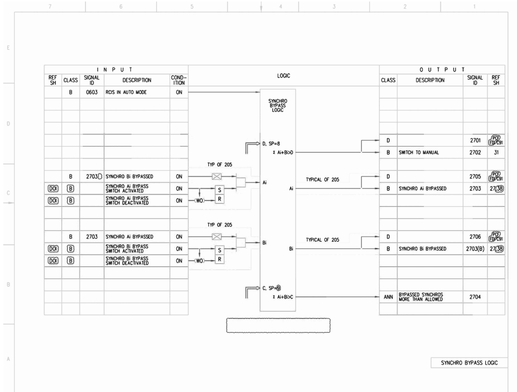
Figure 7.7-3 – Rod Control and Information System IBD (Sheet 27 of 87)
