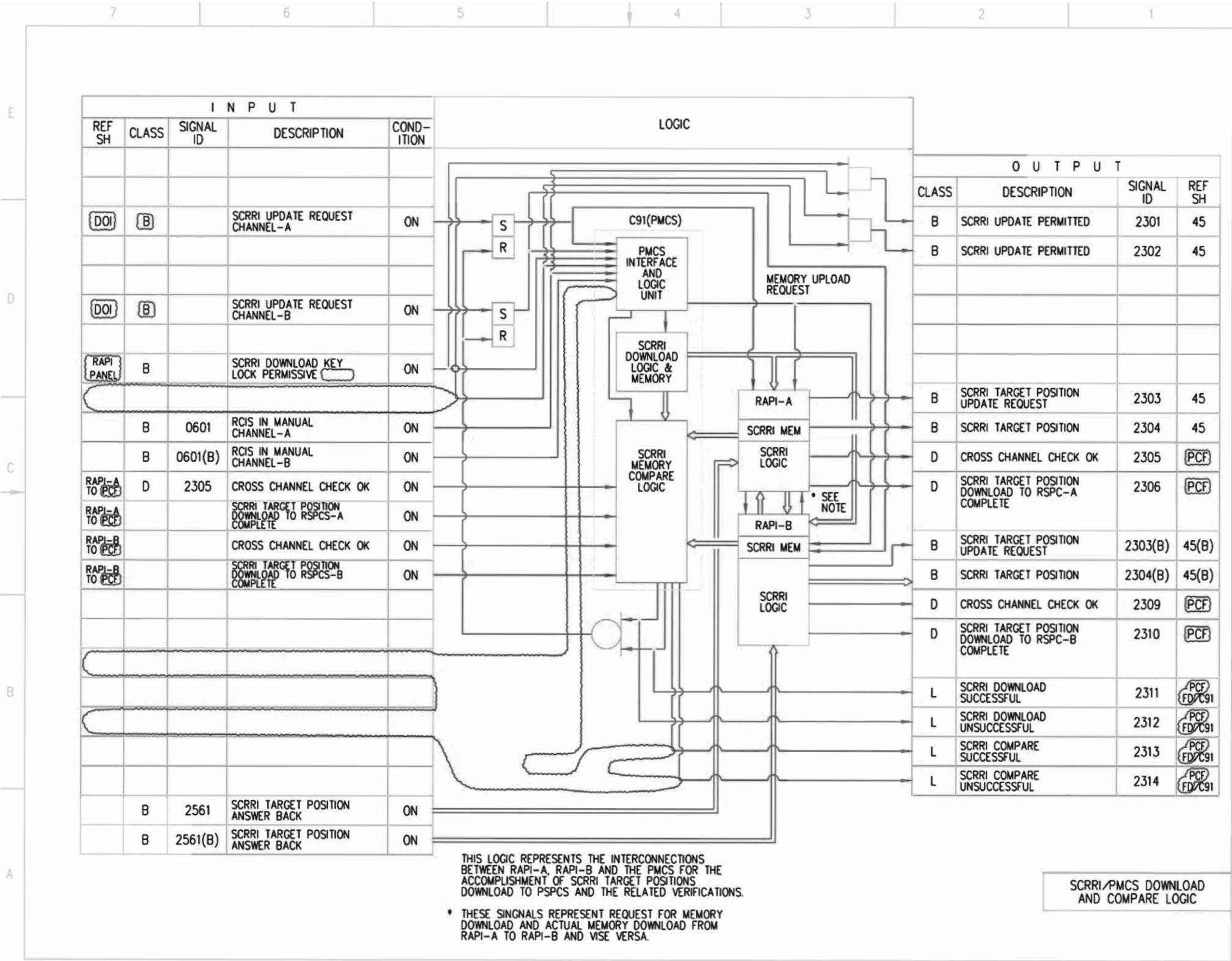
Figure 7.7-3 – Rod Control and Information System IBD (Sheet 23 of 87)
