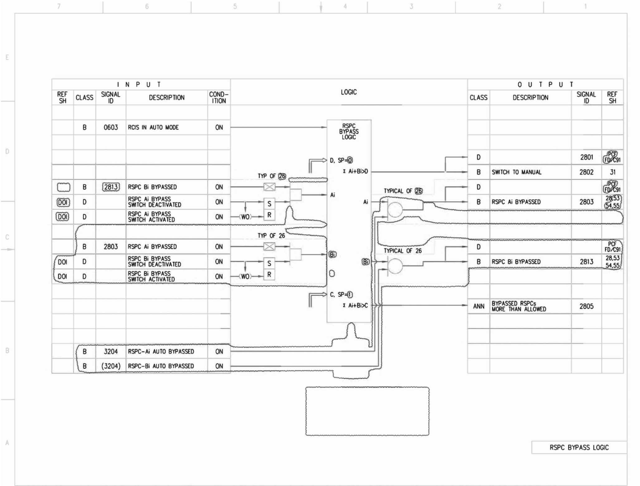
Figure 7.7-3 – Rod Control and Information System IBD (Sheet 28 of 87)
