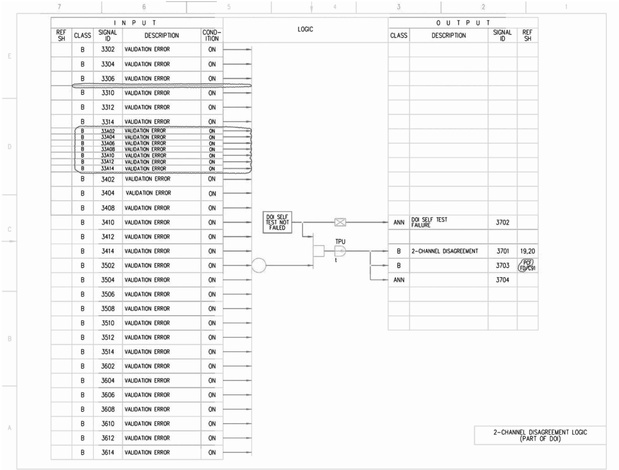
Figure 7.7-3 – Rod Control and Information System IBD (Sheet 37 of 87)
