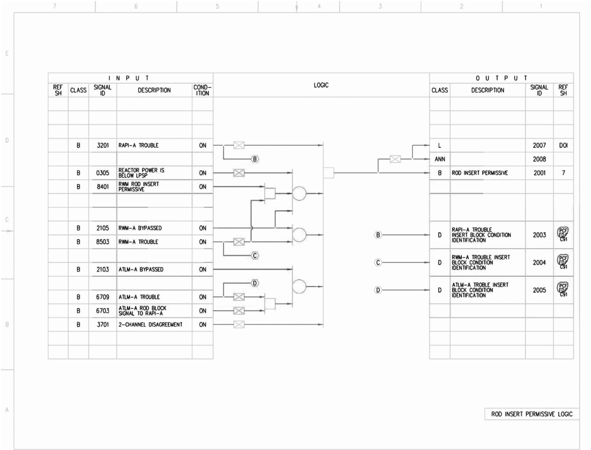
Figure 7.7-3 – Rod Control and Information System IBD (Sheet 20 of 87)
