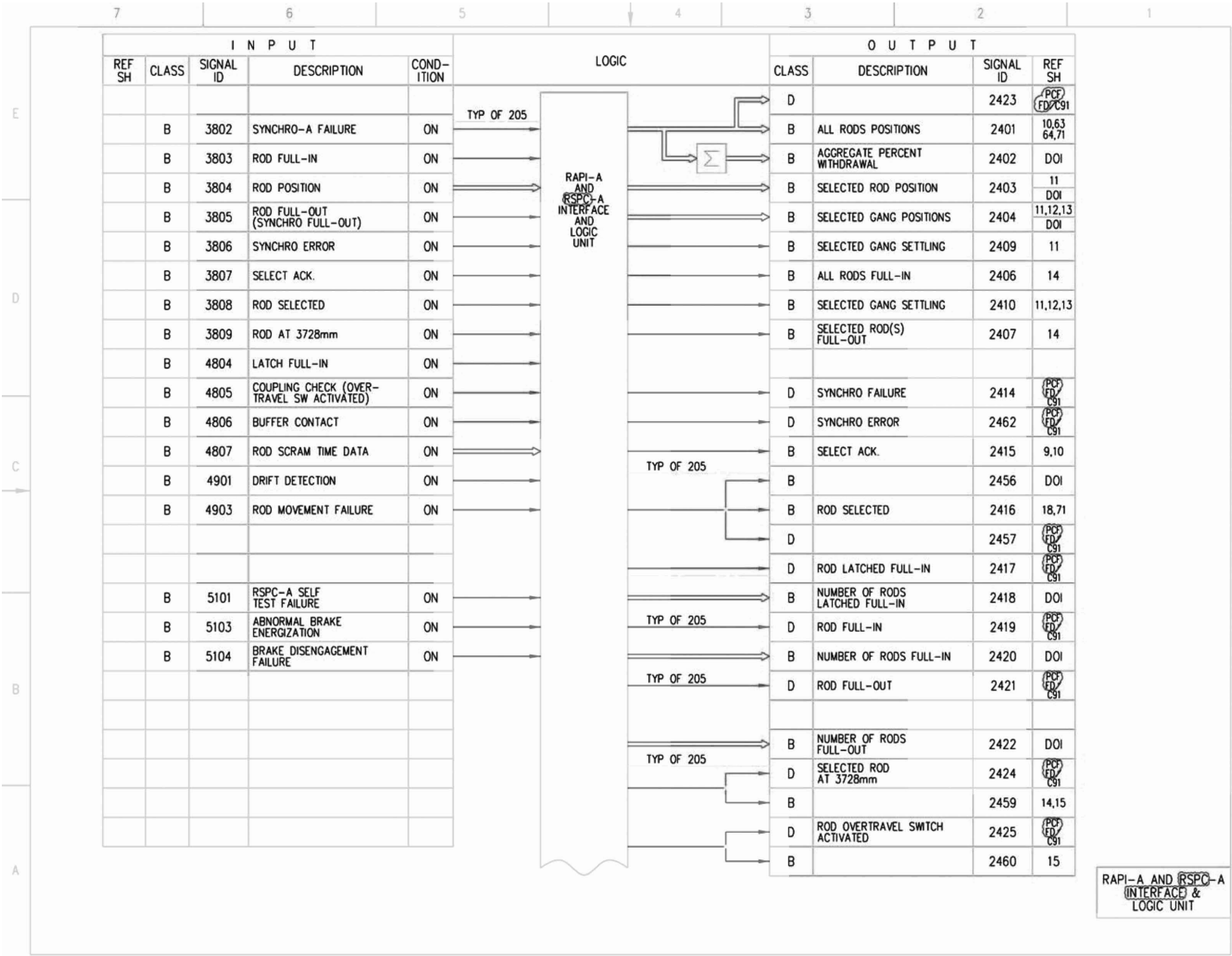
Figure 7.7-3 – Rod Control and Information System IBD (Sheet 24 of 87)
