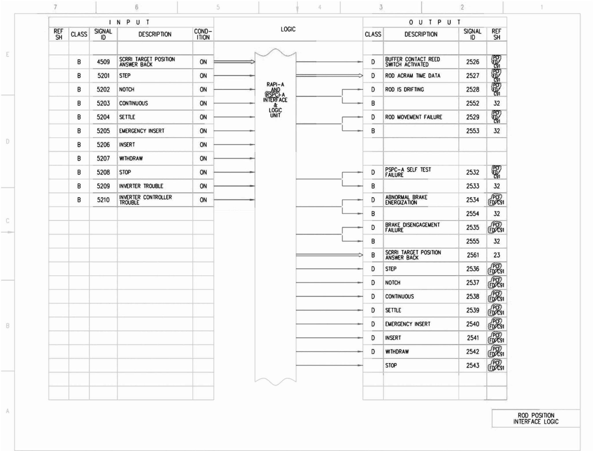
Figure 7.7-3 – Rod Control and Information System IBD (Sheet 25 of 87)
