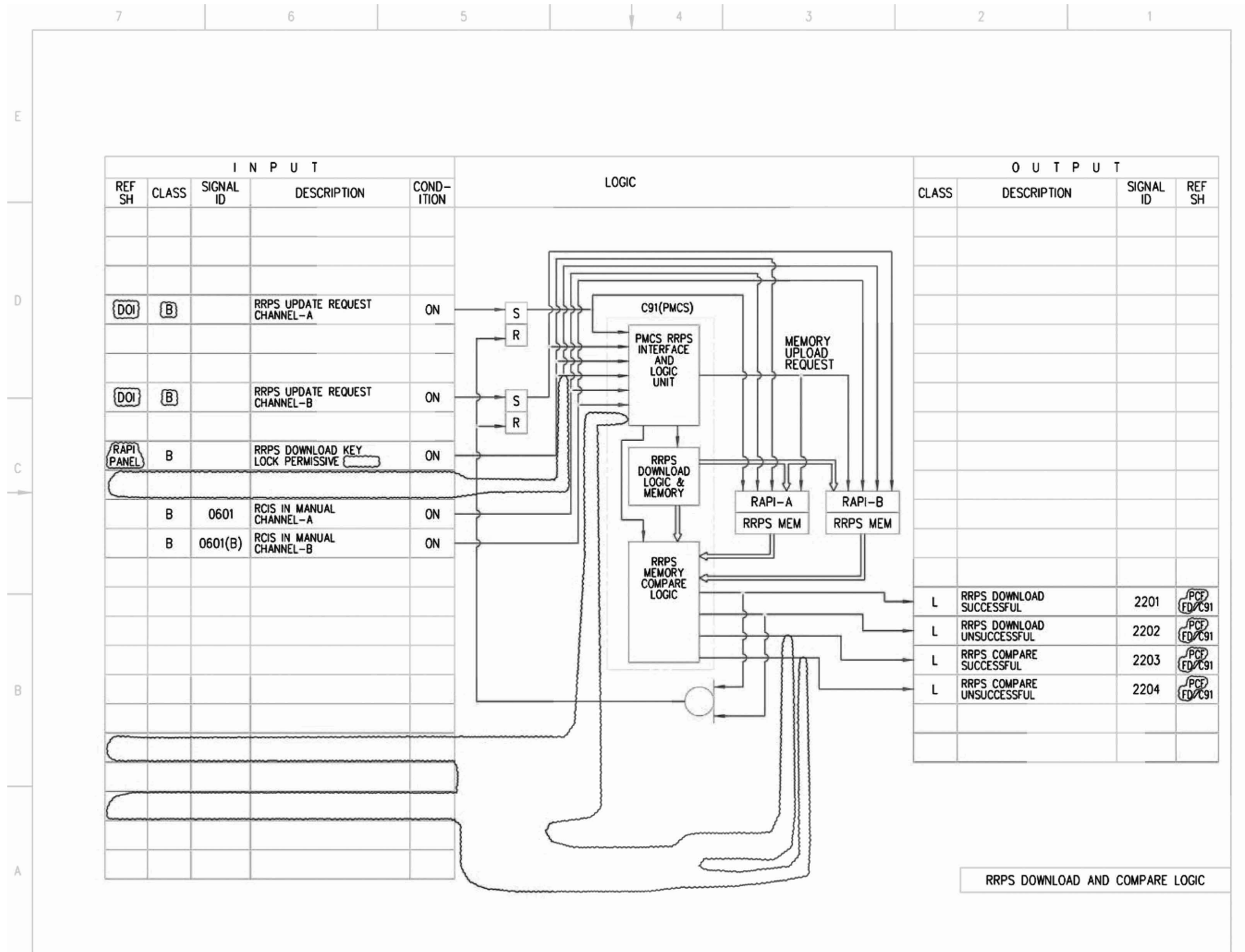
Figure 7.7-3 – Rod Control and Information System IBD (Sheet 22 of 87)
