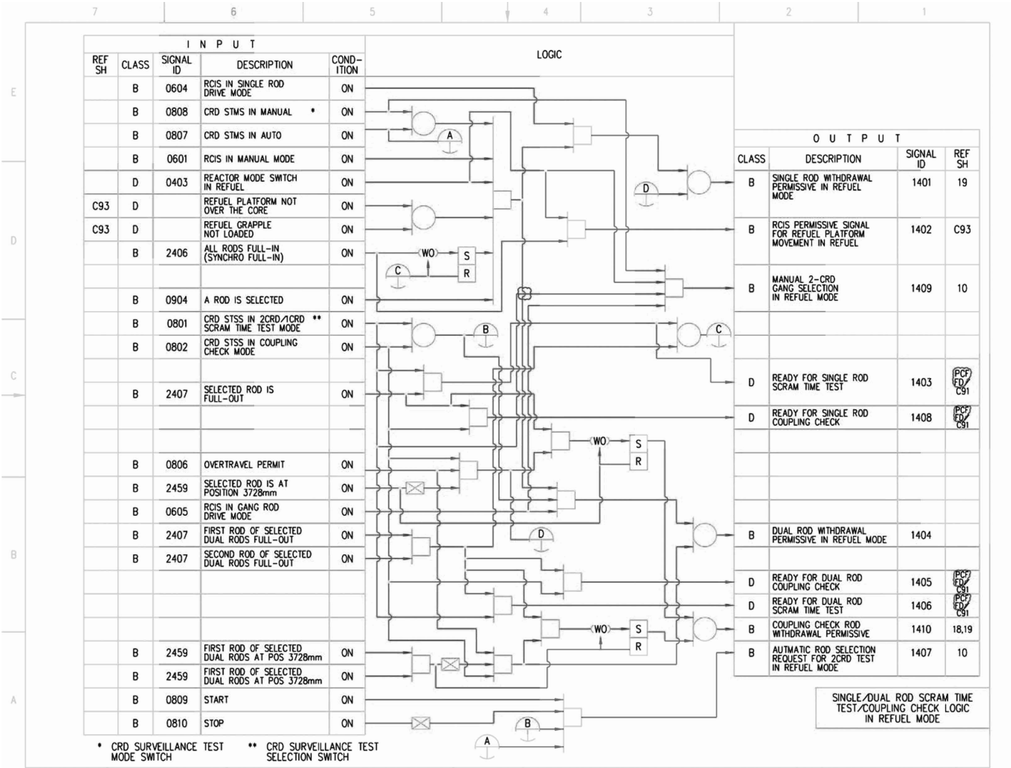
Figure 7.7-3 – Rod Control and Information System IBD (Sheet 14 of 87)
