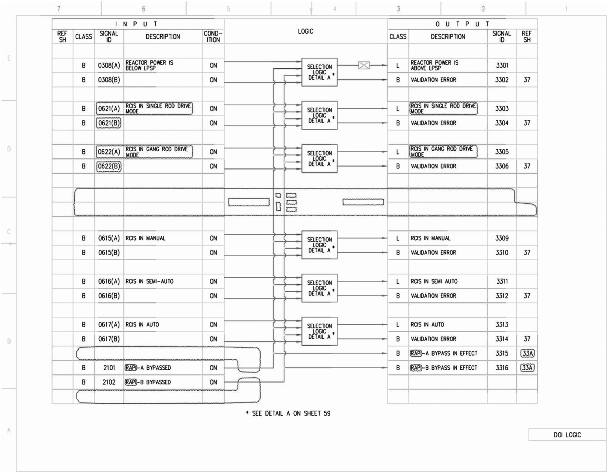
Figure 7.7-3 – Rod Control and Information System IBD (Sheet 33 of 87)
