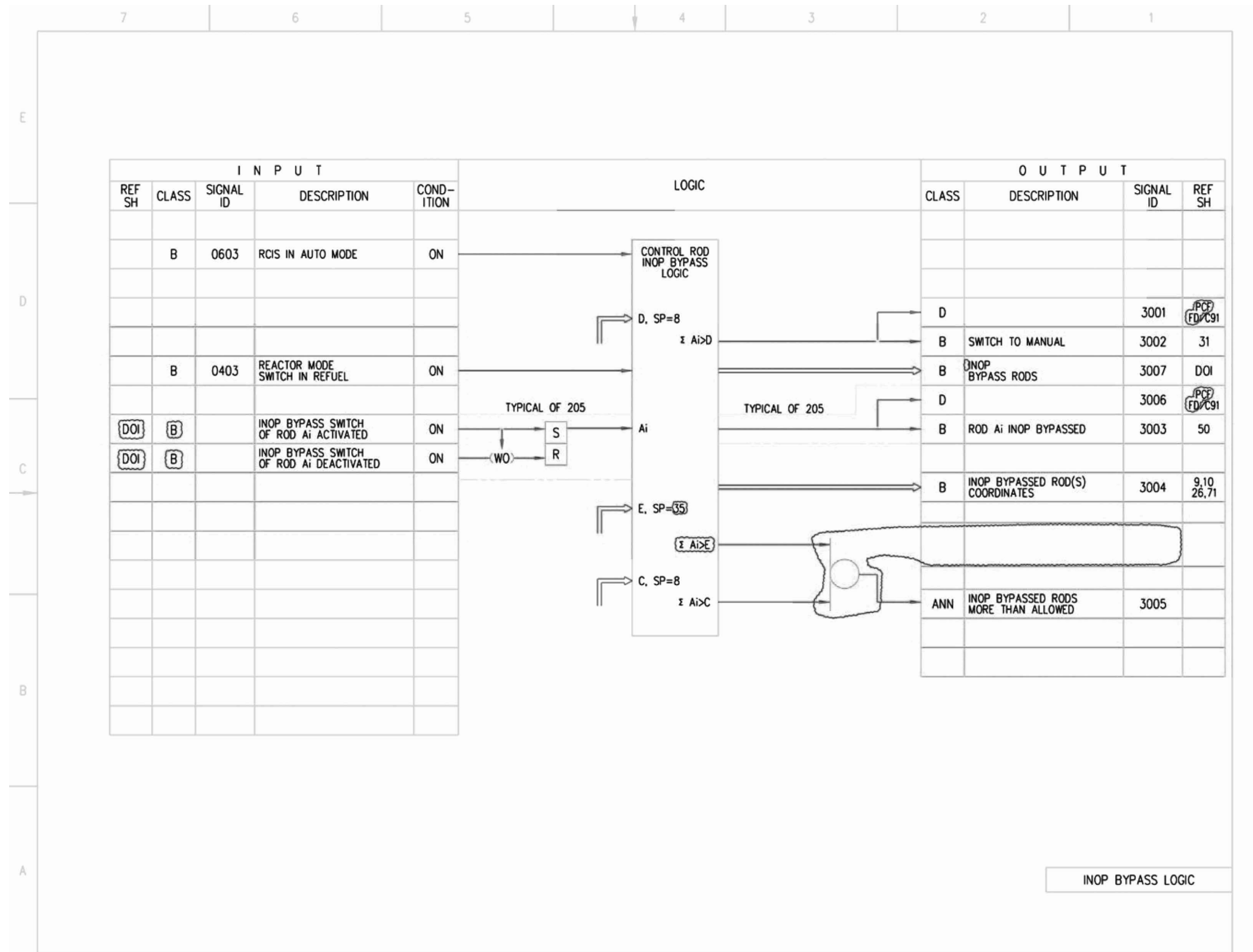
Figure 7.7-3 – Rod Control and Information System IBD (Sheet 30 of 87)
