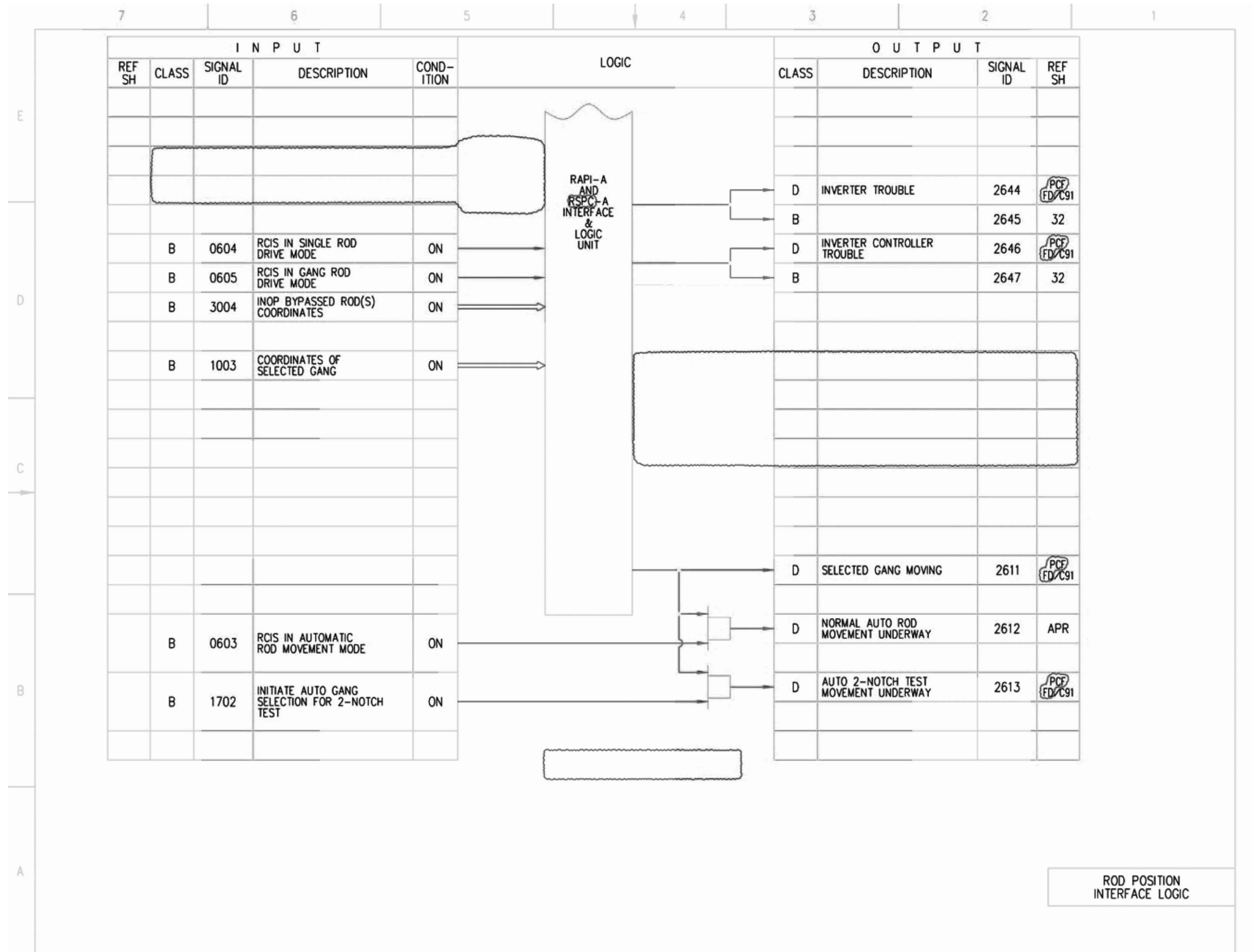
Figure 7.7-3 – Rod Control and Information System IBD (Sheet 26 of 87)
