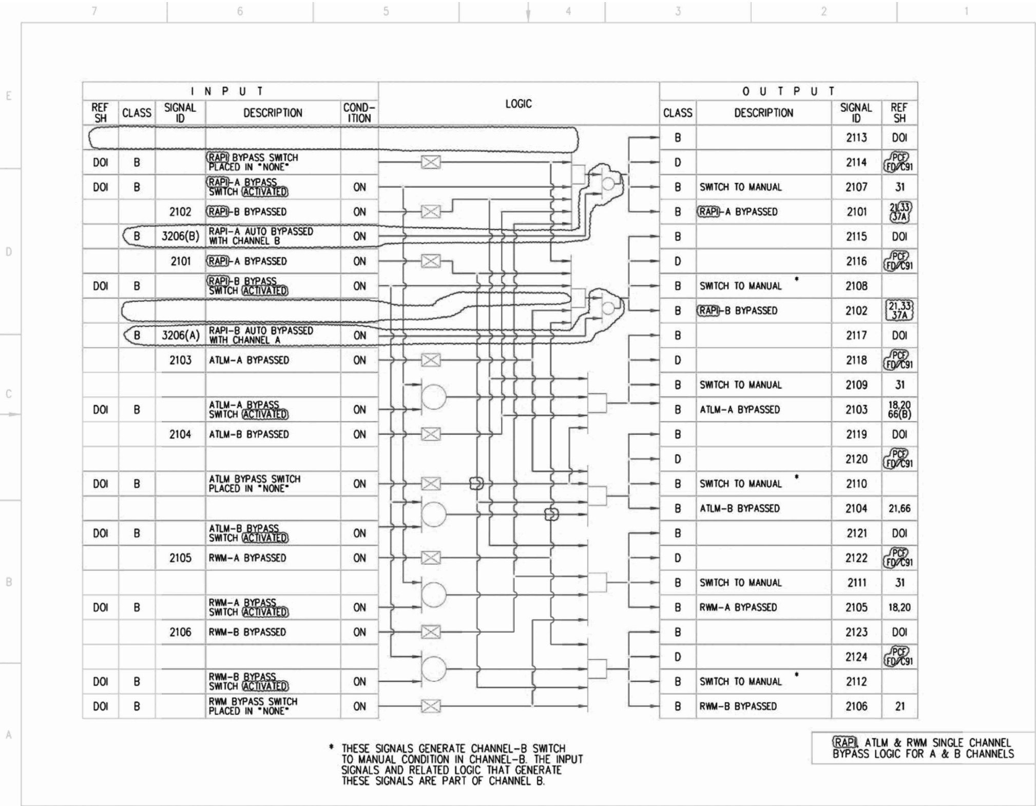
Figure 7.7-3 – Rod Control and Information System IBD (Sheet 21 of 87)
