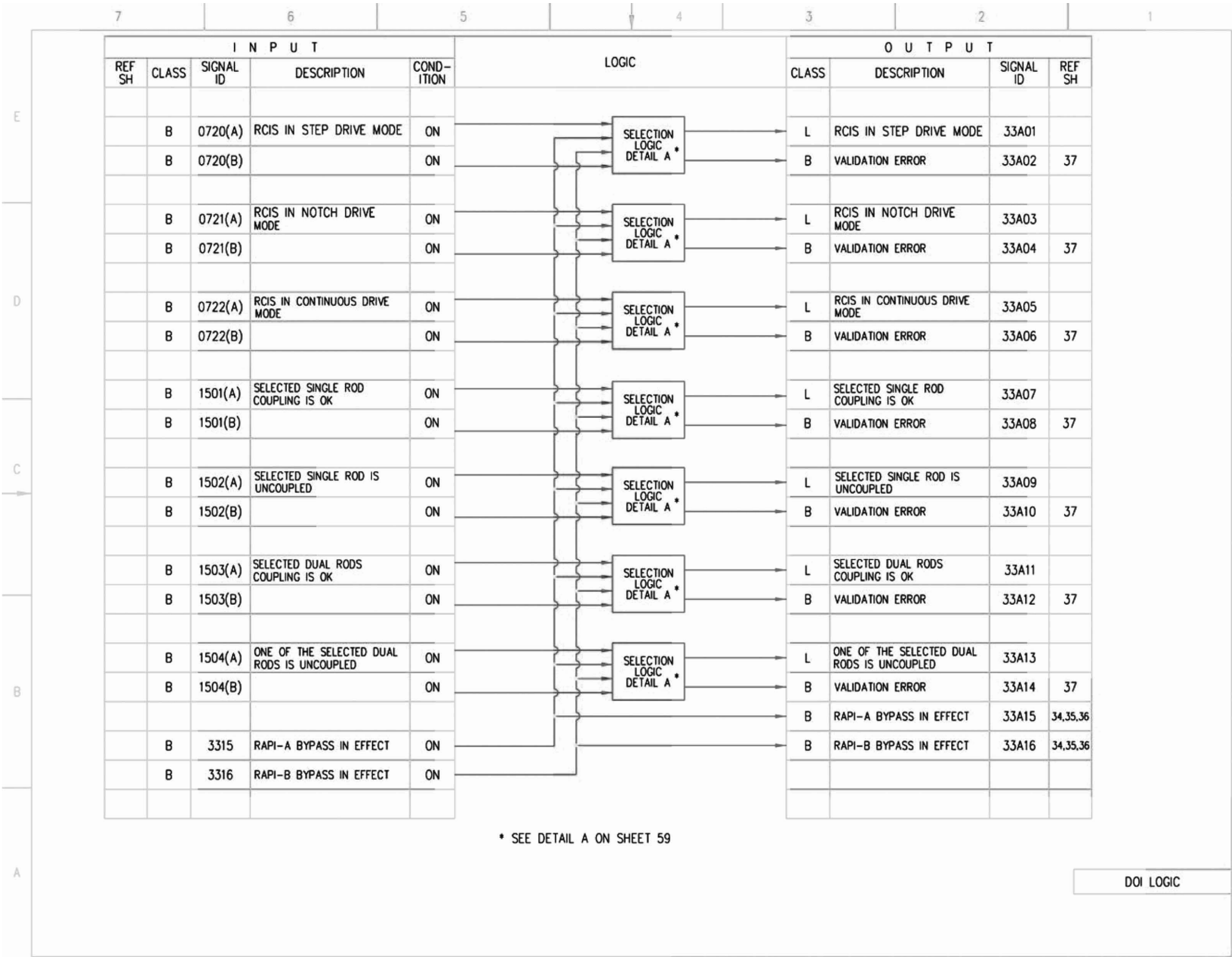
Figure 7.7-3 – Rod Control and Information System IBD (Sheet 33a of 87)
