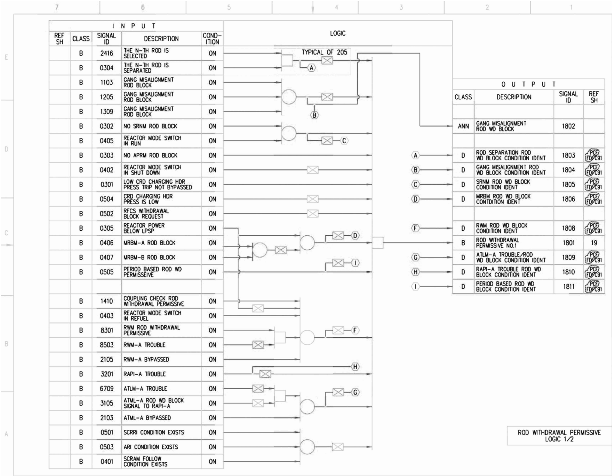
Figure 7.7-3 – Rod Control and Information System IBD (Sheet 18 of 87)
