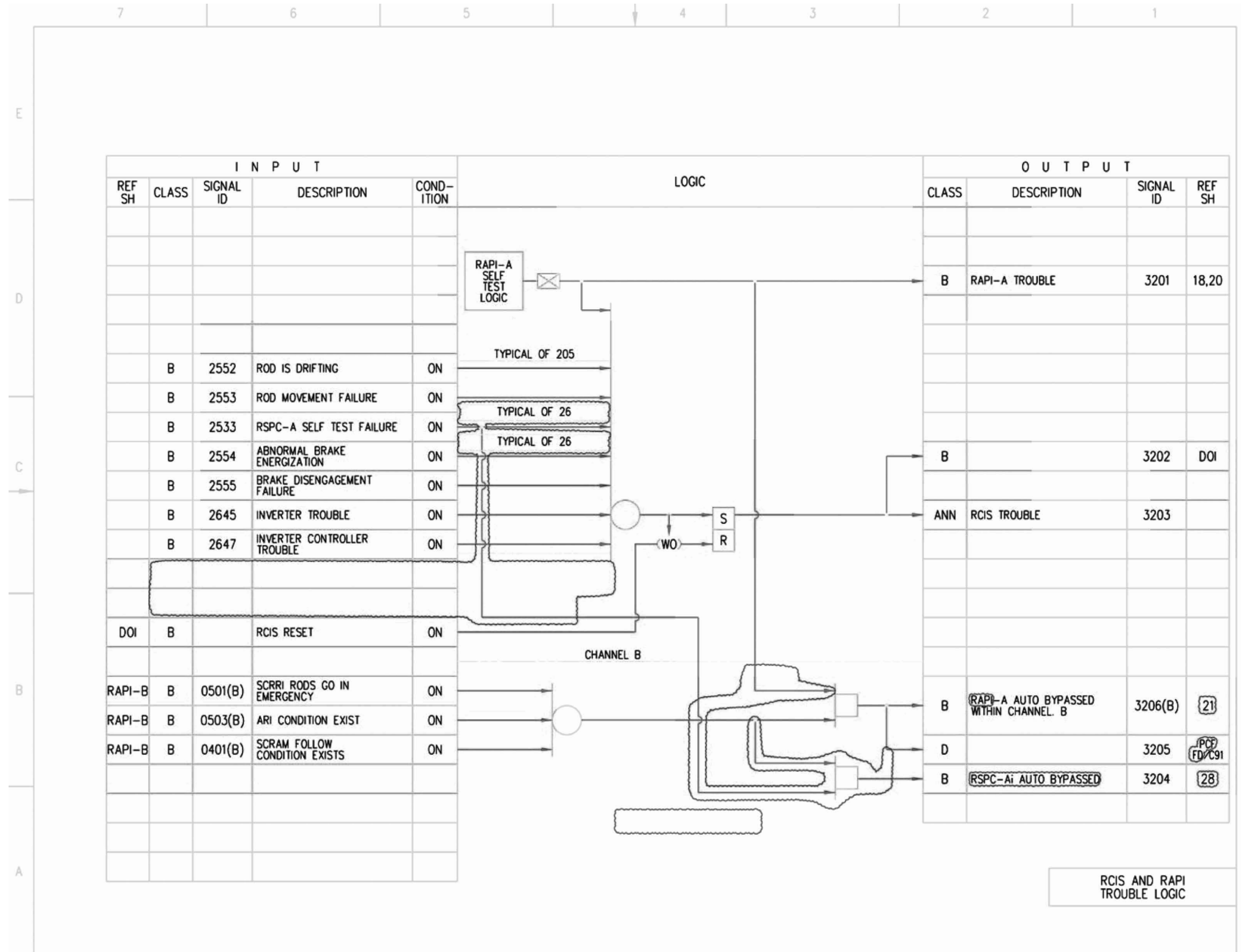
Figure 7.7-3 – Rod Control and Information System IBD (Sheet 32 of 87)
