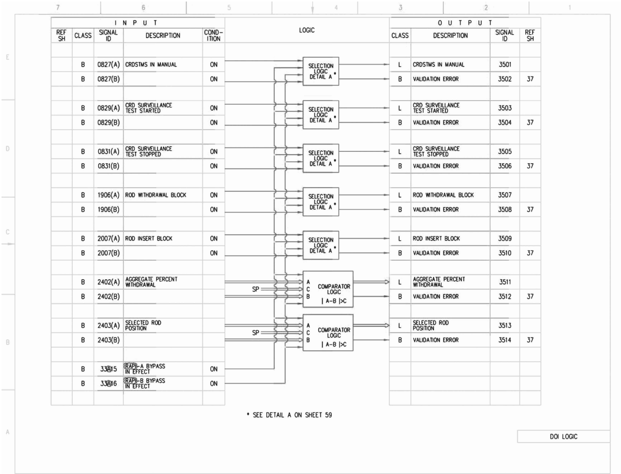
Figure 7.7-3 – Rod Control and Information System IBD (Sheet 35 of 87)
