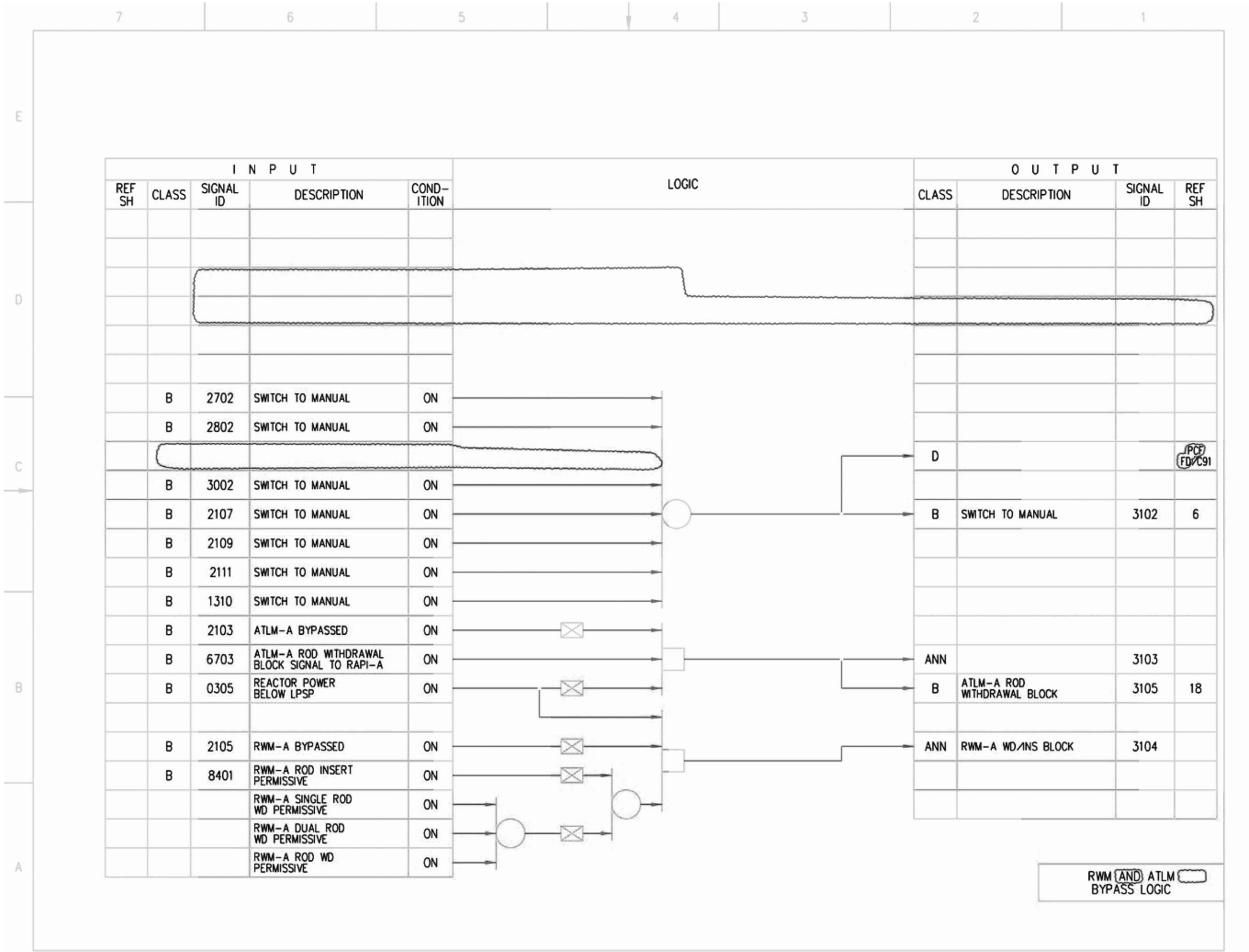
Figure 7.7-3 – Rod Control and Information System IBD (Sheet 31 of 87)
