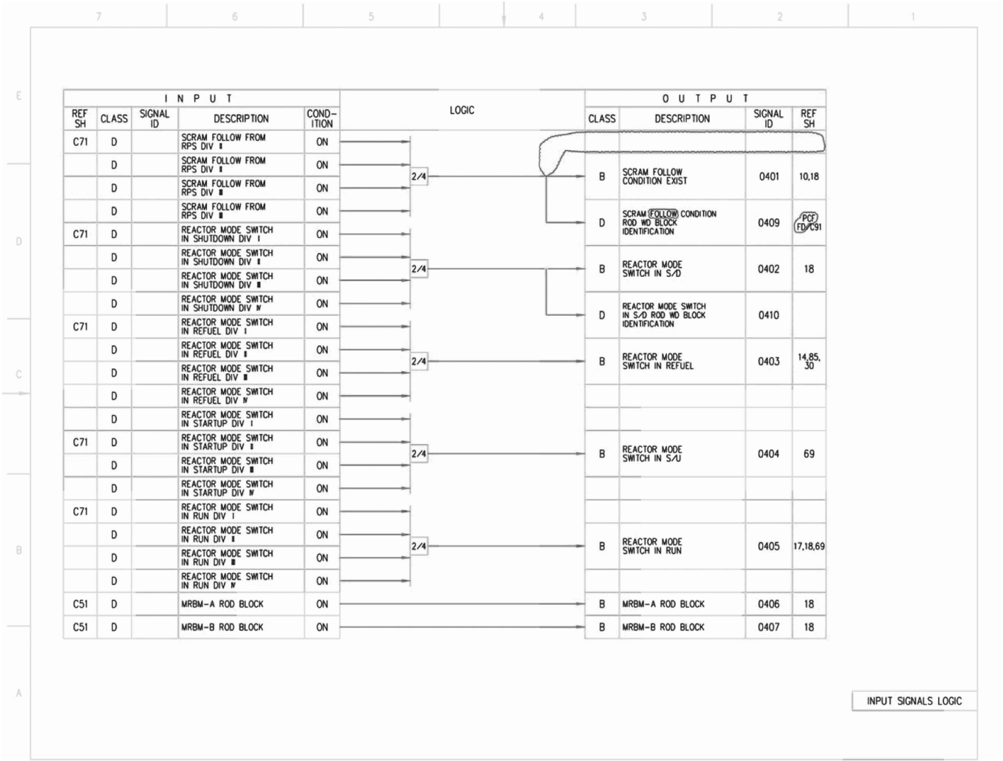
Figure 7.7-3 – Rod Control and Information System IBD (Sheet 4 of 87)
