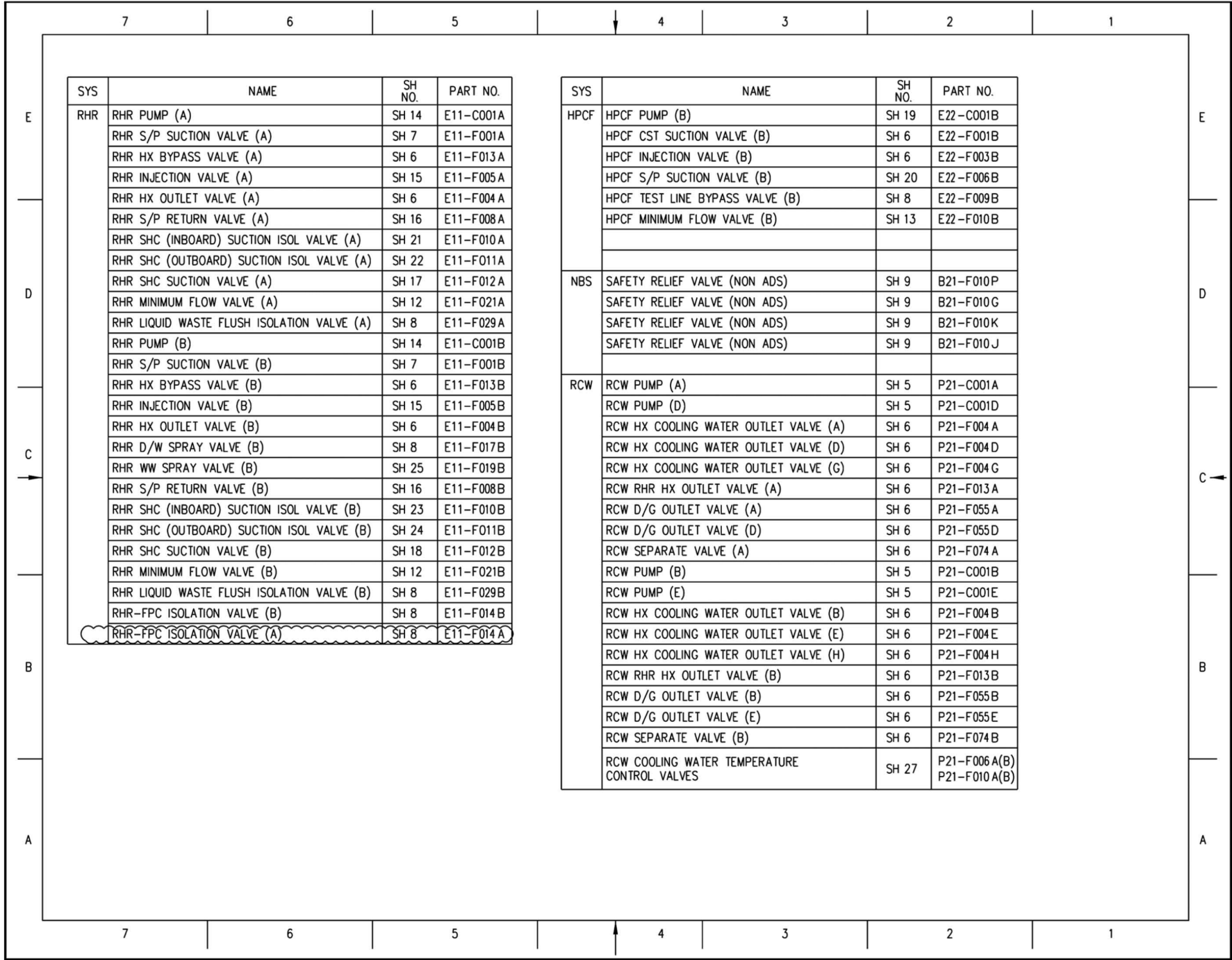
Figure 7.4-3 – Remote Shutdown System IBD (Sheet 2 of 27)
