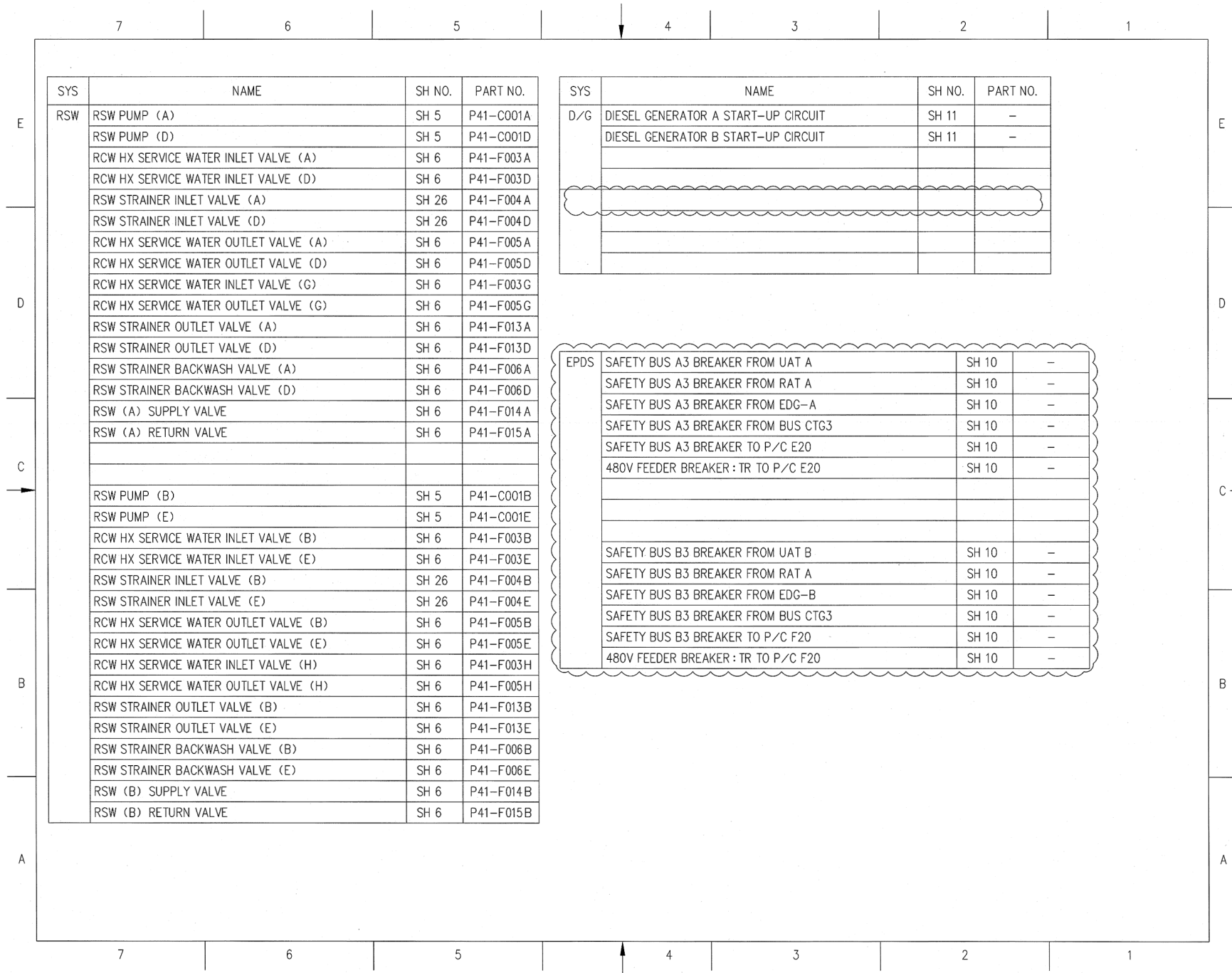
Figure 7.4-3 – Remote Shutdown System IBD (Sheet 3 of 27)
