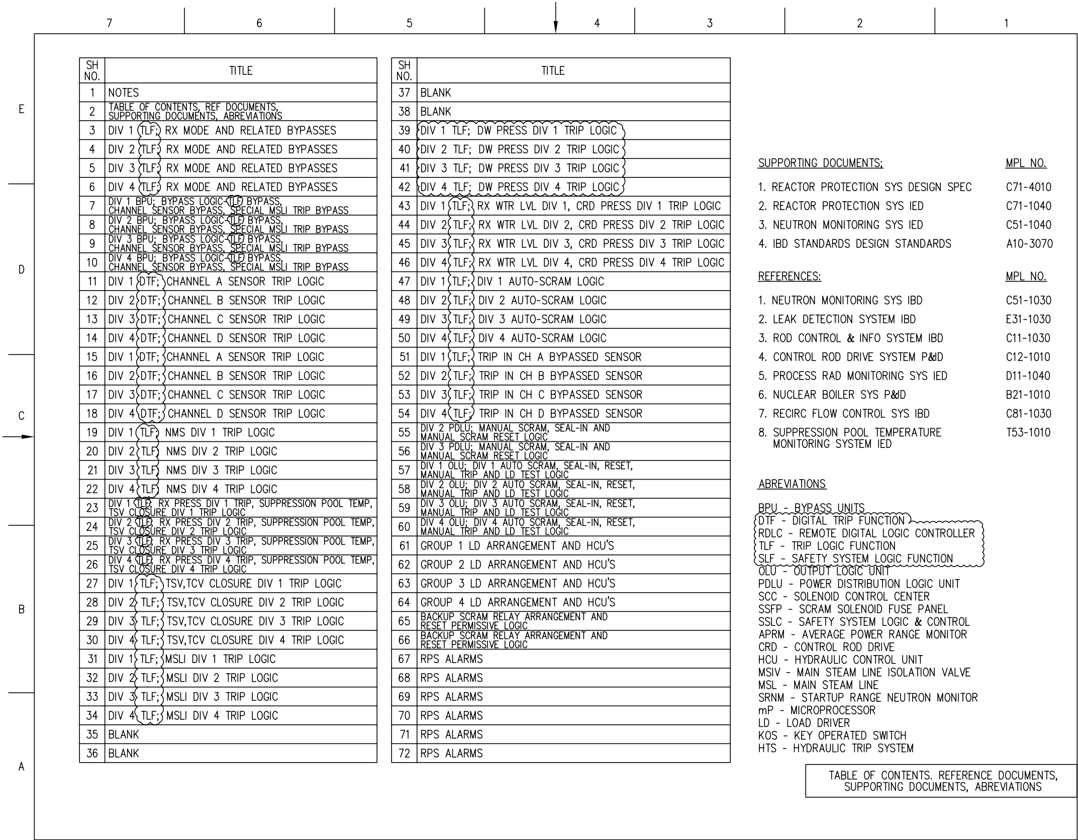
Figure 7.2-10 – Reactor Protection System IBD (Sheet 2 of 72)
