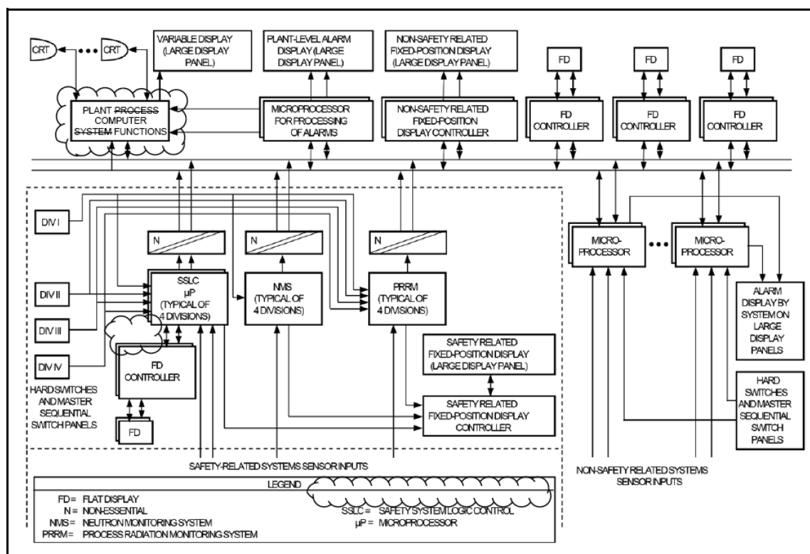
Figure 18C-8 Overall Configuration of Operator Interface System
