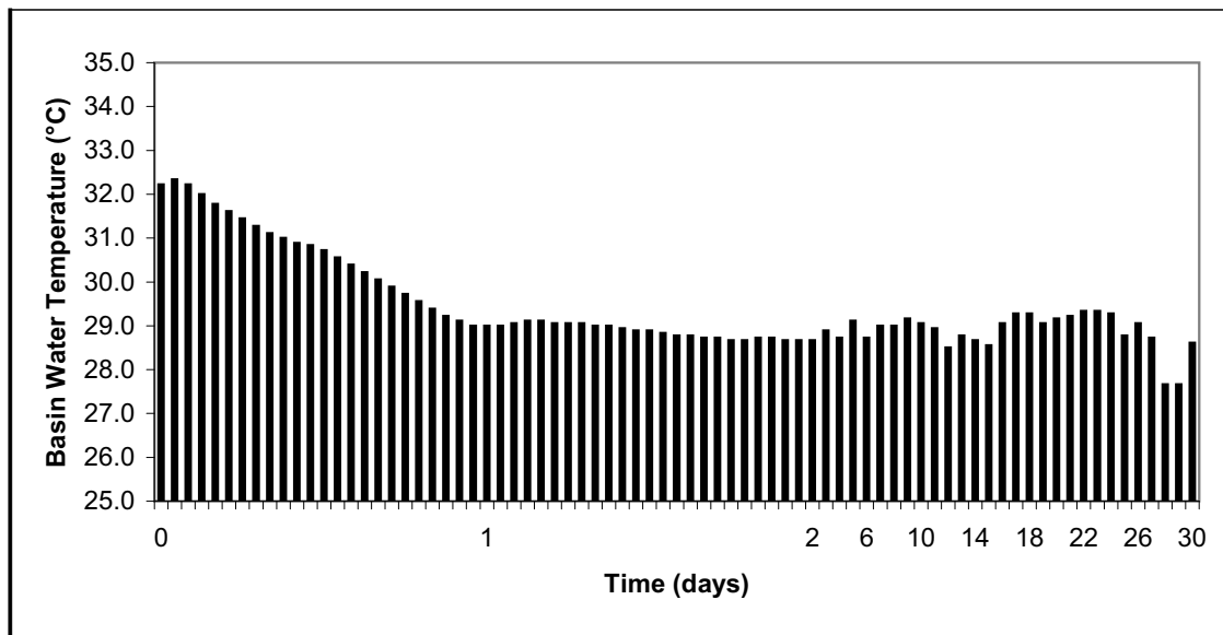
Figure 9.2-17 UHS Basin Water Maximum Temperature (Case D2)
