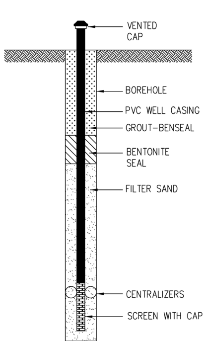
PIEZOMETER DETAIL
