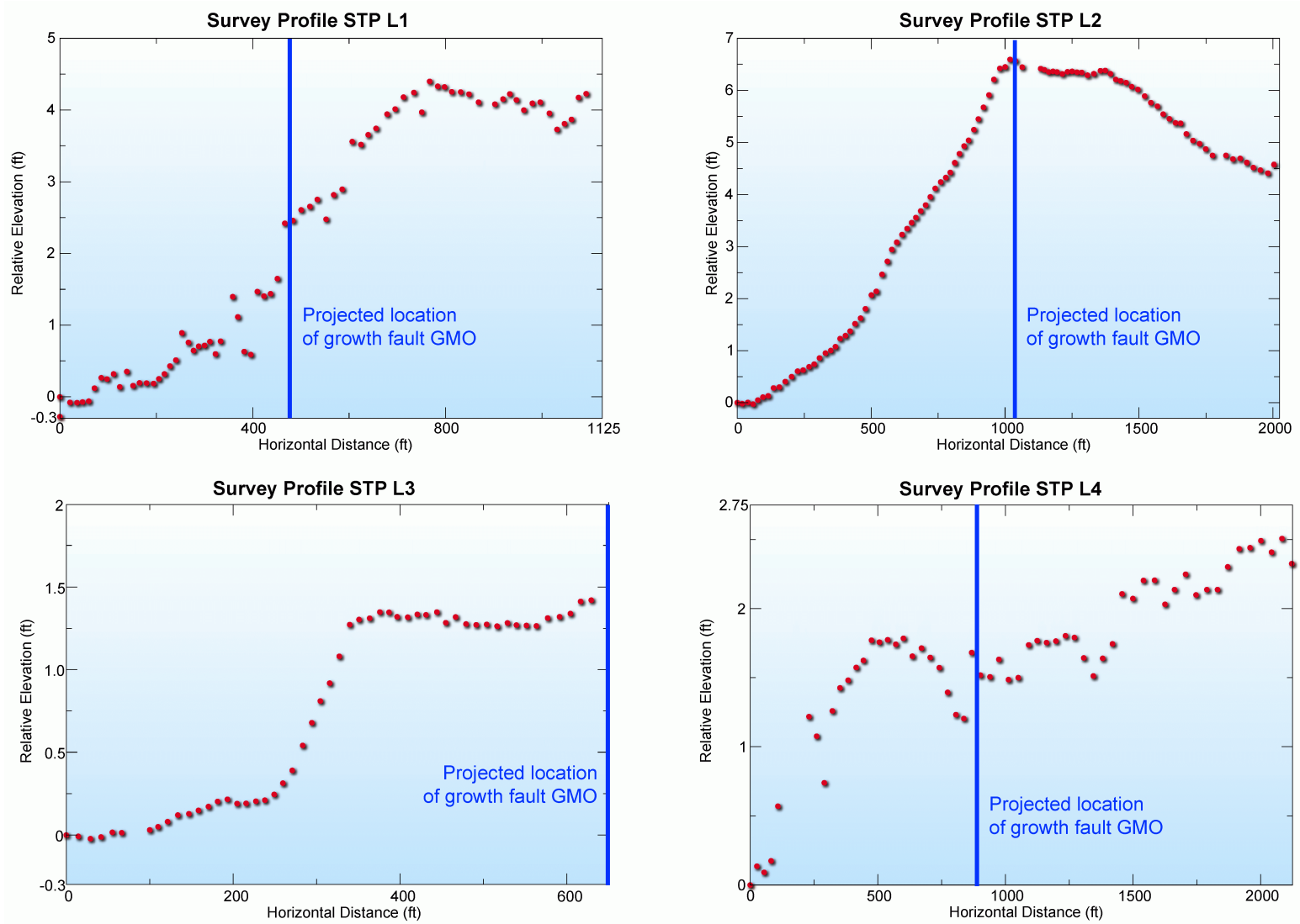
Figure 2.5S.1-46 Field Survey Elevation Profiles
