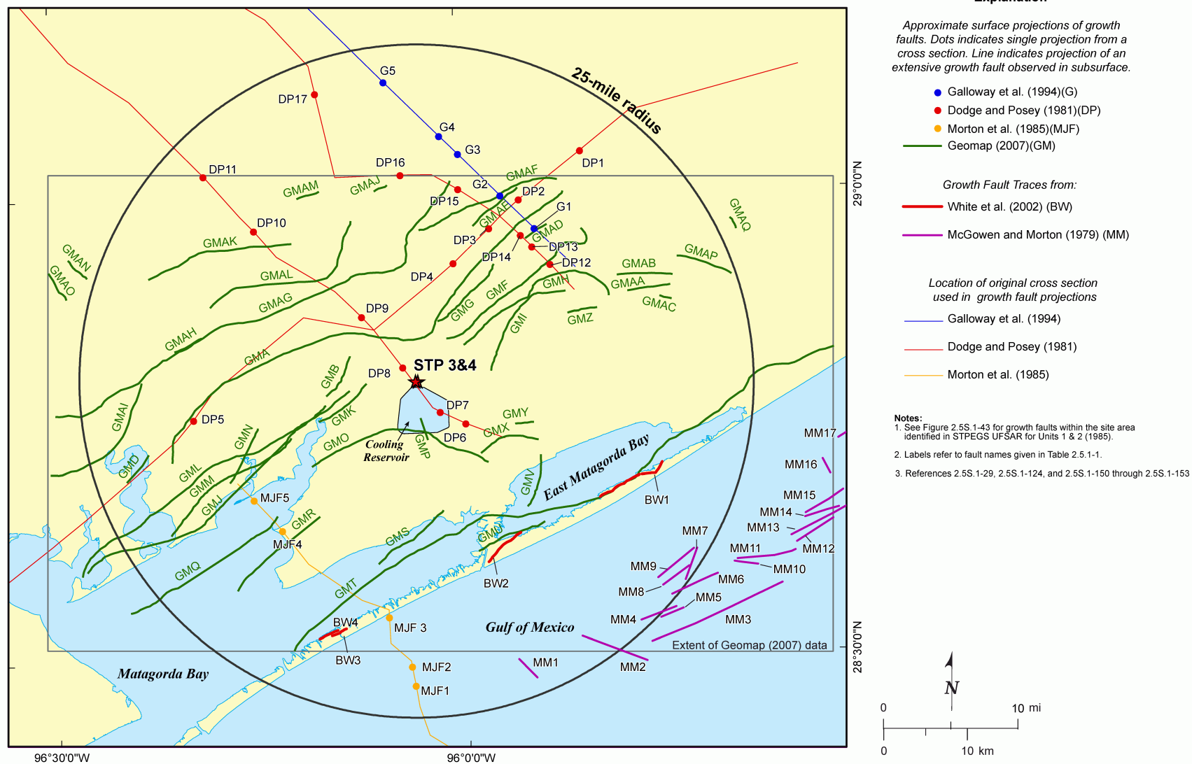
Figure 2.5S.1-42 Site Vicinity (25-mile radius) Growth Faults and Growth Fault Surface Projections
