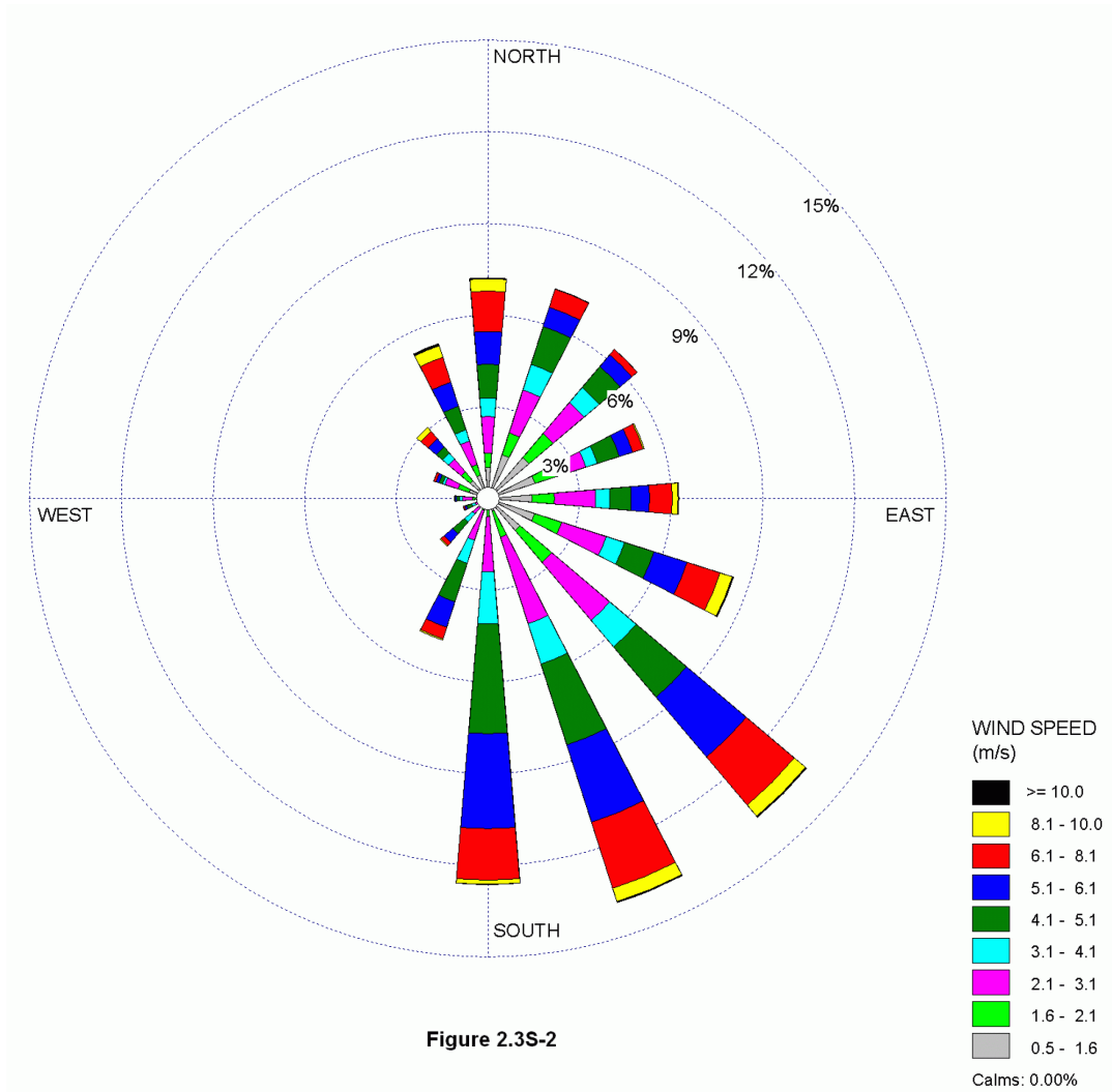
Figure 2.3S-2 STP 3 &amp; 4 10-Meter Level 3-year Composite Wind Rose - Annual (1997, 1999, and 2000)
