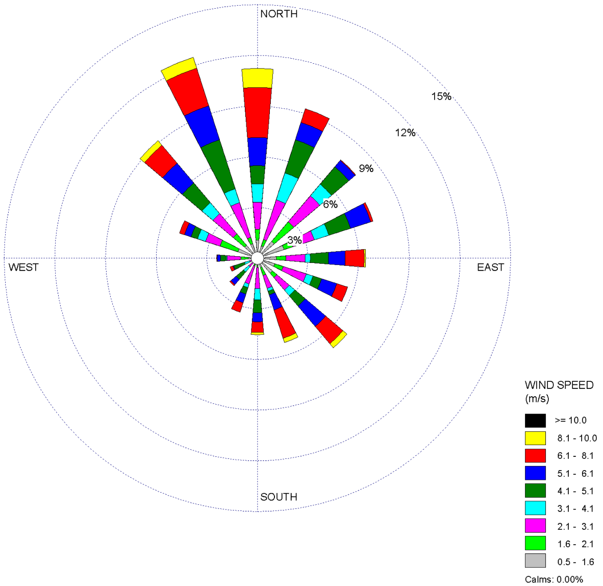
Figure 2.3S-12 STP 3 & 4 60-Meter Level 3-Year Composite Wind Rose - Autumn (1997, 1999, and 2000)
