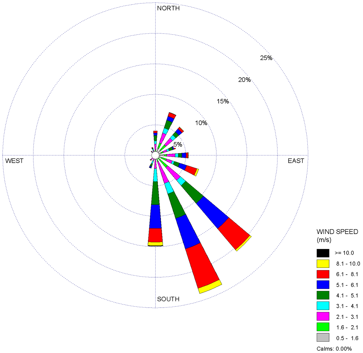
Figure 2.3S-7 STP 3 & 4 10-Meter Level 3-Year Composite Wind Rose - May (1997, 1999, and 2000) - Sheet 5 of 12
