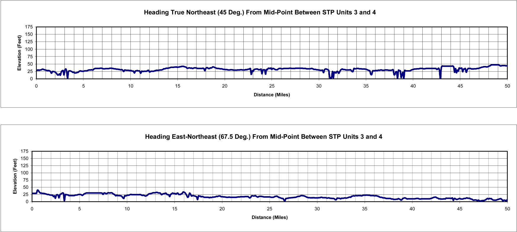
Figure 2.3S-16 Terrain Elevation Profiles Within 50 Miles of the STP 3 & 4 Site (Sheet 2 of 8)
