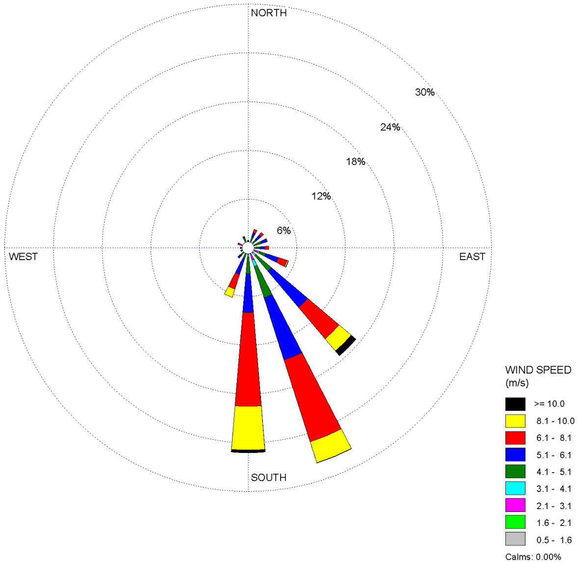
Figure 2.3S-13 STP 3 & 4 60-Meter Level 3-Year Composite Wind Rose - June (1997, 1999, and 2000) - Sheet 6 of 12
