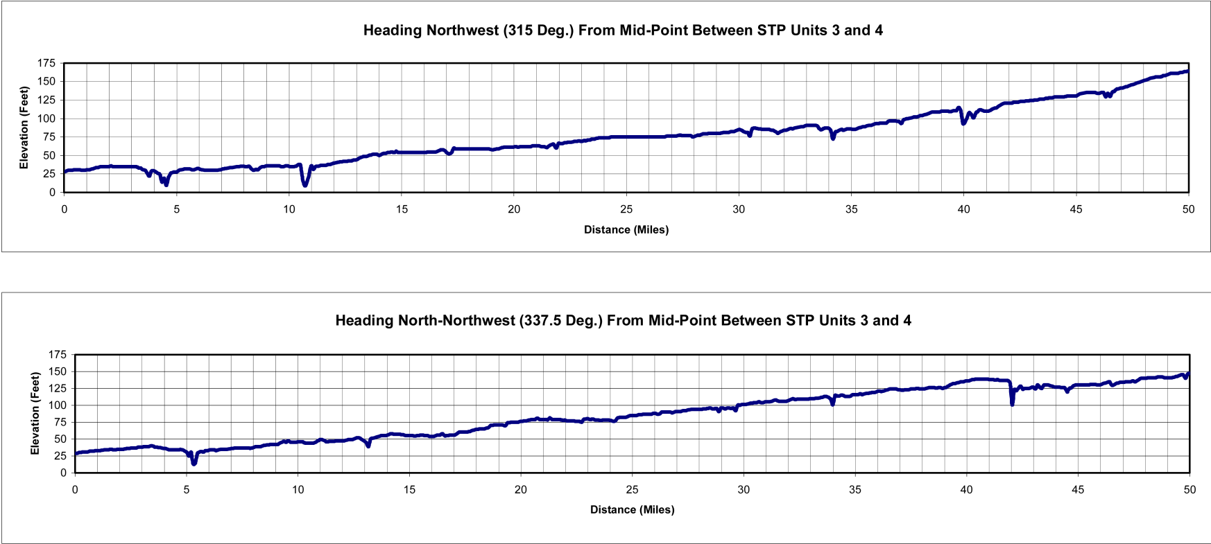
Figure 2.3S-16 Terrain Elevation Profiles Within 50 Miles of the STP 3 & 4 Site (Sheet 8 of 8)
