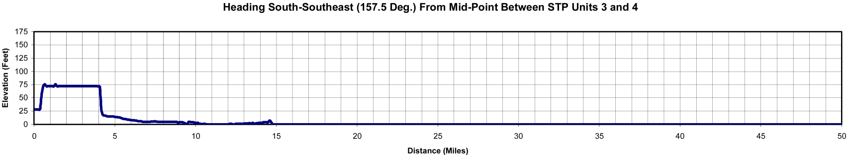
Figure 2.3S-16 Terrain Elevation Profiles Within 50 Miles of the STP 3 & 4 Site (Sheet 4 of 8)
