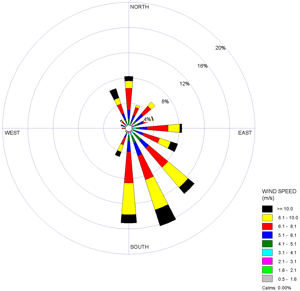
Figure 2.3S-13 STP 3 & 4 60-Meter Level 3-Year Composite Wind Rose - April (1997, 1999, and 2000) - Sheet 4 of 12
