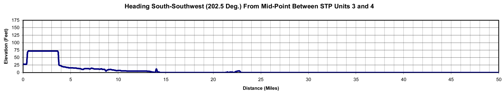
Figure 2.3S-16 Terrain Elevation Profiles Within 50 Miles of the STP 3 & 4 Site (Sheet 5 of 8)
