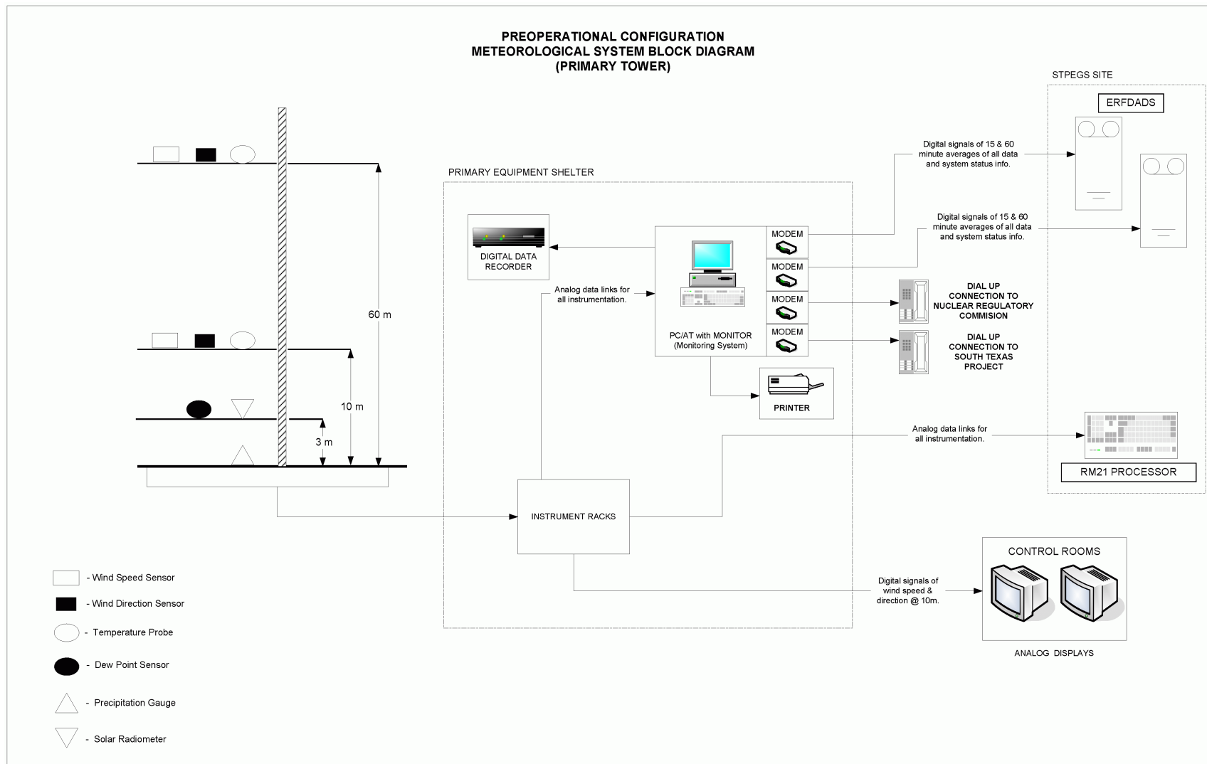
Figure 2.3S-19 Meteorological System Block Diagram (Primary Tower - Preoperational Configuration)
