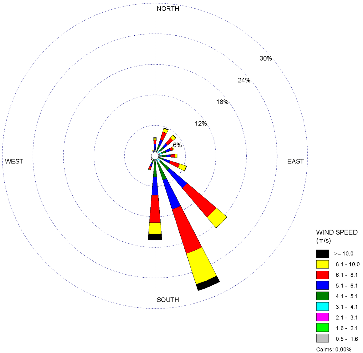
Figure 2.3S-13 STP 3 & 4 60-Meter Level 3-Year Composite Wind Rose - May (1997, 1999, and 2000) - Sheet 5 of 12
