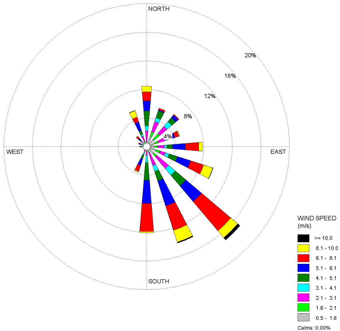
Figure 2.3S-7 STP 3 &amp; 4 10-Meter Level 3-Year Composite Wind Rose - April (1997, 1999, and 2000) - Sheet 4 of 12
