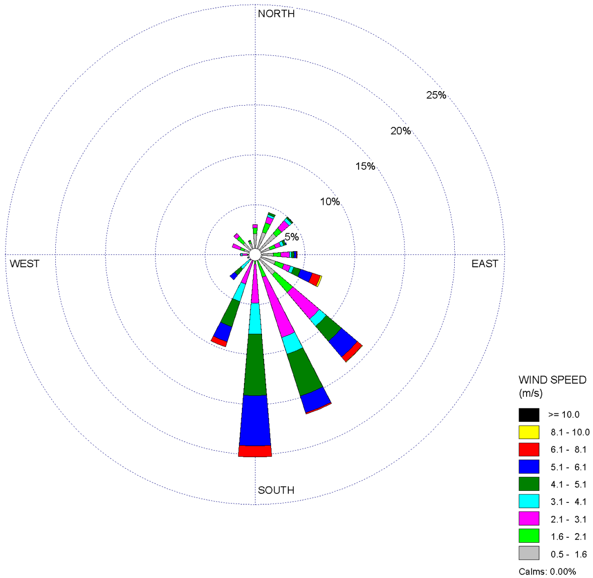
Figure 2.3S-7 STP 3 & 4 10-Meter Level 3-Year Composite Wind Rose - August (1997, 1999, and 2000) - Sheet 8 of 12
