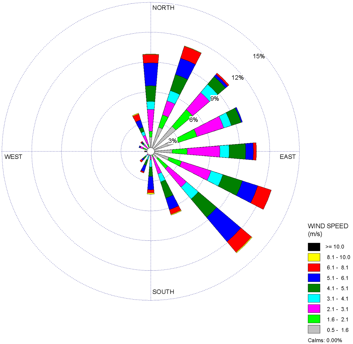
Figure 2.3S-10 STP 3 & 4 60-Meter Level 3-Year Composite Wind Rose - Spring (1997, 1999, and 2000)
