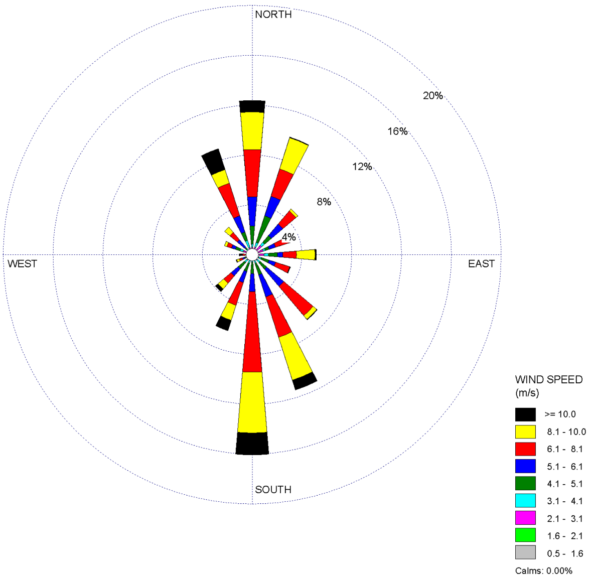
Figure 2.3S-13 STP 3 & 4 60-Meter Level 3-Year Composite Wind Rose - January (1997, 1999, and 2000) - Sheet 1 of 12
