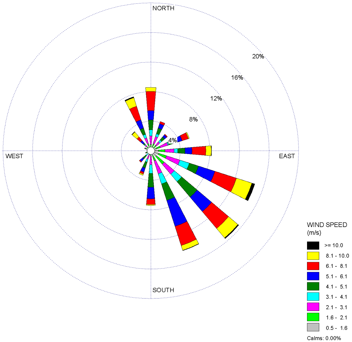
Figure 2.3S-7 STP 3 & 4 10-Meter Level 3-Year Composite Wind Rose - March (1997, 1999, and 2000) - Sheet 3 of 12
