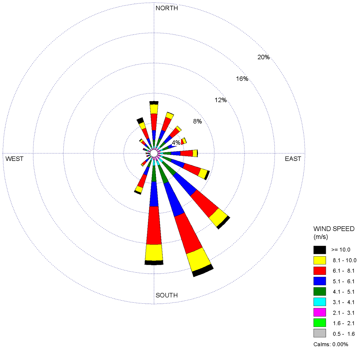
Figure 2.3S-8 STP 3 & 4 60-Meter Level 3-Year Composite Wind Rose - Annual (1997, 1999, and 2000)
