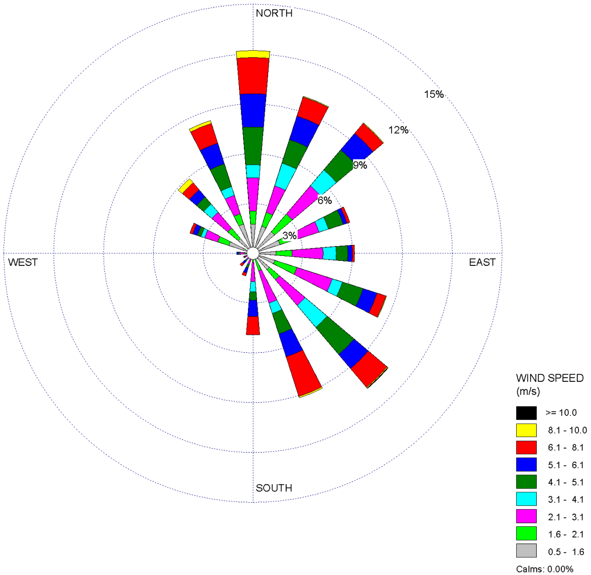
Figure 2.3S-7 STP 3 & 4 10-Meter Level 3-Year Composite Wind Rose - November (1997, 1999, and 2000) - Sheet 11 of 12
