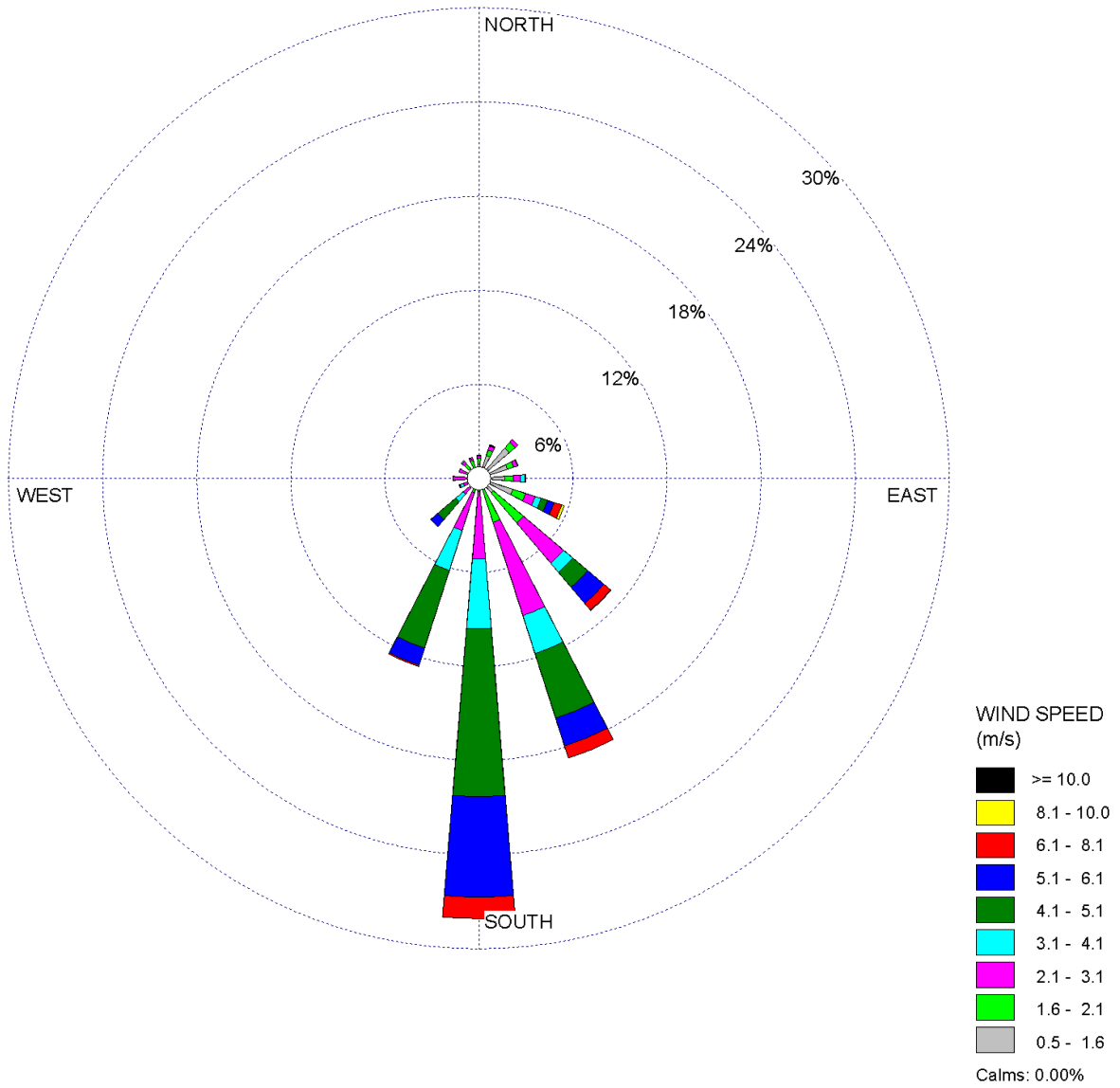
Figure 2.3S-7 STP 3 & 4 10-Meter Level 3-Year Composite Wind Rose - July (1997, 1999, and 2000) - Sheet 7 of 12
