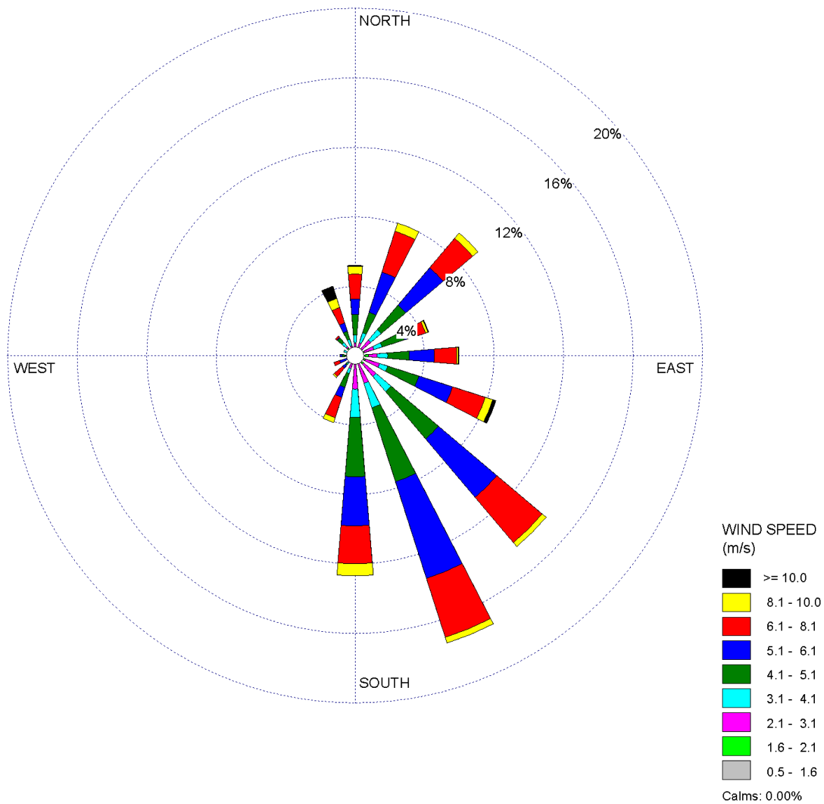
Figure 2.3S-13 STP 3 &amp; 4 60-Meter Level 3-Year Composite Wind Rose - September (1997, 1999, and 2000) - Sheet 9 of 12
