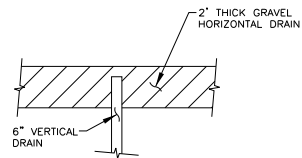
HORIZONTAL & VERTICAL DRAINS TYPICAL SECTION
