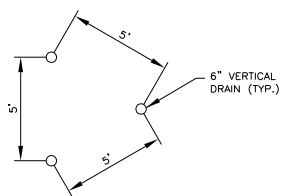
TYPICAL SPACING OF VERTICAL DRAINS
