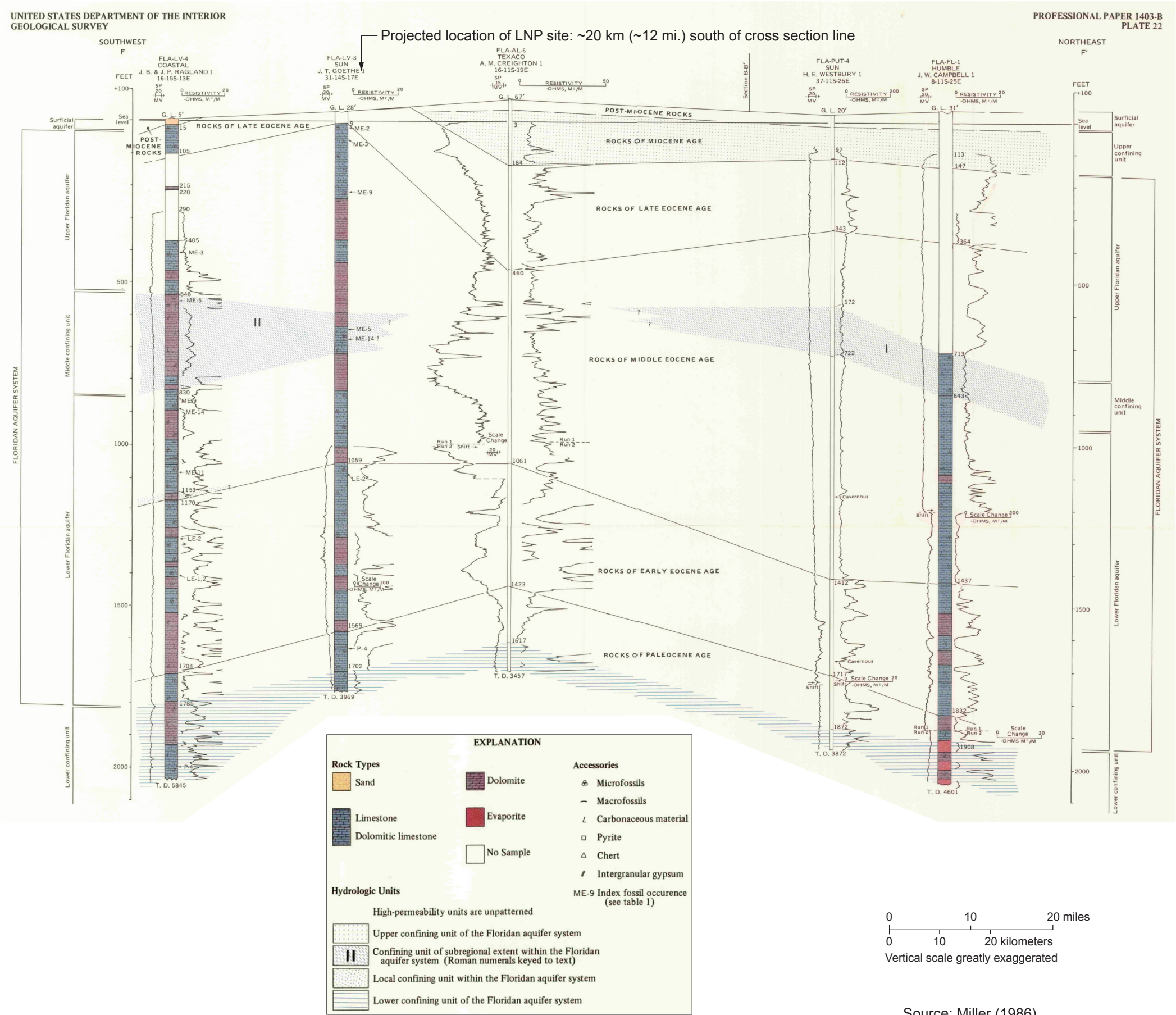
Progress Energy Florida Levy Nuclear Plant Units 1 and 2 Part 2, Final Safety Analysis Report Geohydrologic Cross Section F-F' from Levy County, Florida, to Flagler County, Florida Figure 2.5.1-217 Rev 0
