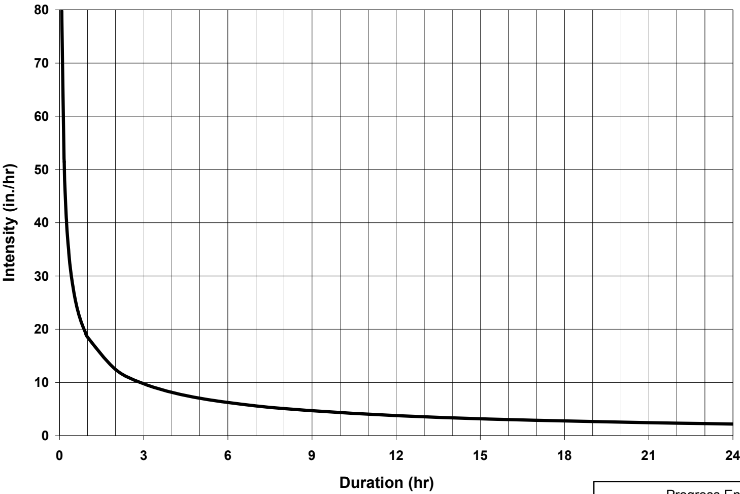
Progress Energy Florida Levy Nuclear Plant Units 1 and 2 Part 2, Final Safety Analysis Report Local Intense Probable Maximum Precipitation Intensity-Duration Curve FIGURE 2.4.2-203 Rev 0
