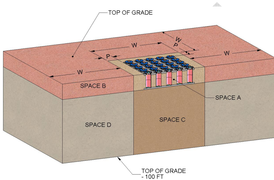
Figure 3.4-1 - SUB-GRADE AND UNDER-GRADE SPACE NOMENCLATURE
