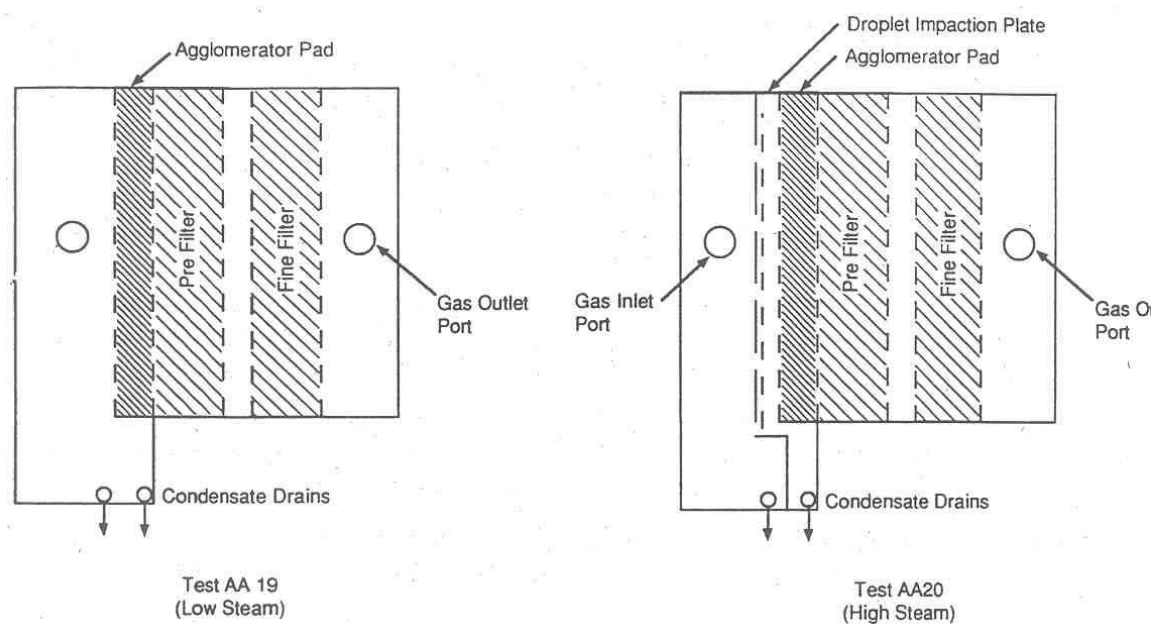
Fig. 5.9-6 Schematic diagram of metal fibre filter
