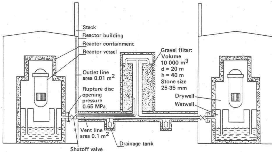
Fig. 5.9-2 FILTRA - schematic drawing
