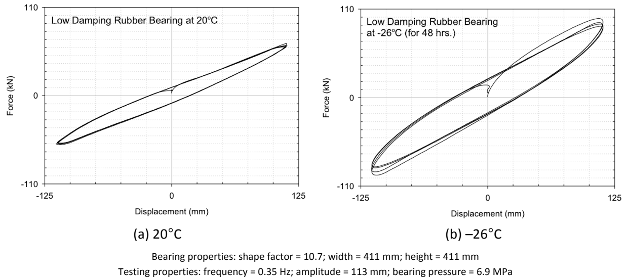
Figure 3.3 Effect of temperature on mechanical properties of LDB (Constantinou et al. 2007)
