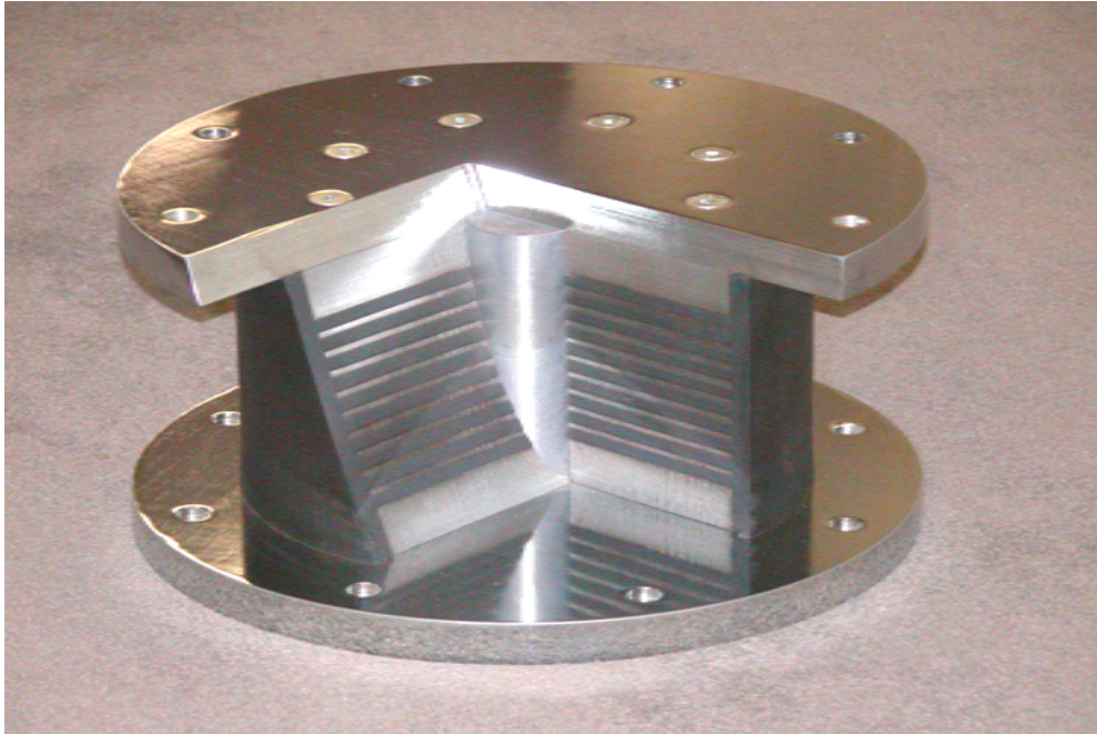
Figure 3.4 A cut-away view of a lead rubber bearing (courtesy of Dynamic Isolation Systems, Inc.)
