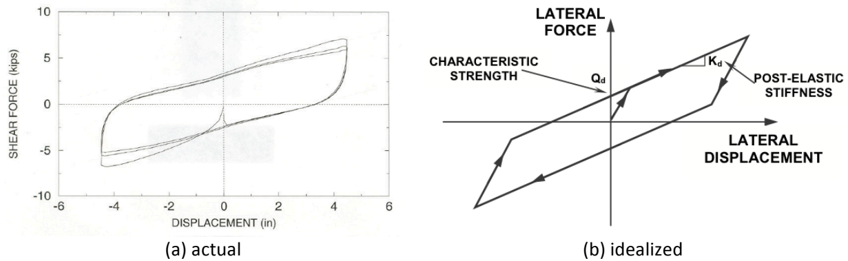
(a) actual Bearing properties: bearing diameter = 184 mm; diameter of lead plug = 38 mm Testing properties: frequency = 0.5 Hz; amplitude = 250% shear strain; bearing pressure = 6.9 MPa
