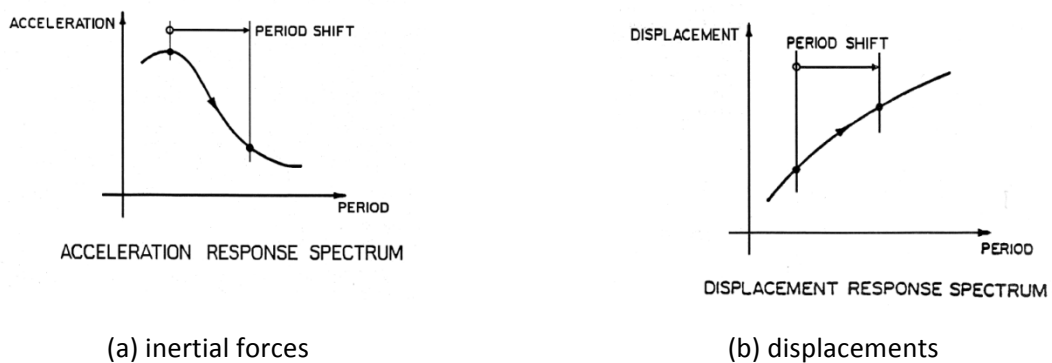
Figure 1.2 Impact of period elongation on inertial forces and displacements in structures (courtesy of DIS Inc, reproduced with permission)
