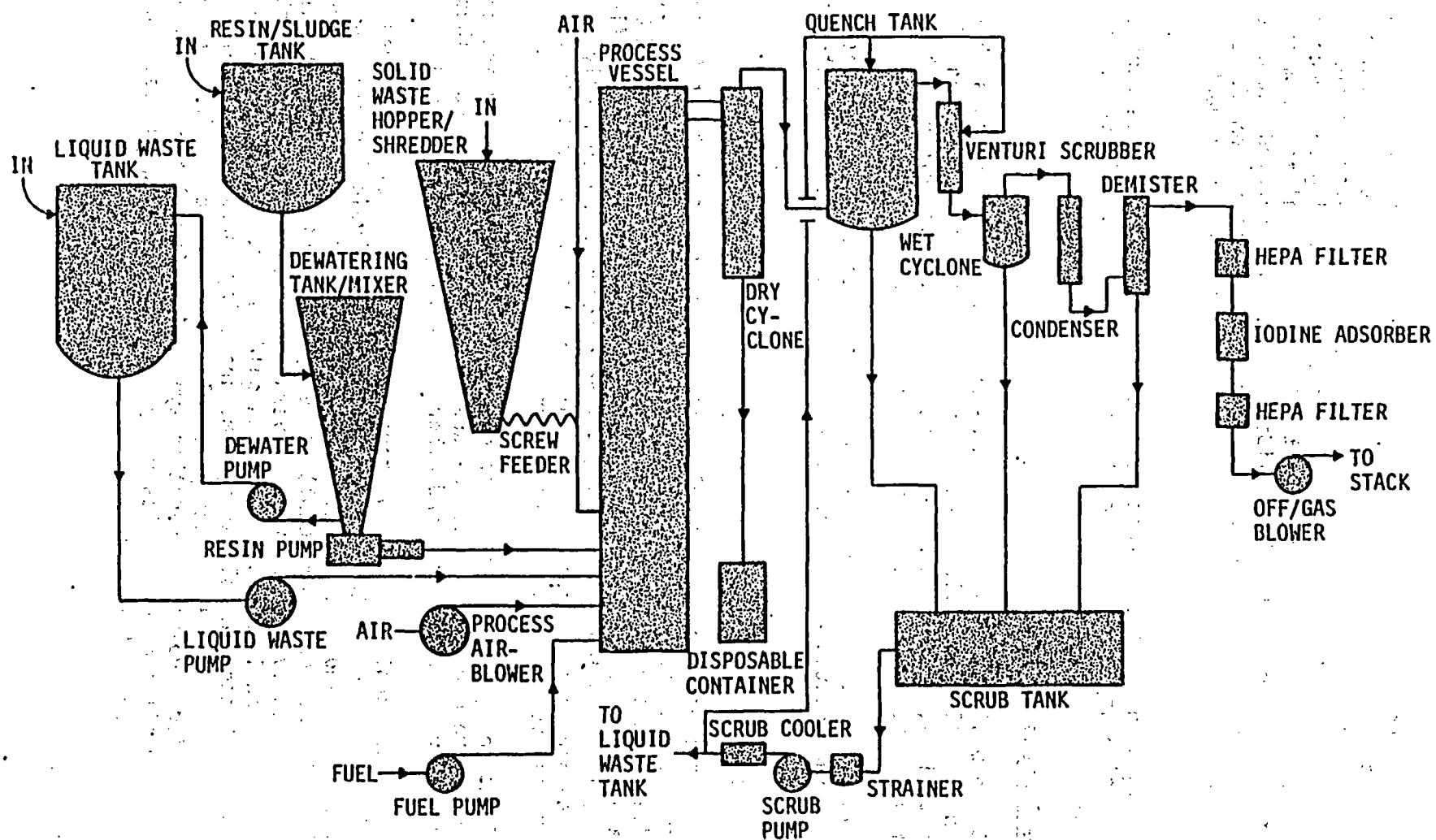
Figure D.7 Flow Diagram of Calciner/Incinerator
