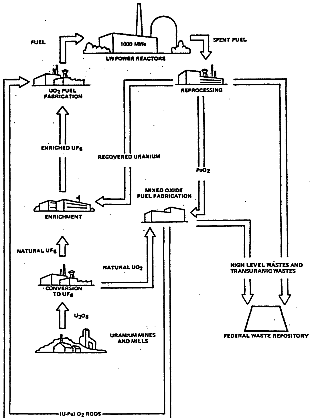
Figure D.3 Uranium and Plutonium Recycle Fuel Cycle
