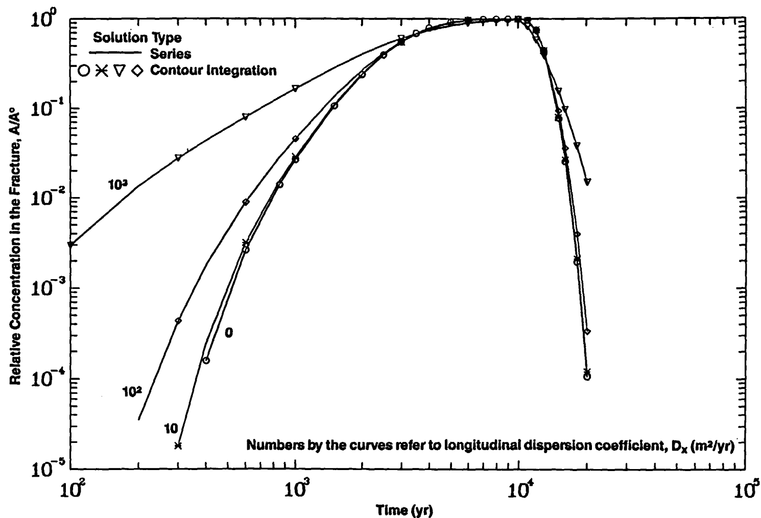
Figure 6-4a. Comparison of Temporal Variation of Relative Concentration of Np-237 in the Fracture for D_{xx} = 0, 10, 100, 1000 m 2 /yr (Case 6B: Multiple Parallel Fractures, Band Release Mode)
