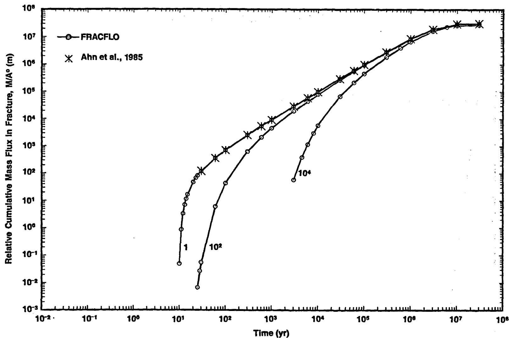
Figure 3-1g. Relative Cumulative Mass Flux of Np-237 in the Fracture Versus Time at x = 100 m and y = 0 m for Different Rock Matrix Retardation Factors ( R' = 1, 10^2, 10^4 ) (Case 1A: Step Release Mode)
