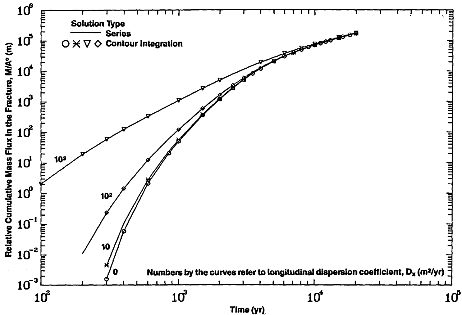
Figure 6-4c. Comparison of Temporal Variation of Relative Cumulative Mass Flux of Np-237 in the Fracture for D_{xx} = 0, 10, 100, 1000 m^2/yr (Case 6B: Multiple Parallel Fractures, Band Release Mode)
