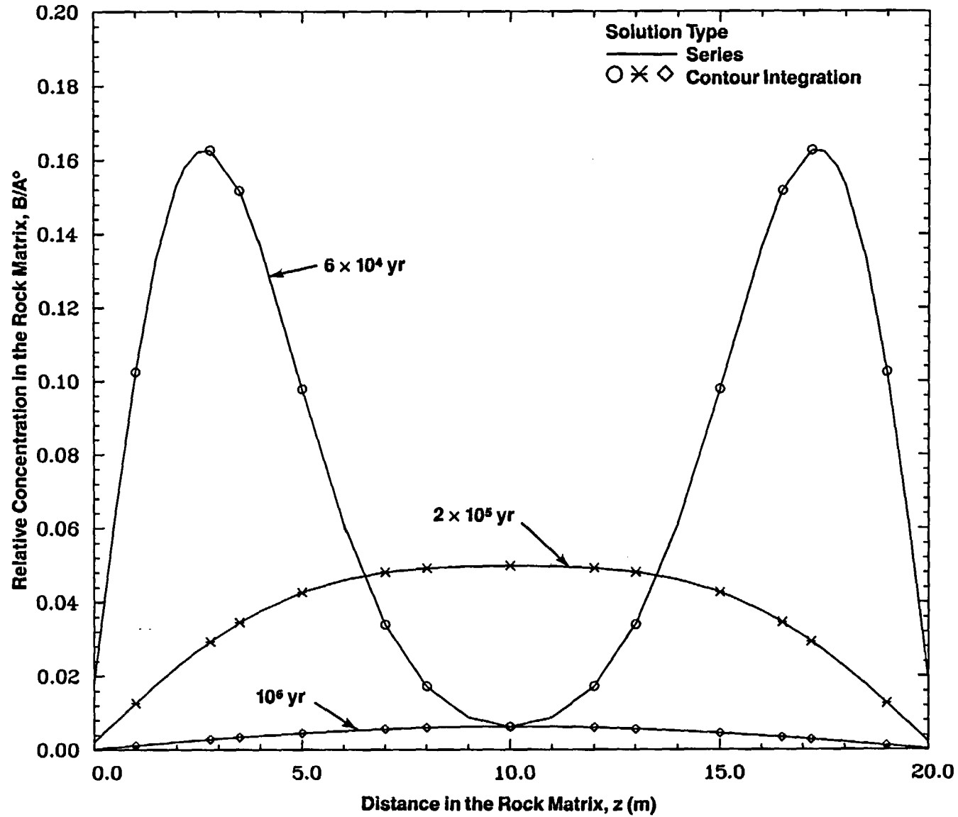
Figure 6-2d. Comparison of Spatial Variation of Relative Concentration of Np-237 in the Rock Matrix for Different Times (Case 5B: Multiple Parallel Fractures, Band Release Mode, No Longitudinal Dispersion)
