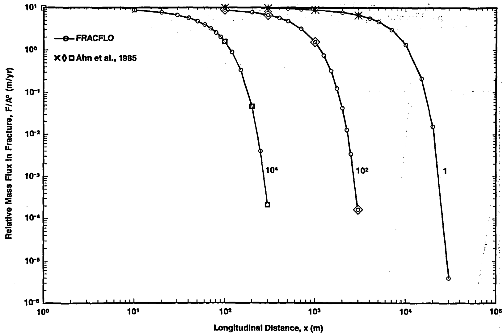
Figure 3-2c. Relative Mass Flux of Np-237 in the Fracture Versus Distance x at y = 0 m, t = 10^4 yr, and D_{xx} = 0 for Different Rock Matrix Retardation Factors ( R' = 1, 10^2, 10^4 ) (Case 1B: Step Release Mode)
