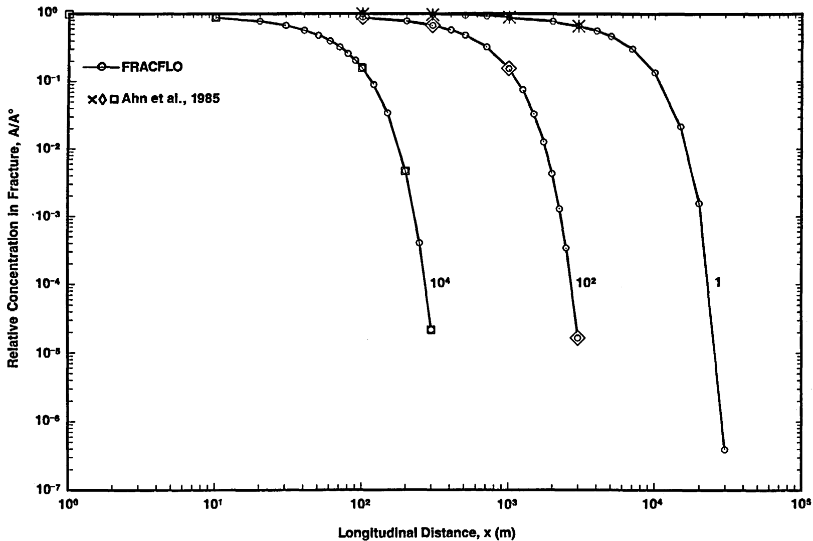
Figure 3-2a. Relative Concentrations of Np-237 in the Fracture Versus Longitudinal Distance x at y = 0 m, t = 10^4 yr, and D_{xx} = 0 for Different Rock Matrix Retardation Factors ( R' = 1, 10^2, 10^4 ) (Case 1B: Step Release Mode)
