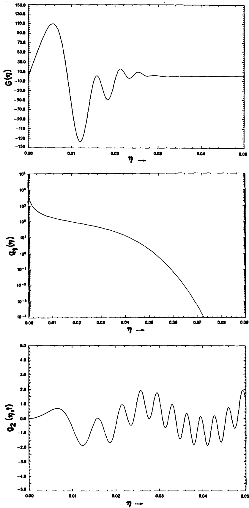
Figure B-3. Variations of Function G(\eta) , g_1(\eta) , and g_2(\eta, t) for x=10,000 m
