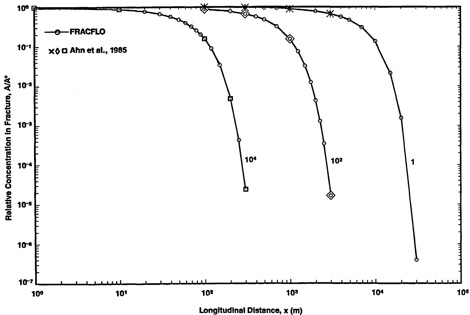
Figure 3-1a. Relative Concentrations of Np-237 in the Fracture Versus Longitudinal Distance x at y = 0 m and t = 10^4 yr for Different Rock Matrix Retardation Factors ( R' = 1, 10^2, 10^4 ) (Case 1A: Step Release Mode)
