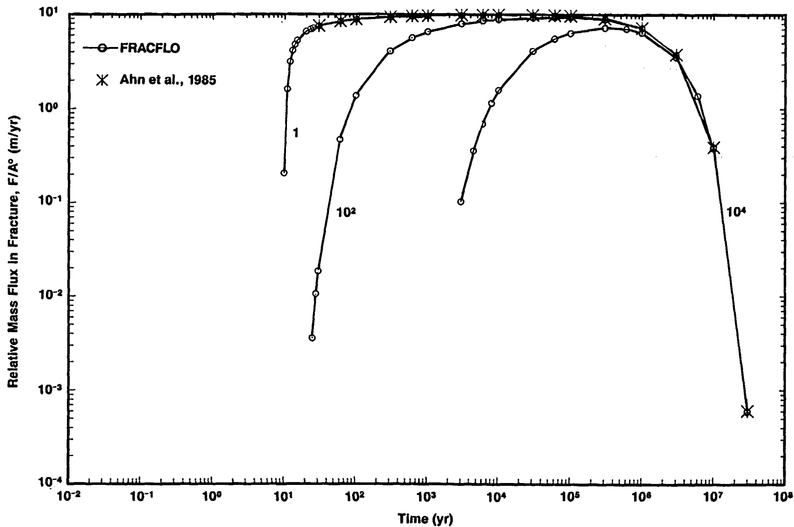
Figure 3-1f. Relative Mass Flux of Np-237 in the Fracture Versus Time at x = 100 m, and y = 0 m for Different Rock Matrix Retardation Factors ( R' = 1, 10^2, 10^4 ) (Case 1A: Step Release Mode)
