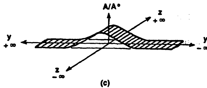
Figure 2-2. Schematic of Multiple Parallel Fracture Rock System (a) Patch Source; (b) Multiple Patch Source; (c) Gaussian Distributed Source
