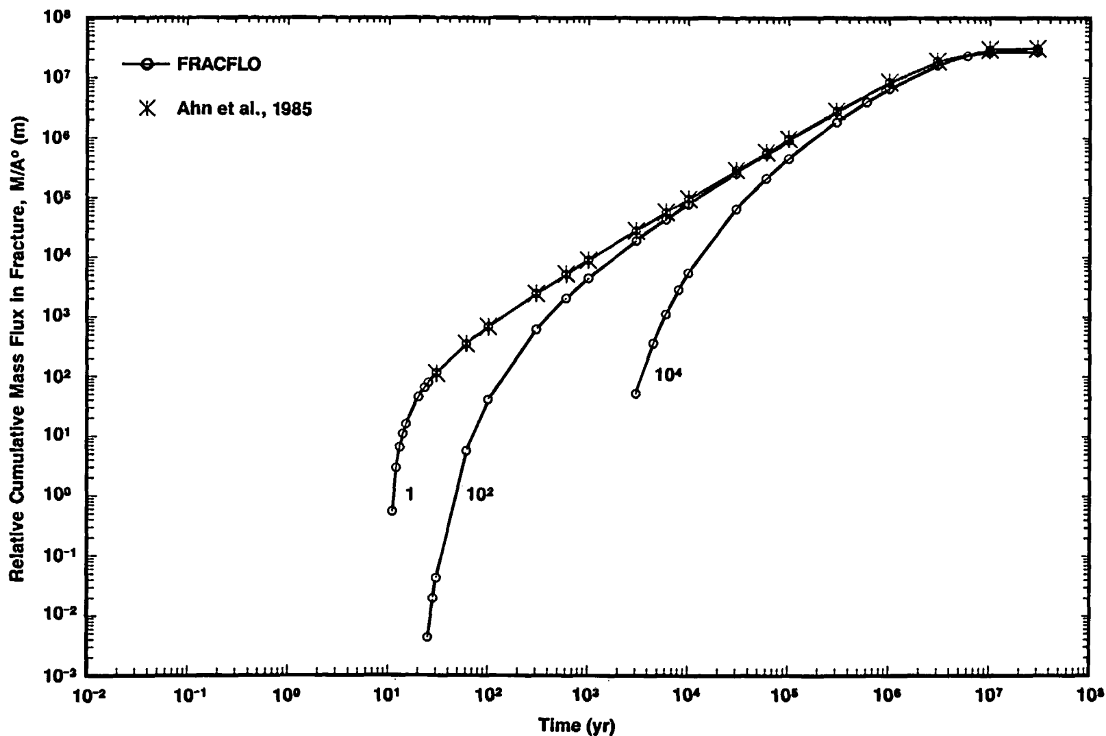
Figure 3-2g. Relative Cumulative Mass Flux of Np-237 in the Fracture Versus Time at x = 100 m, y = 0 m, and D_{xx} = 0 for Different Rock Matrix Retardation Factors ( R' = 1, 10^2, 10^4 ) (Case 1B: Step Release Mode)
