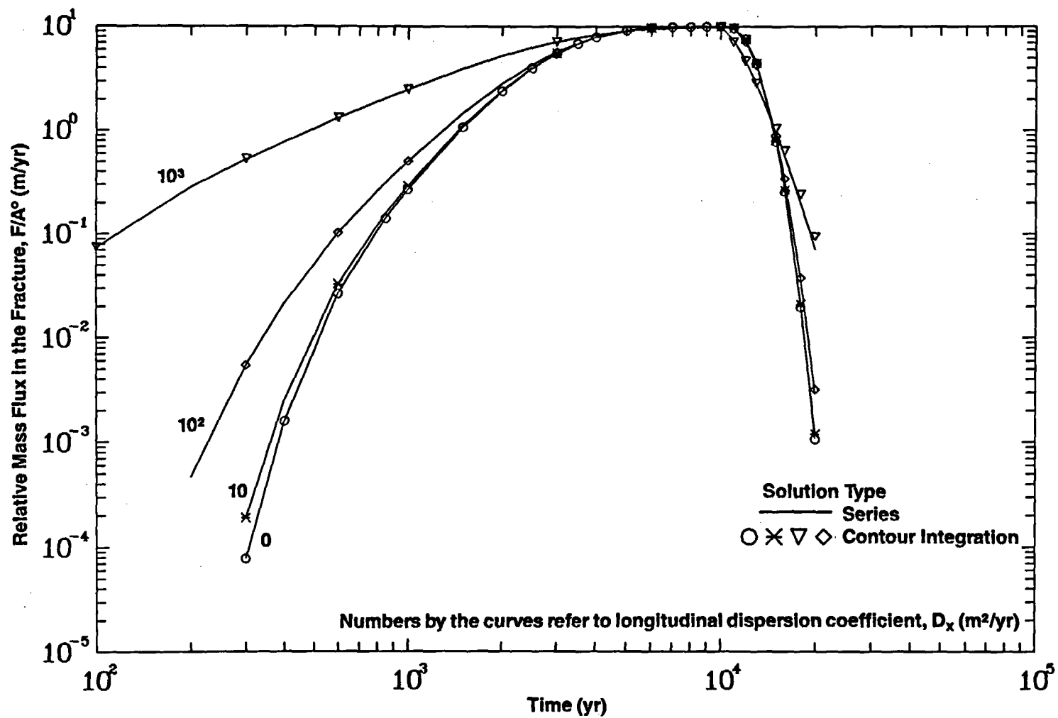
Figure 6-4b. Comparison of Temporal Variation of Relative Mass Flux of Np-237 in the Fracture for D_{xx} = 0, 10, 100, 1000 m²/yr (Case 6B: Multiple Parallel Fractures, Band Release Mode)
