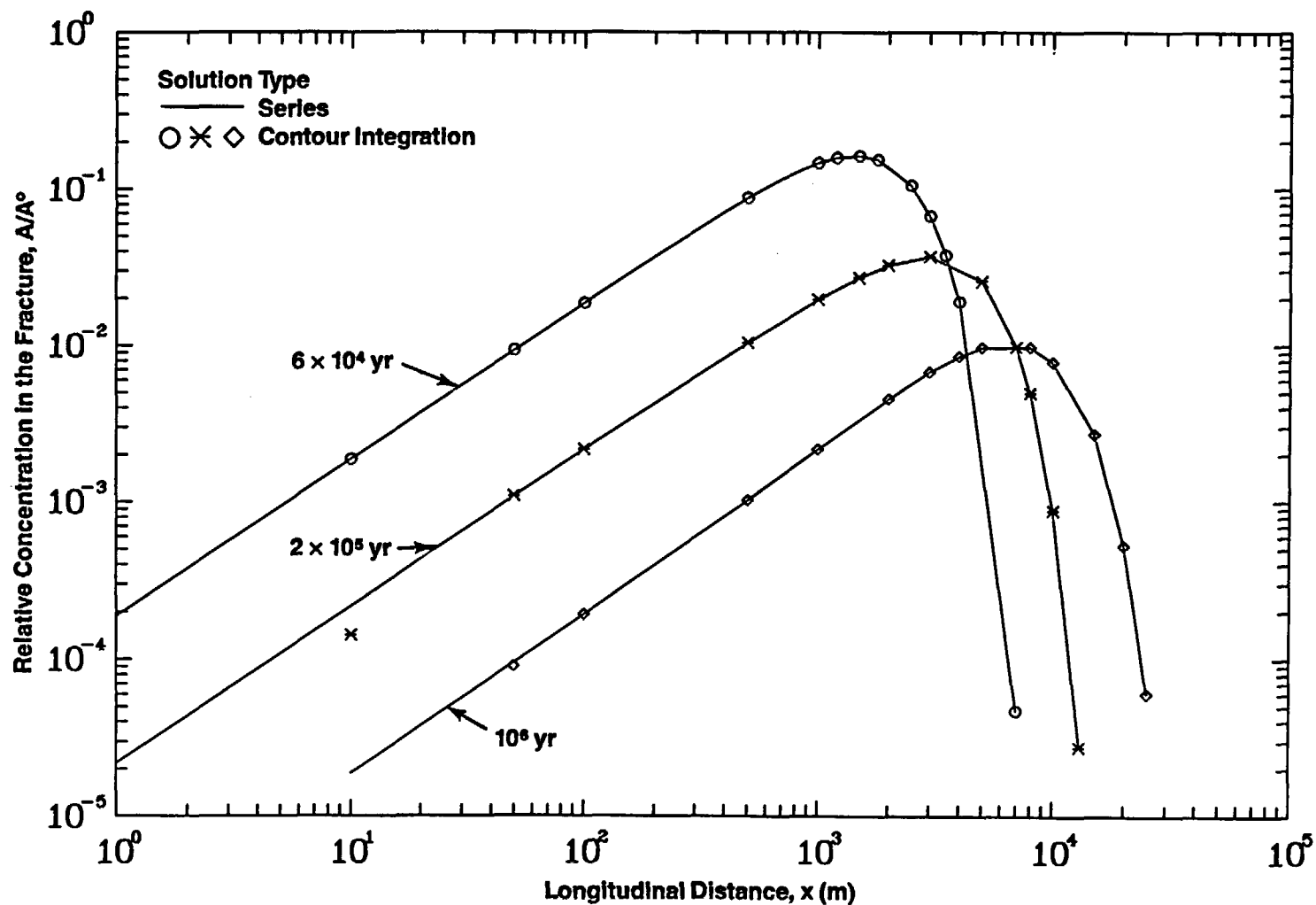
Figure 6-2a. Comparison of Spatial Variation of Relative Concentration of Np-237 in the Fracture for Different Times (Case 5B: Multiple Parallel Fractures, Band Release Mode, No Longitudinal Dispersion)
