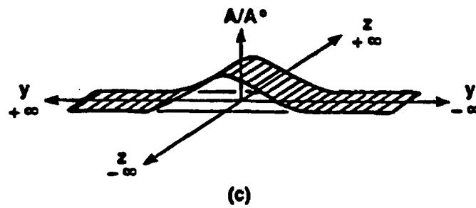
Figure 2-1. Schematic of a Single Fracture Rock System (a) Patch Source; (b) Multiple Patch Source; (c) Gaussian Distribution Source
