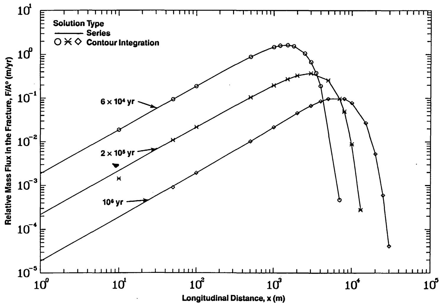
Figure 6-2b. Comparison of Spatial Variation of Relative Mass Flux of Np-237 in the Fracture for Different Times (Case 5B: Multiple Parallel Fractures, Band Release Mode, No Longitudinal Dispersion)
