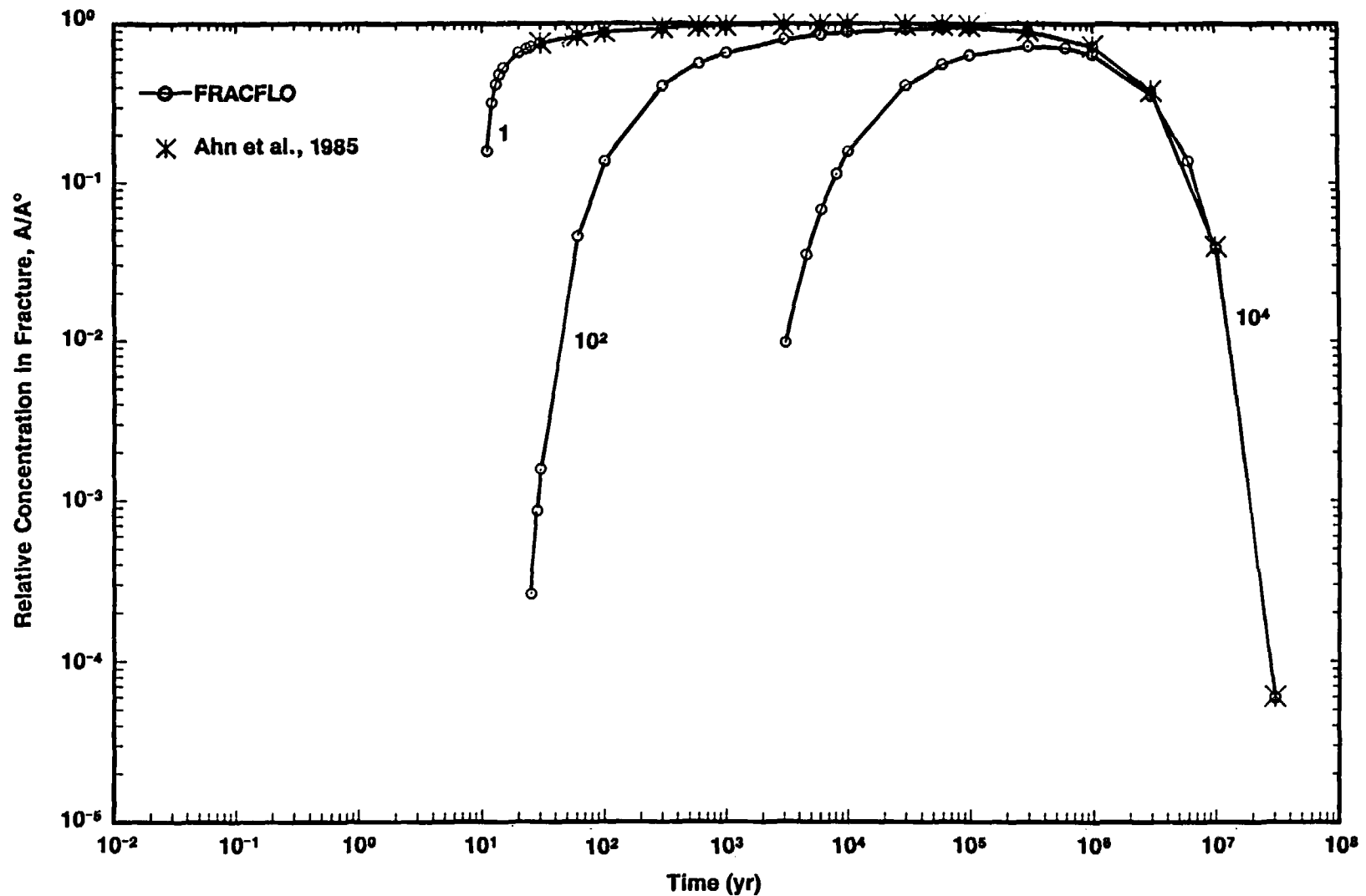
Figure 3-2e. Breakthrough Curves Showing the Relative Concentration of Np-237 in the Fracture Versus Time at x = 100 m, y = 0 m, and D_{xx} = 0 for Different Rock Matrix Retardation Factors ( R' = 1, 10^2, 10^4 ) (Case 1B: Step Release Mode)
