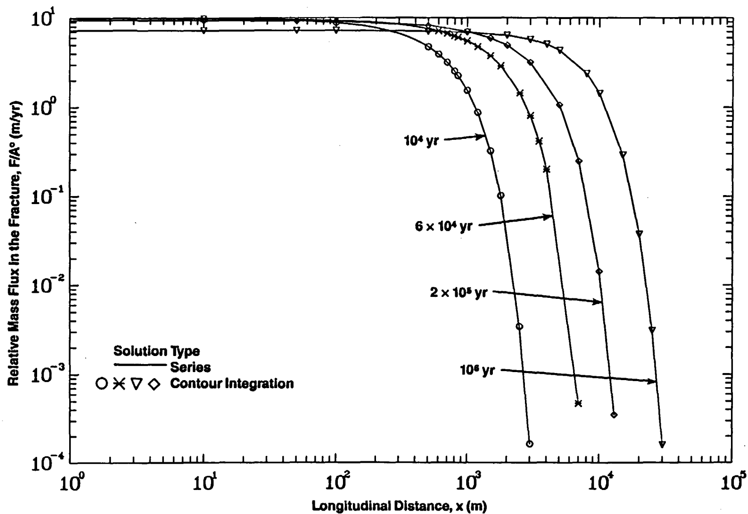
Figure 6-1b. Comparison of Spatial Variation of Relative Mass Flux of Np-237 in the Fracture for Different Times (Case 5A: Multiple Parallel Fractures, Step Release Mode, No Longitudinal Dispersion)
