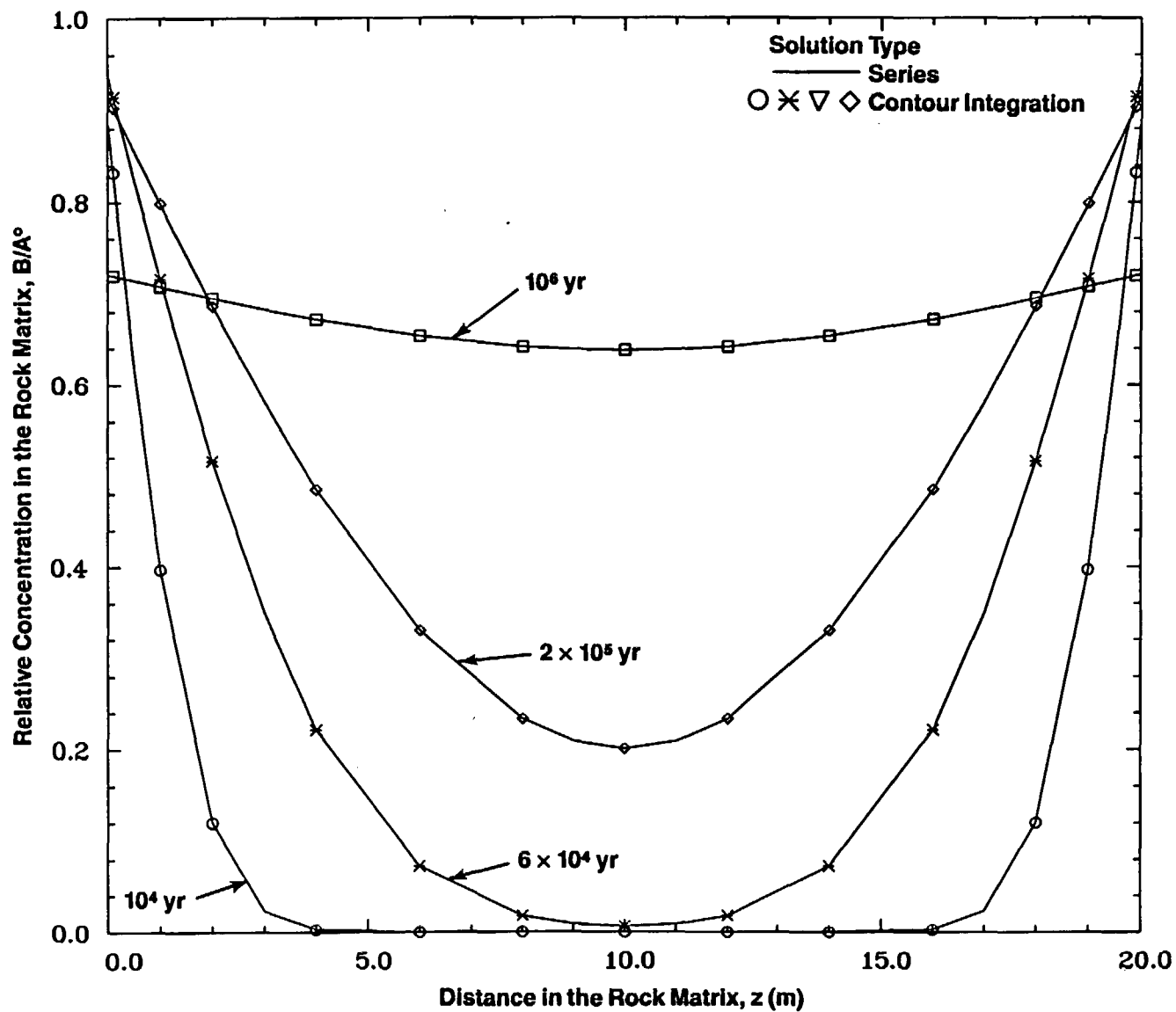
Figure 6-1d. Comparison of Spatial Variation of Relative Concentration of Np-237 in the Rock Matrix for Different Times (Case 5A: Multiple Parallel Fractures, Step Release Mode, No Longitudinal Dispersion)
