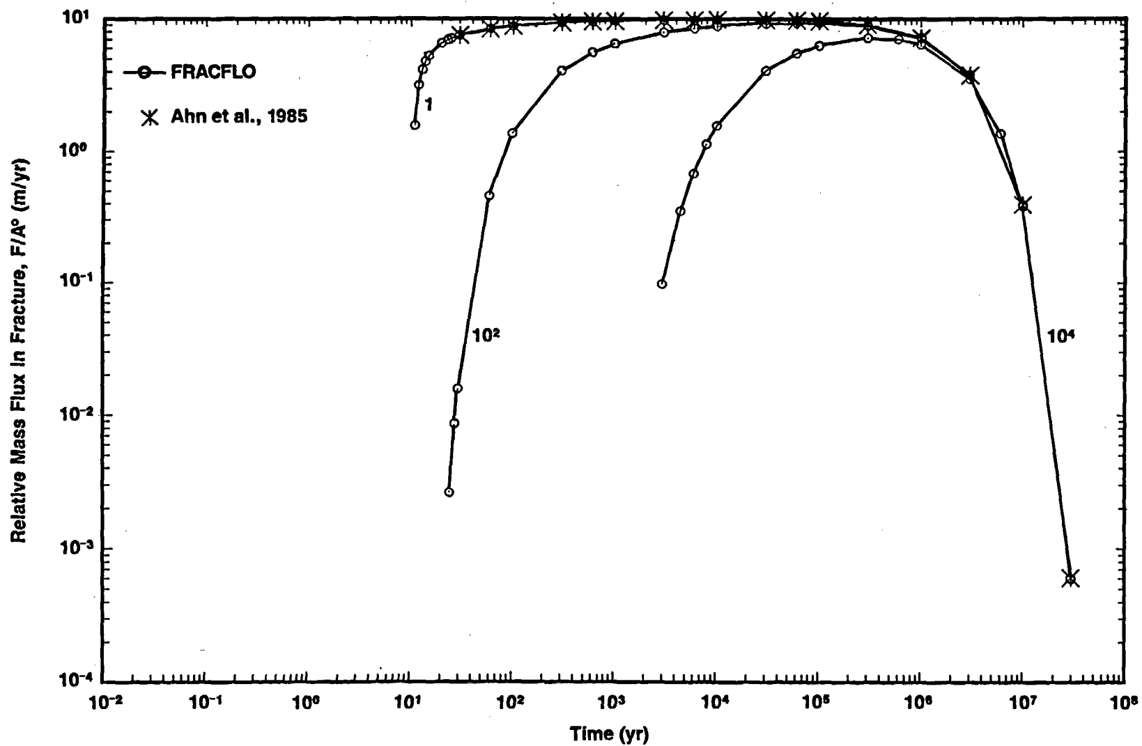
Figure 3-2f. Relative Mass Flux of Np-237 in the Fracture Versus Time at x = 100 m, y = 0 m, and D_{xx} = 0 for Different Rock Matrix Retardation Factors ( R' = 1, 10^2, 10^4 ) (Case 1B: Step Release Mode)
