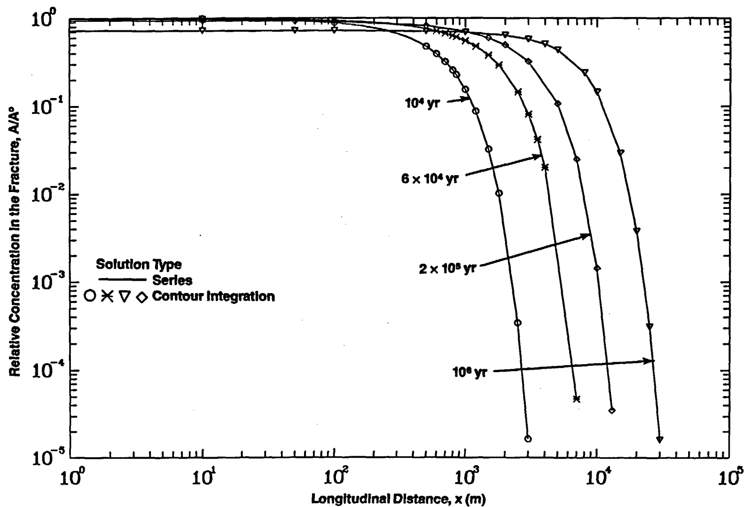
Figure 6-1a. Comparison of Spatial Variation of Relative Concentration of Np-237 In the Fracture for Different Times (Case 5A: Multiple Parallel Fractures, Step Release Mode, No Longitudinal Dispersion)
