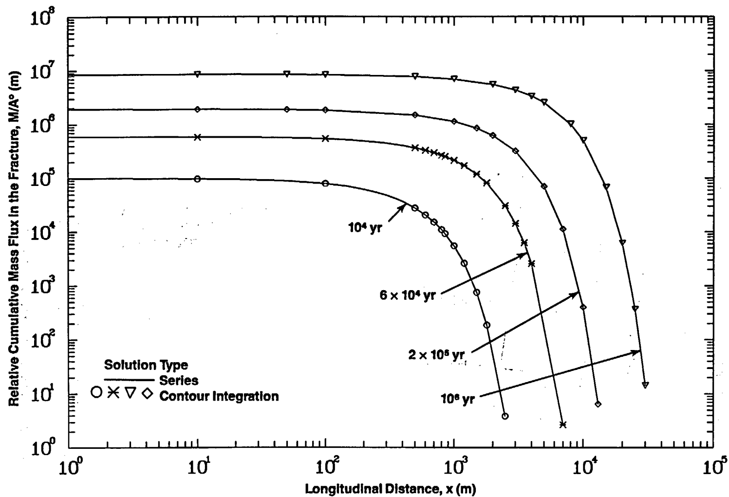
Figure 6-1c. Comparison of Spatial Variation of Relative Cumulative Mass Flux of Np-237 in the Fracture for Different Times (Case 5A: Multiple Parallel Fractures, Step Release Mode, No Longitudinal Dispersion)
