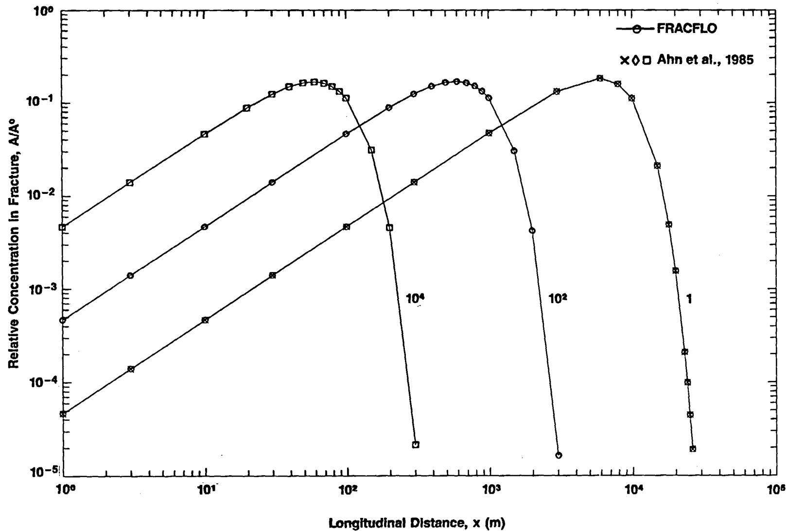
Figure 3-3a. Relative Concentrations of Np-237 in the Fracture Versus Longitudinal Distance x at y = 0 m, t = 10^4 yr, and D_{xx} = 0 for Different Rock Matrix Retardation Factors ( R' = 1, 10^2, 10^4 ) (Case 2: Band Release Mode)
