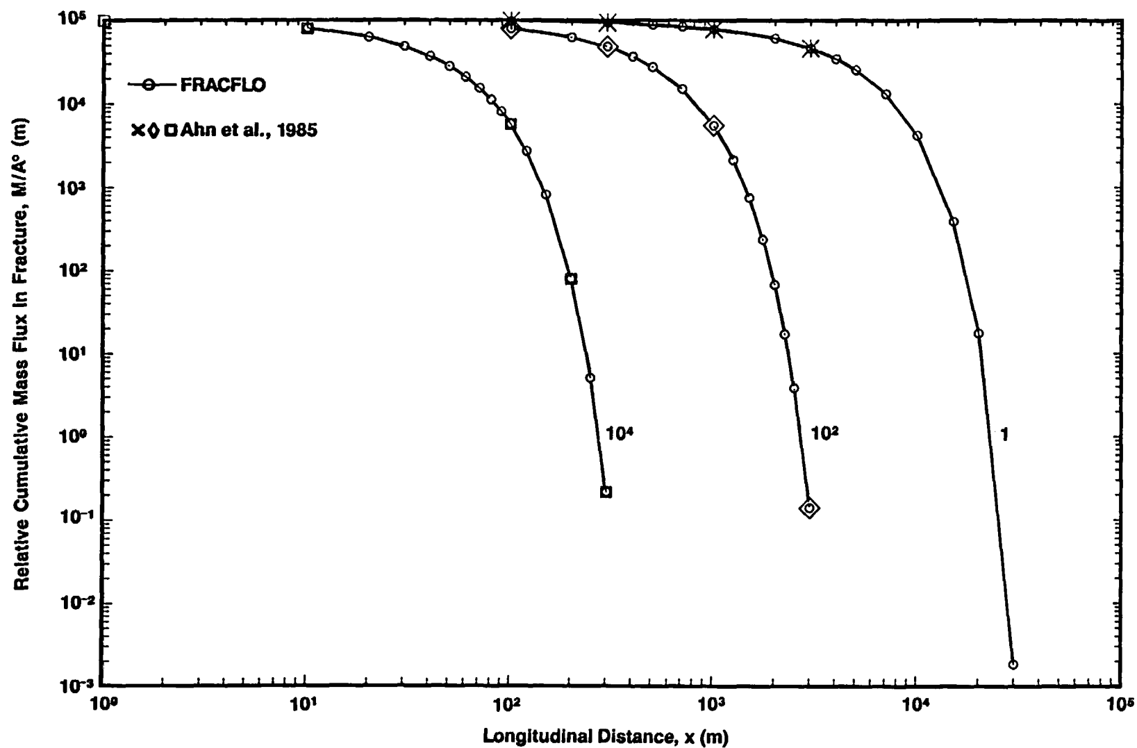
Figure 3-1d. Relative Cumulative Mass Flux of Np-237 in the Fracture Versus Longitudinal Distance x at y = 0 m and t = 10^4 yr for Different Rock Matrix Retardation Factors ( R' = 1, 10^2, 10^4 ) (Case 1A: Step Release Mode)
