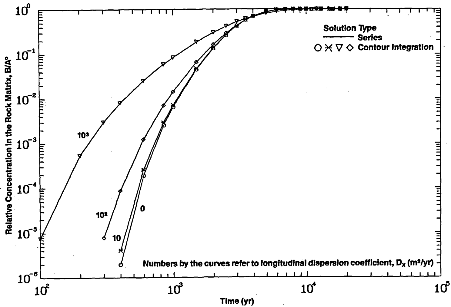
Figure 6-3d. Comparison of Temporal Variation of Relative Concentration of Np-237 in the Rock Matrix at Elevation z = 0.3 m for D_{xx} = 0, 10, 100, 1000 m^2/yr (Case 6A: Multiple Parallel Fractures, Step Release Mode)
