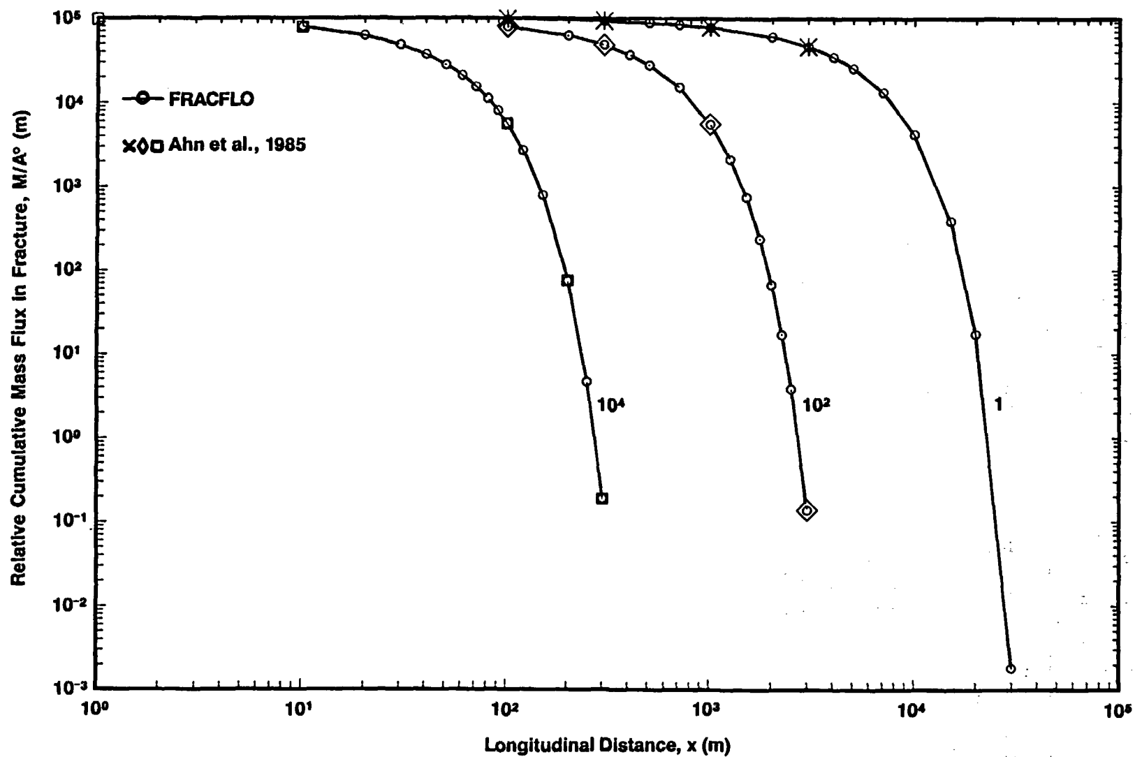
Figure 3-2d. Relative Cumulative Mass Flux of Np-237 in the Fracture Versus Longitudinal Distance x at y = 0 m, t = 10^4 yr, and D_{xx} = 0 for Different Rock Matrix Retardation Factors ( R' = 1, 10^2, 10^4 ) (Case 1B: Step Release Mode)
