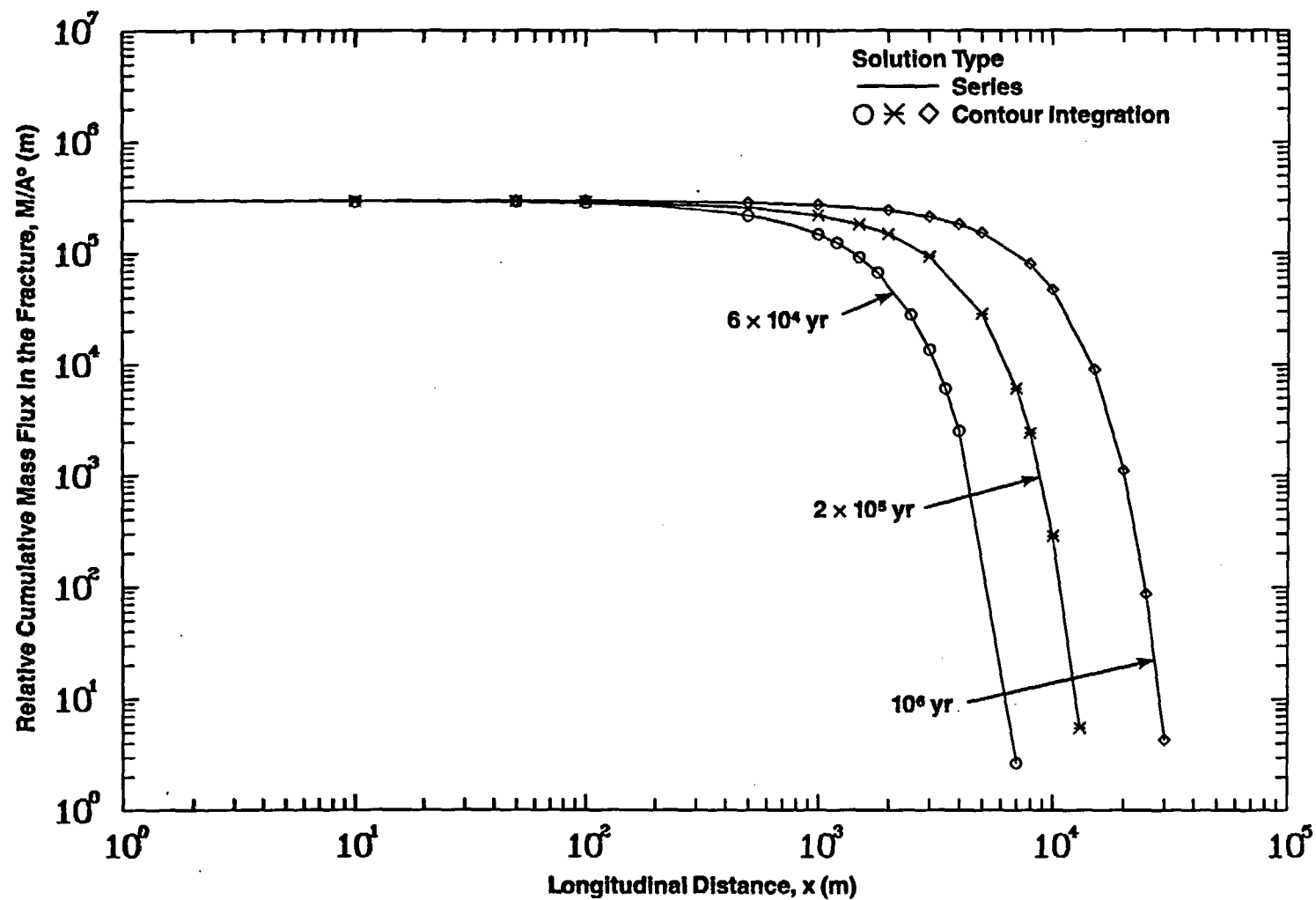
Figure 6-2c. Comparison of Spatial Variation of Relative Cumulative Mass Flux of Np-237 in the Fracture for Different Times (Case 5B: Multiple Parallel Fractures, Band Release Mode, No Longitudinal Dispersion)
