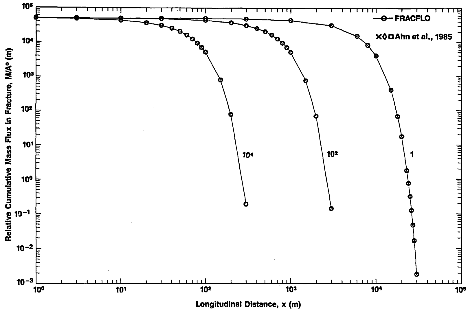
Figure 3-3c. Relative Cumulative Mass Flux of Np-237 in the Fracture Versus Longitudinal Distance x at y = 0 m, t = 10^4 yr, and D_{xx} = 0 for Different Rock Matrix Retardation Factors ( R' = 1, 10^2, 10^4 ) (Case 2: Band Release Mode)
