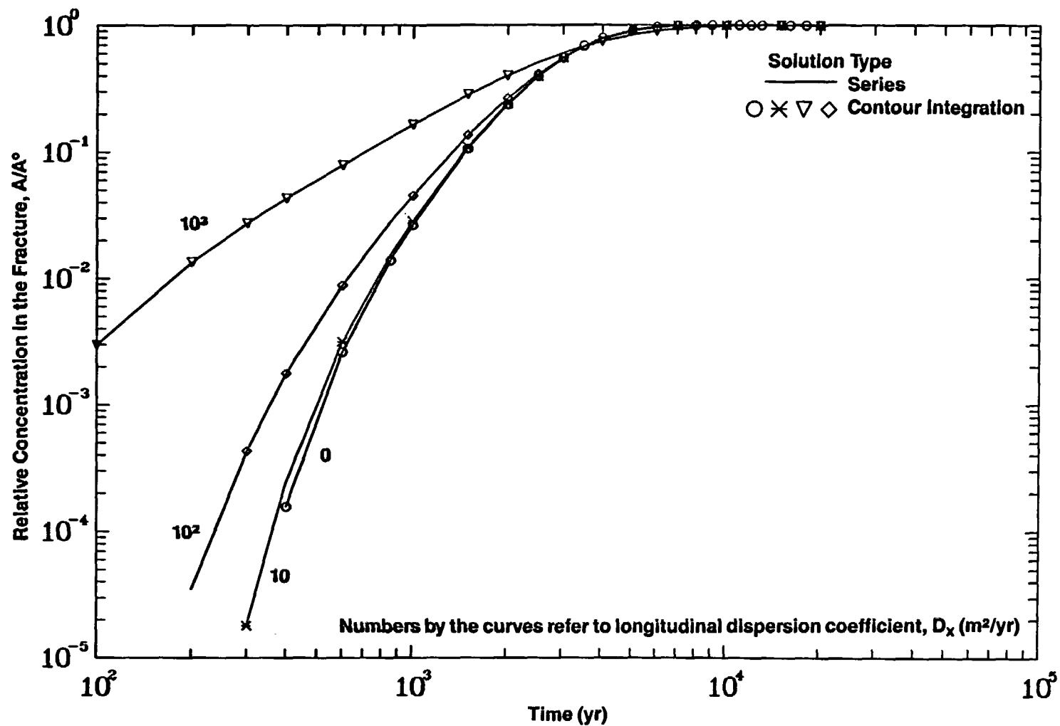
Figure 6-3a. Comparison of Temporal Variation of Relative Concentration of Np-237 in the Fracture for D_{xx} = 0, 10, 100, 1000 m^2/yr (Case 6A: Multiple Parallel Fractures, Step Release Mode)
