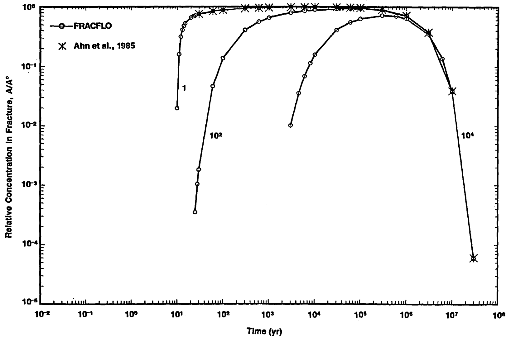
Figure 3-1e. Breakthrough Curves Showing Relative Concentrations of Np-237 in the Fracture Versus Time at x = 100 m and y = 0 m for Different Rock Matrix Retardation Factors ( R' = 1, 10^2, 10^4 ) (Case 1A: Step Release Mode)
