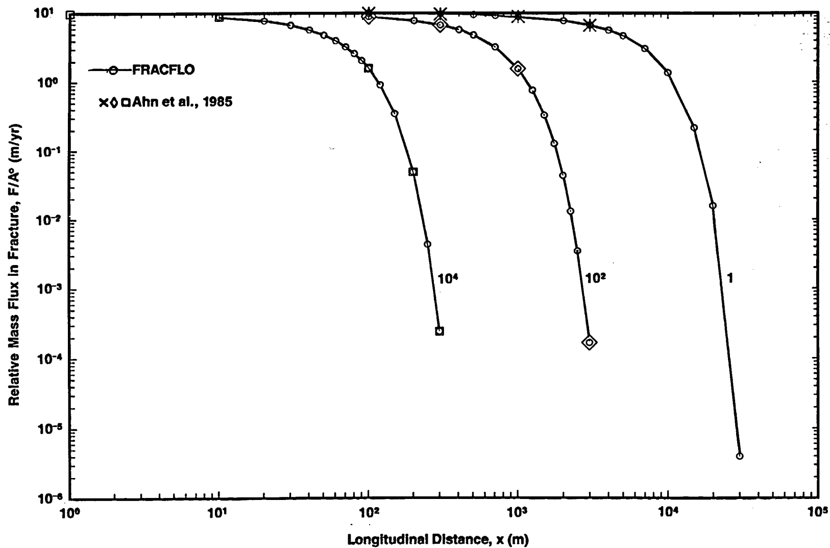
Figure 3-1c. Relative Mass Flux of Np-237 in the Fracture Versus Distance x at y = 0 m and t = 10^4 yr for Different Rock Matrix Retardation Factors ( R' = 1, 10^2, 10^4 ) (Case 1A: Step Release Mode)
