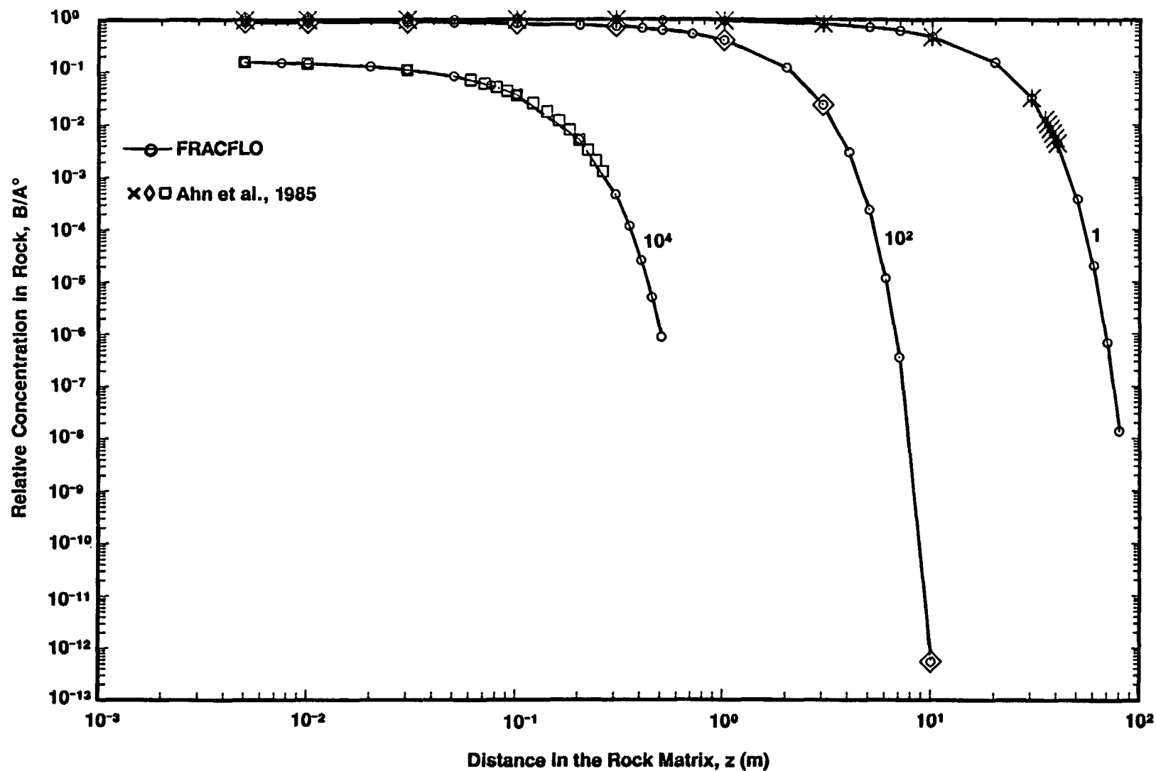
Figure 3-2b. Relative Concentrations of Np-237 in the Rock Matrix Versus Distance In the Rock Matrix at x = 100 m, y = 0 m, t = 10^4 yr, and D_{xx} = 0 for Different Rock Matrix Retardation Factors ( R' = 1, 10^2, 10^4 ) (Case 1B: Step Release Mode)
