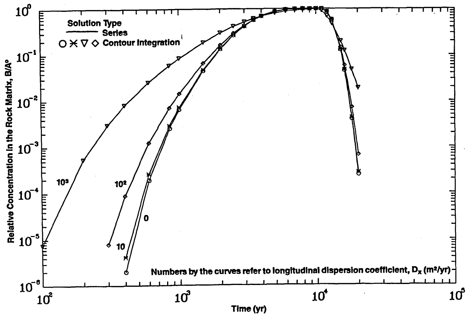
Figure 6-4d. Comparison of Temporal Variation of Relative Concentration of Np-237 In the Rock Matrix at Elevation z = 0.3 m for D_{xx} = 0, 10, 100, 1000 m²/yr (Case 6B: Multiple Parallel Fractures, Band Release Mode)
