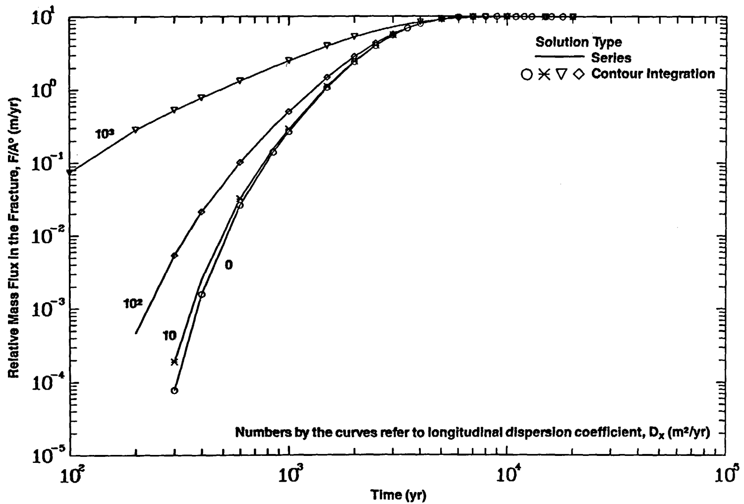
Figure 6-3b. Comparison of Temporal Variation of Relative Mass Flux of Np-237 in the Fracture for D_{xx} = 0, 10, 100, 1000 m²/yr (Case 6A: Multiple Parallel Fractures, Step Release Mode)
