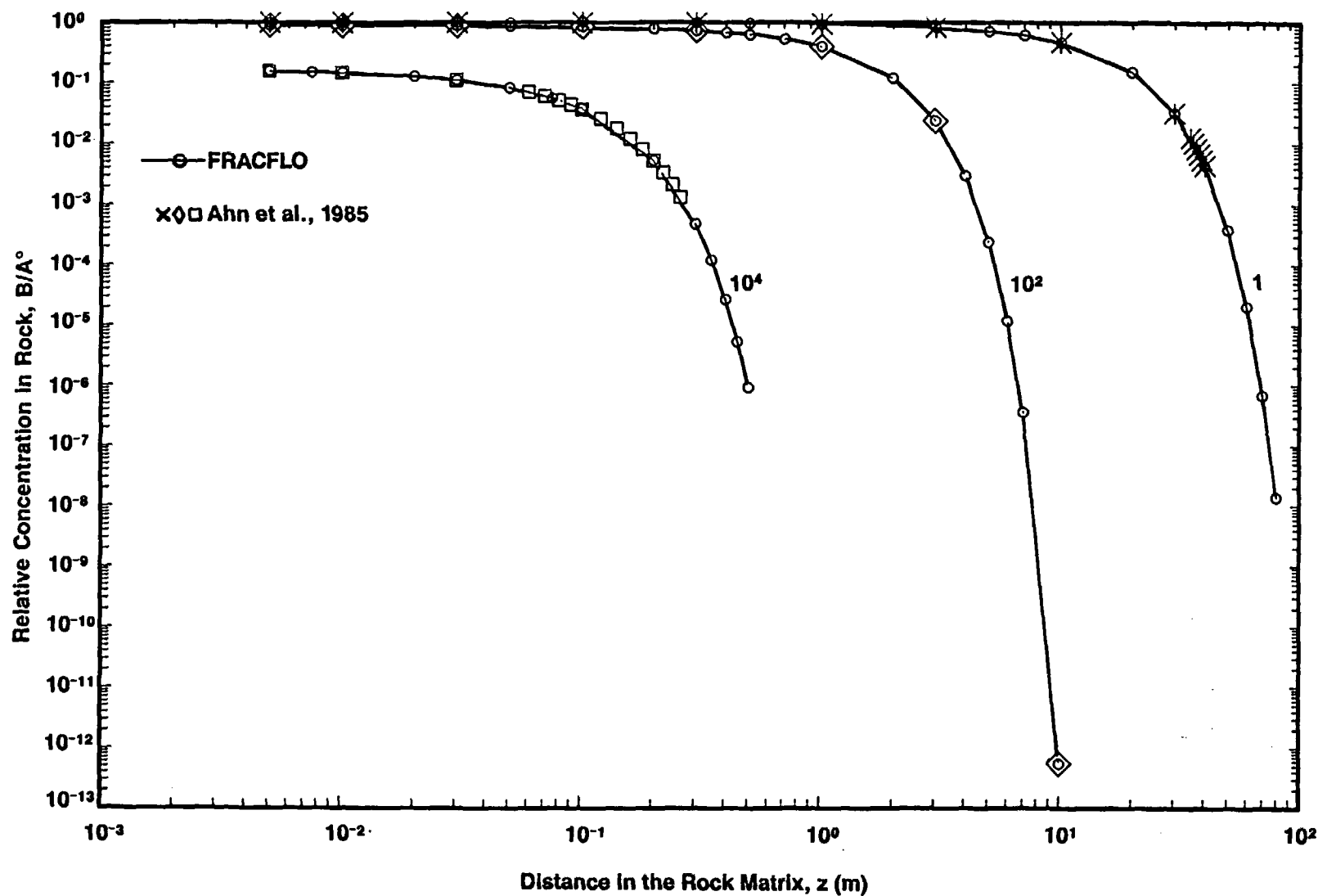
Figure 3-1b. Relative Concentrations of Np-237 In the Rock Matrix Versus Distance In the Rock Matrix z at x = 100 m, y = 0 m, and t = 10^4 yr for Different Rock Matrix Retardation Factors ( R' = 1, 10^2, 10^4 ) (Case 1A: Step Release Mode)
