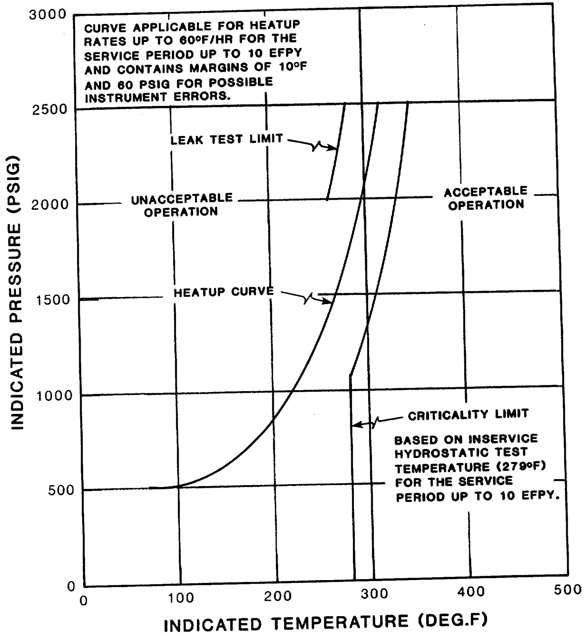
FIGURE 3.4-2 BEAVER VALLEY UNIT 2 REACTOR COOLANT SYSTEM HEATUP LIMITATIONS APPLICABLE FOR THE FIRST 10 EFY
