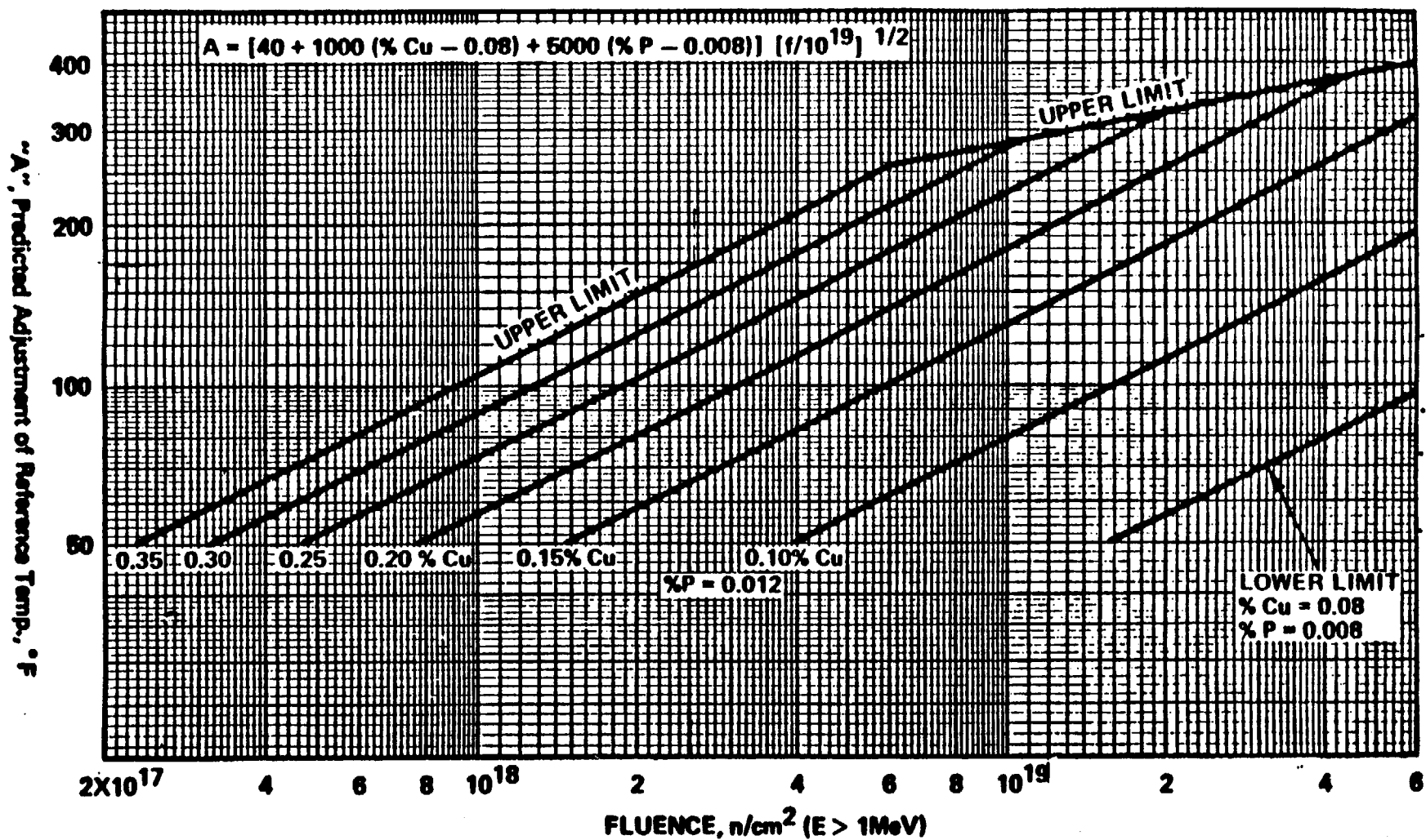
Figure B 3/4.4-2 Predicted Adjustment of Reference Temperature, "A", as a Function of Fluence and Copper Content For Copper and Phosphorus Contents Other Than Those Plotted, Use the Expression for "A" Given on the Figure
