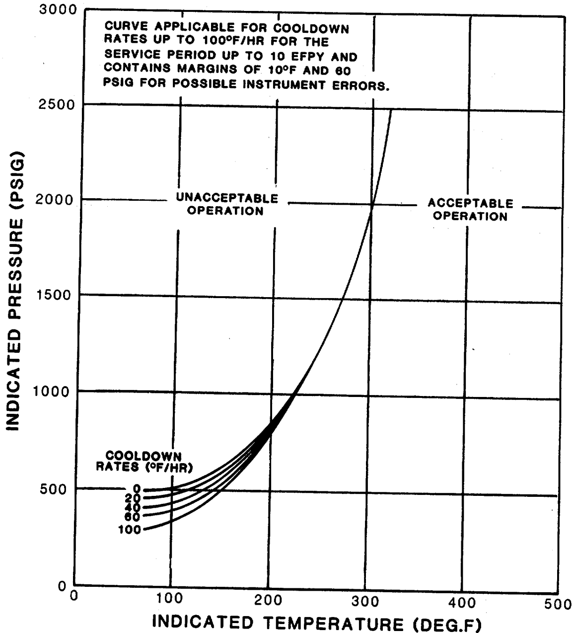
FIGURE 3.4-3 BEAVER VALLEY UNIT NO. 2 REACTOR COOLANT SYSTEM COOLDOWN LIMITATIONS APPLICABLE FOR THE FIRST 10 EFY
