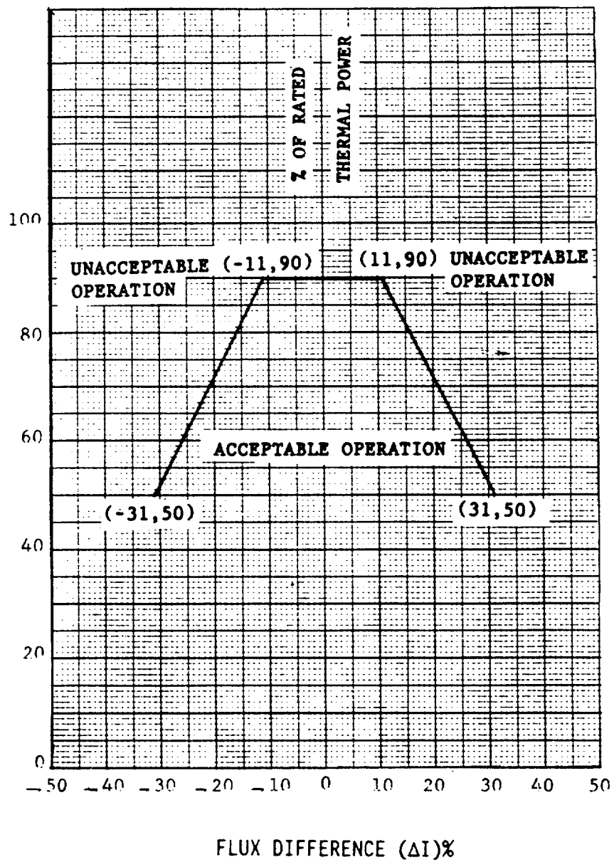
FIGURE 3.2-1 AXIAL FLUX DIFFERENCE LIMITS AS A FUNCTION OF RATED THERMAL POWER
