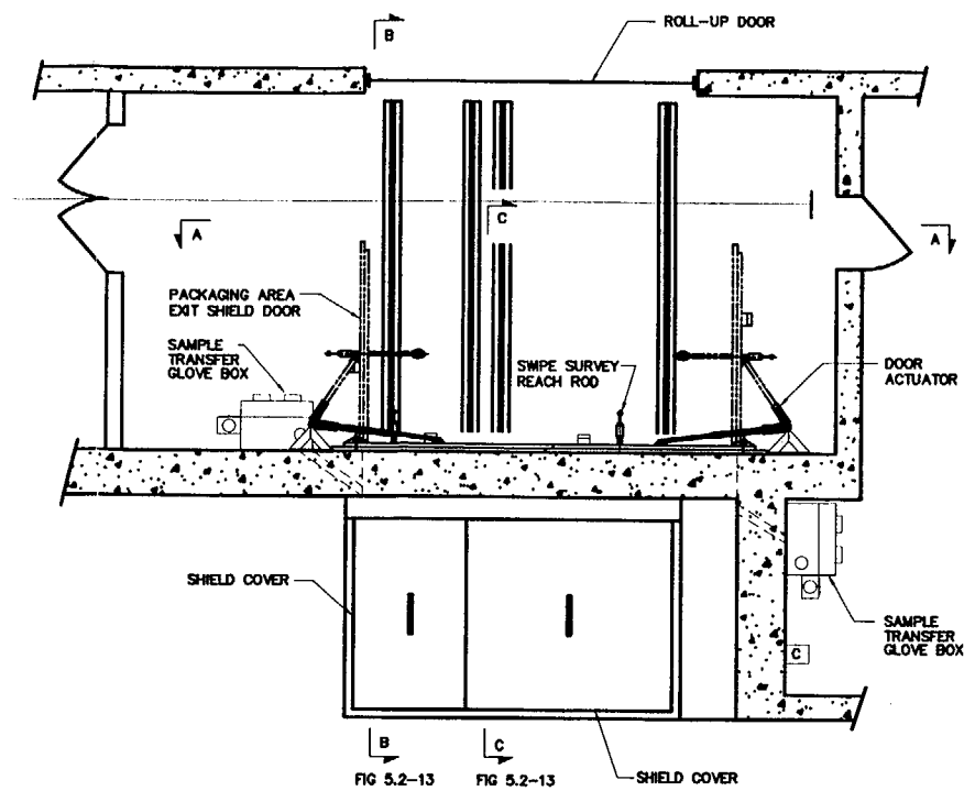
PARTIAL PLAN BELOW EL. 8'-0"
