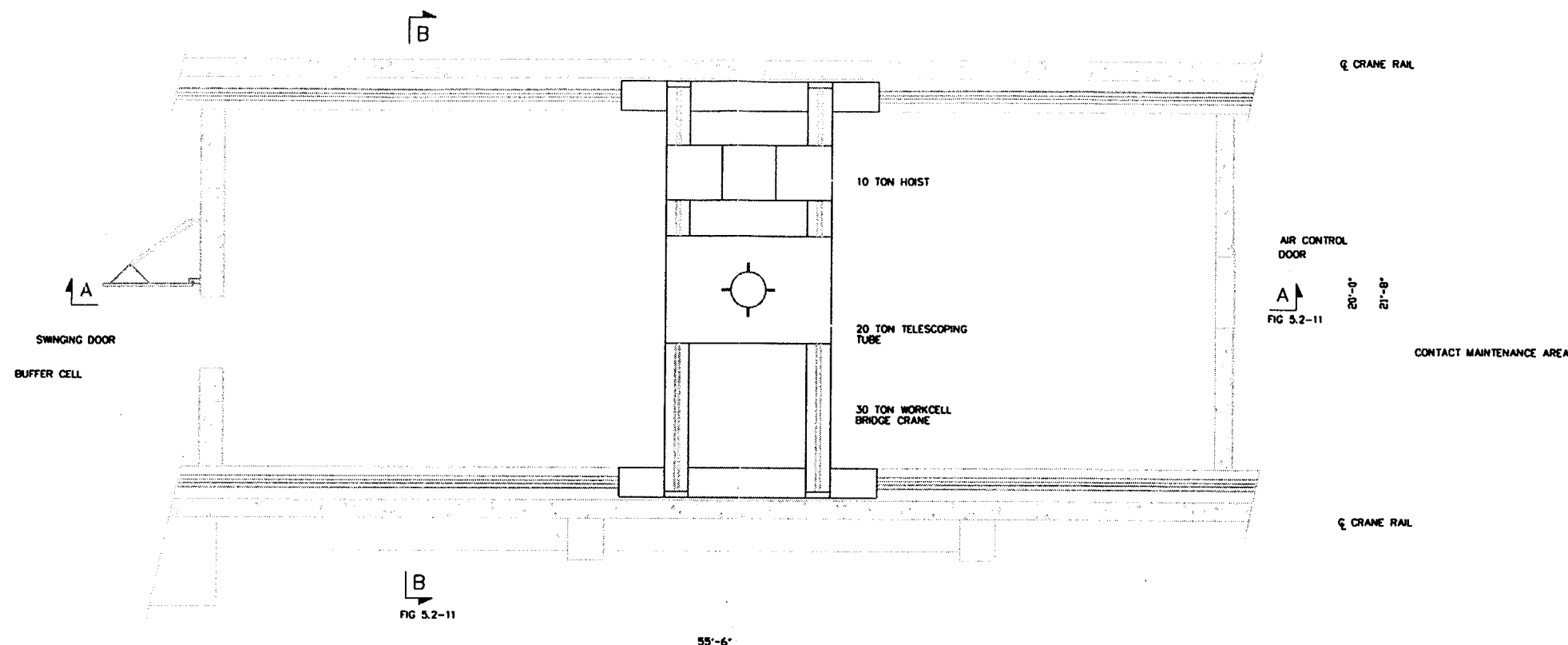
PLAN AT THIRD LEVEL ELEVATION 26'-0" DETAIL AT LOWER LEVELS NOT SHOWN FOR CLARITY
