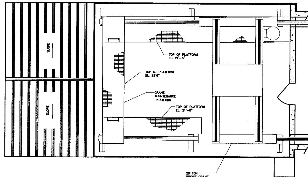
PLAN AT THIRD LEVEL ELEVATION @ 28'-0" DETAIL AT LOWER LEVELS NOT SHOWN FOR CLARITY
