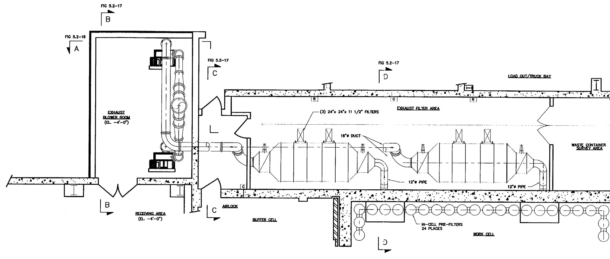
PARTIAL PLAN AT FIRST LEVEL FINISHED FLOOR ELEVATION 0'-0"
