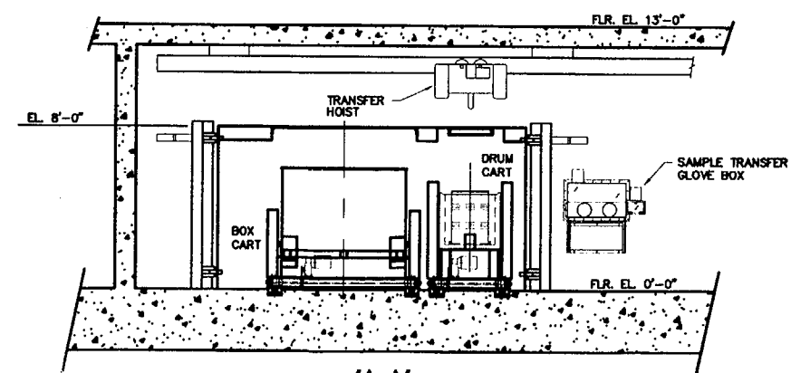
"A-A" SHIELD DOOR OPEN
