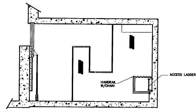
SUSPENDED INTERMEDIATE LEVEL PLATFORMS ELEVATION @ 5'-4" & 15'-5" DETAIL AT FIRST LEVEL NOT SHOWN FOR CLARITY
