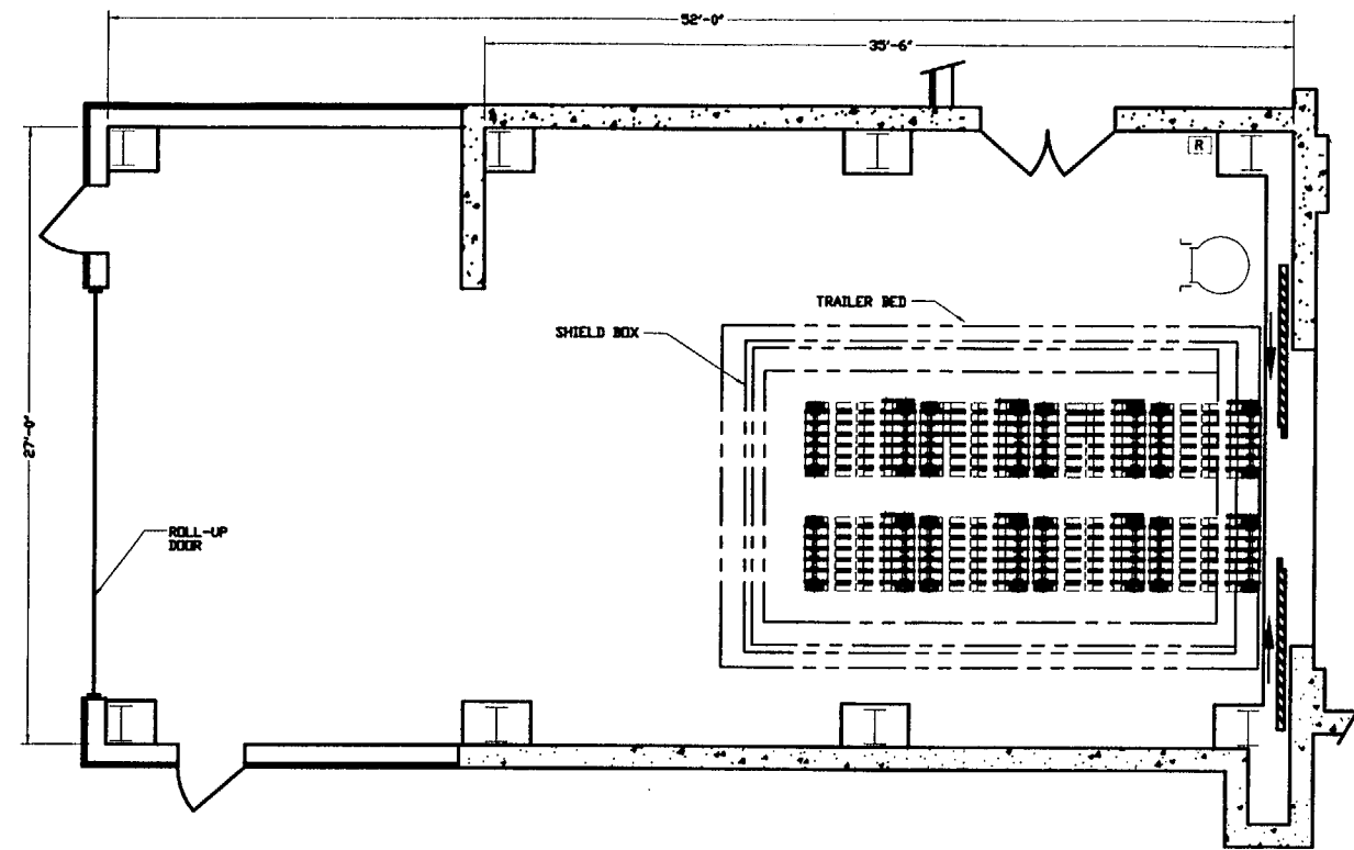
PLAN AT FIRST LEVEL ELEVATION @ -4'-0"
