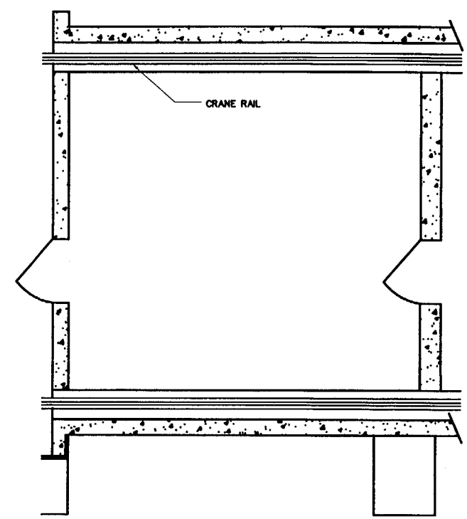
PLAN AT THIRD LEVEL ELEVATION @ 26'-0" DETAIL AT LOWER LEVELS NOT SHOWN FOR CLARITY
