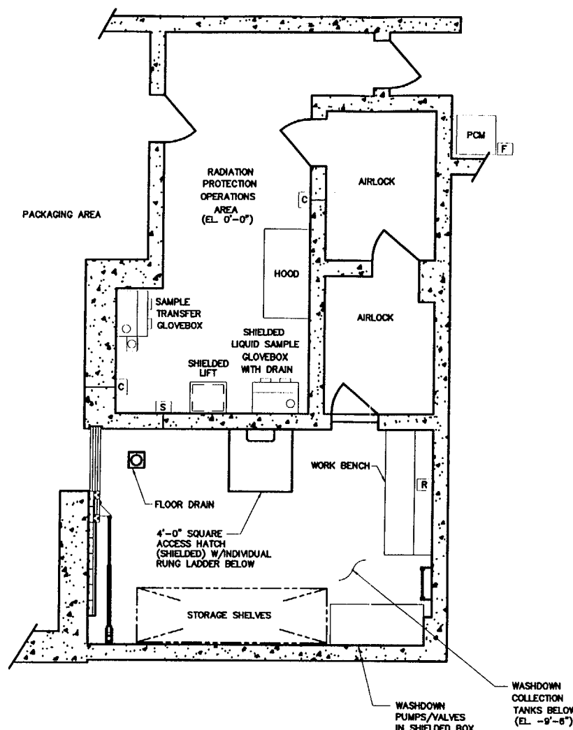
PLAN AT FIRST LEVEL ELEVATION @ 0'-0"
