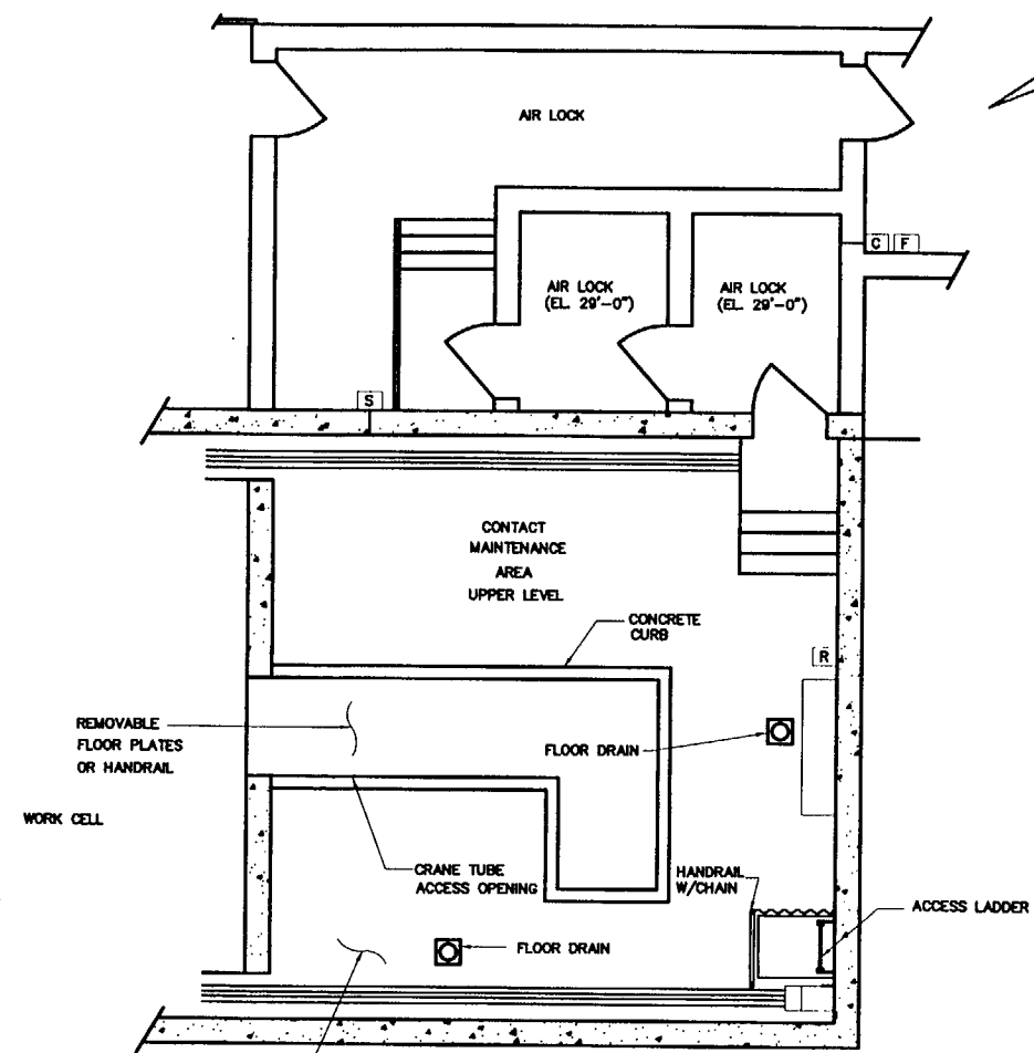
PLAN AT THIRD LEVEL ELEVATION @ 29'-0"
