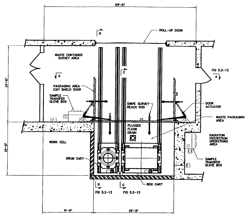
PARTIAL PLAN BELOW EL. 8'-0"
