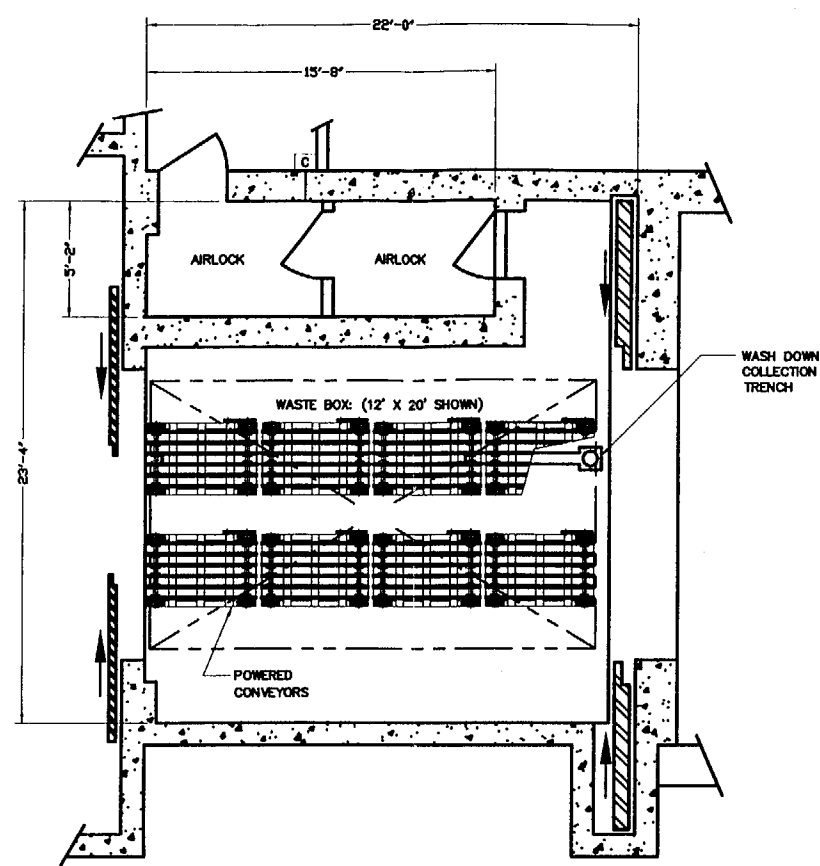
PLAN AT FIRST LEVEL ELEVATION @ 0'-0"
