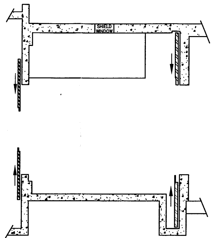
PLAN AT SECOND LEVEL ELEVATION @ 13'-0" DETAIL AT FIRST LEVEL NOT SHOWN FOR CLARITY
