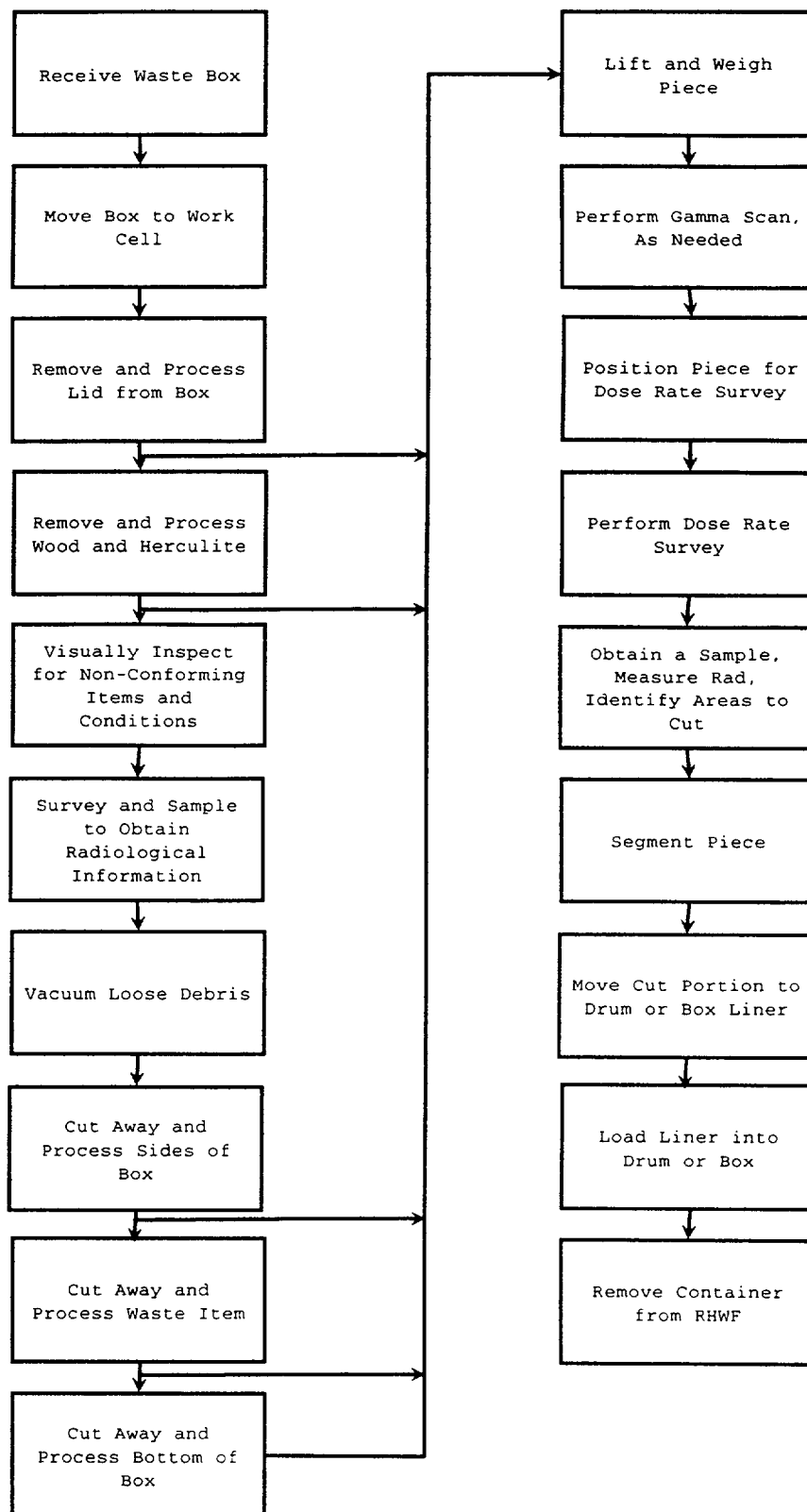
Figure 1.3-1. Remote-Handled Waste Facility Simplified Process Flow Diagram
