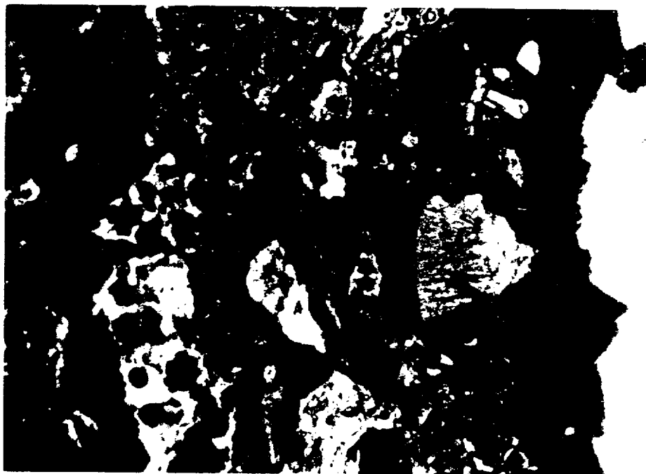
Figure 10. Photomicrograph of sample YMSC 14. Calcrete layer in bedded tuff containing pumice fragments and a partial spherulite in fine calcite with dark granules. Field of view is 3 mm x 2 mm. Plane-polarized light.
