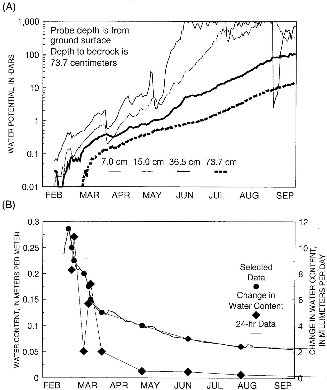
Figure 6-6. Graphs of water-potential measurements near borehole USW UZ-N15 using heat dissipation probes, (DTN: GS960908312211.004), (A) measured at four depths for 1995 and (B) used to calculate flux.
