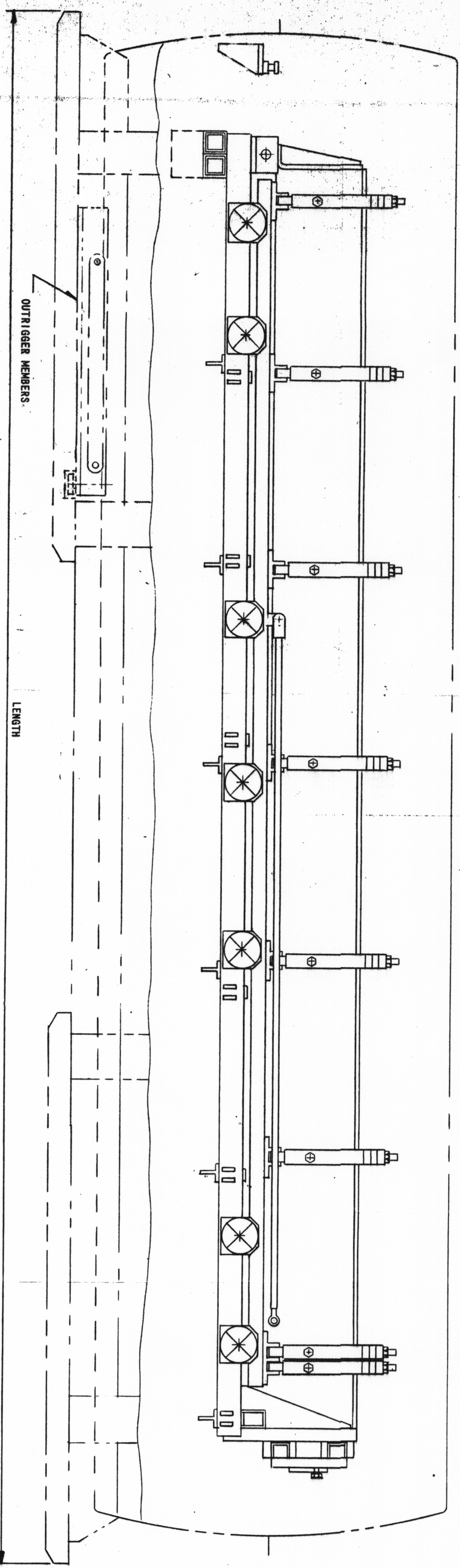
ARRANGEMENT OF SHIPPING CONTAINER DURING SHIPPING
