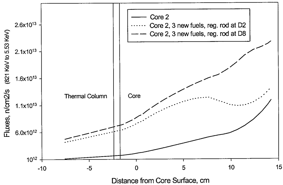
Figure 3. Neutron Leakage (821 KeV to 5.53 KeV) near the Core-Thermal Column Interface
