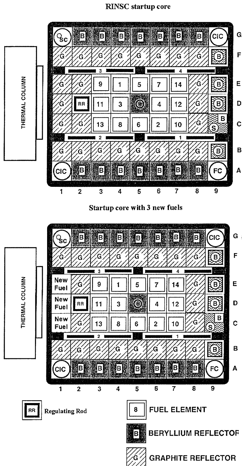
Figure 4. Fresh Core Models in the RINSC Thermal Hydraulic Calculations
