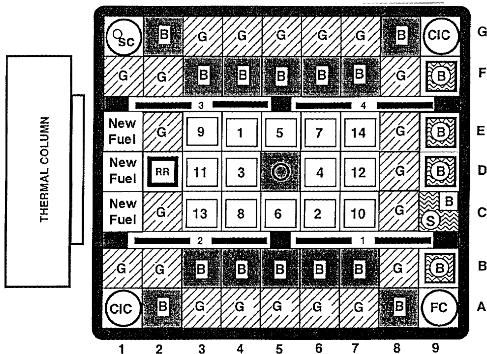
Figure 2. Expanded Core with Additional Fuel Elements to Increase Fast Leakage.
