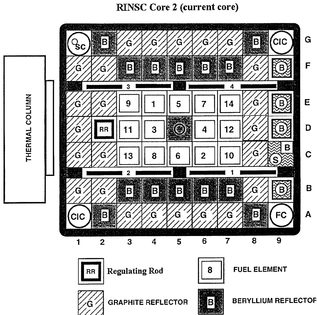
Figure 1. RINSC Core 2 (current core)
