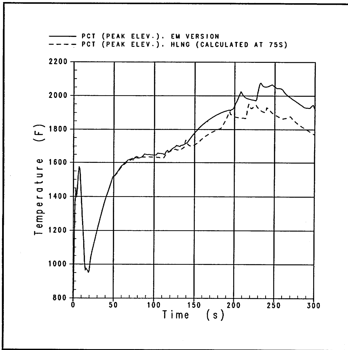
Figure 7 4-loop, Late Reflood PCT Peak Cladding Temperature (°F) Hot Leg Nozzle Gap (Calculated from 75s Gap)
