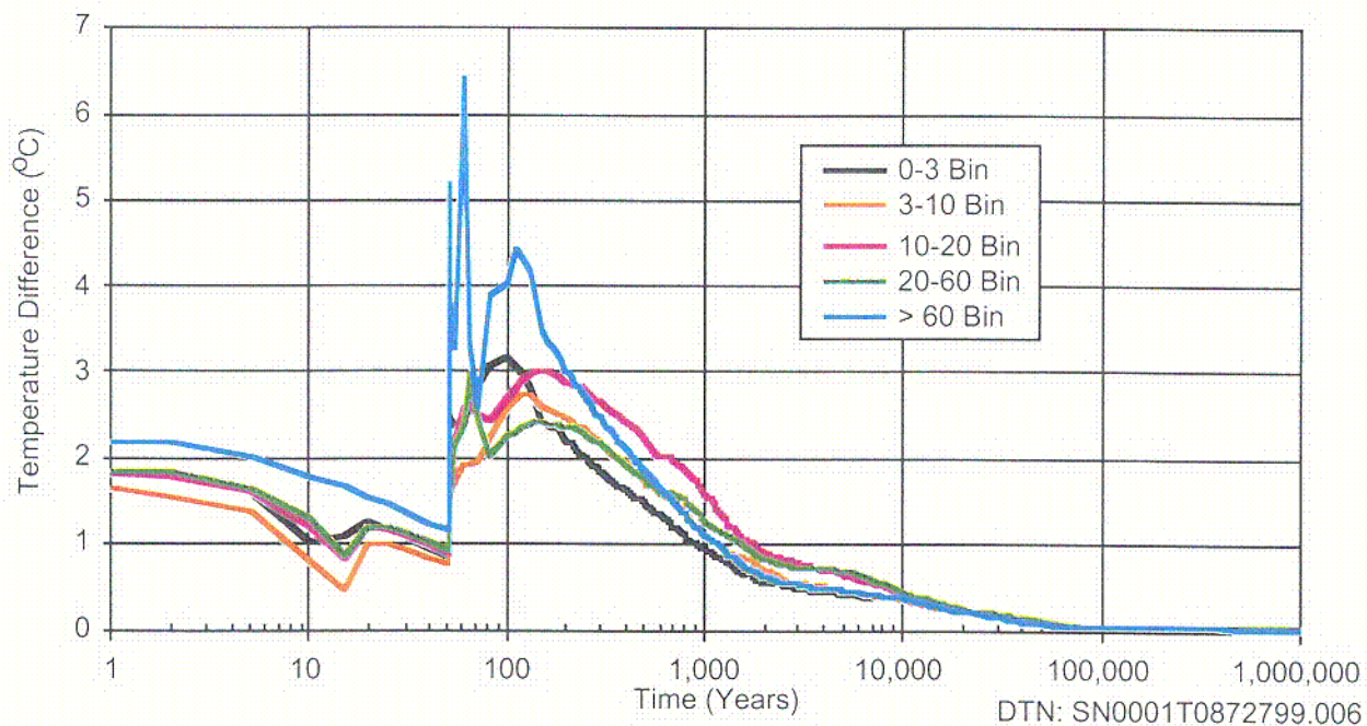
Figure 1. Difference Between CSNF and HLW Upper Drift Wall Temperatures, Drift-Scale Property Set, Site Recommendation Base Case with Backfill, Mean Infiltration Case
