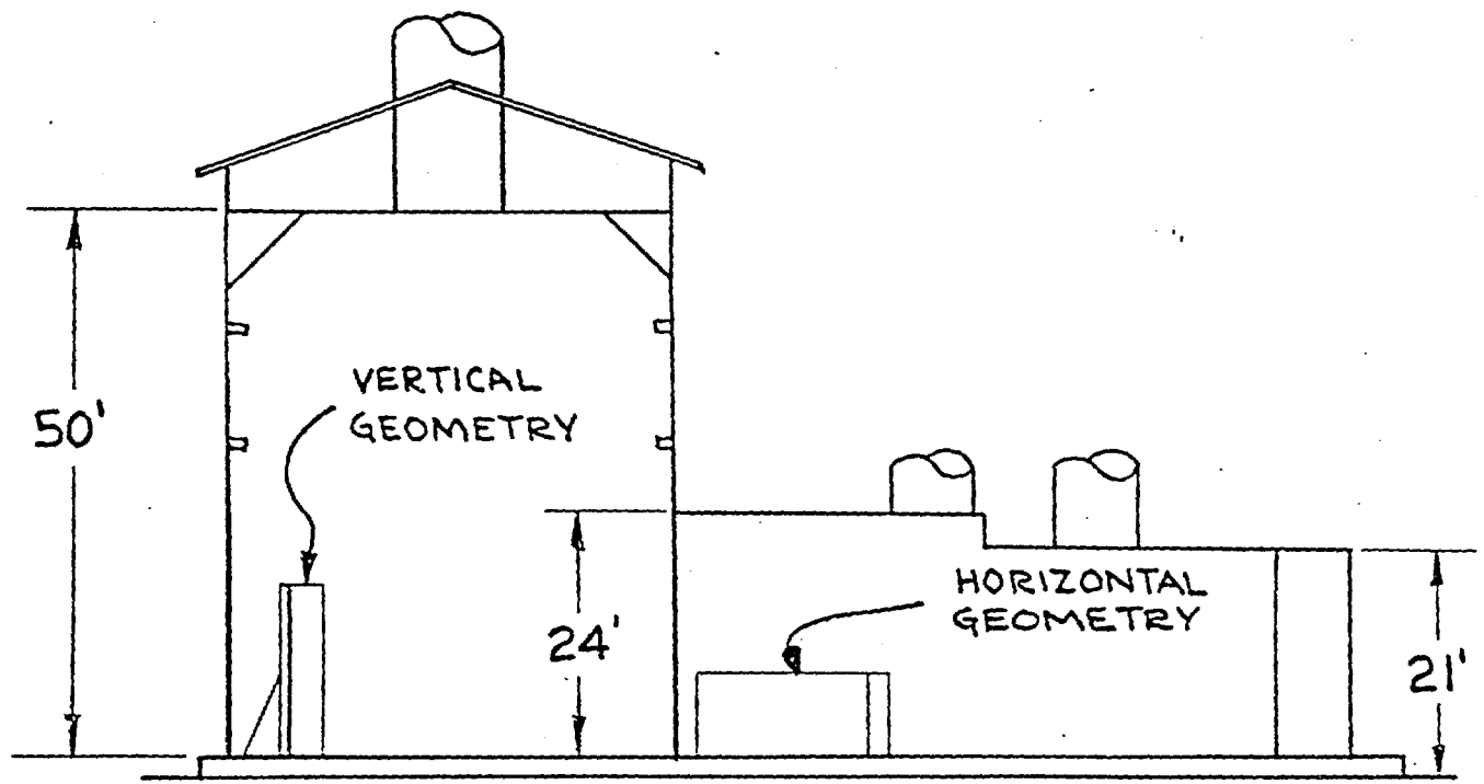
ELEVATION VIEW
