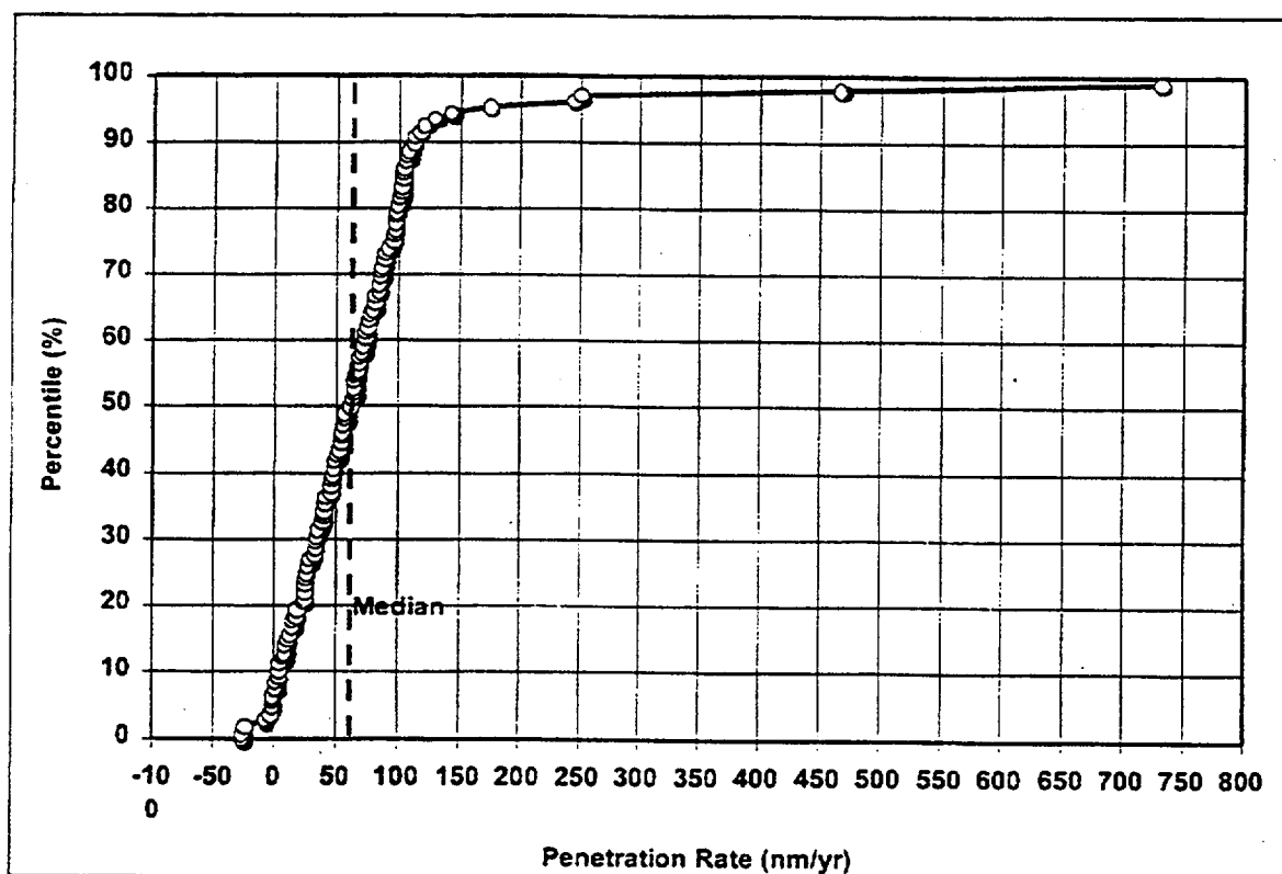
Figure 25. GC of Alloy 22, 6, and 12 Month Crevice Samples from LTCTF, Percentile Versus Corrosion Rate
