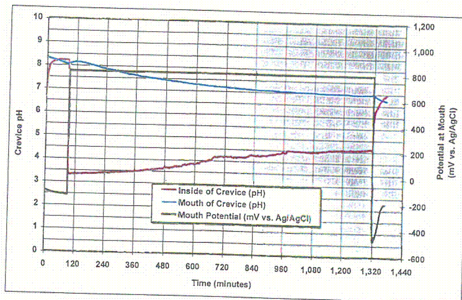
Figure 37. Stainless Steel 316L, 4M NaCl, 200 mV and 23 °C, Crevice pH Versus Time
