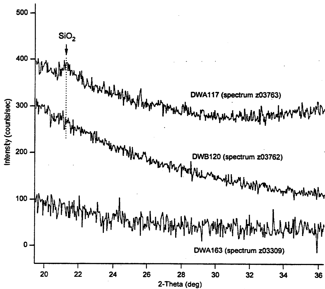
Figure 22. SCW Test Coupons: X-Ray Spectra of Scales on SCW Test Coupons
