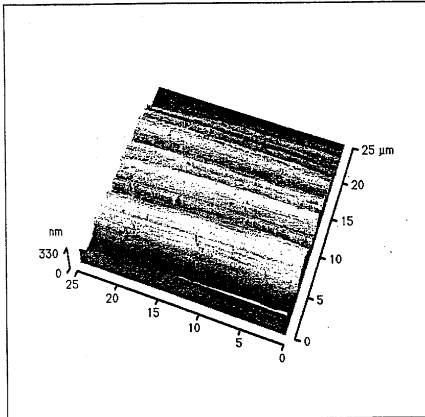
Figure 27. AFM Image of Alloy 22 Control Sample
