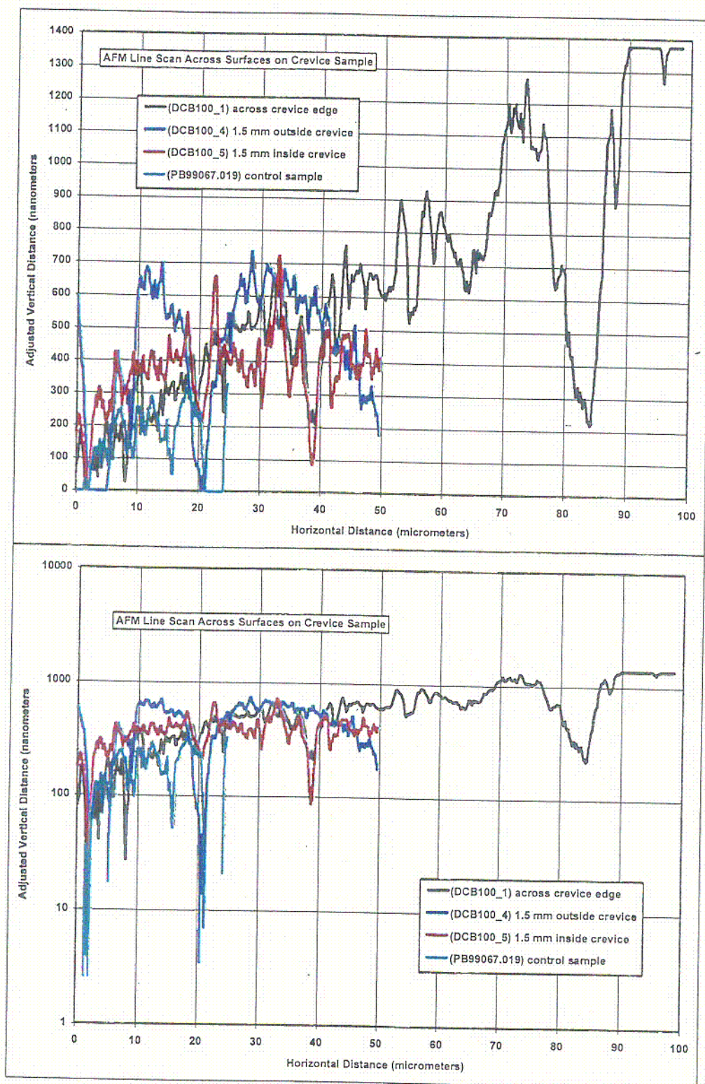
Figure 35. A Comparison of AFM Line Scans across Different Regions of Exposed Crevice Sample, with Comparison to Line Scan on Surface of Unexposed Control Sample
