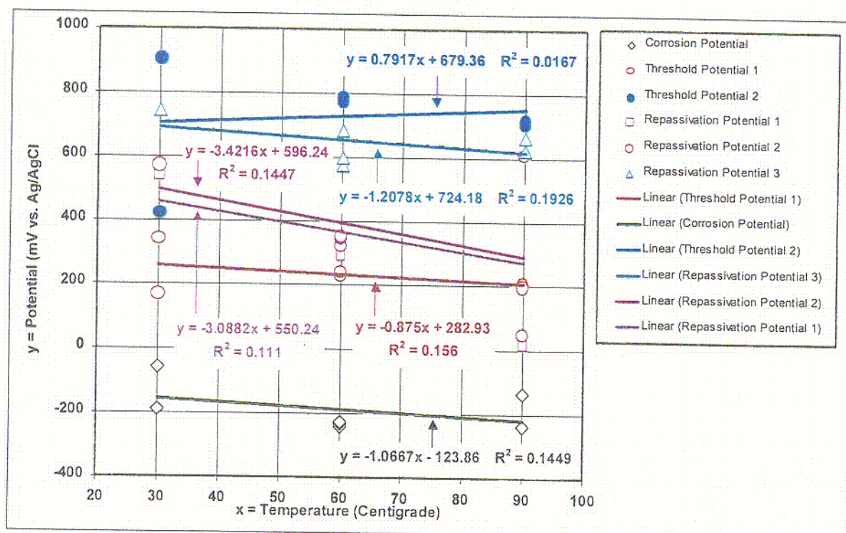
Figure 12. Potentials Versus Temperature: Alloy 22 in SDW
