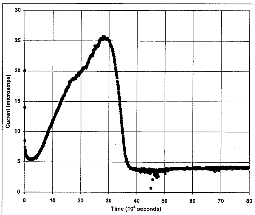
Figure 10. Potentiostatic Polarization of Alloy 22 in SCW at 90°C and 200mV Versus Ag/AgCl
