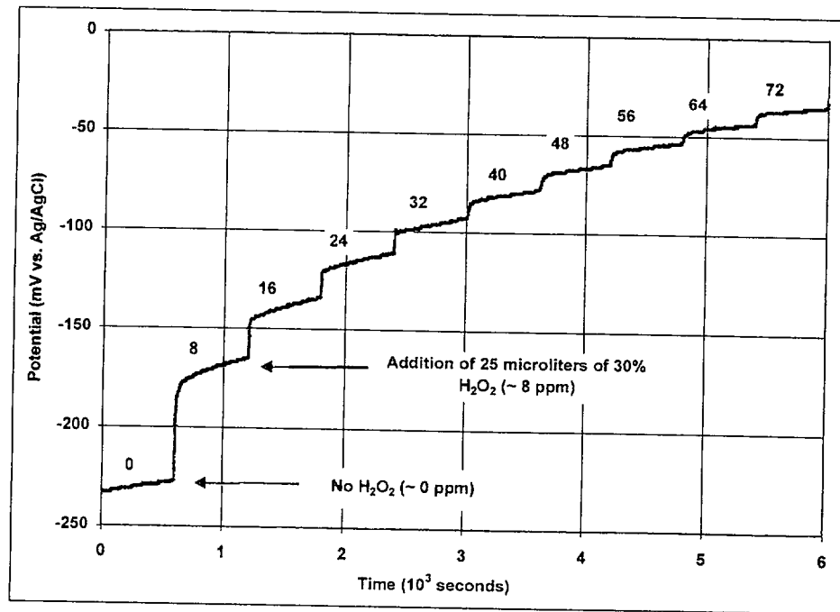
Figure 17. Effect of Hydrogen Peroxide on Corrosion Potential of Alloy 22 in SCW at 25°C
