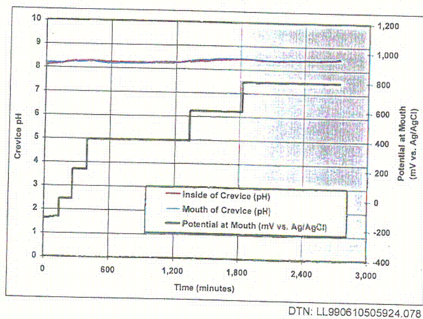
Figure 42. Alloy 22, SCW at 23 °C, Crevice pH Versus Time
