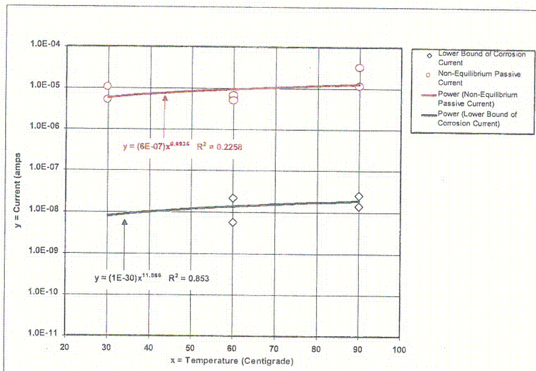
Figure 18. Bounding Currents Versus Temperature, Alloy 22 in SDW
