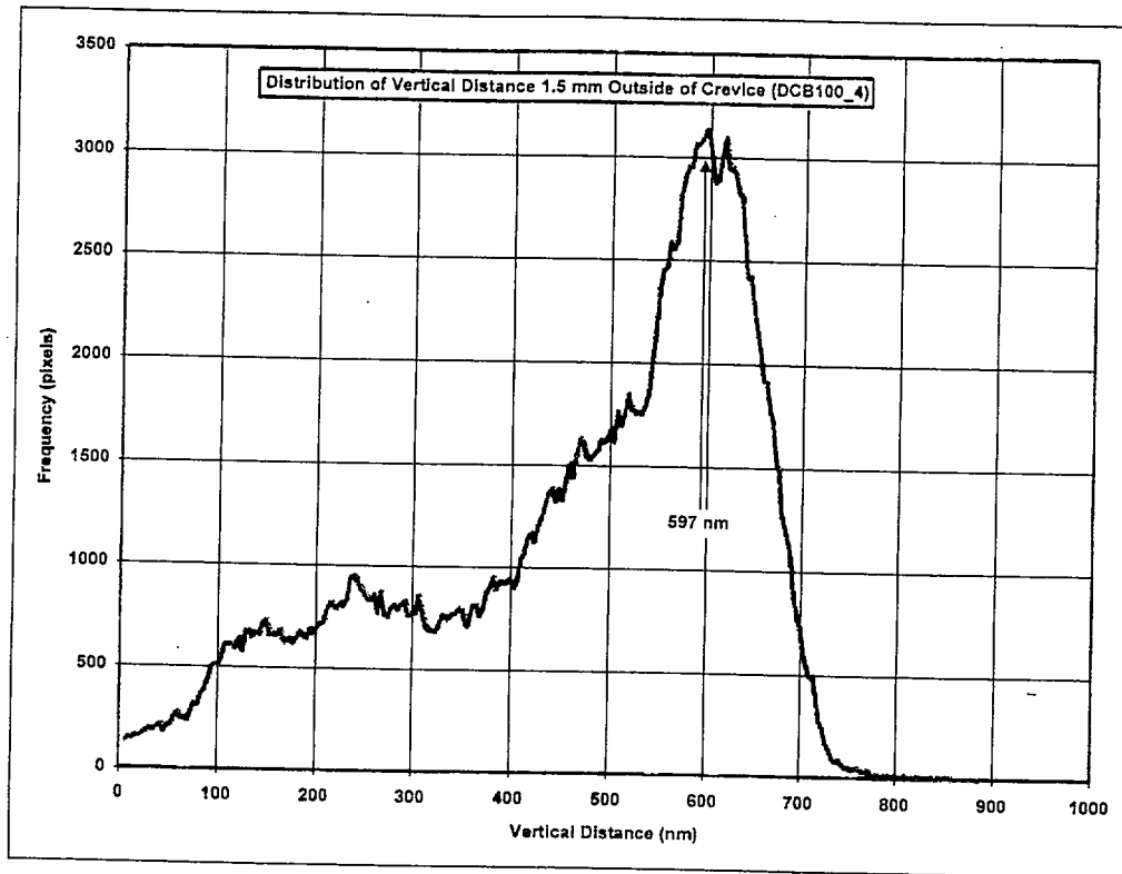
Figure 31. Histogram of AFM Measurements of Vertical Distance made 1.5 mm outside of Crevice (DCB100_4)
