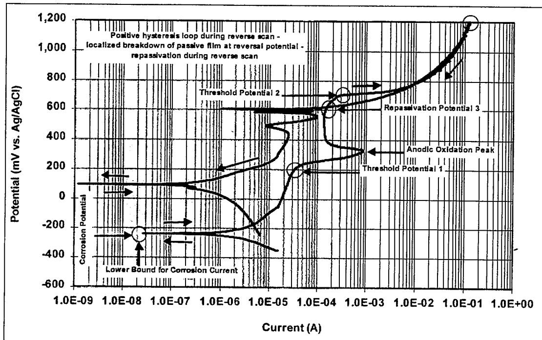
Figure 5. Type 2 – Alloy 22 in SCW at 90°C (DEA016)
