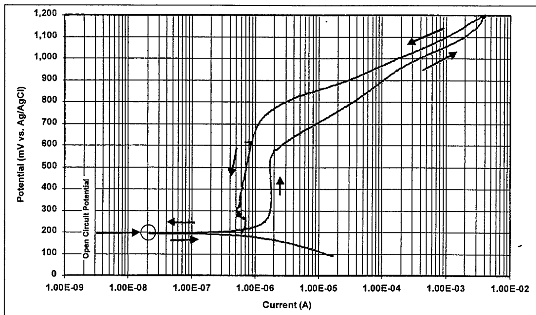
Figure 9. Baseline – Pt in SCW at 90°C (PT001)
