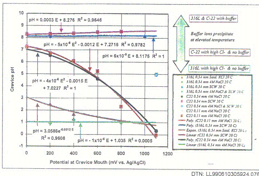
Figure 43. Determination of Crevice pH for WP Materials
