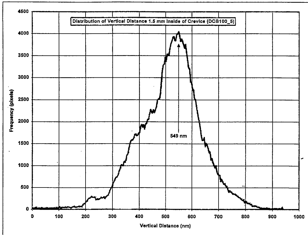
Figure 33. Histogram of AFM Measurements of Vertical Distance made 1.5 mm inside of Crevice (DCB100_5)
