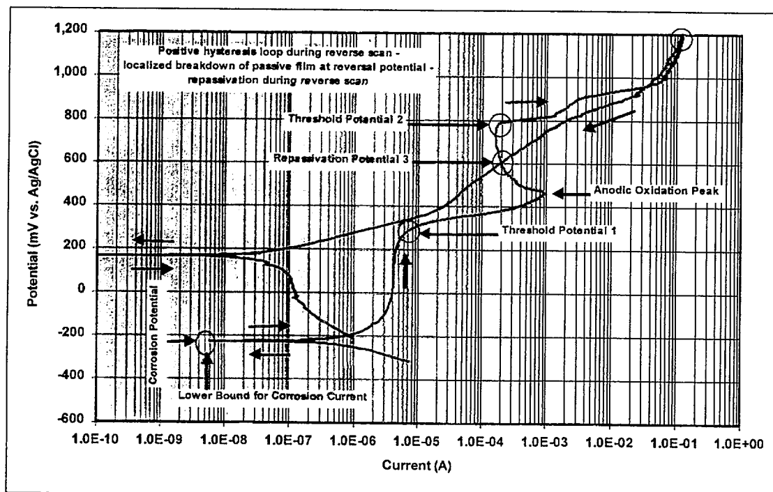
Figure 5. Type 2 – Alloy 22 in SCW at 90°C (DEA016)
