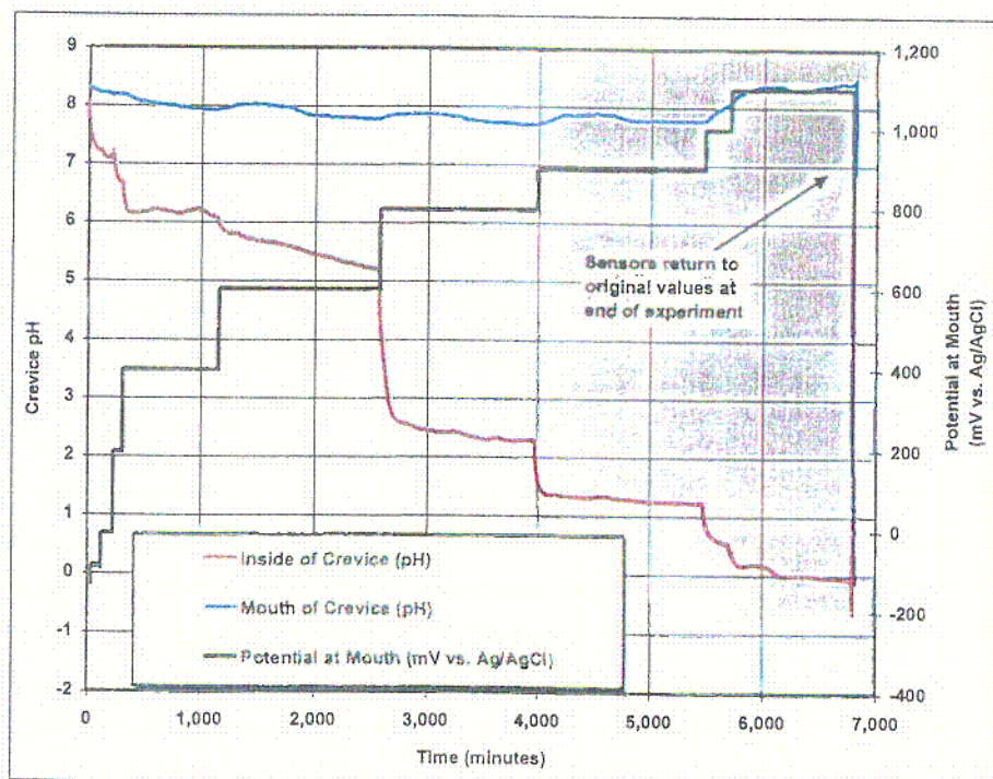
Figure 39. Alloy 22, 4M NaCl, 1100 mV and 20 °C, Crevice pH Versus Time
