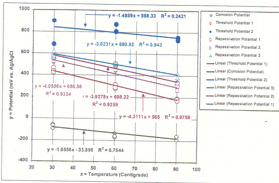
Figure 12. Potentials Versus Temperature: Alloy 22 in SDW
