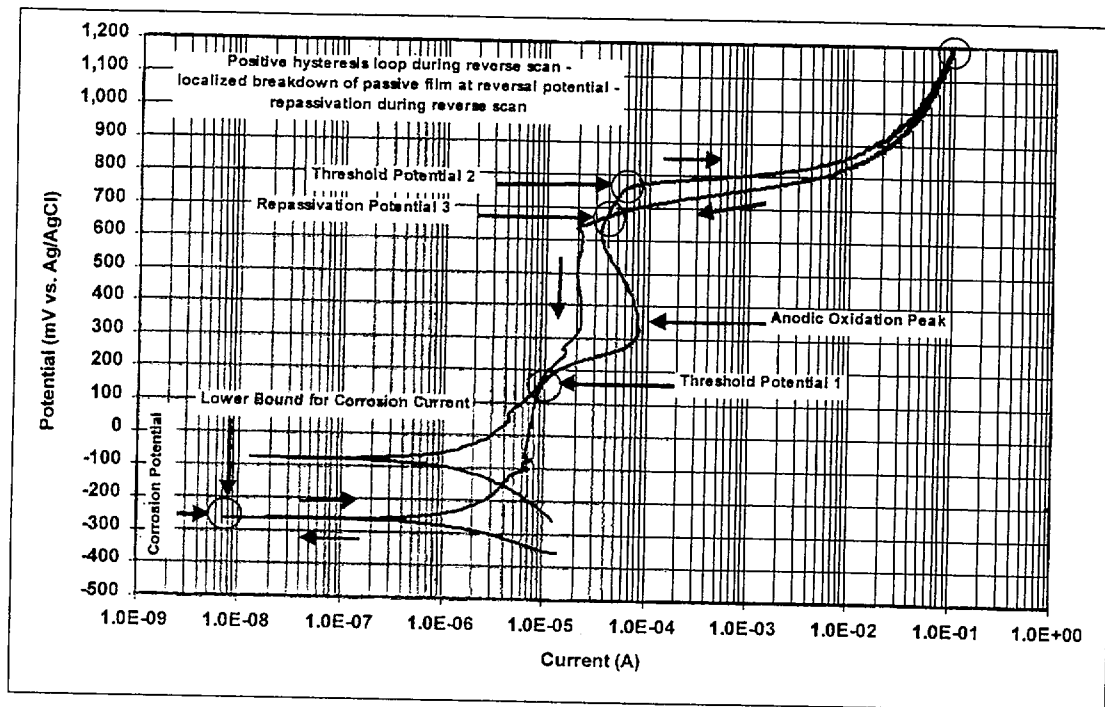
Figure 7. Type 2 - 316L in SCW at 90°C (PEA002)
