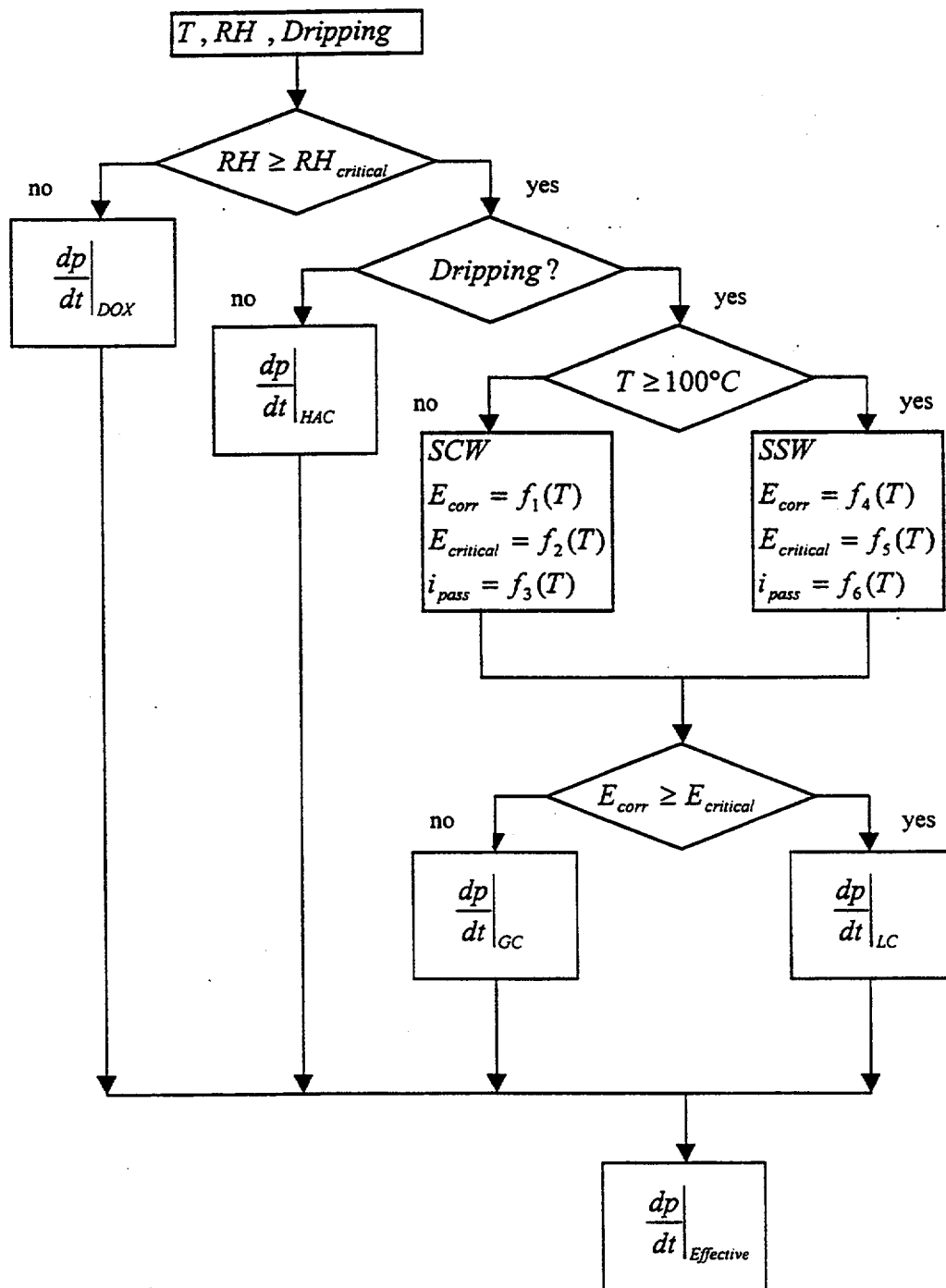
Figure 57. Schematic Representation of Corrosion Model for Alloy 22 Outer Barrier
