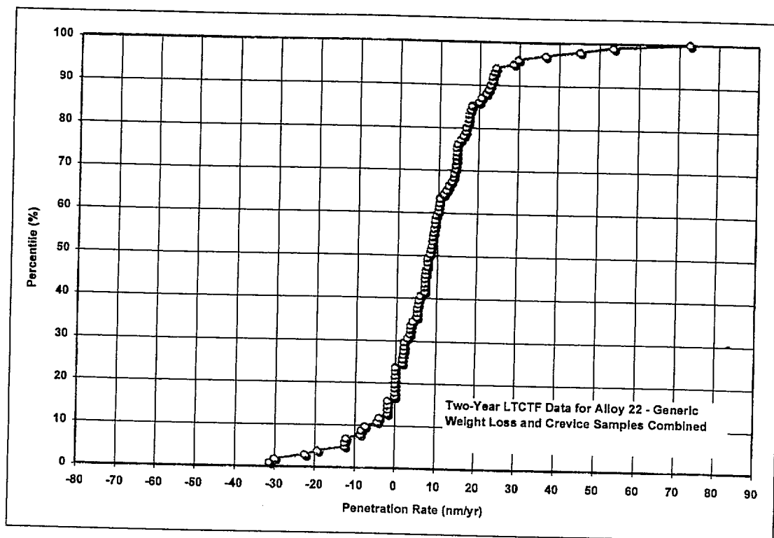
Figure 49. Additional Two-Year GC Corrosion Rate Data from LTCTF Based upon Both Generic Weight Loss and Crevice Samples, including those with Apparent Negative Rates
