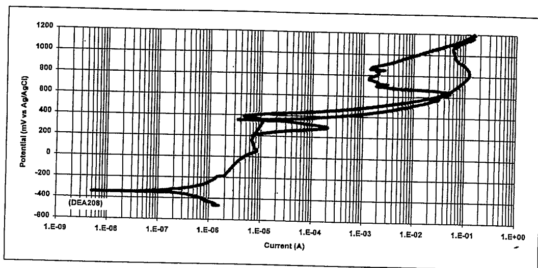
Figure 55. CP Curve for Thermally Alloy 22 in 110°C BSW – Aged at 700°C for 173 Hours (DEA208)
