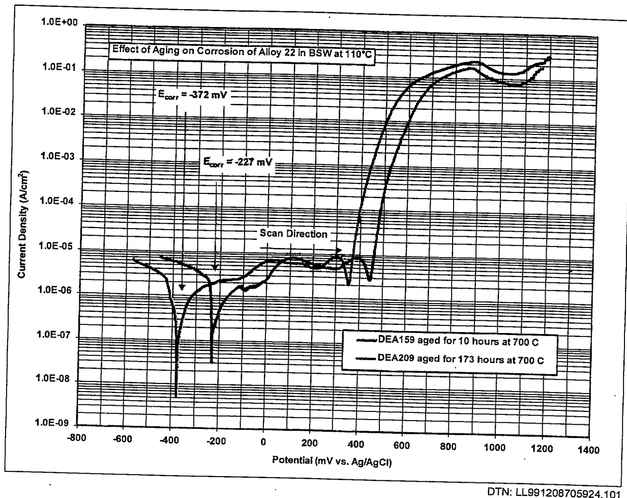
Figure 46. Effect of Thermal Aging at 700°C on the Corrosion Resistance of Alloy 22 in BSW-13 at 110°C (DEA159 and DEA209)
