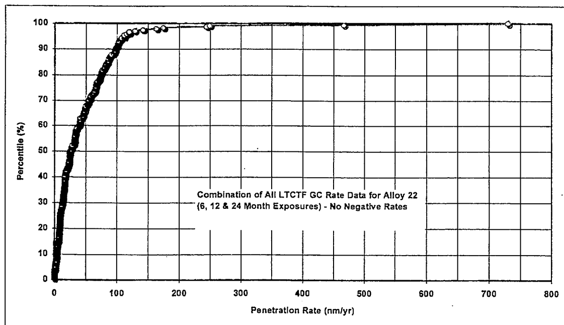
Figure 51. Combination of All GC Rate Data for Alloy 22 from LTCTF, including 6-, 12- and 24-Month (Two-Year) Exposures
