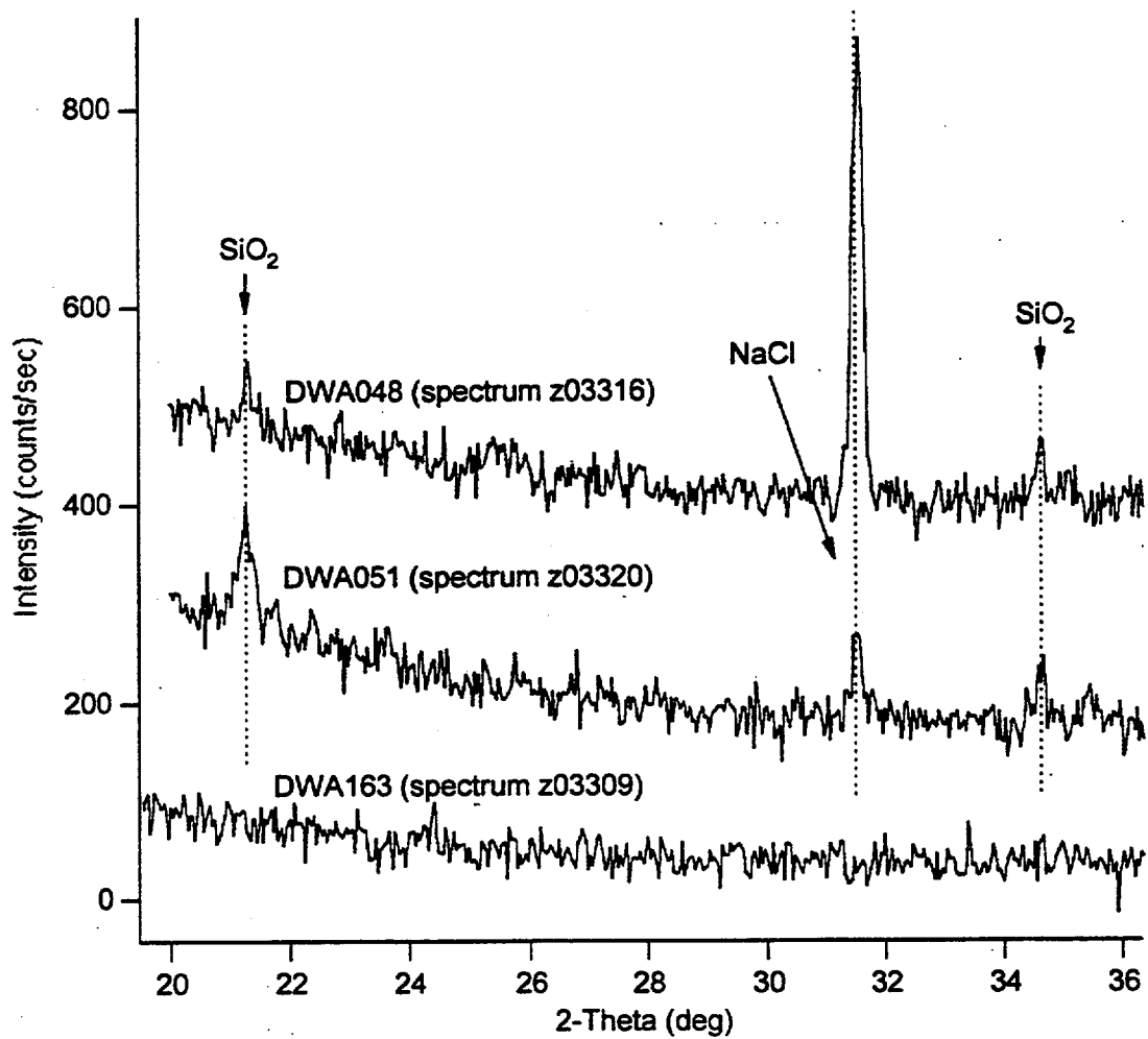
Figure 5. SAW Test Coupons: X-Ray Spectra of scales on SAW Coupons
