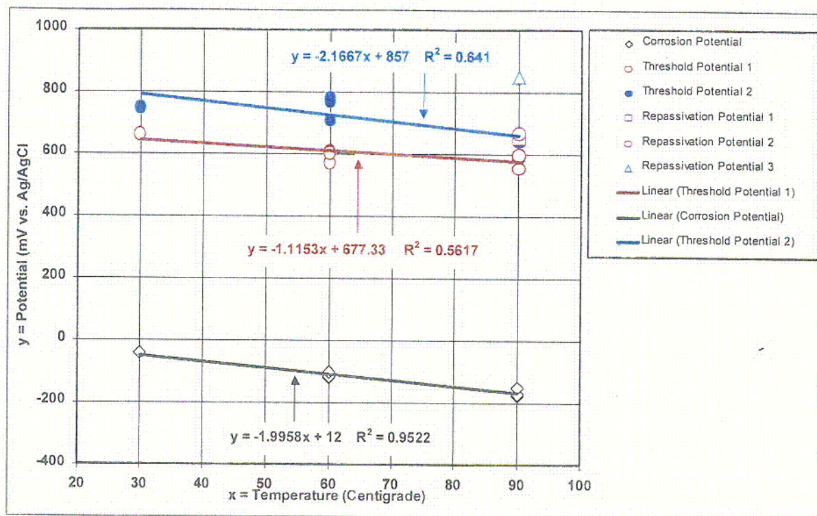
Figure 14. Potentials Versus Temperature: Alloy 22 in SAW
