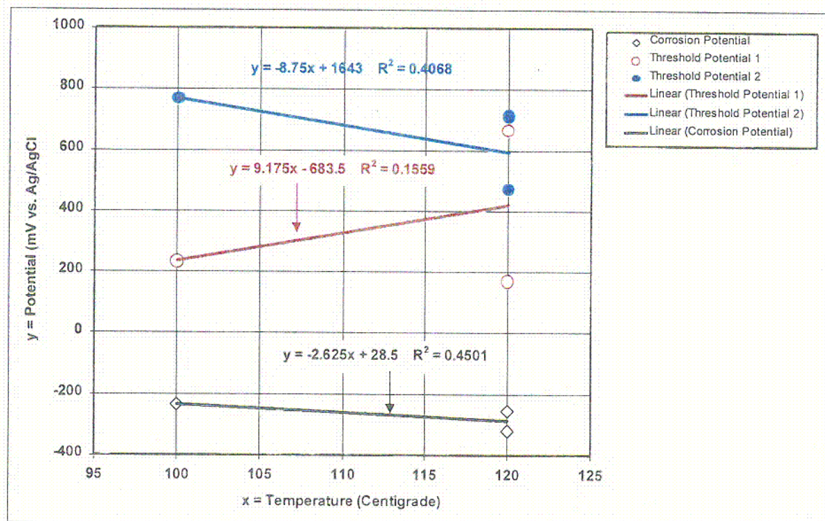
Figure 14. Potentials Versus Temperature: Alloy 22 in SAW
