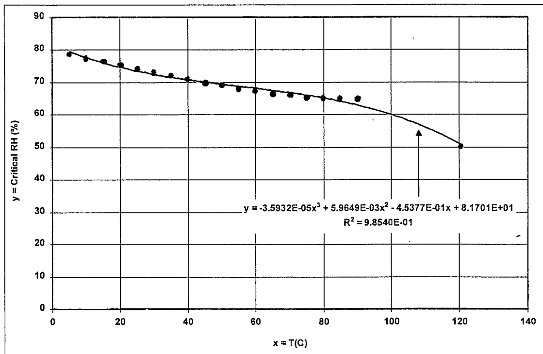
Figure 2. Deliquescence Point for Sodium Nitrate Solutions
