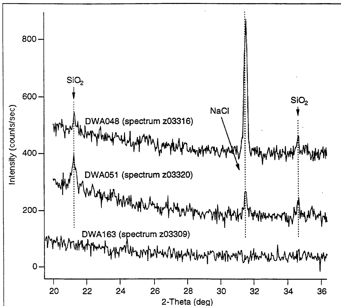
Figure 29. X-ray Diffraction Pattern of Silicate Deposit on-Sample Exposed to LTCTF
