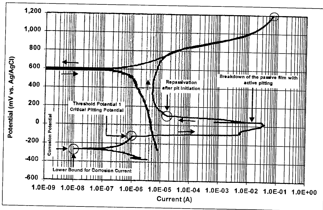
Figure 8. Type 3 - 316L in SSW at 100°C (PEA016)
