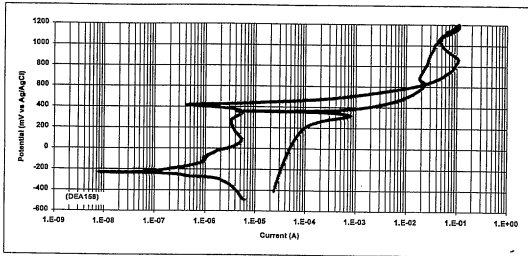
Figure 53. CP Curve for Thermally Alloy 22 in 110°C BSW – Aged at 700°C for 10 Hours (DEA158)
