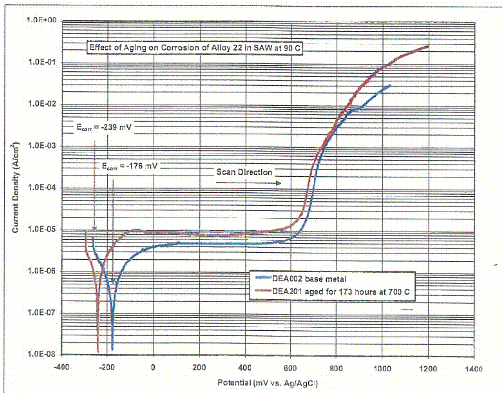
Figure 44. Effect of Thermal Aging for 173 Hours at 700°C on the Corrosion Resistance of Alloy 22 in SAW at 90°C (DEA002 and DEA201)
