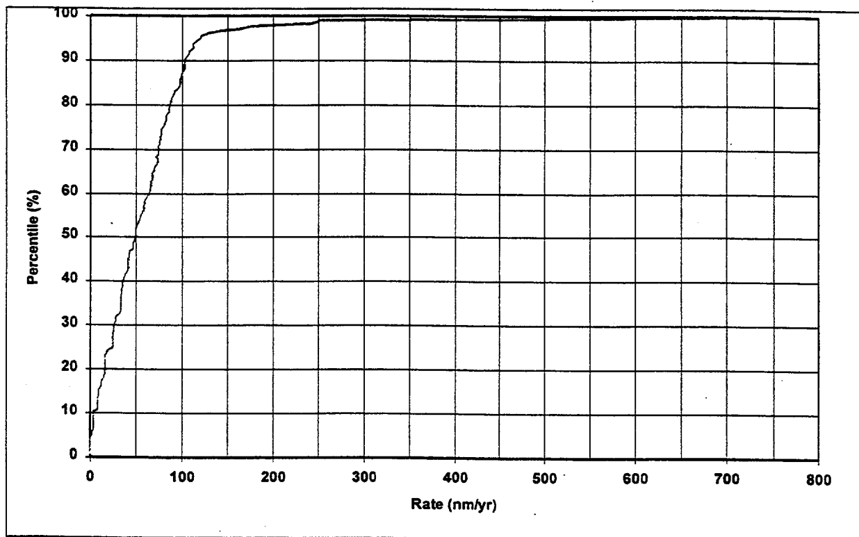
Figure 26. GC Rates of Alloy 22 with Combined Data and Negative Values Neglected
