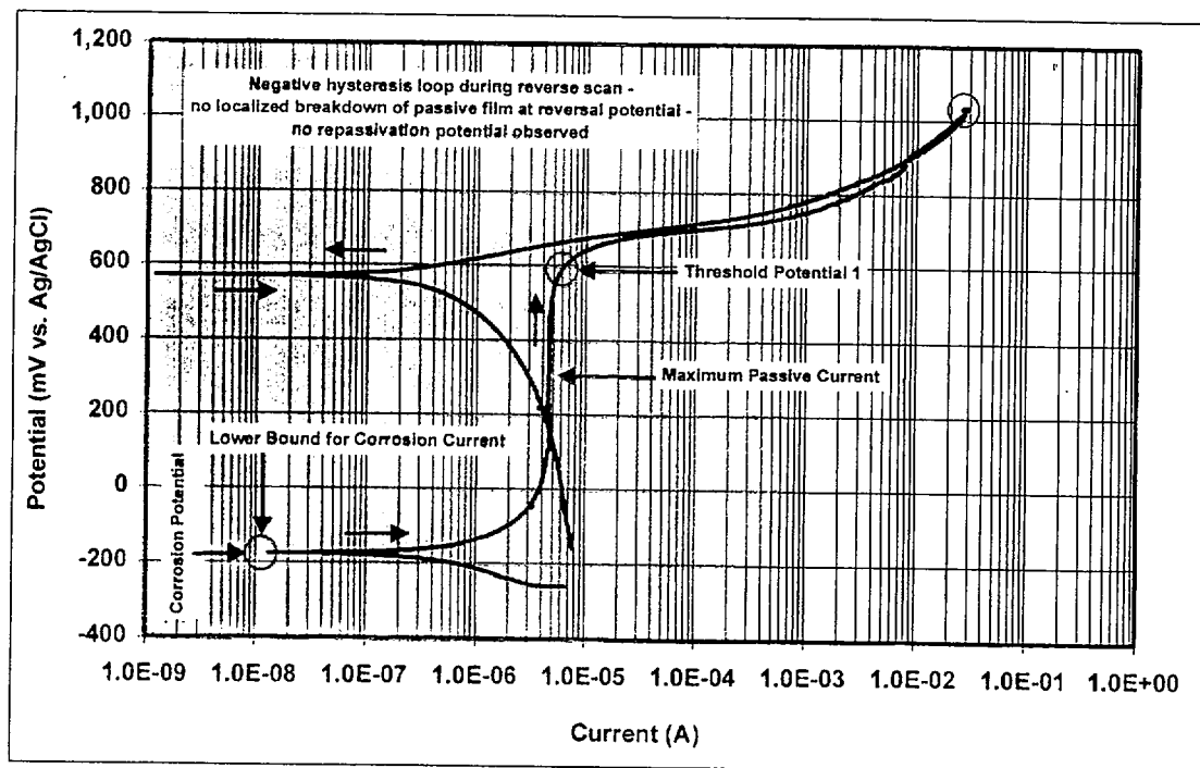
Figure 3. Type 1 – Alloy 22 in SSW at 120°C (DEA033)
