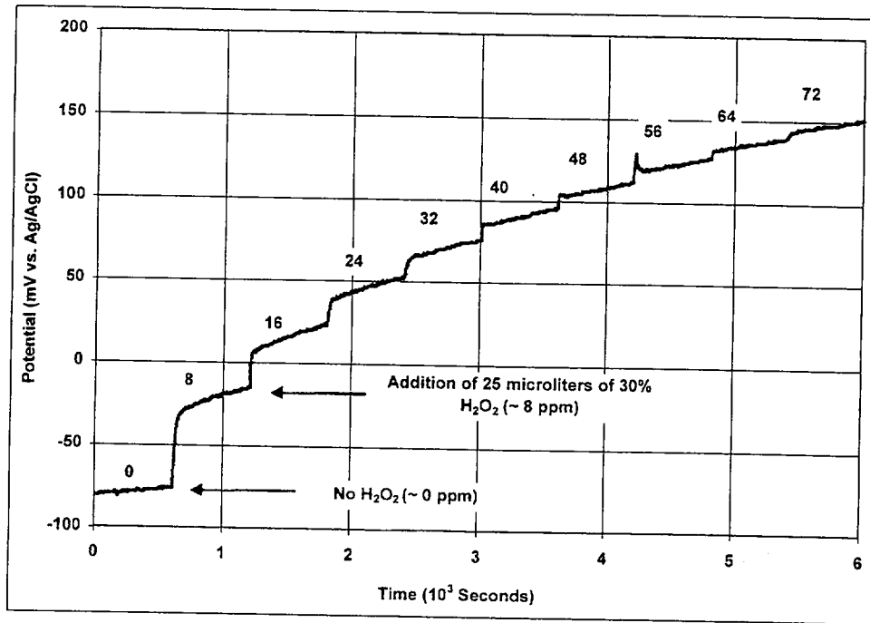
Figure 16. Effect of Hydrogen Peroxide on Corrosion Potential of Alloy 22 in SAW at 25°C
