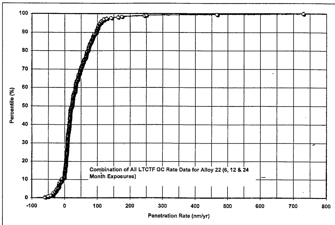
Figure 51. Combination of All GC Rate Data for Alloy 22 from LTCTF, including 6-, 12- and 24-Month (Two-Year) Exposures
