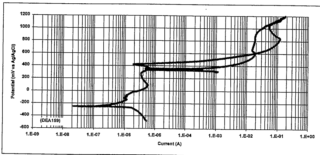
Figure 54. CP Curve for Thermally Alloy 22 in 110°C BSW – Aged at 700°C for 10 Hours (DEA159)
