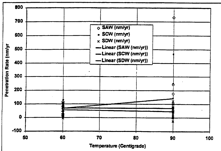
Figure 24. GC of Alloy 22, 6, and 12 Month Crevice Samples from LTCTF, Corrosion Rate Versus Temperature
