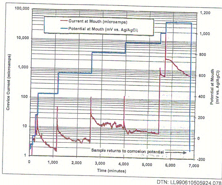
Figure 41. Alloy 22, 4M NaCl at 23 °C, Crevice Current Versus Time
