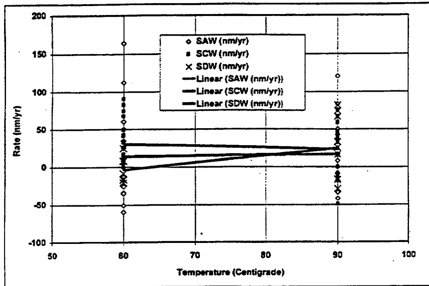
Figure 22. GC of Alloy 22, 6, and 12 Month Weight Loss Samples from LTCTF, Corrosion Rate Versus Temperature
