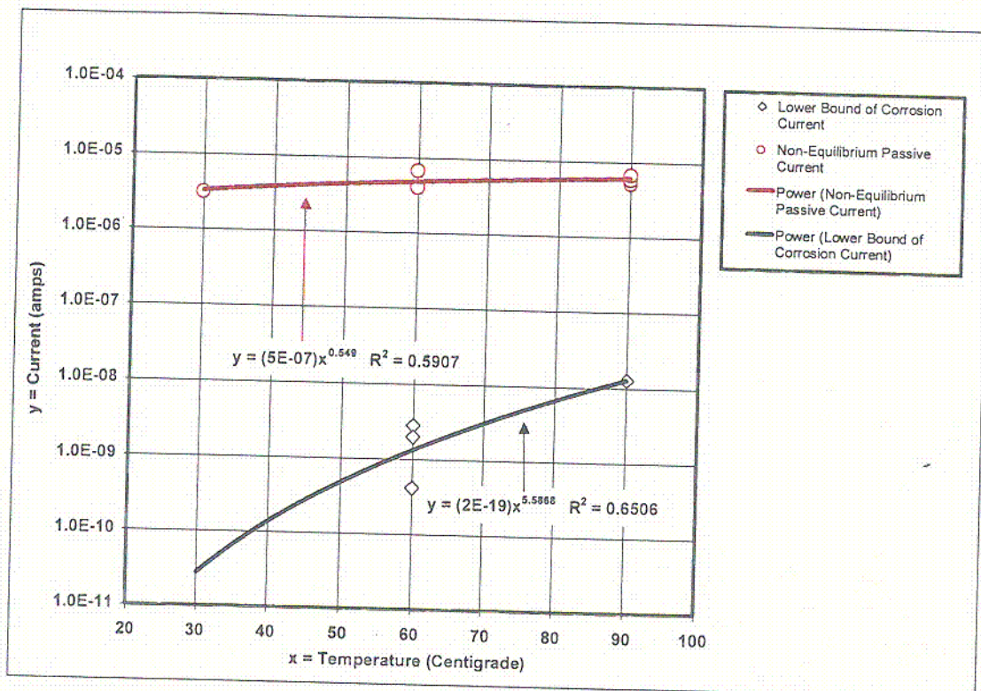
Figure 20. Bounding Currents Versus Temperature, Alloy 22 in SAW
