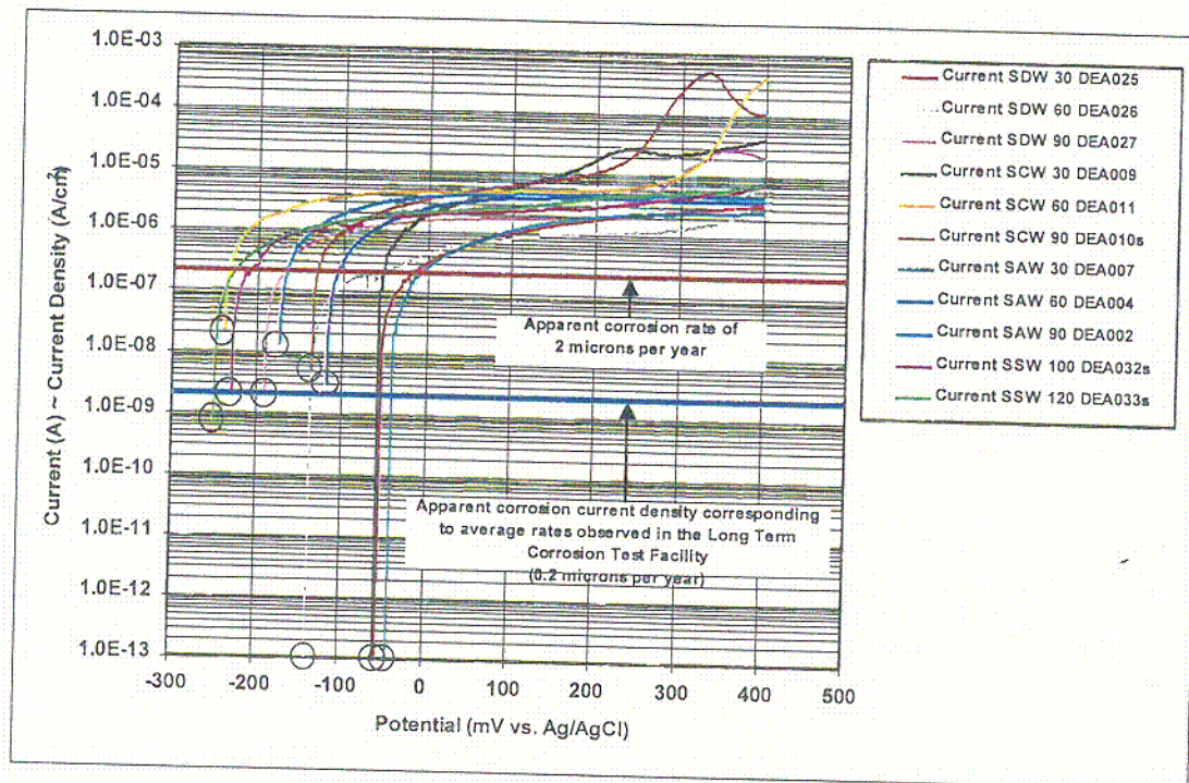
Figure 11. Alloy 22 in Various Repository Media – Comparison of CP Data
