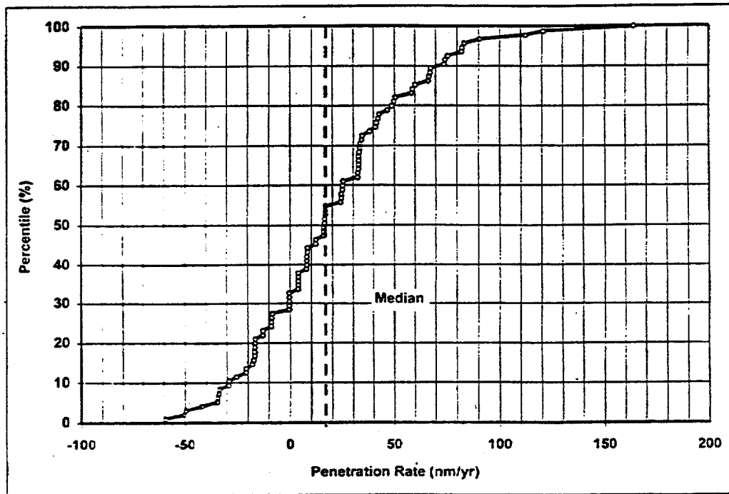
Figure 23. GC of Alloy 22, 6, and 12 Month Weight Loss Samples from LTCTF, Percentile Versus Corrosion Rate
