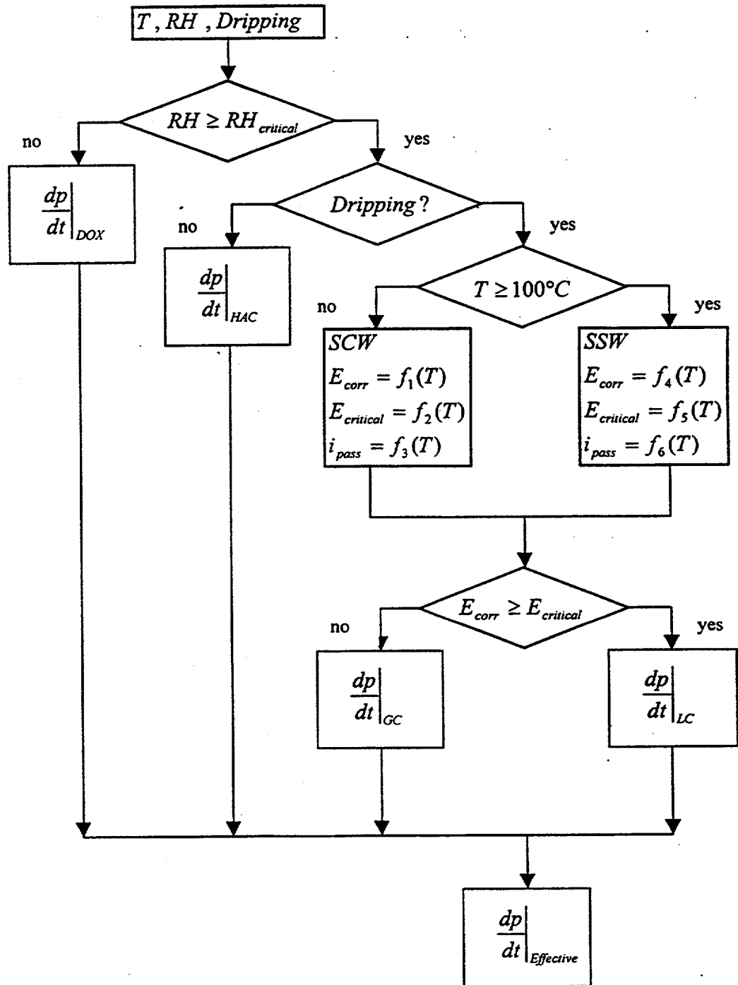
Figure 1. Schematic Representation of Corrosion Model for Alloy 22 Outer Barrier
