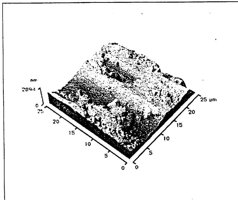
Figure 27. AFM Image of Alloy 22 Control Sample
