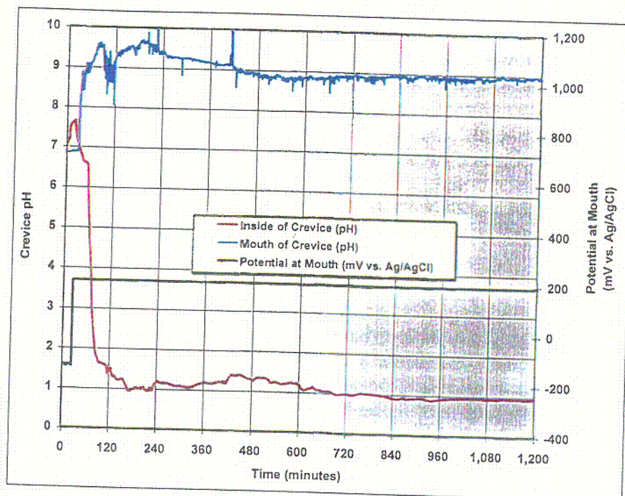
Figure 37. Stainless Steel 316L, 4M NaCl, 200 mV and 23 °C, Crevice pH Versus Time
