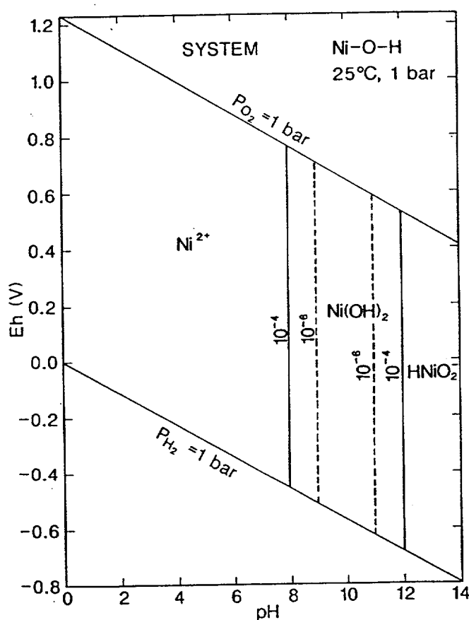
Figure 4. Eh-pH diagram for part of the system Ni-O-H. Assumed activity for Ni = 10^{-4} – 10^{-6} (Brookins 1988).
