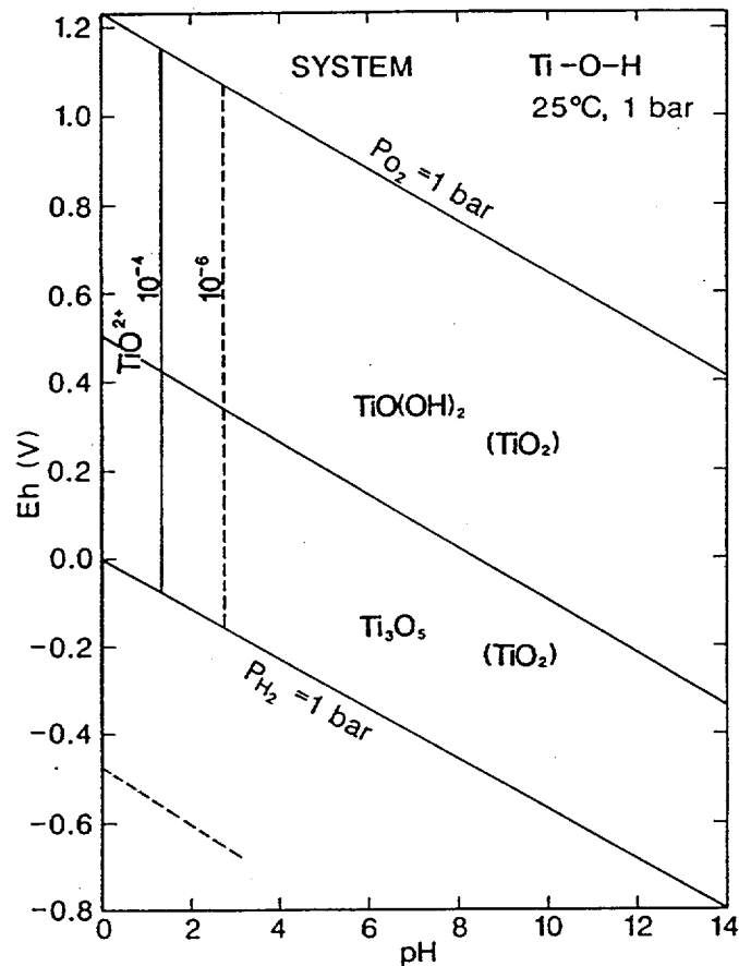
Figure 7. Eh-pH diagram for part of the system Ti-O-H. Assumed activity for Ti = 10^{-6} . Note \text{TiO}_2 occupies all Eh-pH space shown as \text{TiO(OH)}_2 and \text{Ti}_3\text{O}_5 (Brookins 1988).
