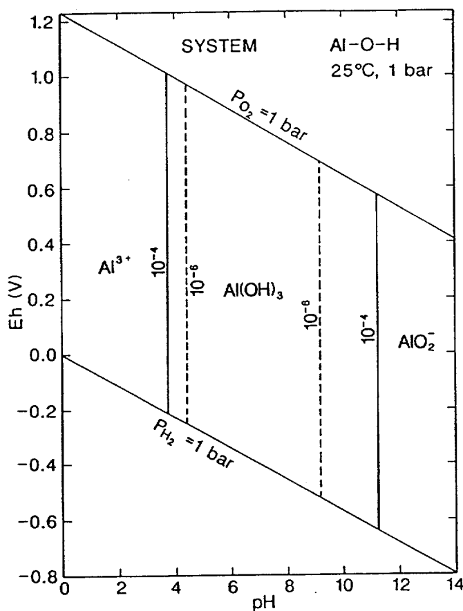
Figure 8. Eh-pH diagram for part of the system Al-O-H. Assumed activity for Al = 10^{-4.6} (Brookins 1988).
