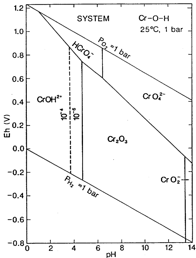
Figure 5. Eh-pH diagram for part of the system Cr-O-H. Assumed activity for Cr = 10^{-4} , 10^{-6} (Brookins 1988).
