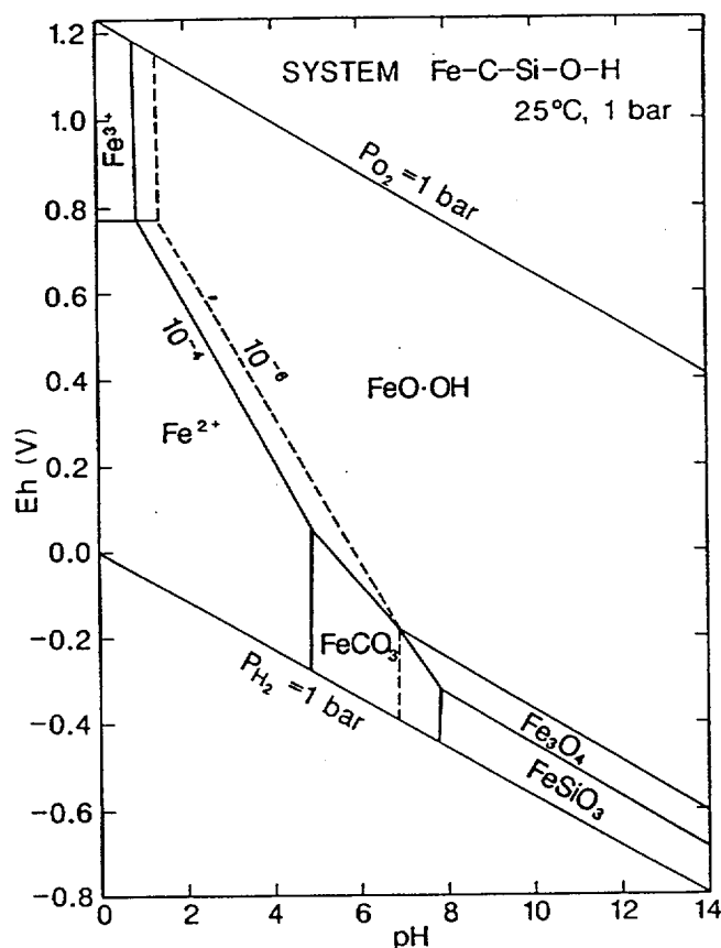
Figure 2. Eh-pH diagram for part of the system Fe-C-Si-O-H. Assumed activities for dissolved species are: Fe = 10^{-6} , Si = 10^{-3} , C = 10^{-3} . Goethite and magnetite assumed as Fe(III) solid phases (Brookins 1988).
