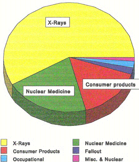
Figure 8: Man-Made Radiation Sources (BIER V)
