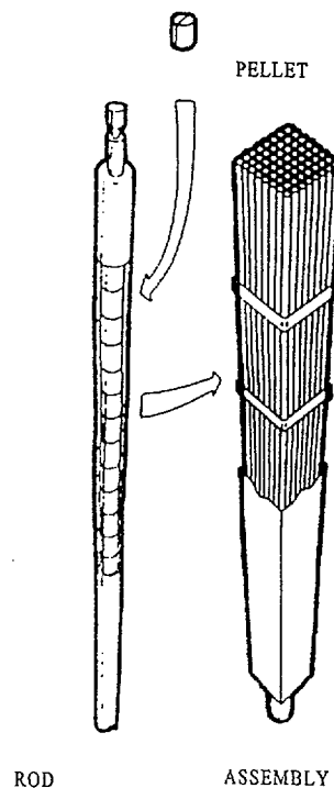
Figure 11: Fuel Pellets, Rods & Assemblies
