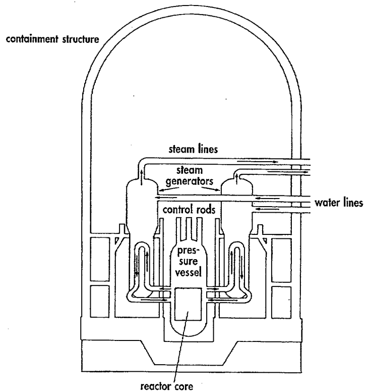
Figure 14: Primary Containment Structure
