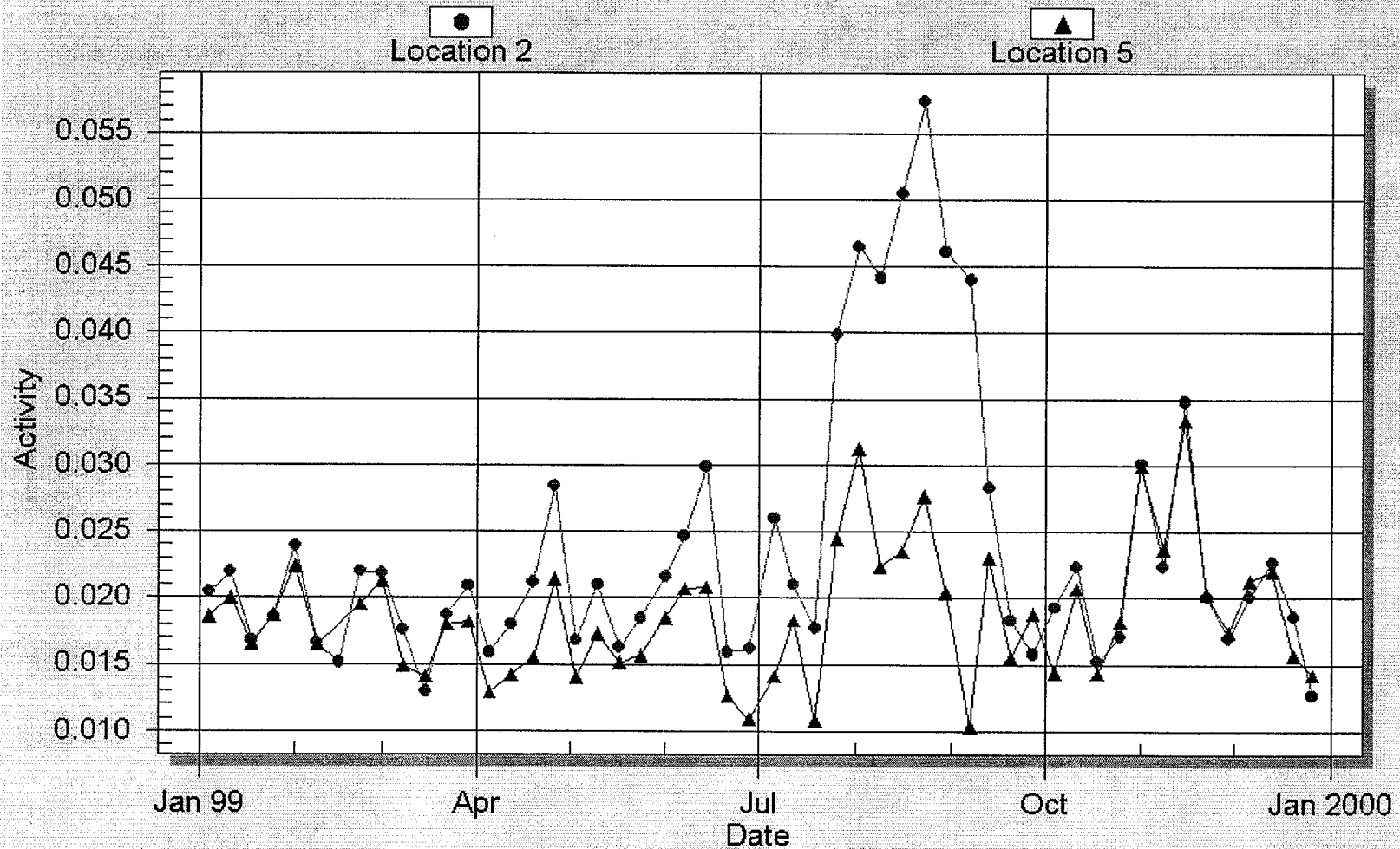
Figure 19 HNP From 1/1/99 To 12/31/99 AIR PARTICULATE GROSS BETA - Activity (pCi/cubic meter)
