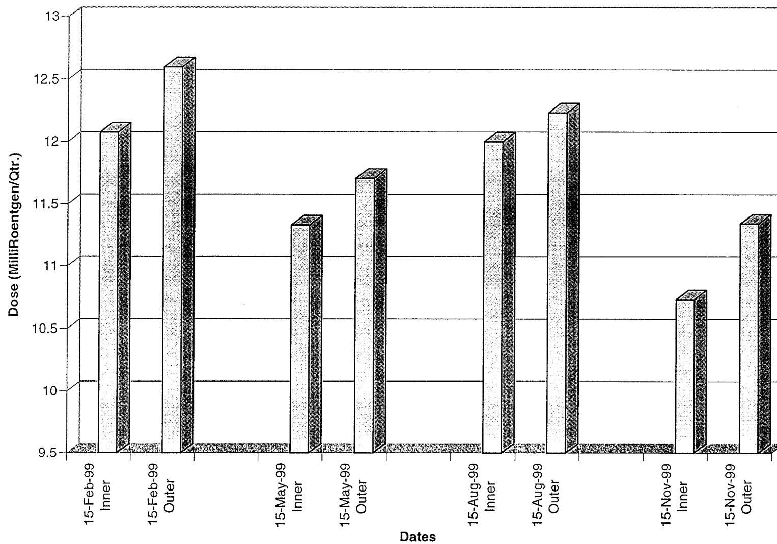
Figure 26 HNP 1999 TLD Averages for Inner and Outer Ring Locations
