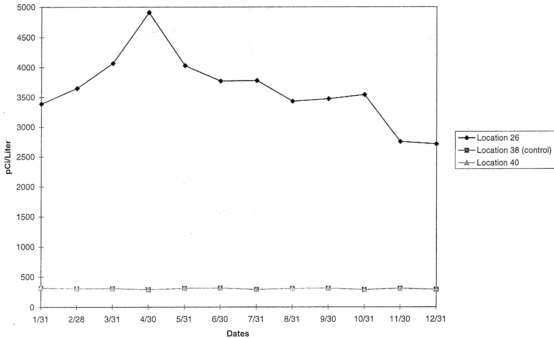
Figure 25 HNP 1999 Surface Water Tritium
