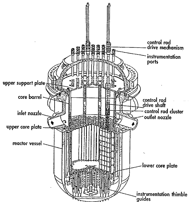
Figure 13: Reactor Vessel
