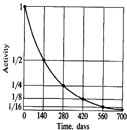
Figure 4: Radioactive Decay
