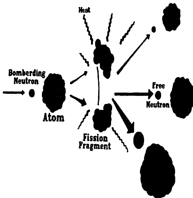
Figure 9: Nuclear Fission
