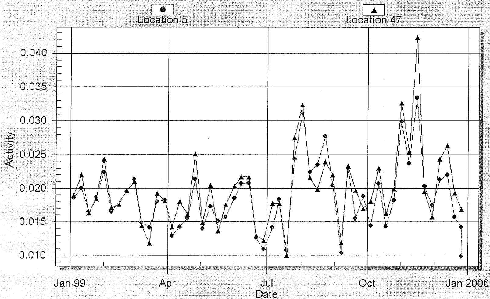
Figure 22 HNP From 1/1/99 To 12/31/99 AIR PARTICULATE for GROSS BETA - Activity (pCi/cubic meter)
