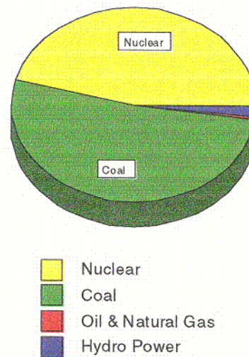
Figure 2: 1999 Energy Sources
