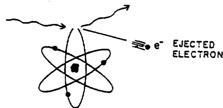
Figure 5: Ionization
