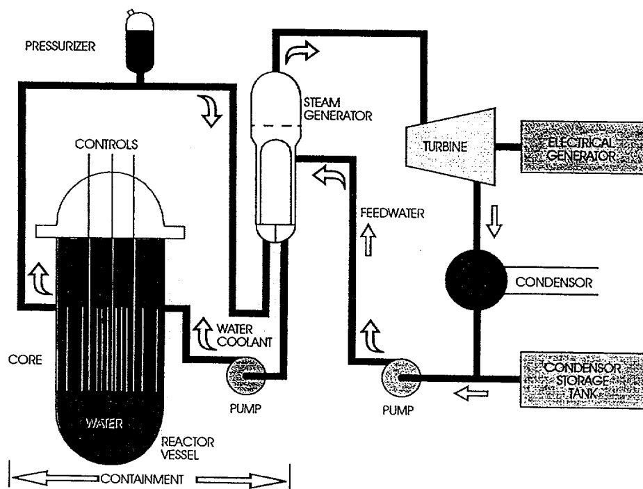
Figure 12: Major Plant Systems for The Pressurized Water Reactor
