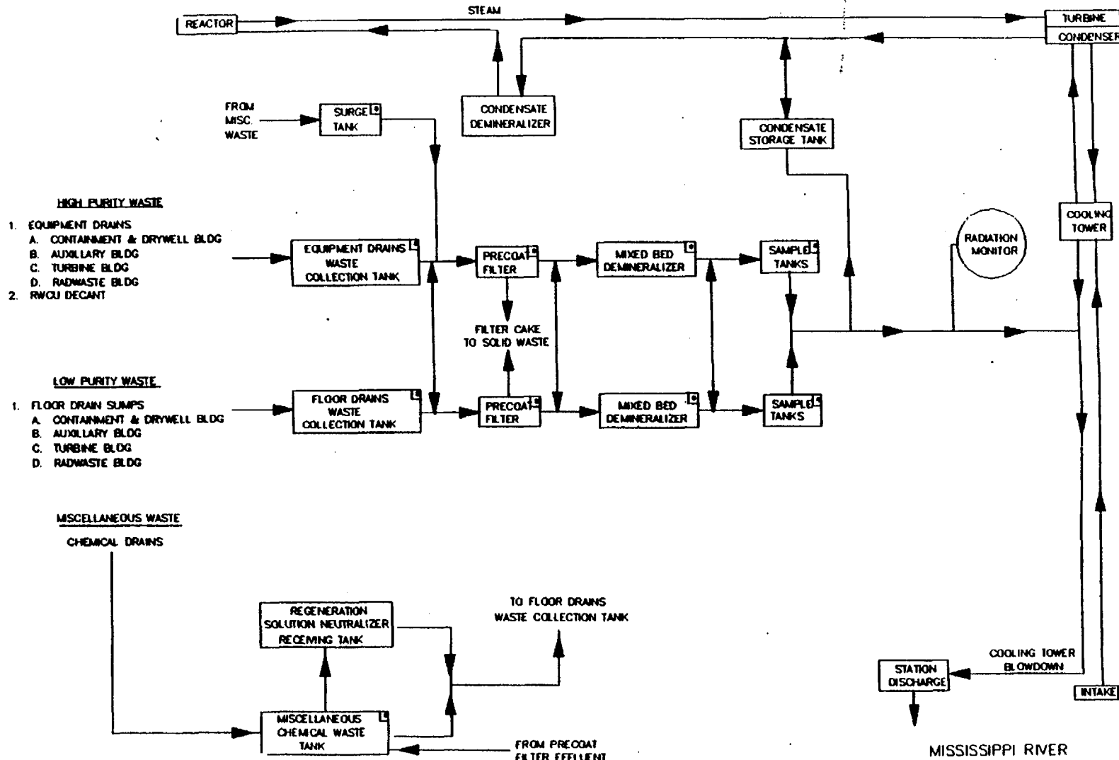
Figure 1.3-1 Liquid Radwaste Treatment System
