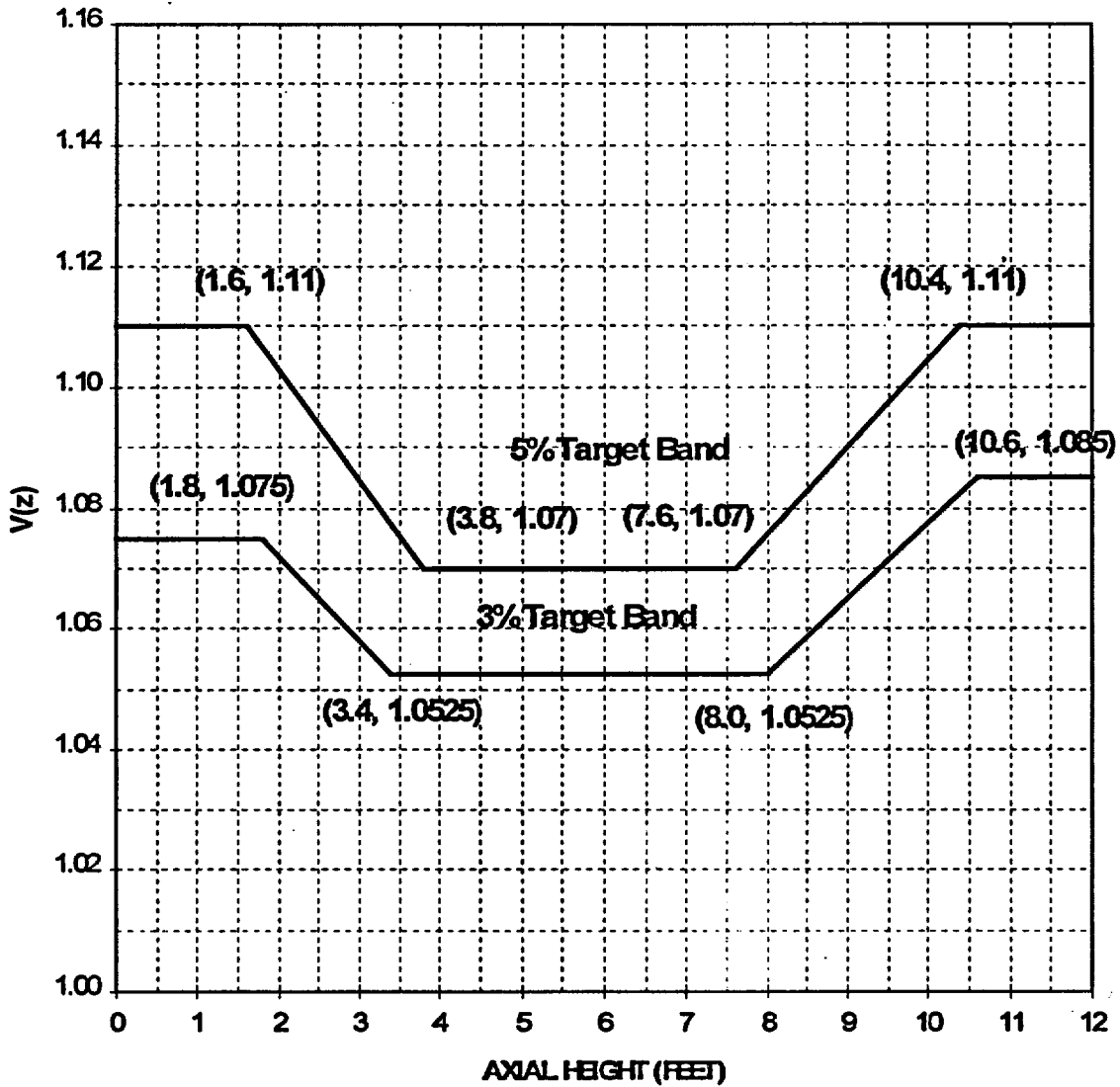
Figure 3.0, V(z) as a Function of Core Height
