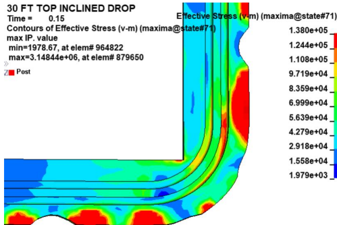
FIGURE 2.7.24 EFFECTIVE STRESS IN THE SEAL SEATING REGION ON TOP FLANGE – HAC TOP INCLINED DROP
