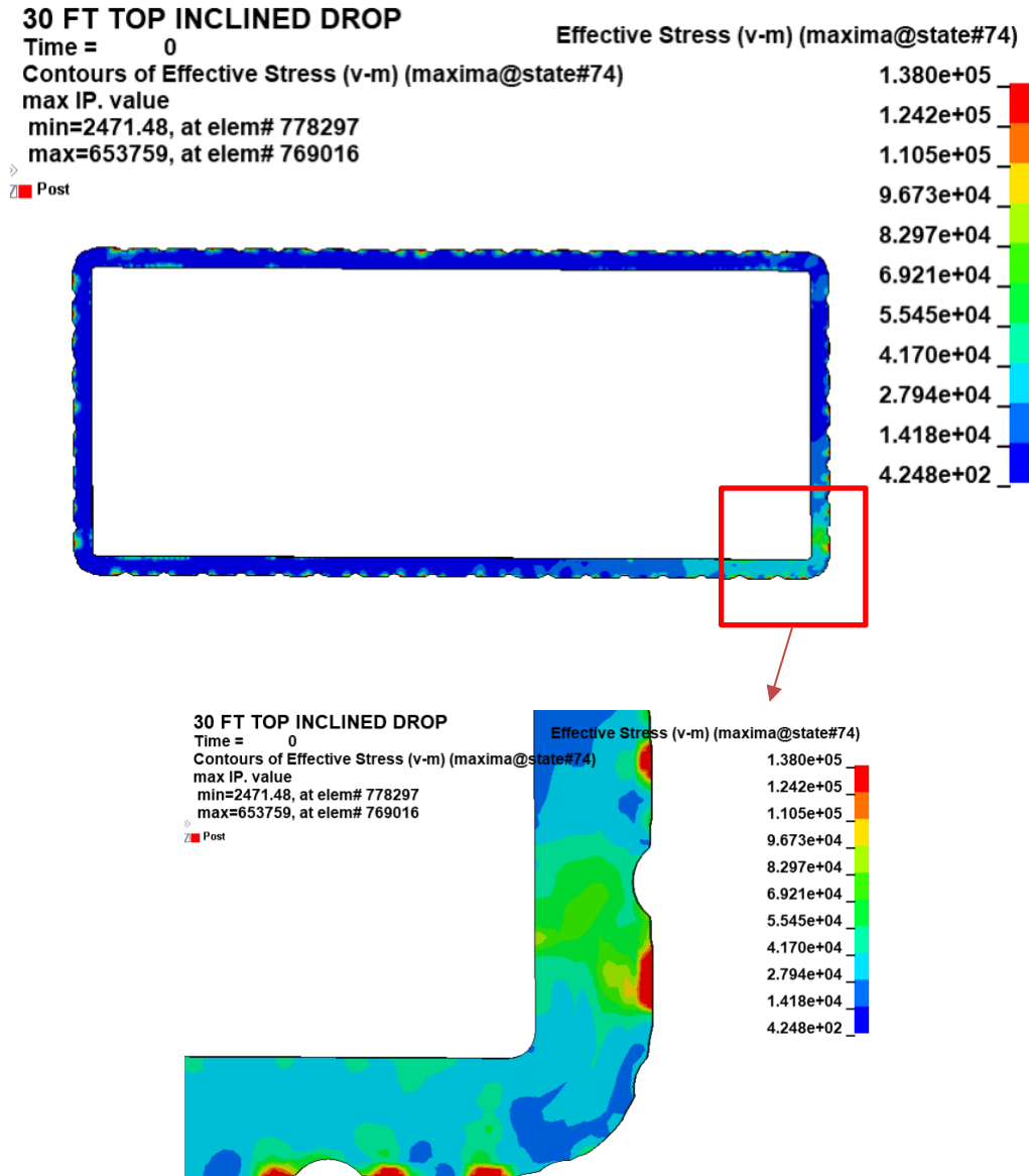
FIGURE 2.7.25 EFFECTIVE STRESS IN THE SEAL SEATING REGION ON CLOSURE LID – HAC TOP INCLINED DROP
