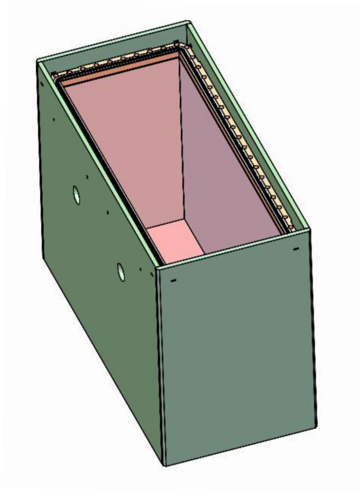
FIGURE 2.3.2: CONTAINMENT BOUNDARY AND DOSE BLOCKER BASE PLATES WELDED IN PLACE; CONTAINMENT FLANGE WITH WELD OVERLAY INSTALLED AND MACHINED
