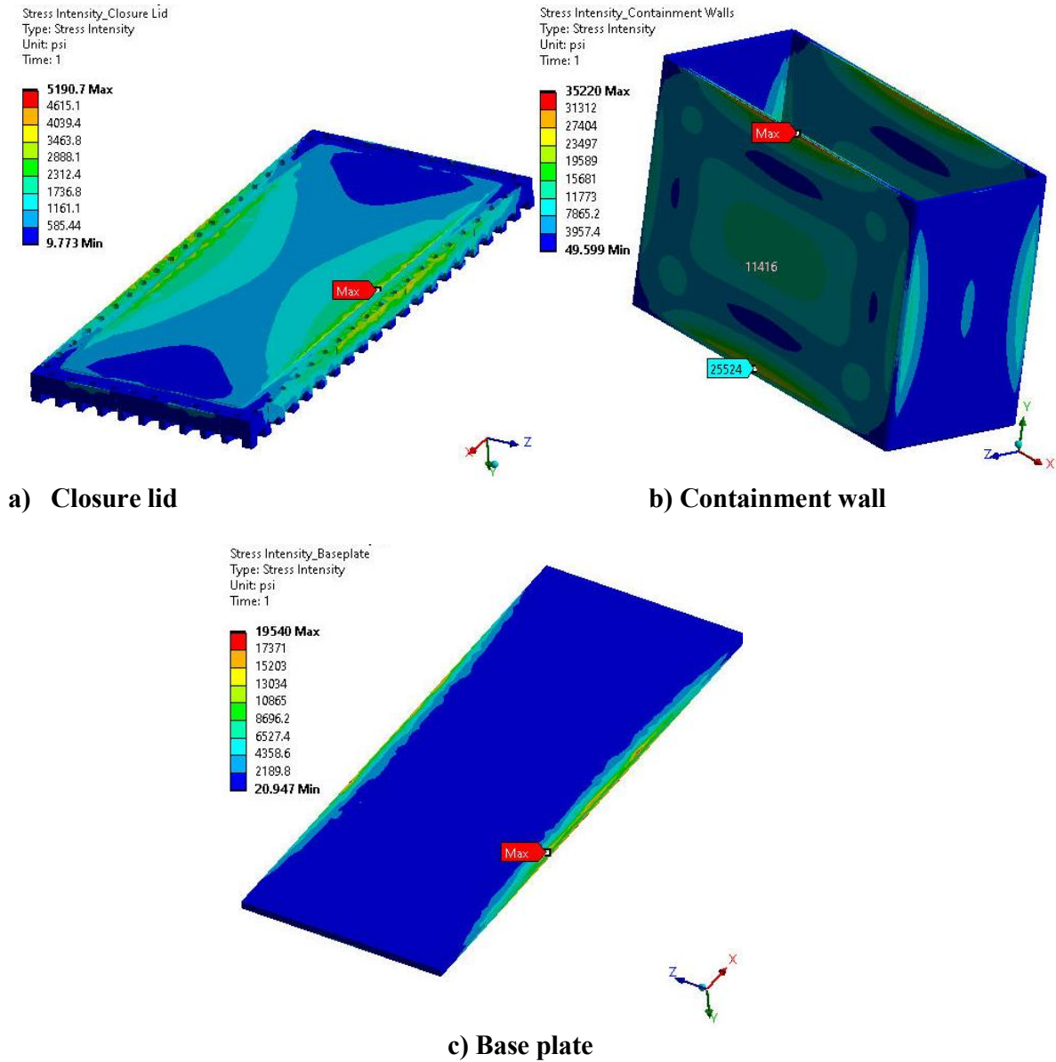
FIGURE 2.6.8 STRESS INTENSITY IN THE CONTAINMENT SHELL, BASEPLATE AND THE CLOSURE LID – EXTERNAL PRESSURE LOADING
