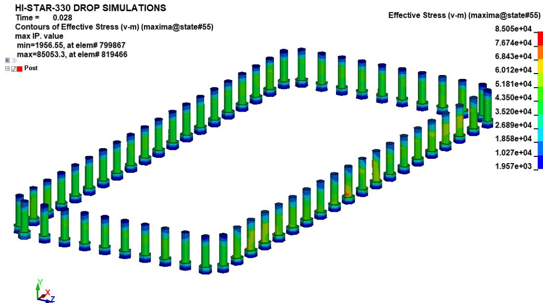
FIGURE 2.7.7 EFFECTIVE STRESS IN THE CLOSURE LID BOLTS SUBSEQUENT TO THE PUNCTURE DROP EVENT – TOP END DROP (OVER SEALING REGION)
