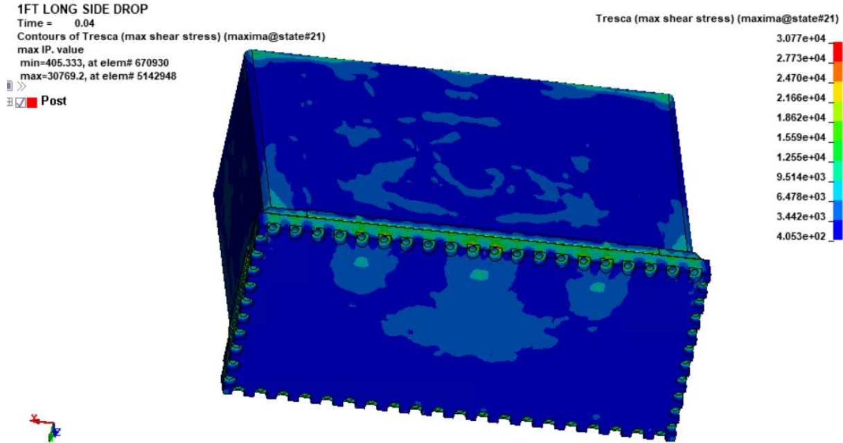
FIGURE 2.6.11: MAXIMUM SHEAR STRESS IN THE CONTAINMENT WALLS, BASEPLATE, TOP FLANGE AND CLOSURE LID– NCT SIDE DROP (LONG SIDE) EVENT
