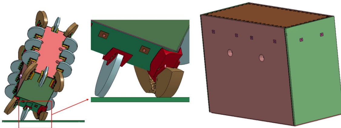
FIGURE 2.7.6 PHYSICAL STATE OF THE CASK SUBSEQUENT TO THE DROP EVENT – TOP CGOC DROP
