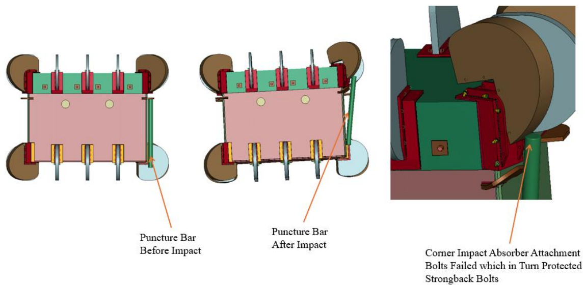
FIGURE 2.7.13 PHYSICAL STATE OF THE CASK AT THE END OF BOTTOM END DROP FOLLOWED BY PUNCTURE ONTO THE CORNER IMPACT ABSORBER ATTACHMENT
