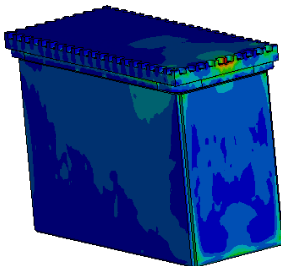
FIGURE 2.7.20 MAXIMUM SHEAR STRESS IN THE CONTAINMENT BOUNDARY – ADDITIONAL HAC SHORT SIDE DROP
