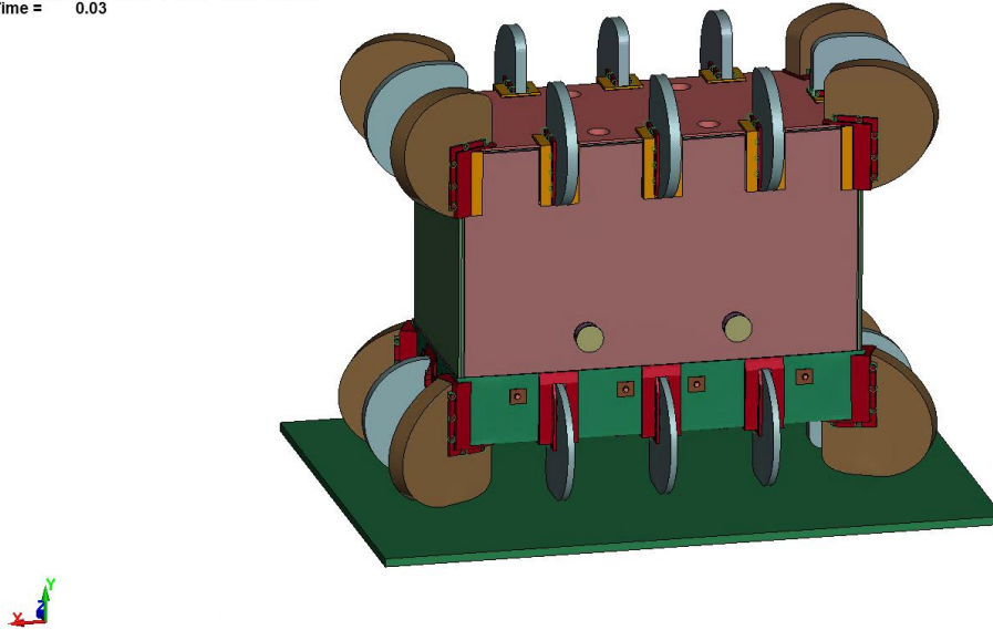
FIGURE 2.7.5 PHYSICAL STATE OF THE CASK SUBSEQUENT TO THE DROP EVENT – TOP END DROP
