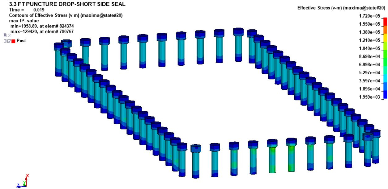
FIGURE 2.7.9 EFFECTIVE STRESS IN THE CLOSURE ID BOLTS - 1M SHORT SIDE DROP PUNCTURE EVENT
