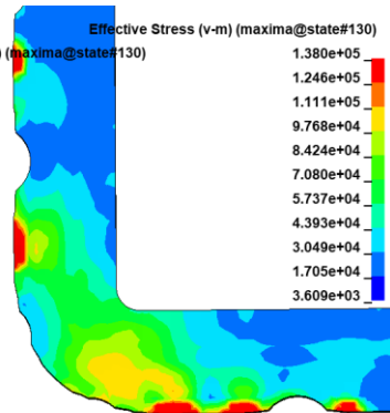
FIGURE 2.7.23 EFFECTIVE STRESS IN THE SEAL SEATING REGION ON CLOSURE LID – HAC TOP CGOC DROP
