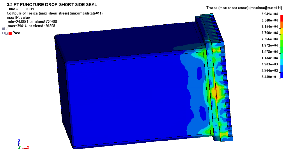
FIGURE 2.7.8 MAXIMUM SHEAR STRESS IN THE CONTAINMENT WALLS, BASEPLATE AND CLOSURE LID - 1M SHORT SIDE DROP PUNCTURE EVENT
