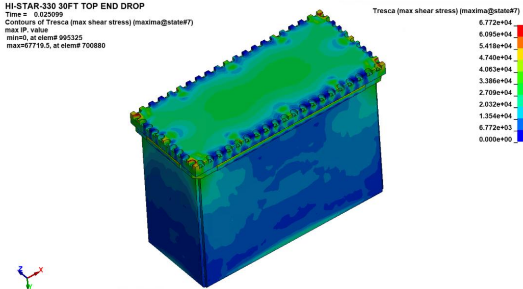
FIGURE 2.7.1 MAXIMUM SHEAR STRESS IN THE CONTAINMENT WALLS, BASEPLATE AND CLOSURE LID – HAC TOP END DROP
