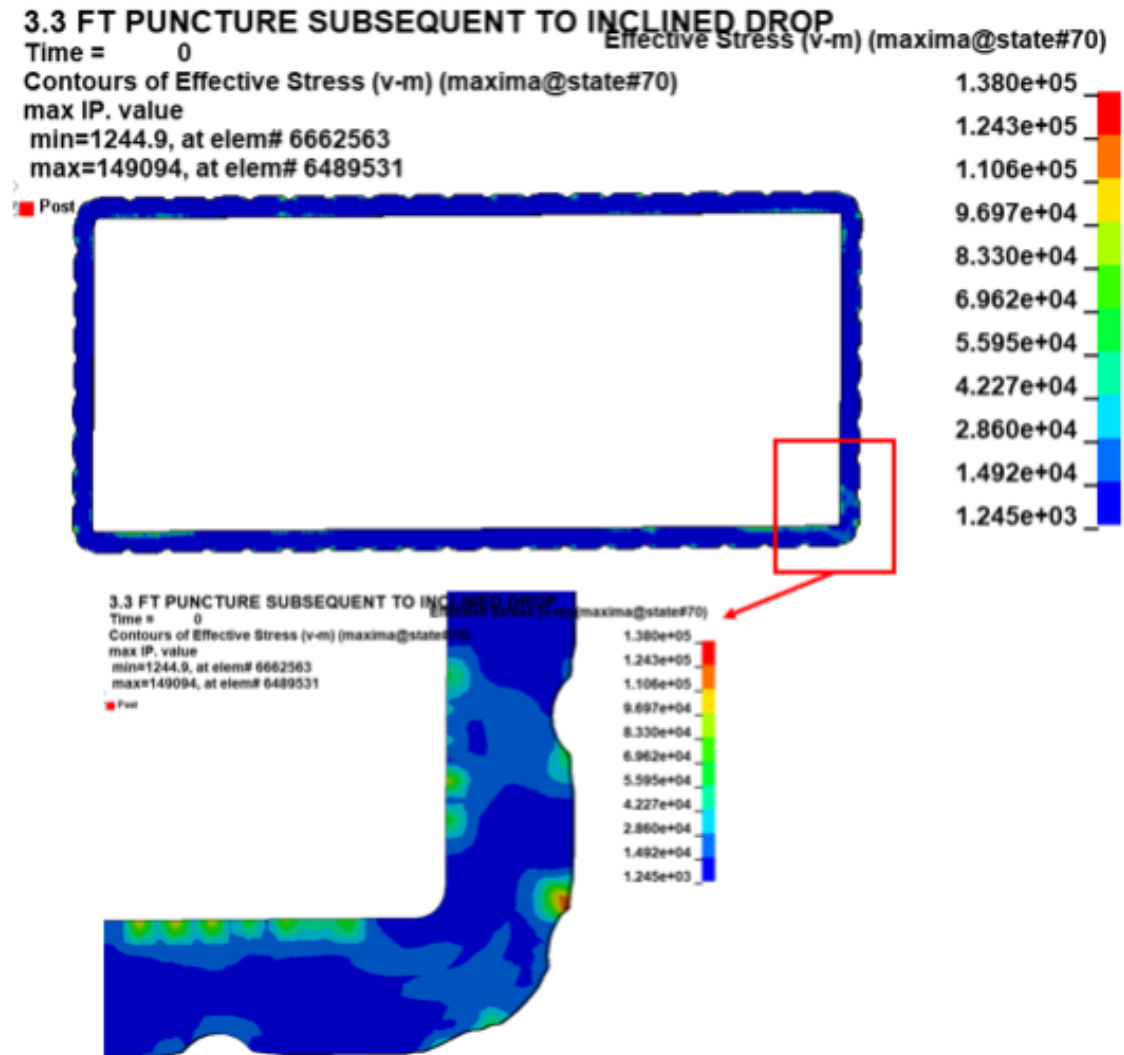
FIGURE 2.7.27 EFFECTIVE STRESS IN THE SEAL SEATING REGION ON CLOSURE LID – HAC INCLINED DROP (TOP END) FOLLOWED BY 1-M PUNCTURE DROP
