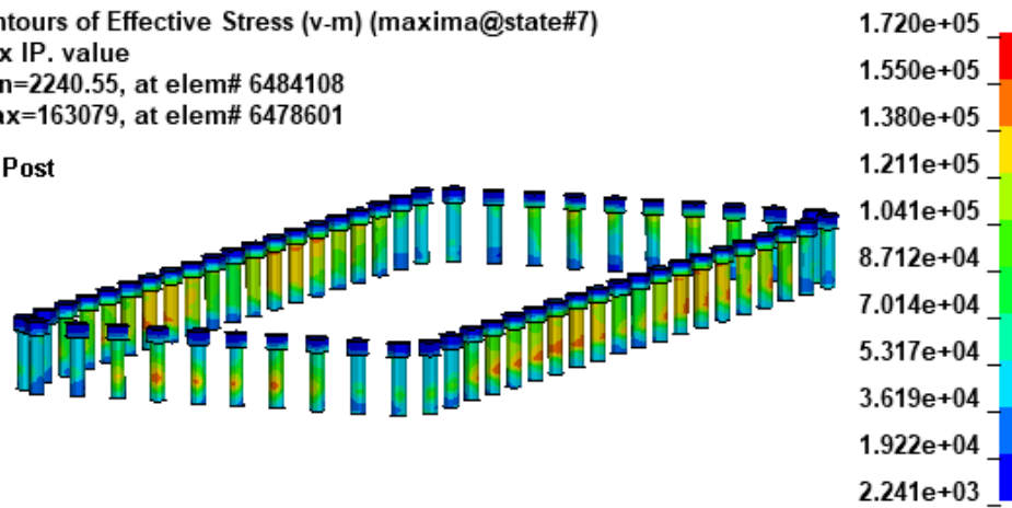
FIGURE 2.7.18 EFFECTIVE STRESS IN THE CLOSURE LID BOLTS – ADDITIONAL HAC TOP END DROP
