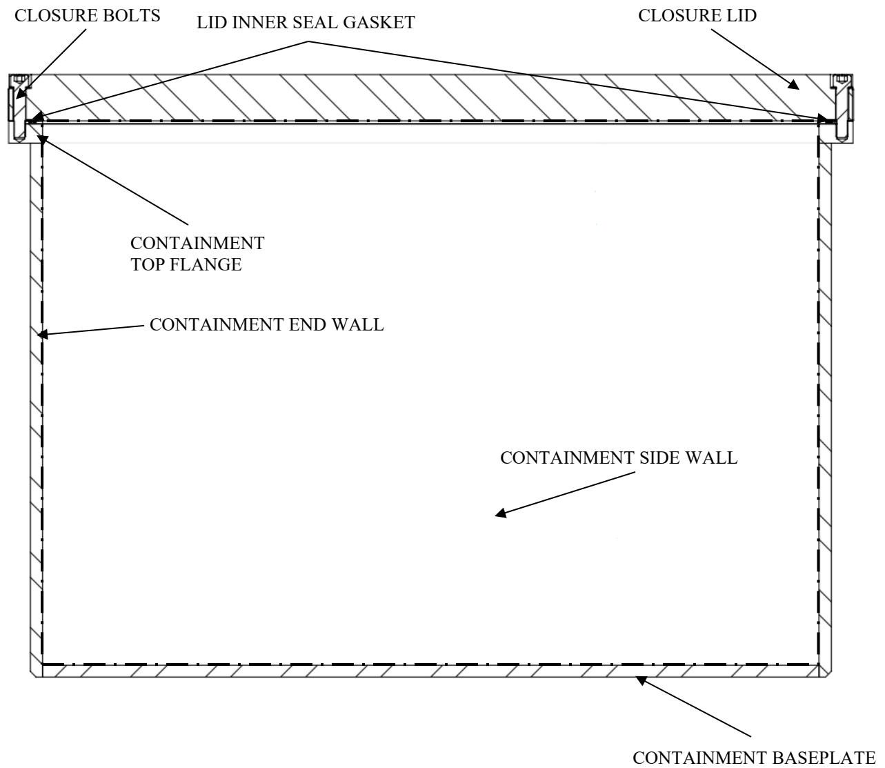
Figure 4.1.1: Containment System Boundary Components
