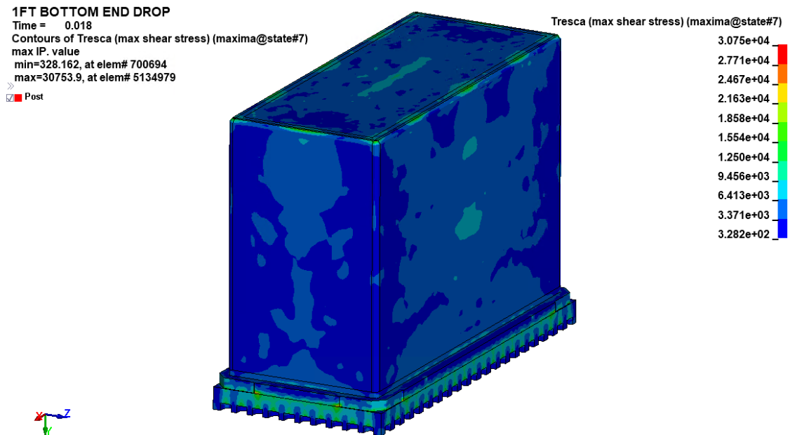
FIGURE 2.6.10 MAXIMUM SHEAR STRESS IN THE CONTAINMENT WALLS, BASEPLATE, TOP FLANGE AND CLOSURE LID– NCT BOTTOM END DROP EVENT
