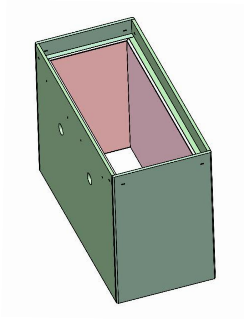
FIGURE 2.3.1: CONTAINMENT BOUNDARY SIDE WALL PLATES WELDED IN PLACE WITHIN DOSE BLOCKER WALL PLATES
