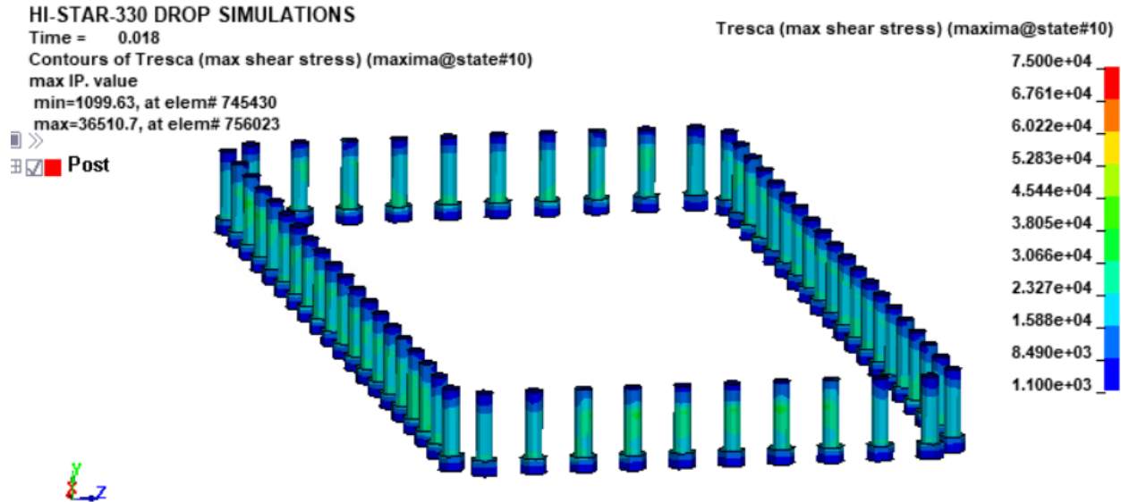
FIGURE 2.6.9: MAXIMUM SHEAR STRESS IN THE CLOSURE LID BOLTS – NCT TOP END DROP EVENT
