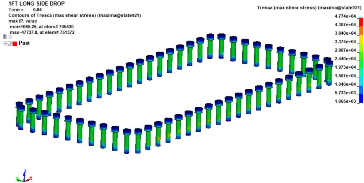
FIGURE 2.6.12 MAXIMUM SHEAR STRESS IN THE CLOSURE LID BOLTS – NCT SIDE DROP (LONG SIDE) EVENT
