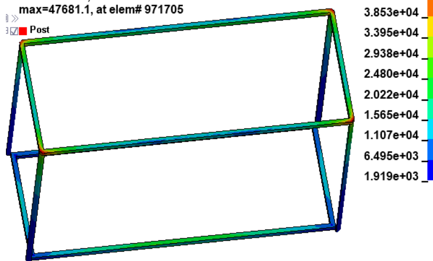
FIGURE 2.7.19 MAXIMUM SHEAR STRESS IN THE CONTAINMENT WELDS – ADDITIONAL HAC TOP END DROP
