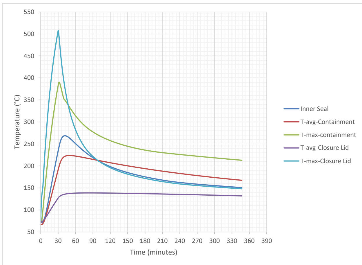
FIGURE 3.4.1 HI-STAR 330 FIRE AND POST FIRE COOLDOWN TEMPERATURE HISTORY
