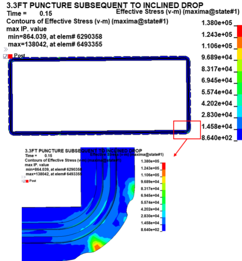
FIGURE 2.7.26 EFFECTIVE STRESS IN THE SEAL SEATING REGION ON TOP FLANGE – HAC INCLINED DROP (TOP END) FOLLOWED BY 1-M PUNCTURE DROP
