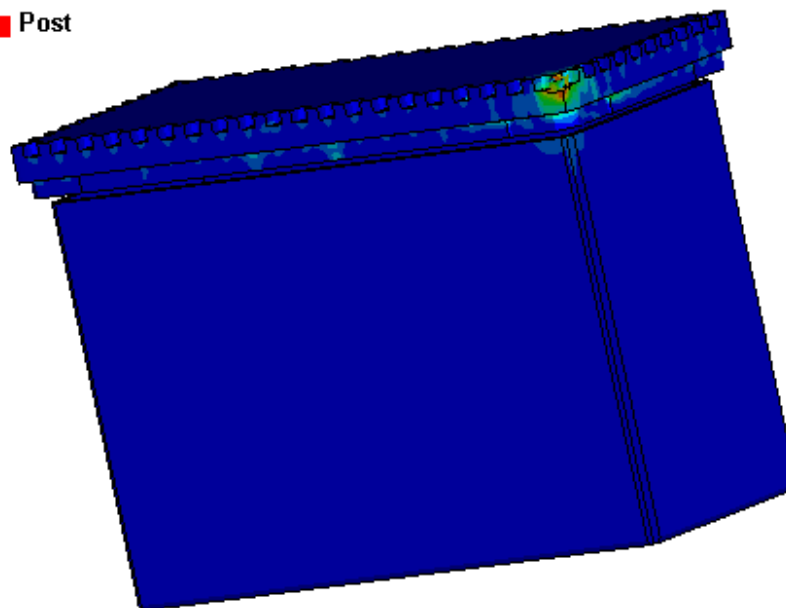
FIGURE 2.7.16 MAXIMUM SHEAR STRESS IN THE CONTAINMENT AT THE END OF INCLINED DROP (TOP END) FOLLOWED BY 1-M PUNCTURE DROP
