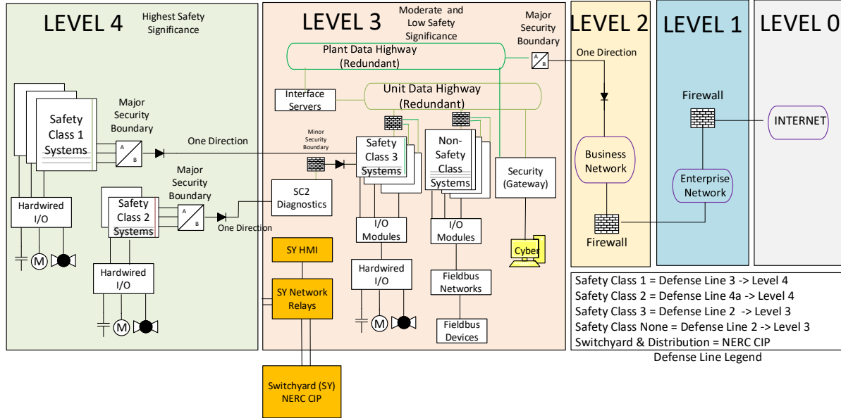
Figure 7.4-5: Cyber Security Architecture Security Boundaries
