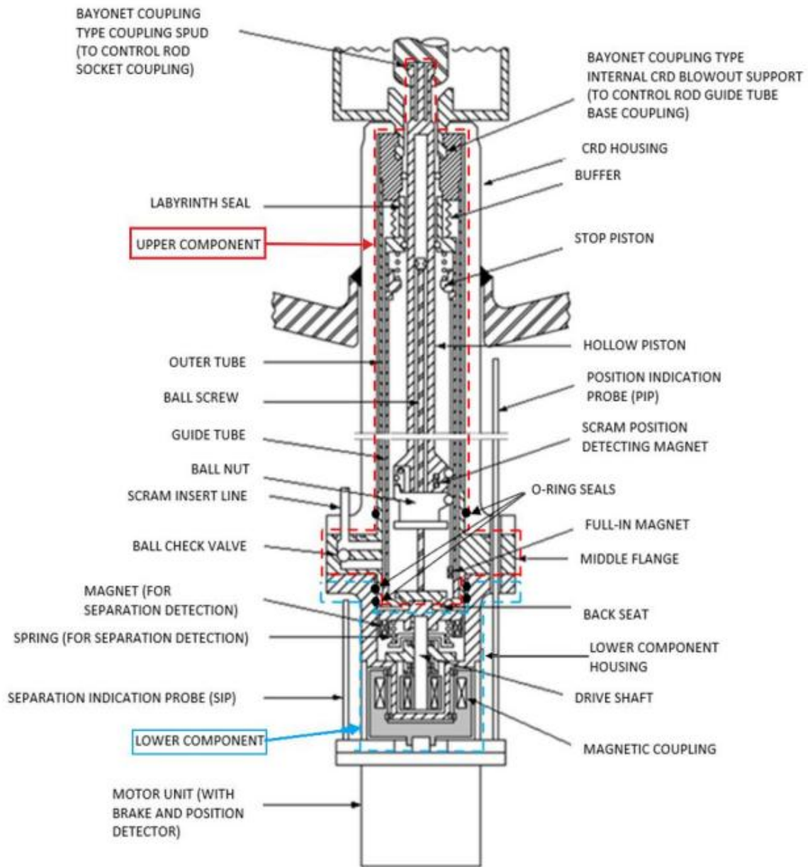
Figure 4.6-2: Schematic Representation of Magnet Coupling Fine Motion Control Rod Drive
