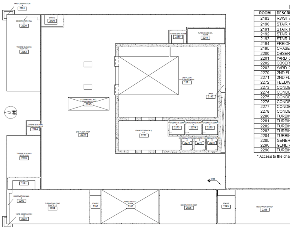
Figure 12.3-12: Turbine Building Level 6.1 Meters Radiation Zones
