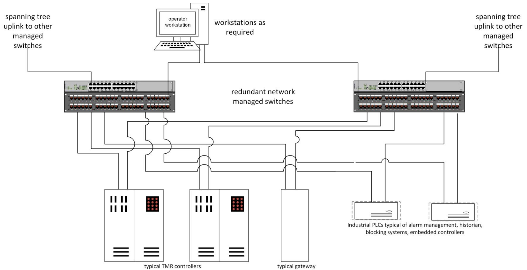
Figure 7.2-2: Typical Instrumentation and Control Controller and Component Network Connections
