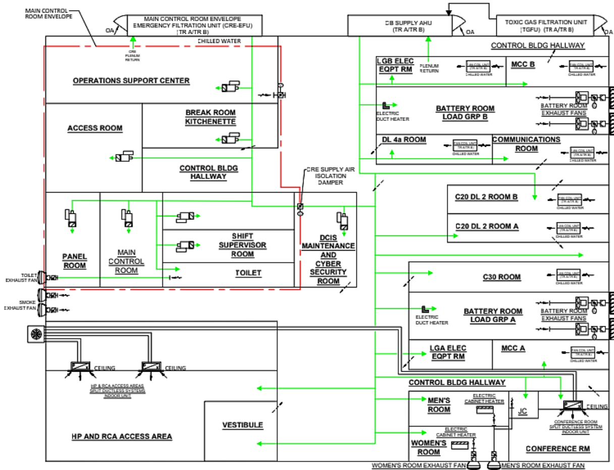
Figure 9.4-1: Control Building Heating, Ventilation, and Cooling Simplified Diagram
