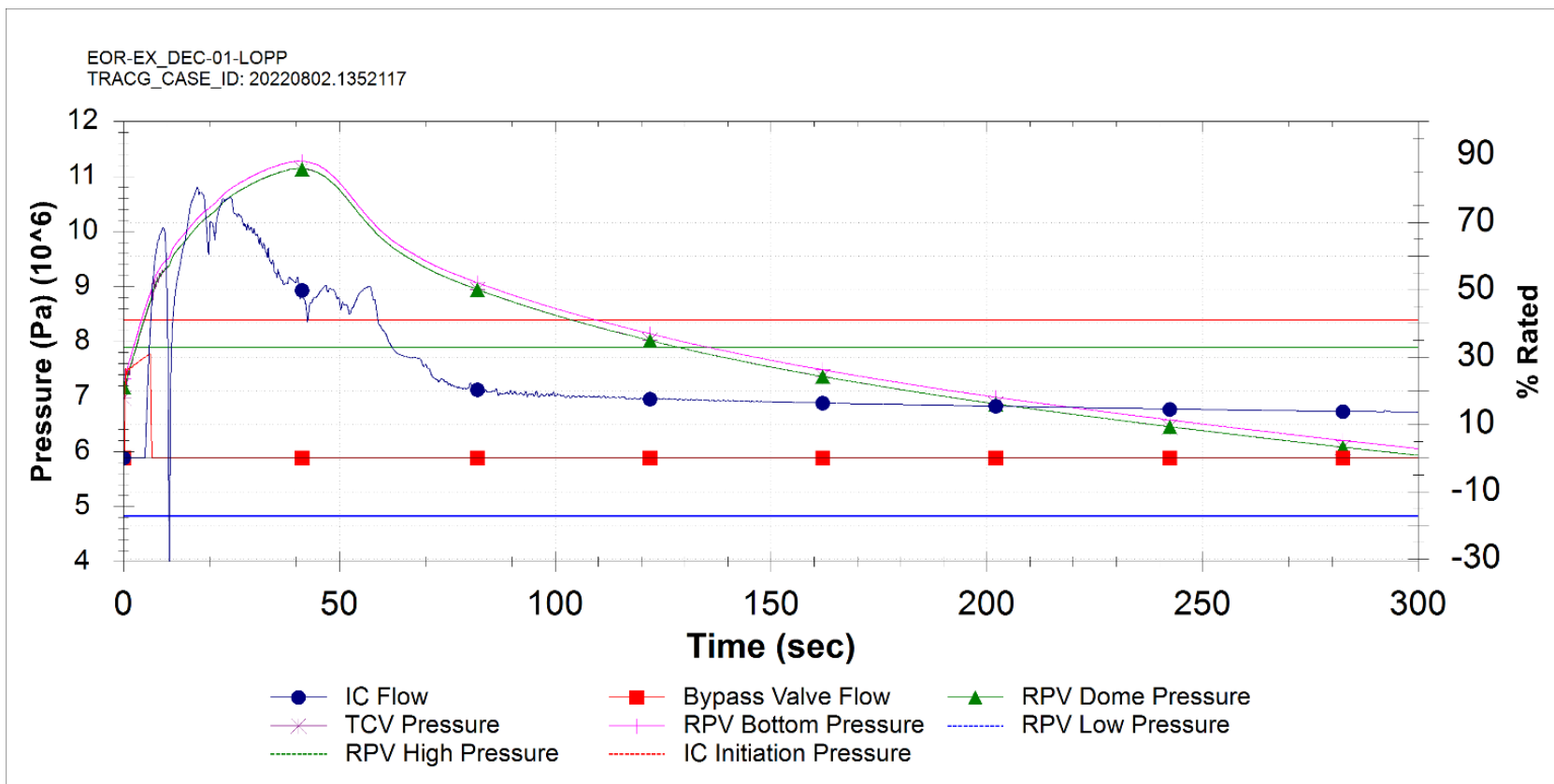
Figure 15.5-138: Loss of Preferred Power (DEC)
