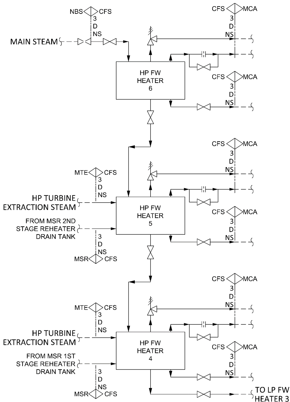
Figure 10.4-9: CFS HP Heaters and Drains Simplified Diagram
