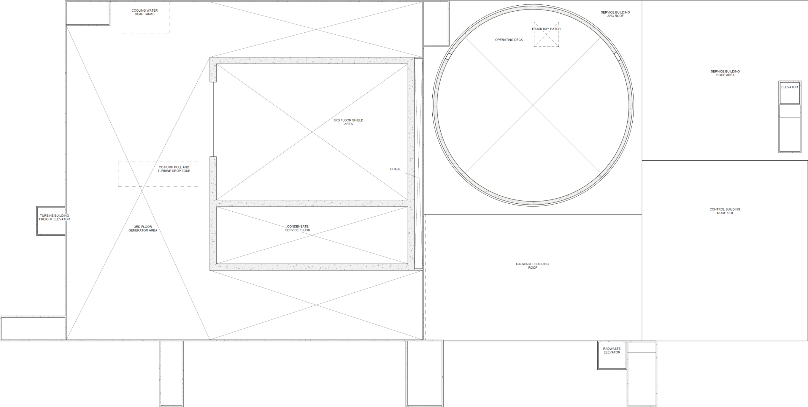
Figure 1.2-6: BWRX-300 Plan View Elevation 18.0m (Roof)
