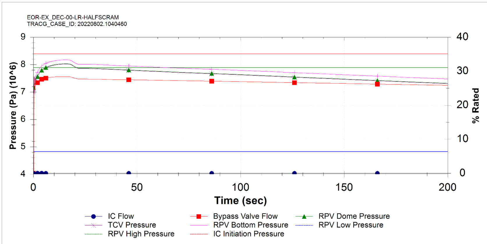
Figure 15.5-126: Complex Sequence Generator Load Rejection (DEC)
