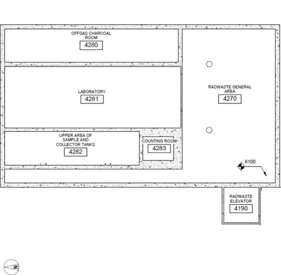
Figure 12.3-15: Radwaste Building Level 6.1 Meters Radiation Zones
