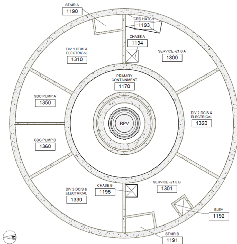
Figure 12.3-3: Reactor Building Level -21.0 Meters Radiation Zones
