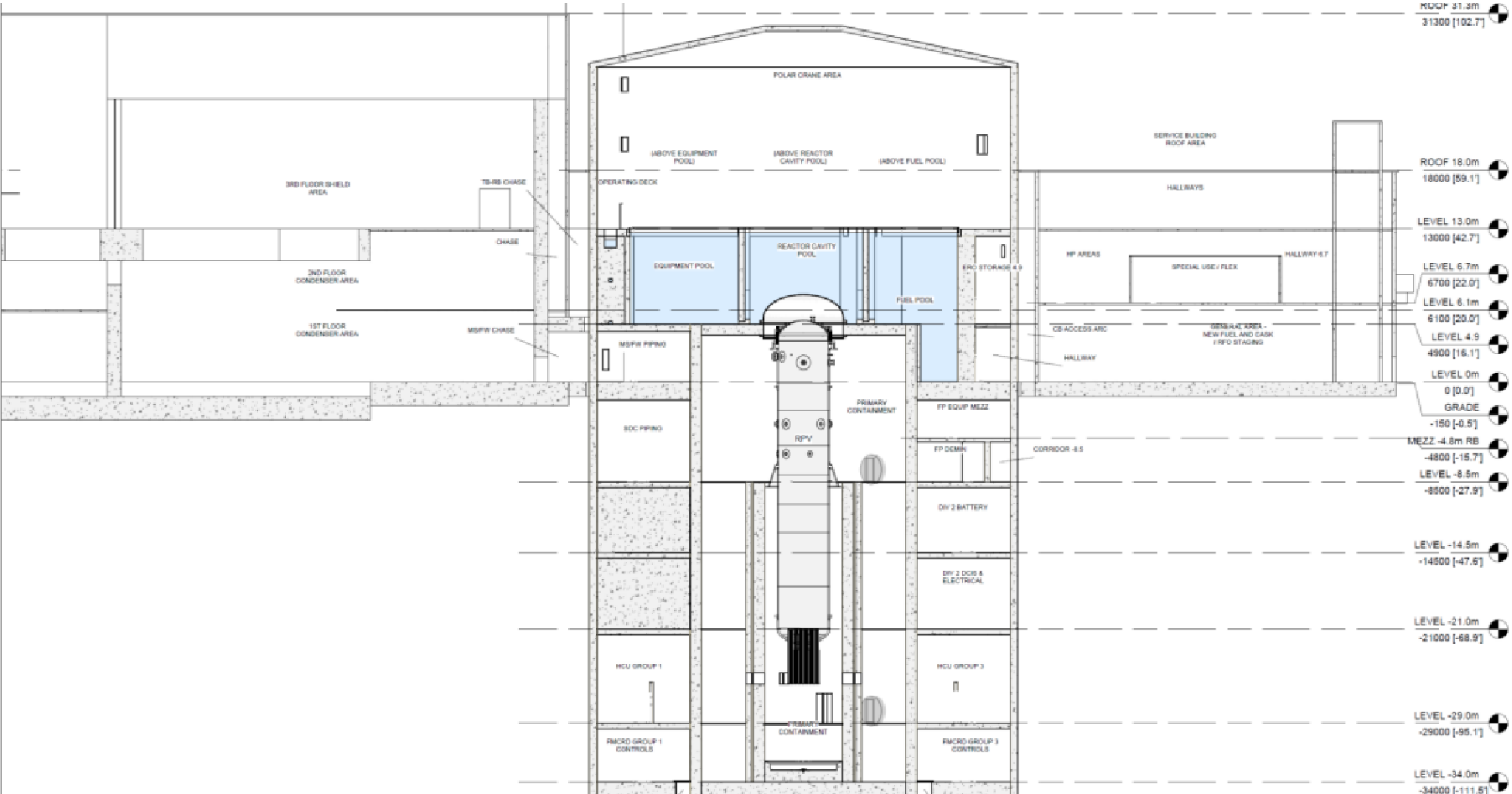
Figure 1.2-2: BWRX-300 Elevation View
