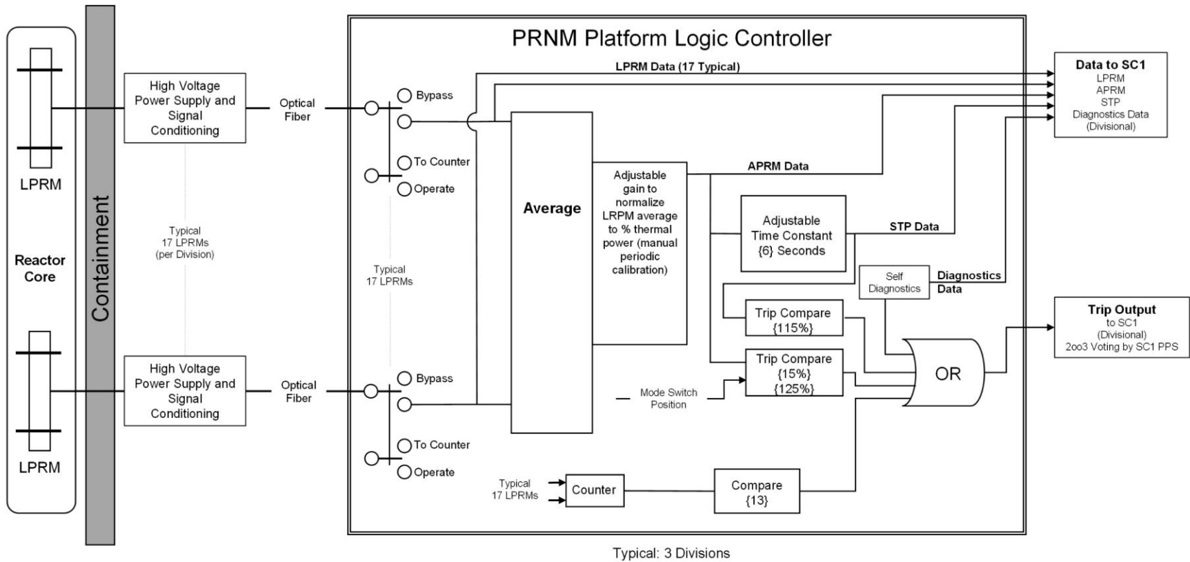
Figure 7.3-7: Representative Safety Class 1 Power Range Neutron Monitoring Block Diagram
