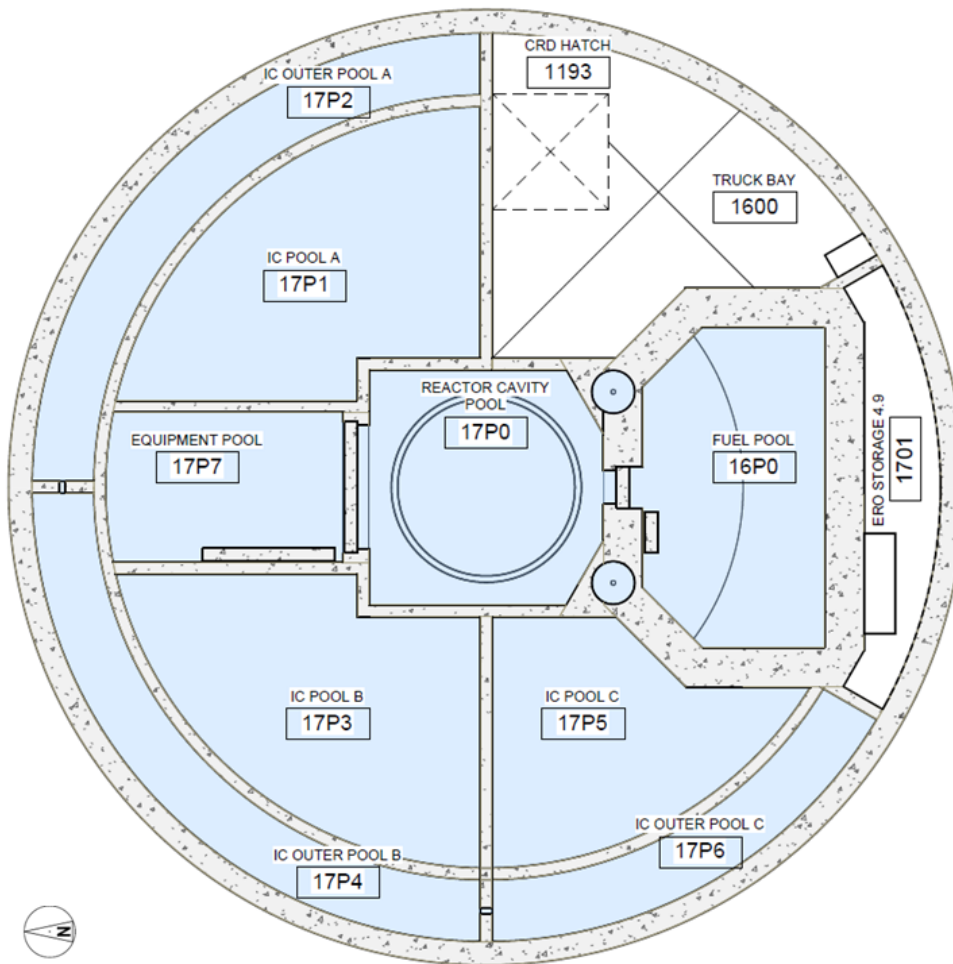
Figure 12.3-8: Reactor Building Level 4.9 Meters Radiation Zones
