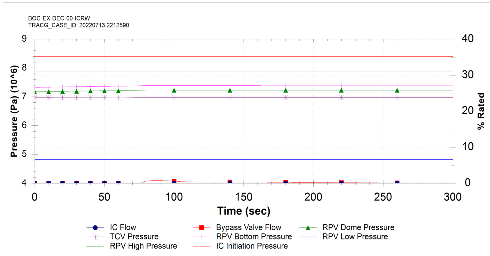
Figure 15.5-150: Inadvertent Control Rod Withdrawal at Power - Single Rod (ICRW)
