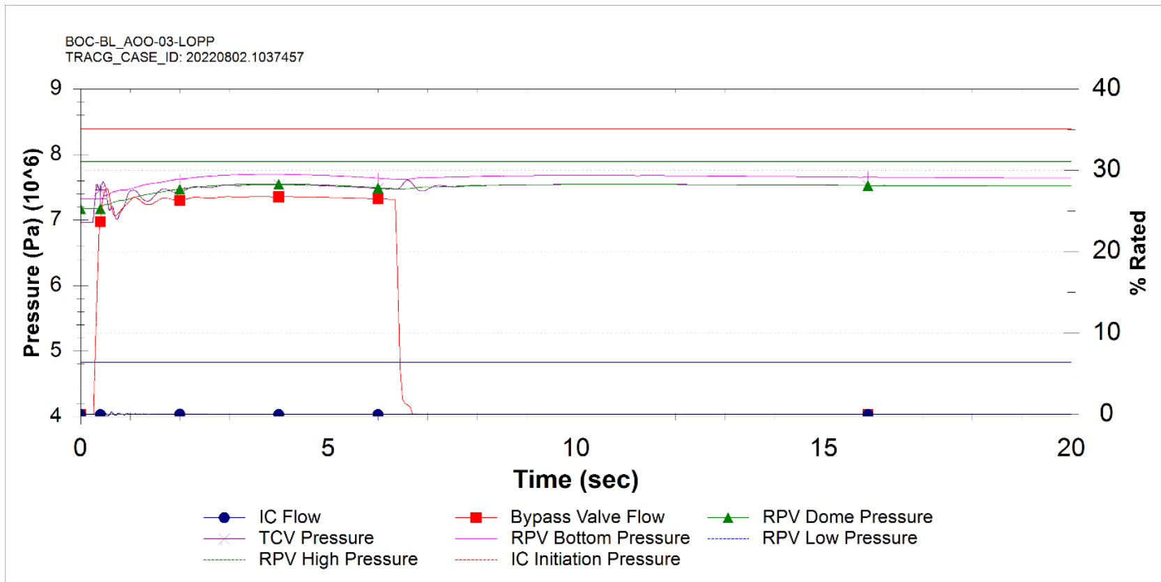
Figure 15.5-29: Loss of Preferred Power (AOO)
