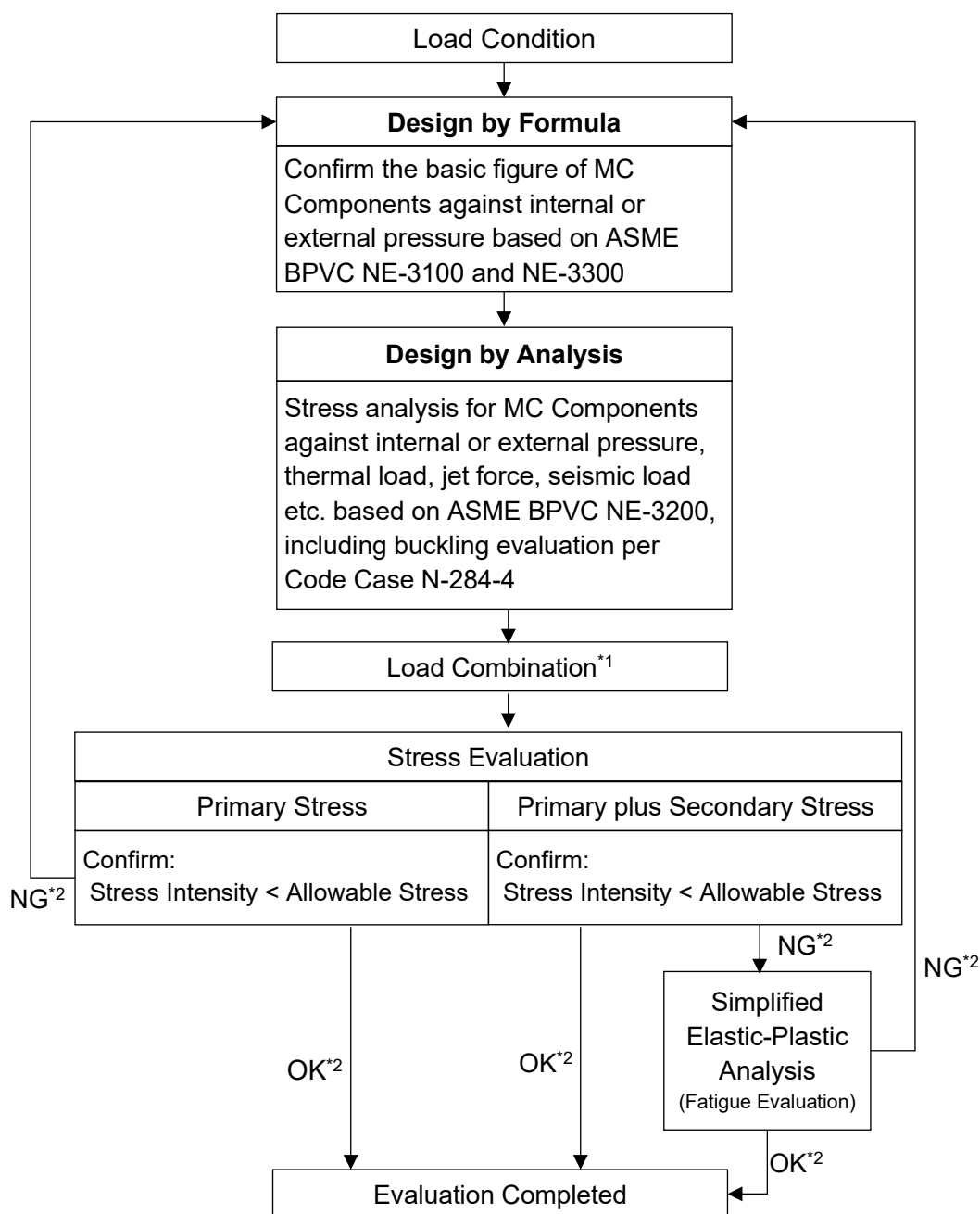
Figure 3.8-7: Design Procedures for Other Class MC Steel Components
