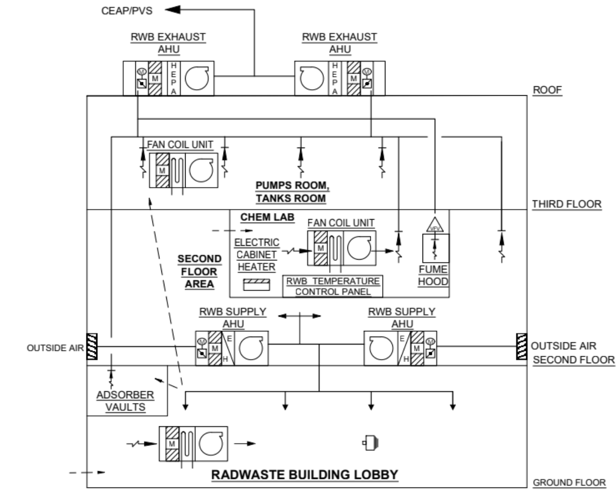
Figure 9.4-2: Radwaste Building Heating, Ventilation, and Cooling Simplified Diagram
