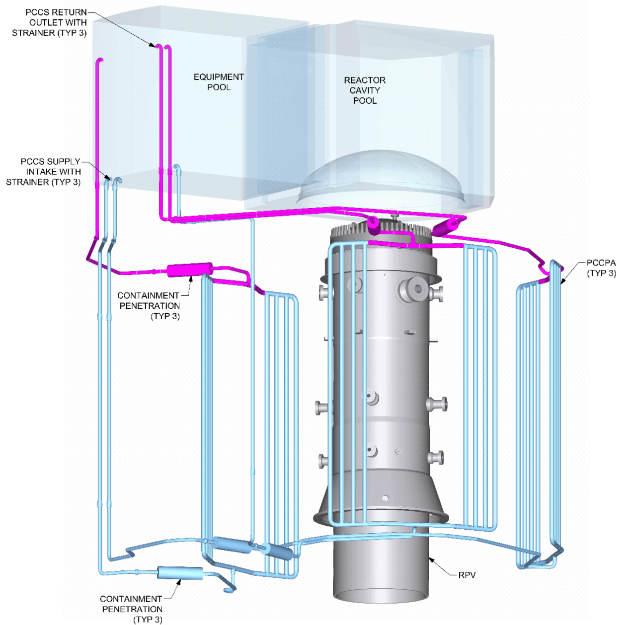
Figure 6.2-1: Passive Containment Cooling System Configuration
