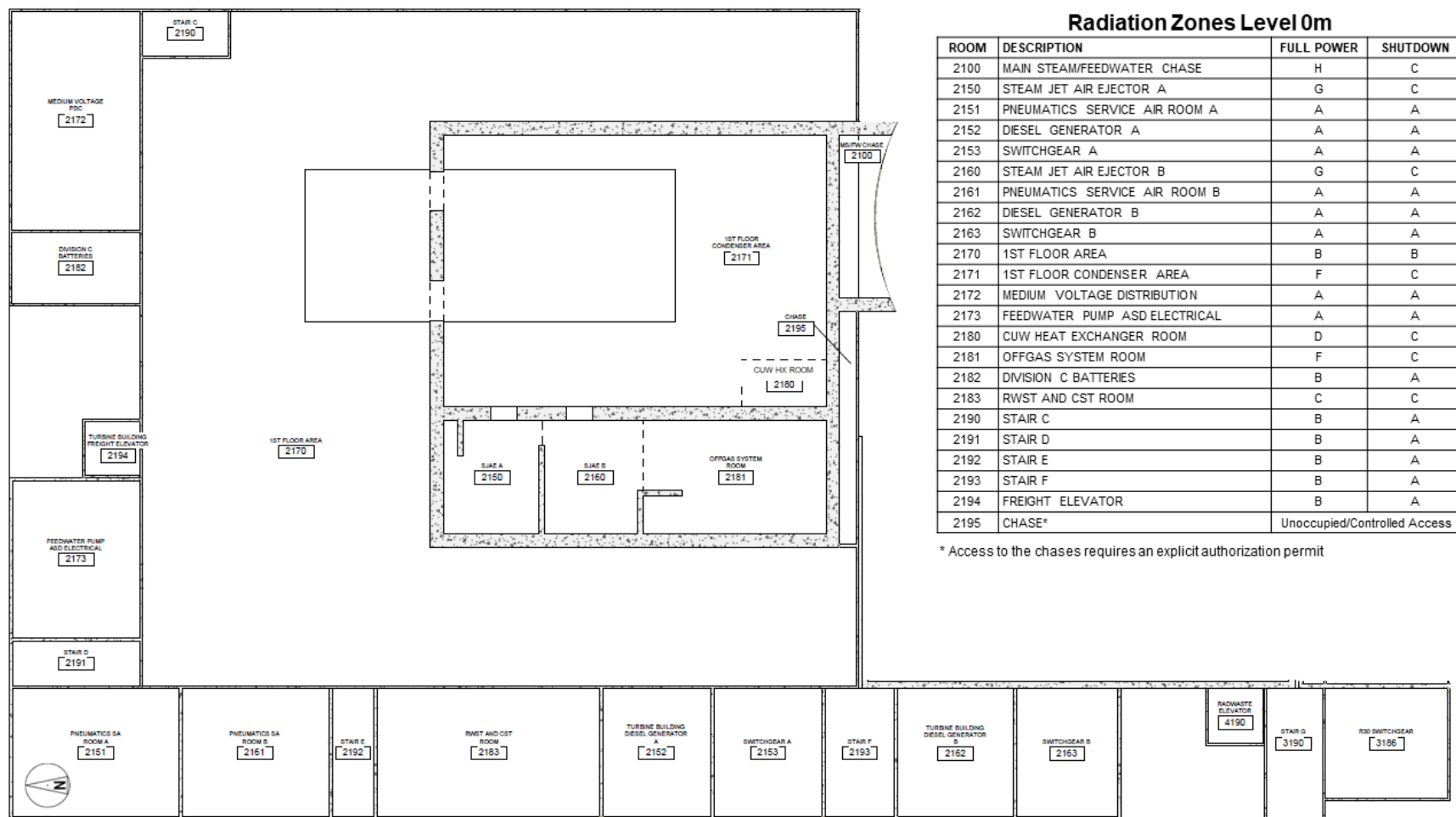
Figure 12.3-11: Turbine Building Level 0.0 Meters Radiation Zones
