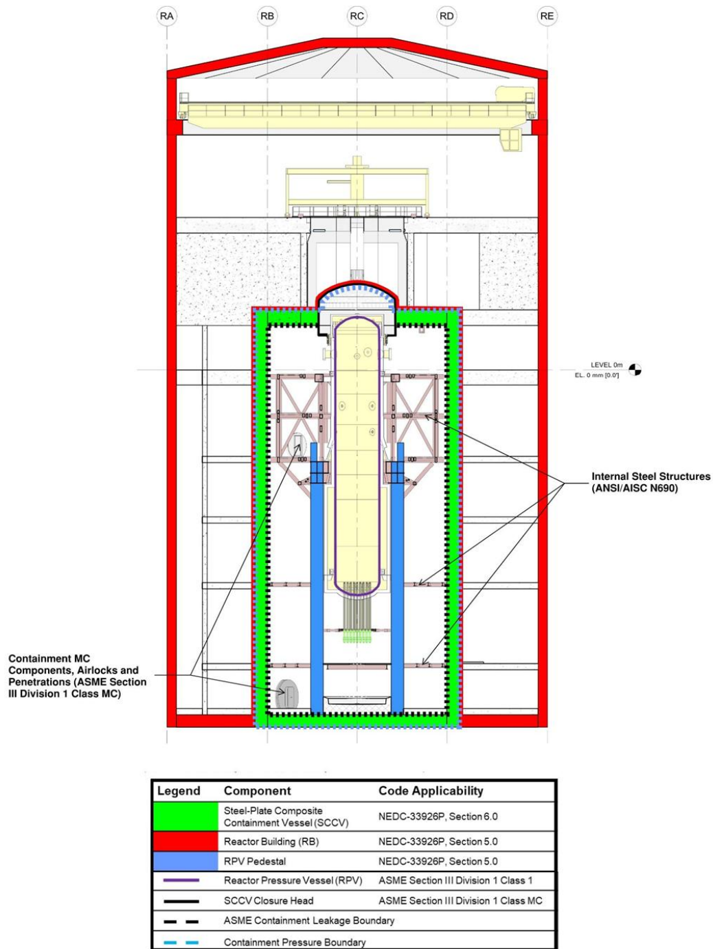
Figure 3.8-2: Structural Boundary of the BWRX-300 Containment, Containment Internal Structures and Reactor Building
