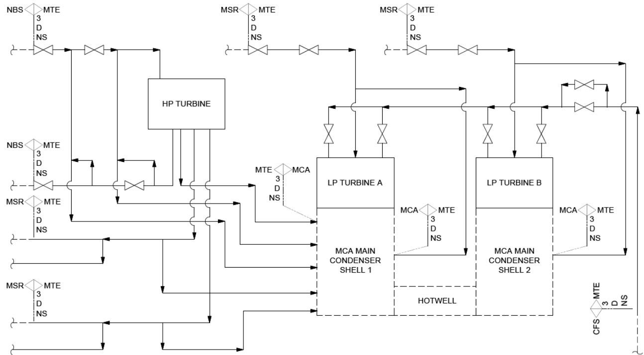
Figure 10.2-1: Main Turbine Equipment System Simplified Single Line Diagram
