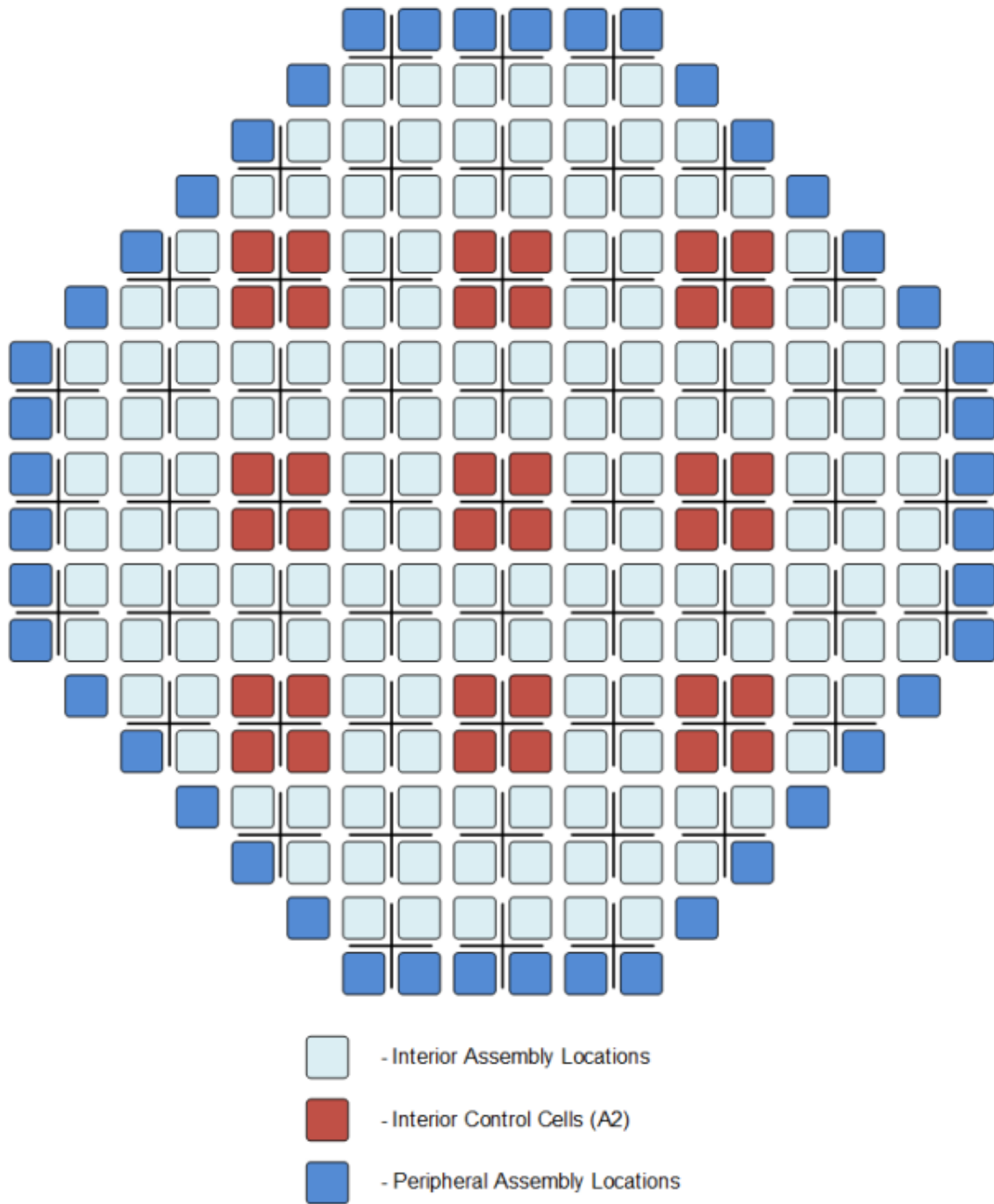
Figure 4.2-3: Control Rods Distributed Throughout Core
