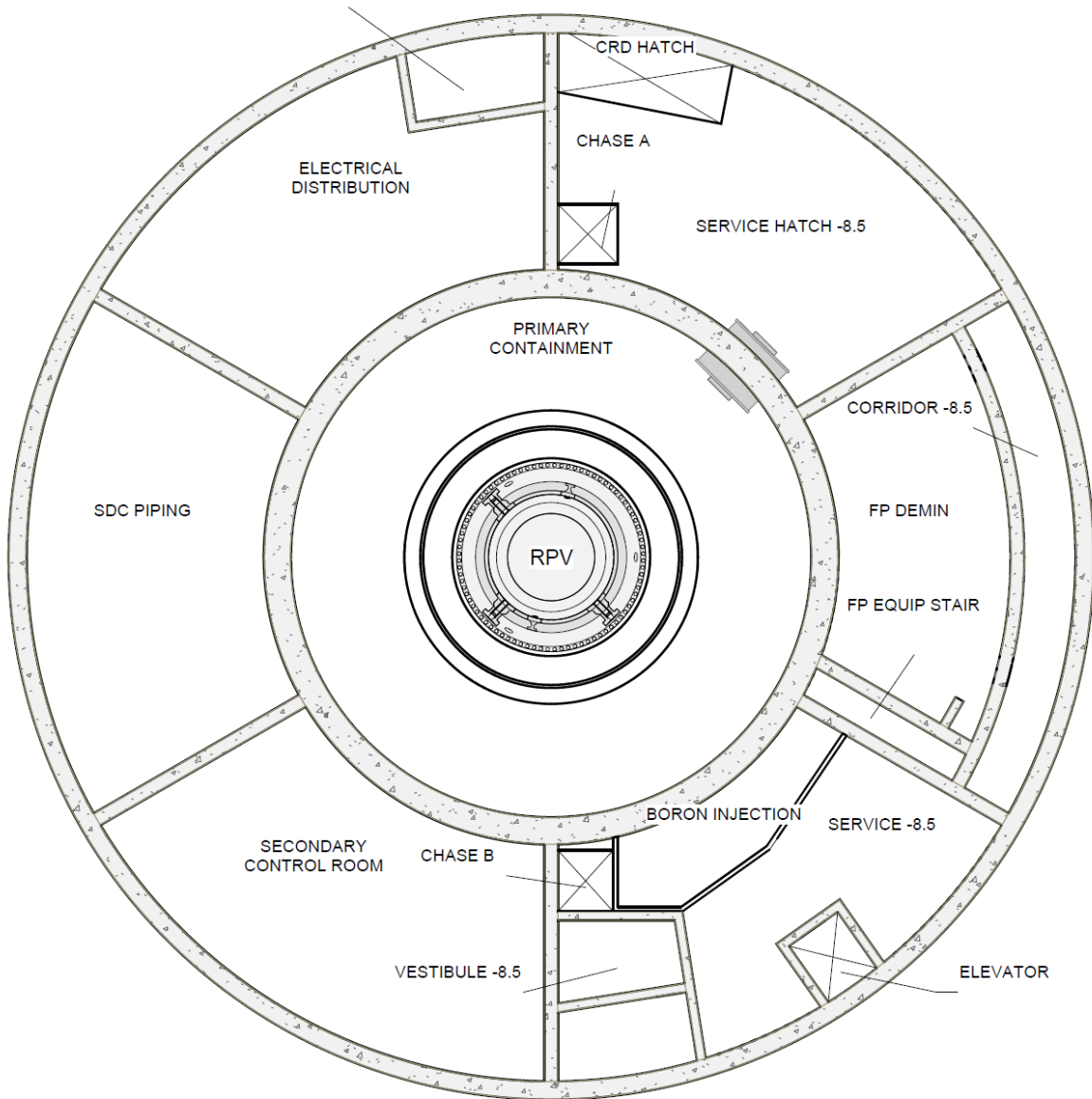
Figure 1.2-9: Reactor Building Plan View, Elevation -8.5m
