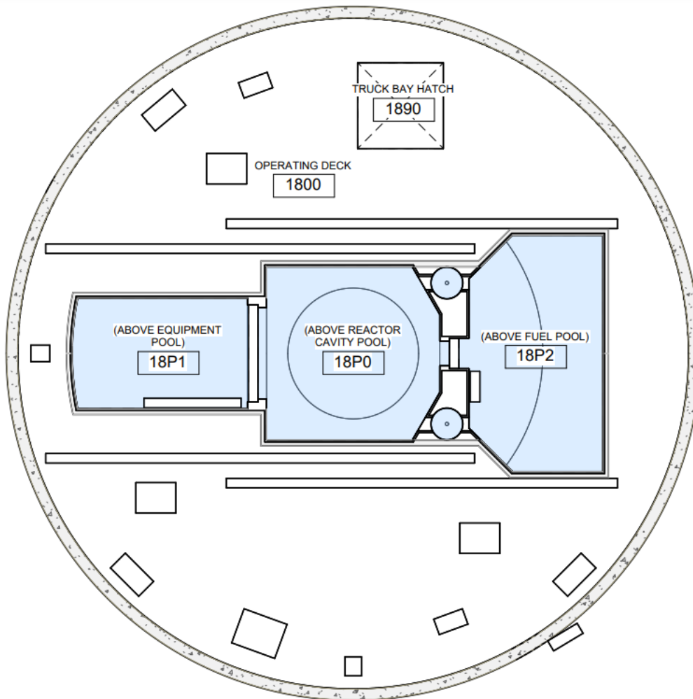
Figure 1.2-8: Reactor Building Plan View Elevation 13.0m
