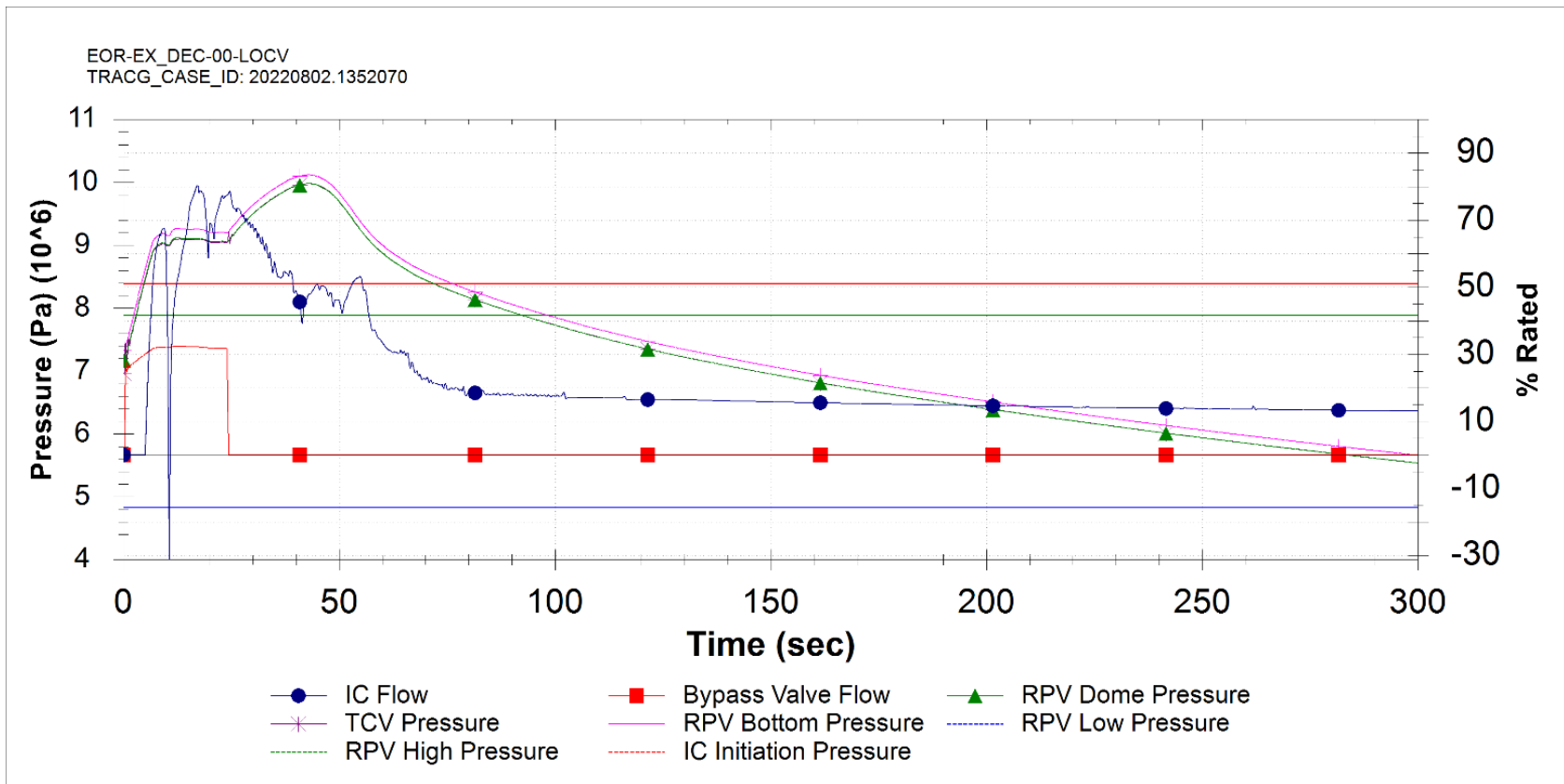
Figure 15.5-132: Loss of Condenser Vacuum (DEC)
