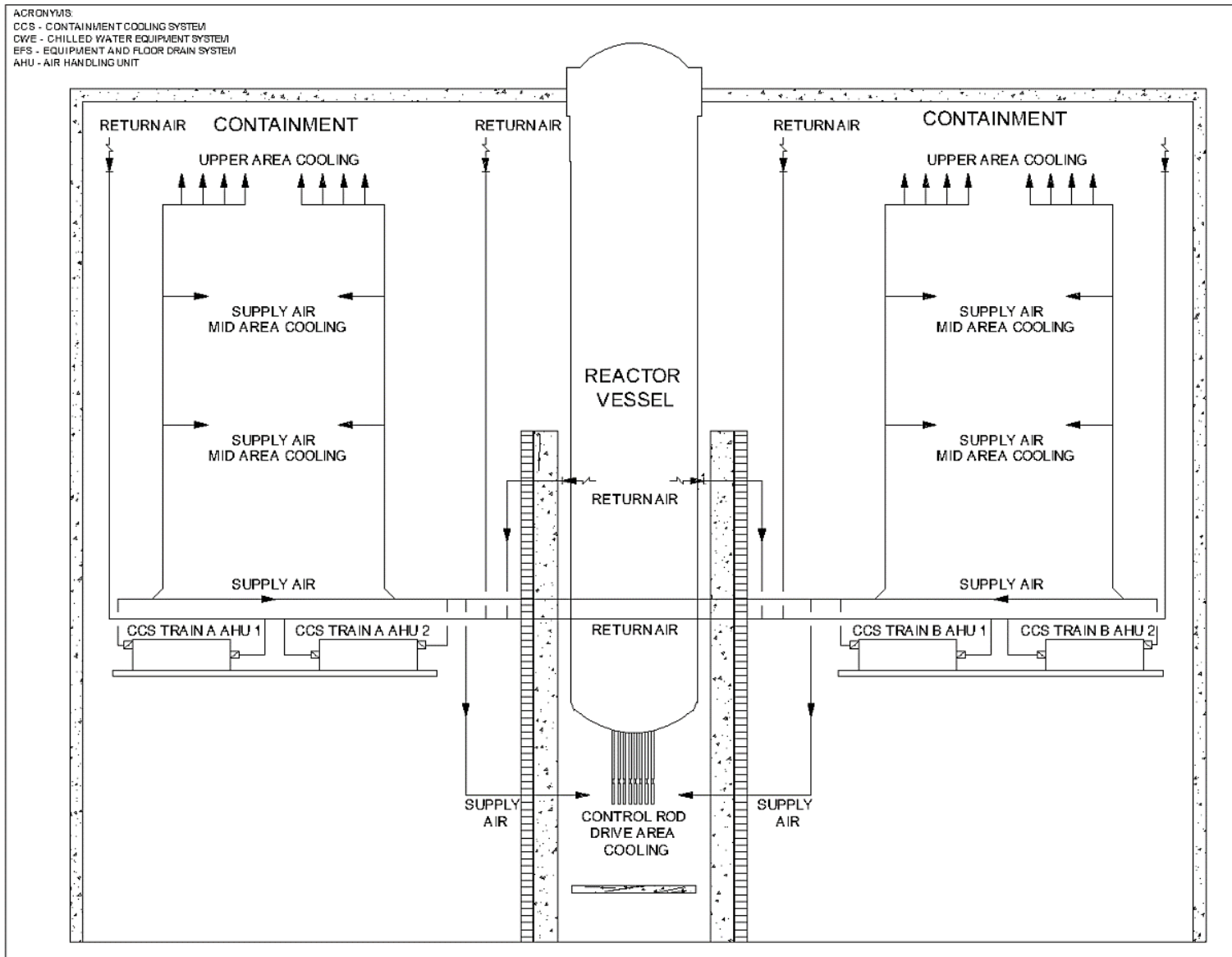
Figure 9.4-6: Containment Cooling System Simplified Diagram
