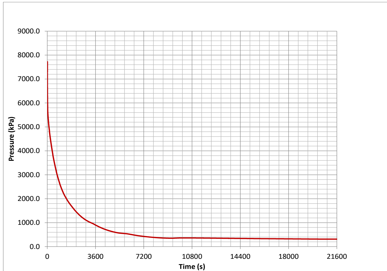
Figure 15.5-162: Reactor Pressure, Large FW Pipe Break, Conservative Case
