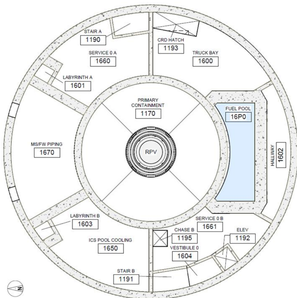
Figure 12.3-7: Reactor Building Level 0.0 Meters Radiation Zones
