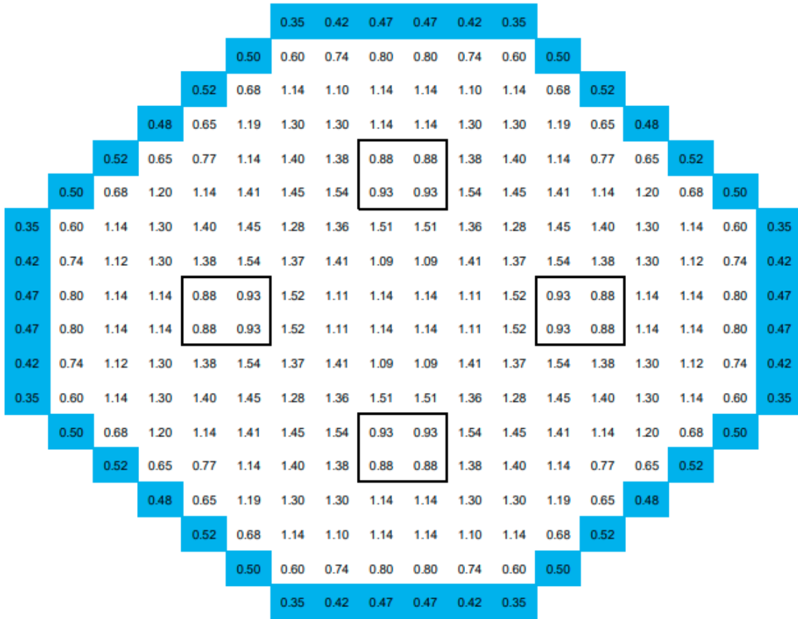
Figure 4.3-4a: Peak to Average Bundle Power Ratio at Beginning of Cycle (Average Bundle Power – 3.625 MW th )
