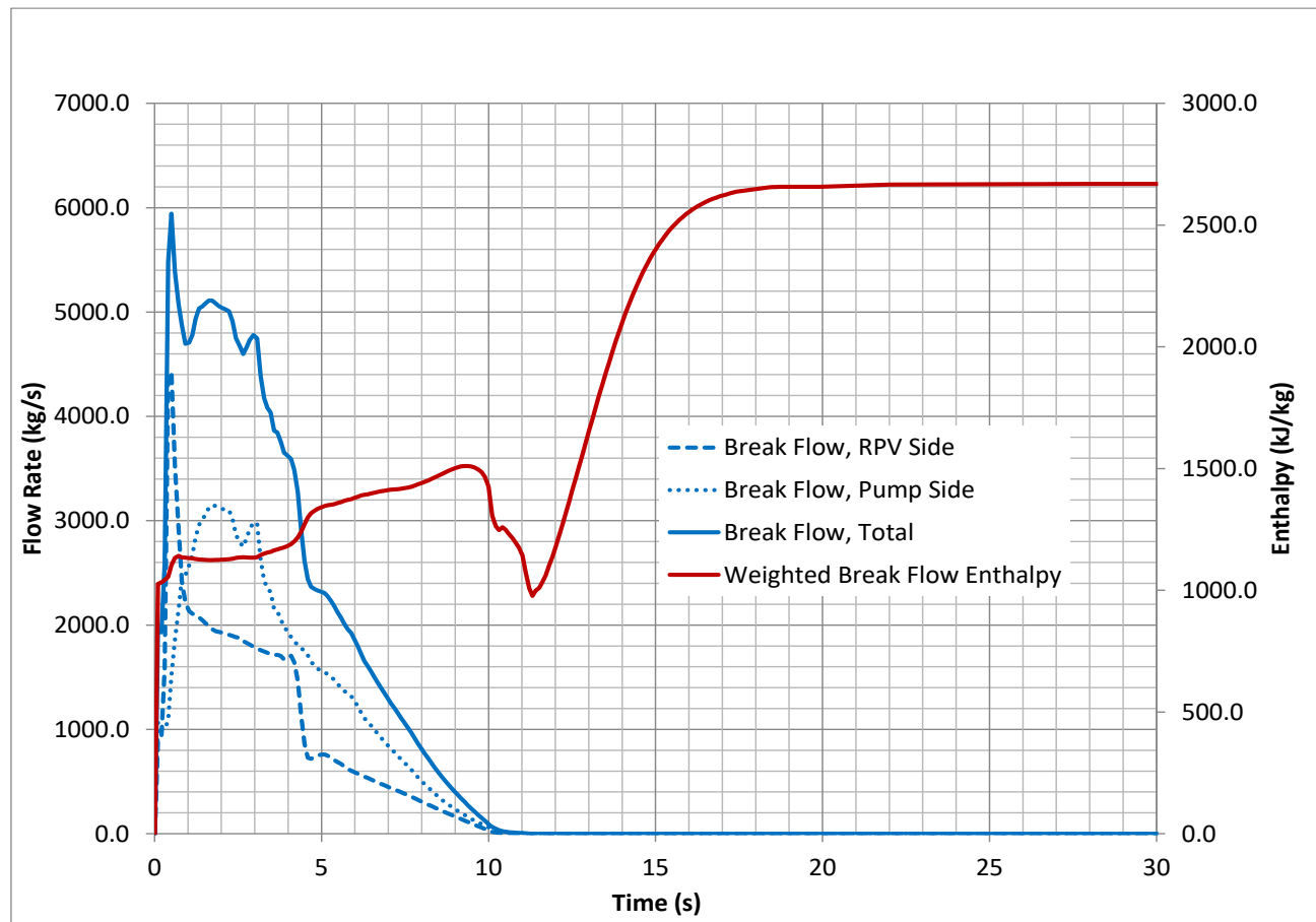
Figure 15.5-164: Break Flow Rate and Enthalpy, Large FW Pipe Break, Conservative Case
