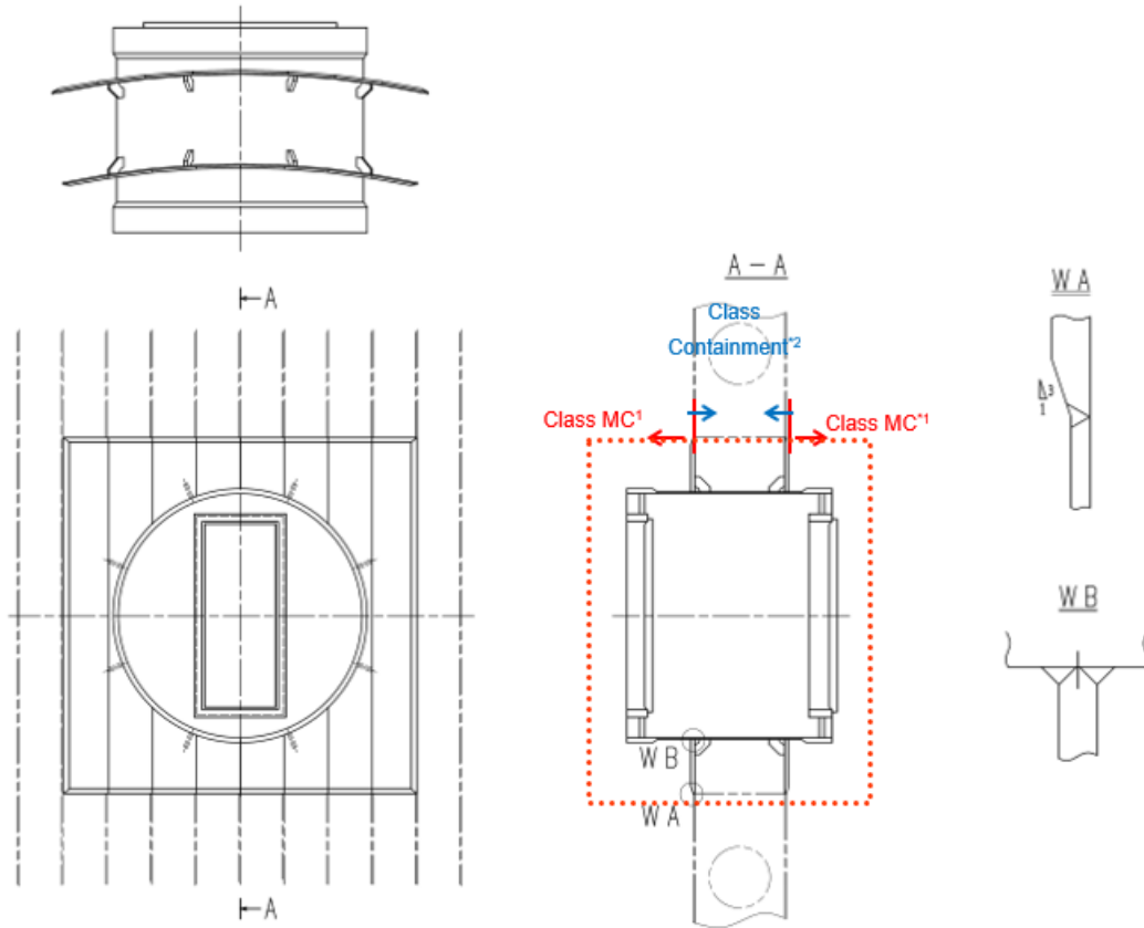
Figure 3.8-4: Containment Airlock Code Jurisdictional Boundary
