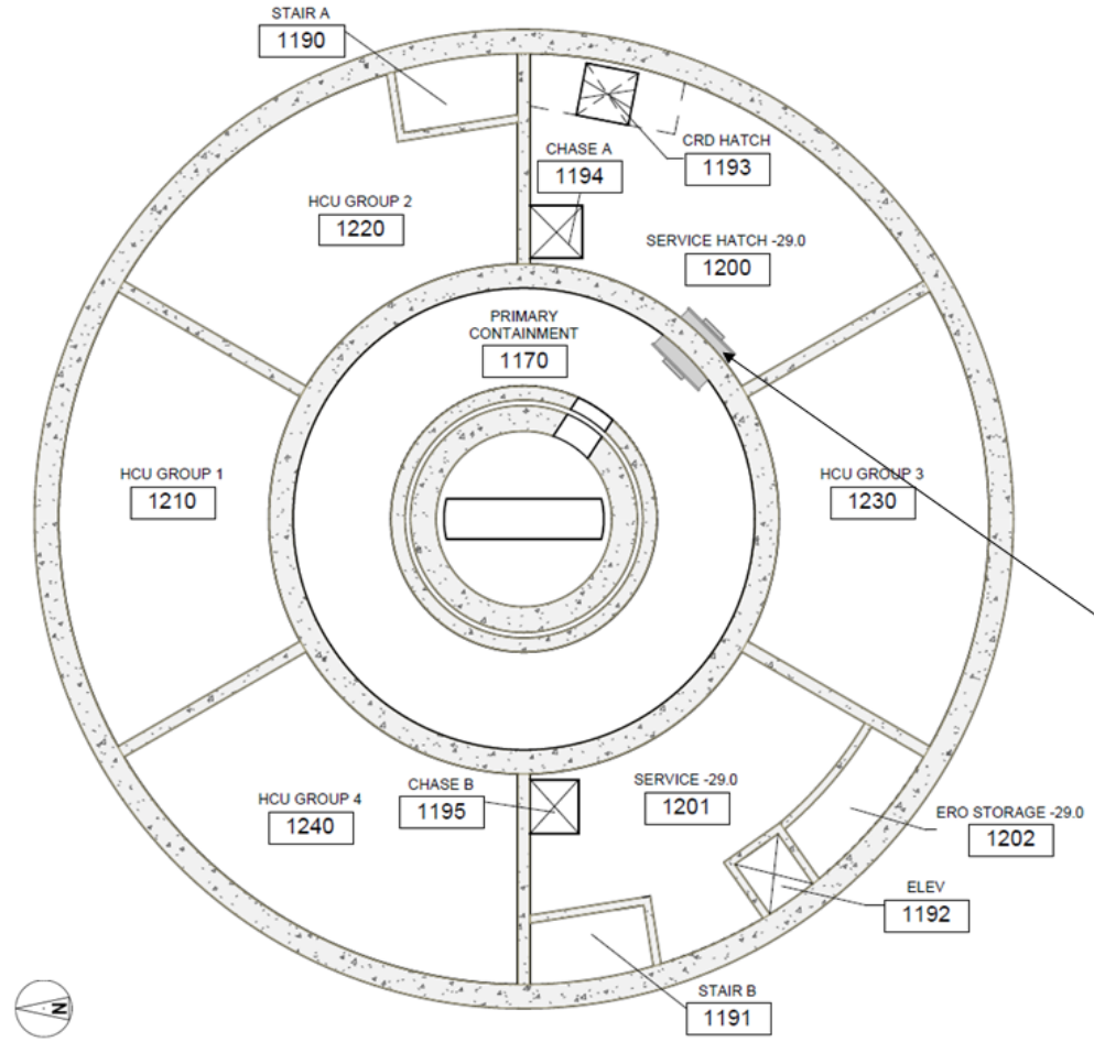
Figure 12.3-2: Reactor Building Level -29.0 Meters Radiation Zones
