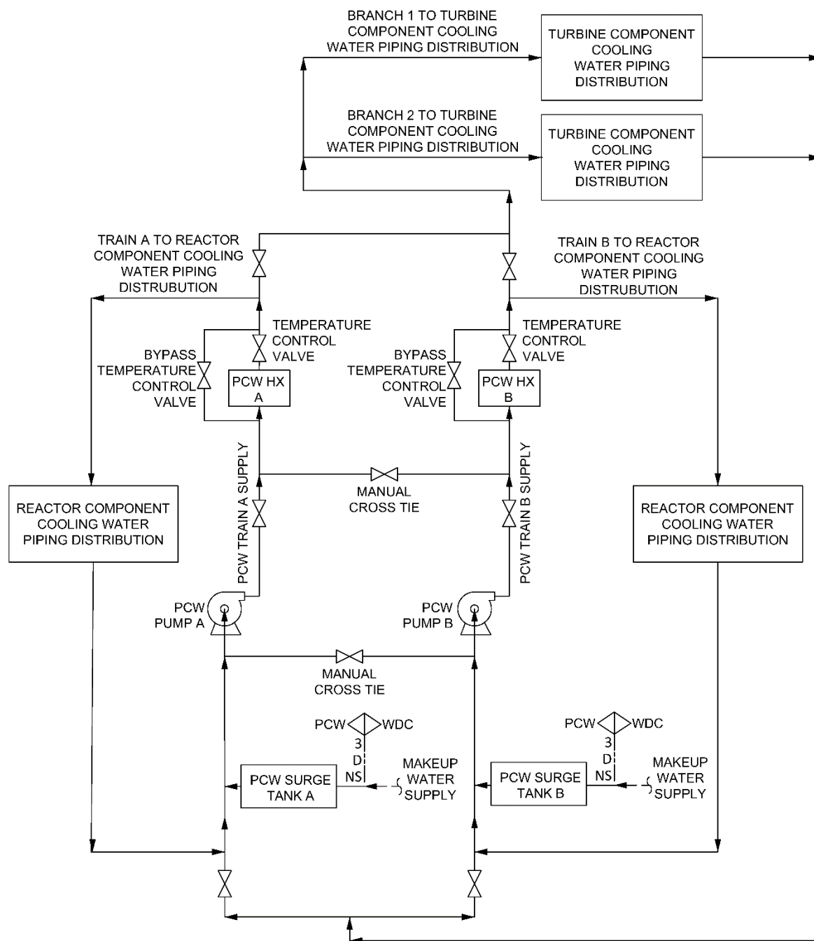
Figure 9.2-2: Plant Cooling Water System Simplified Diagram
