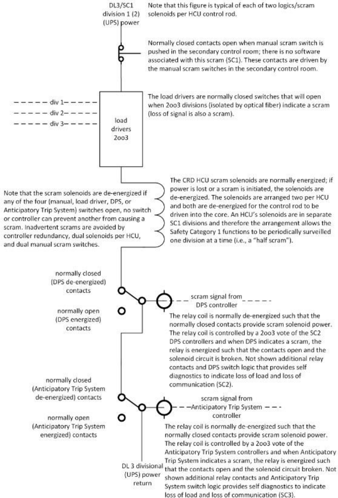
Figure 7.3-4: BWRX-300 Hydraulic Scram Solenoid Control and Power
