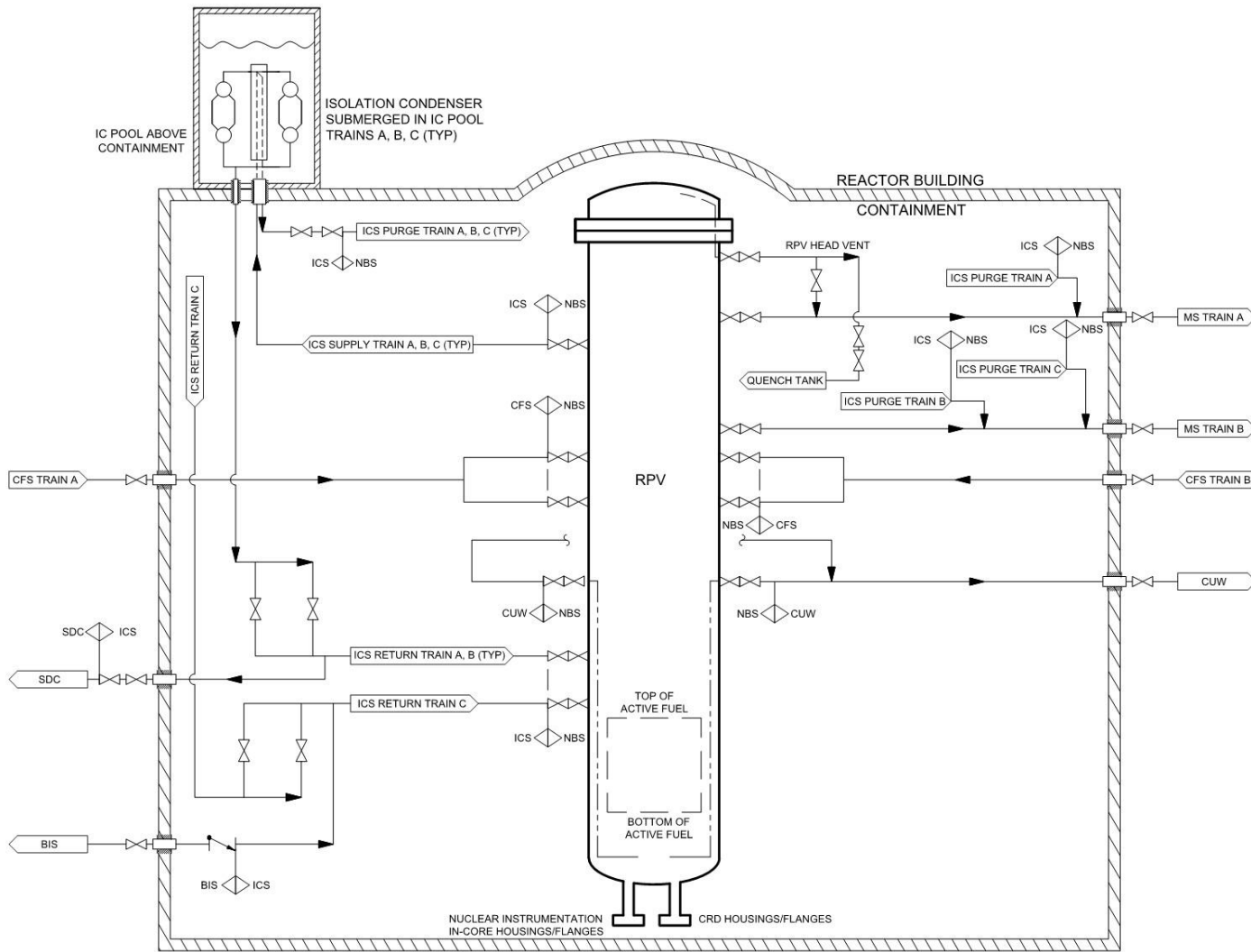
Figure 5.1-2: BWRX-300 Reactor Coolant Pressure Boundary
