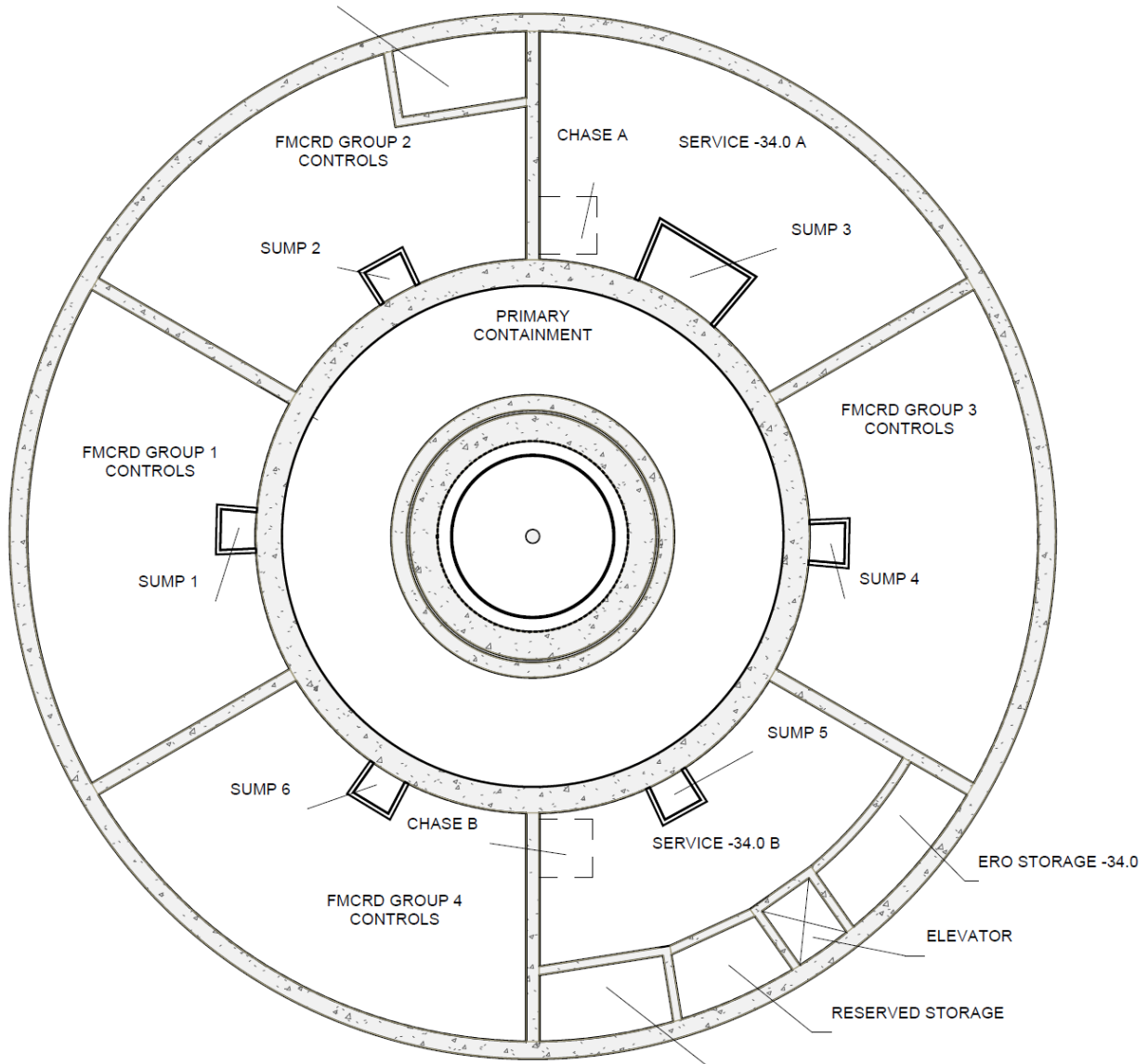
Figure 1.2-13: Reactor Building Plan View, Elevation -34.0m
