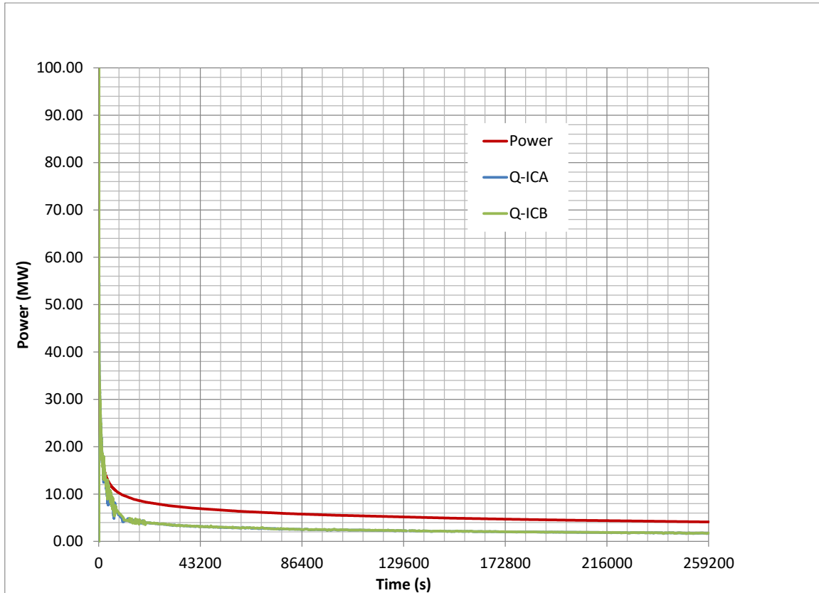
Figure 15.5-112: Reactor Power, Small Liquid Pipe Break, Conservative Case
