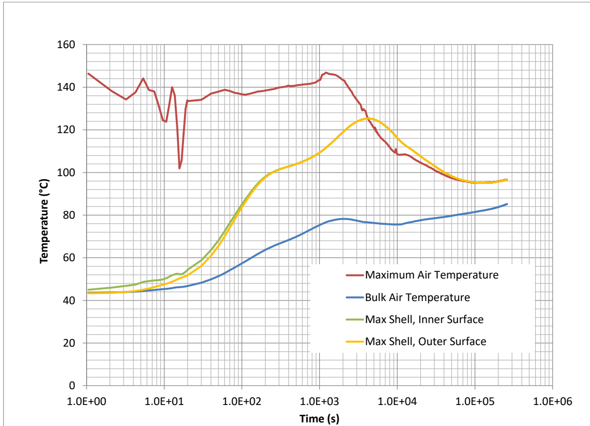
Figure 15.5-111: Containment Temperature, Small Steam Pipe Break with LOPP, Conservative Case
