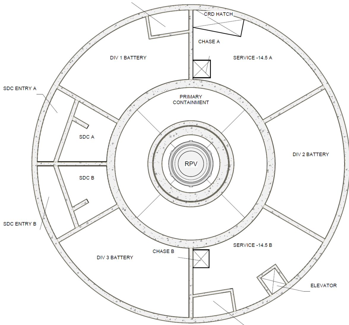
Figure 1.2-10: Reactor Building Plan View, Elevation -14.5m
