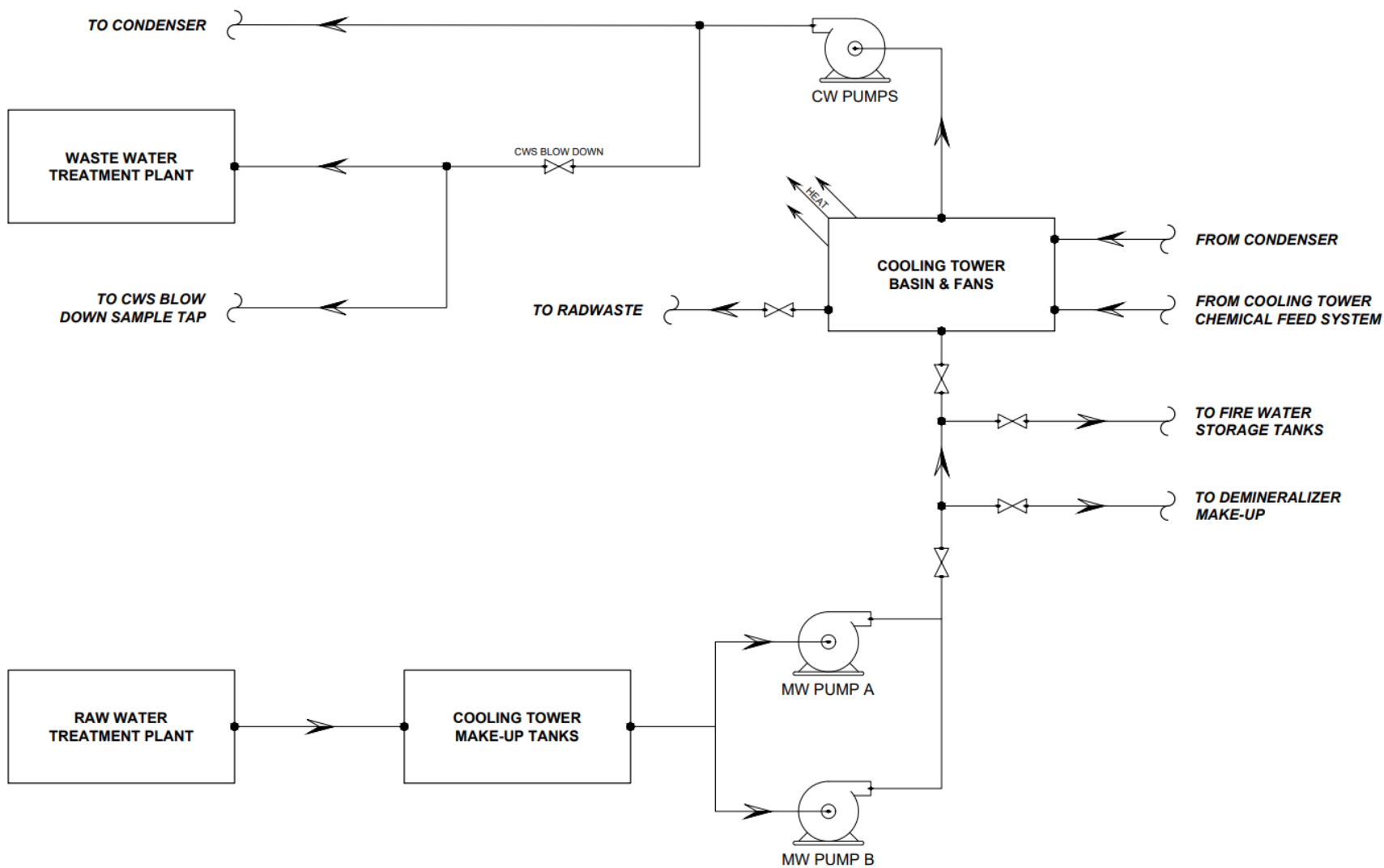
Figure 9.2-7: Normal Heat Sink System Simplified Diagram
