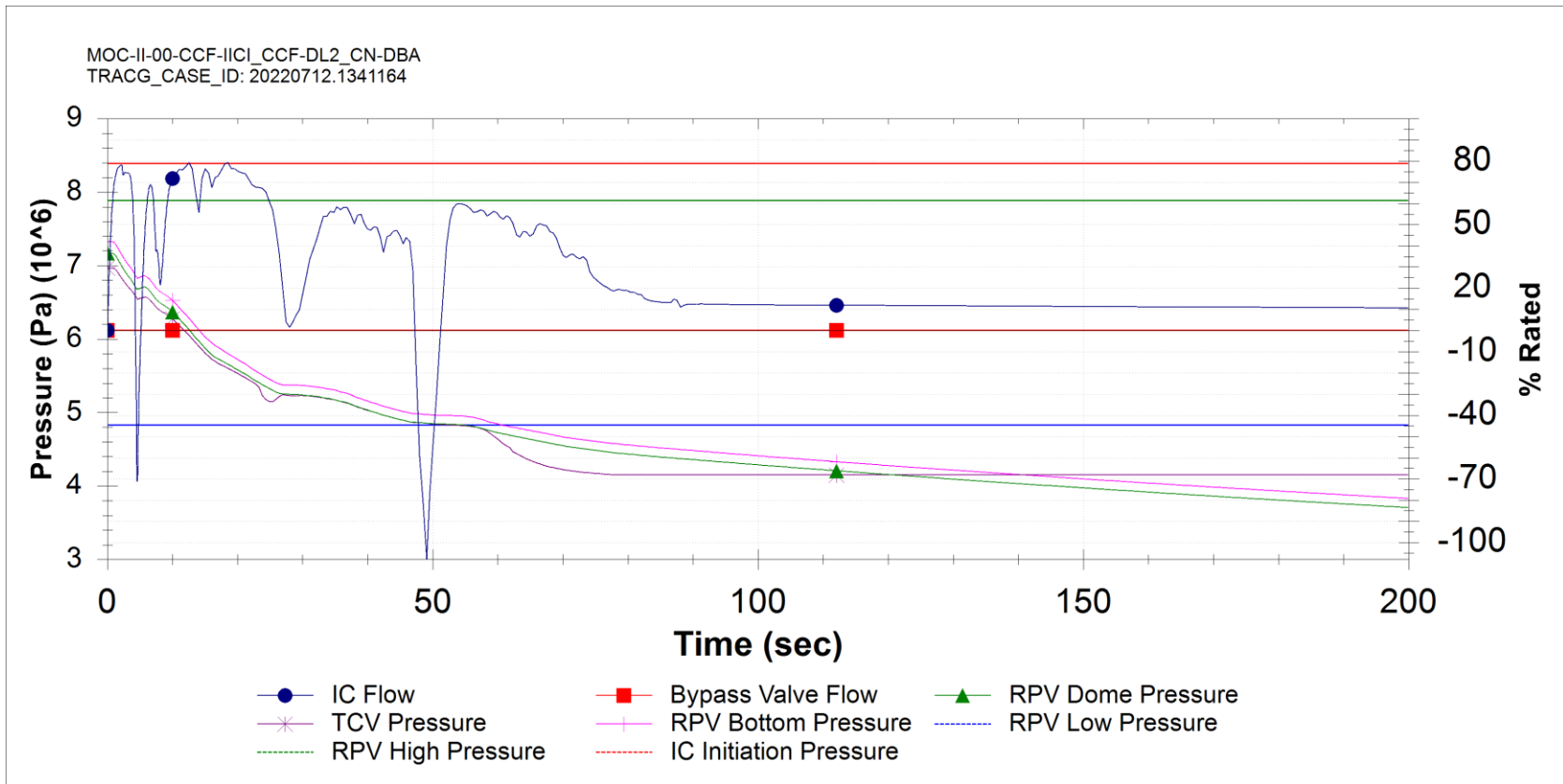
Figure 15.5-83: Inadvertent Isolation Condenser Initiation - All Trains (DBA)
