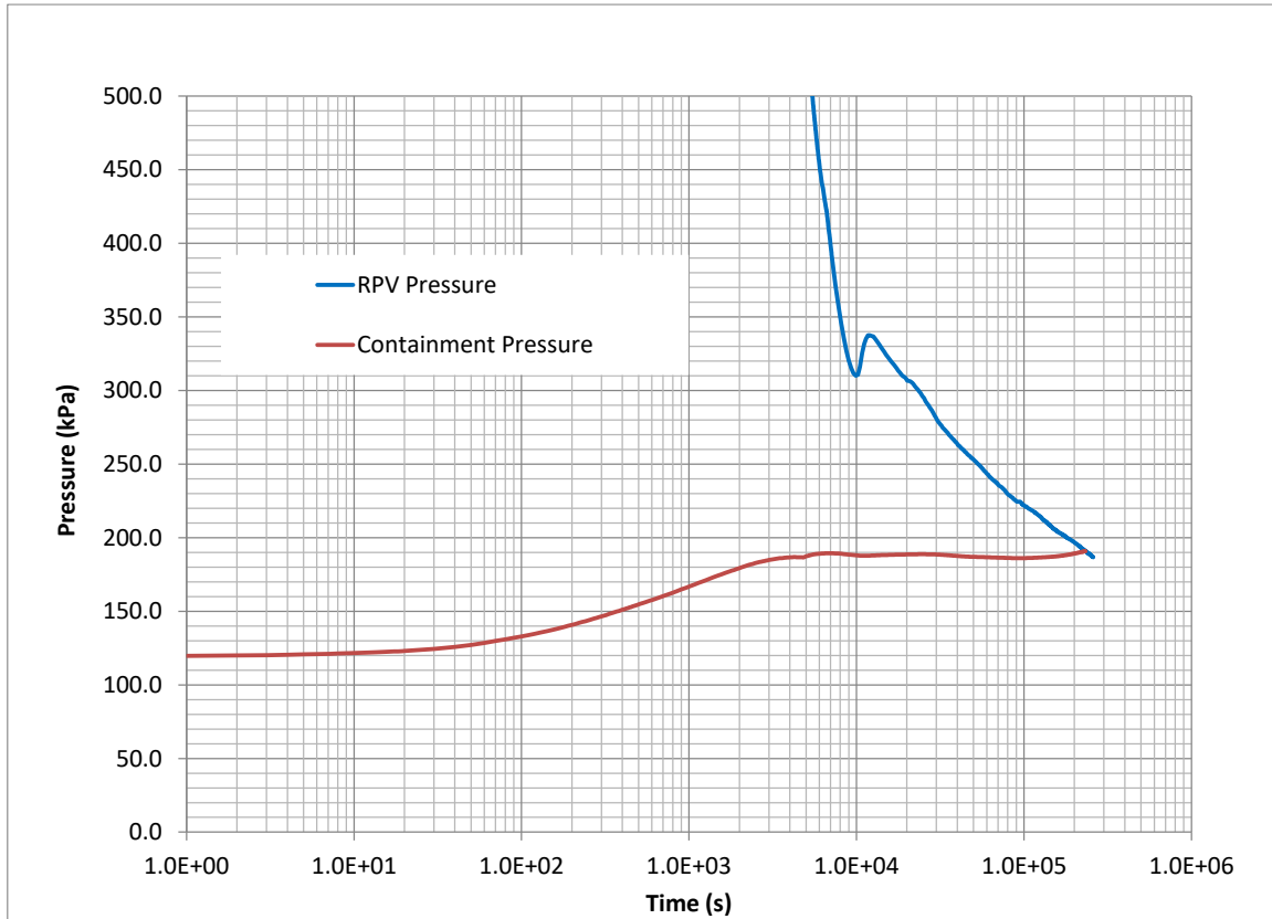
Figure 15.5-117: Containment Pressure, Small Liquid Pipe Break, Conservative Case
