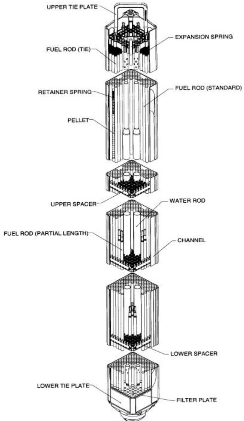
Figure 4.2-1: GNF2 Fuel Assembly
