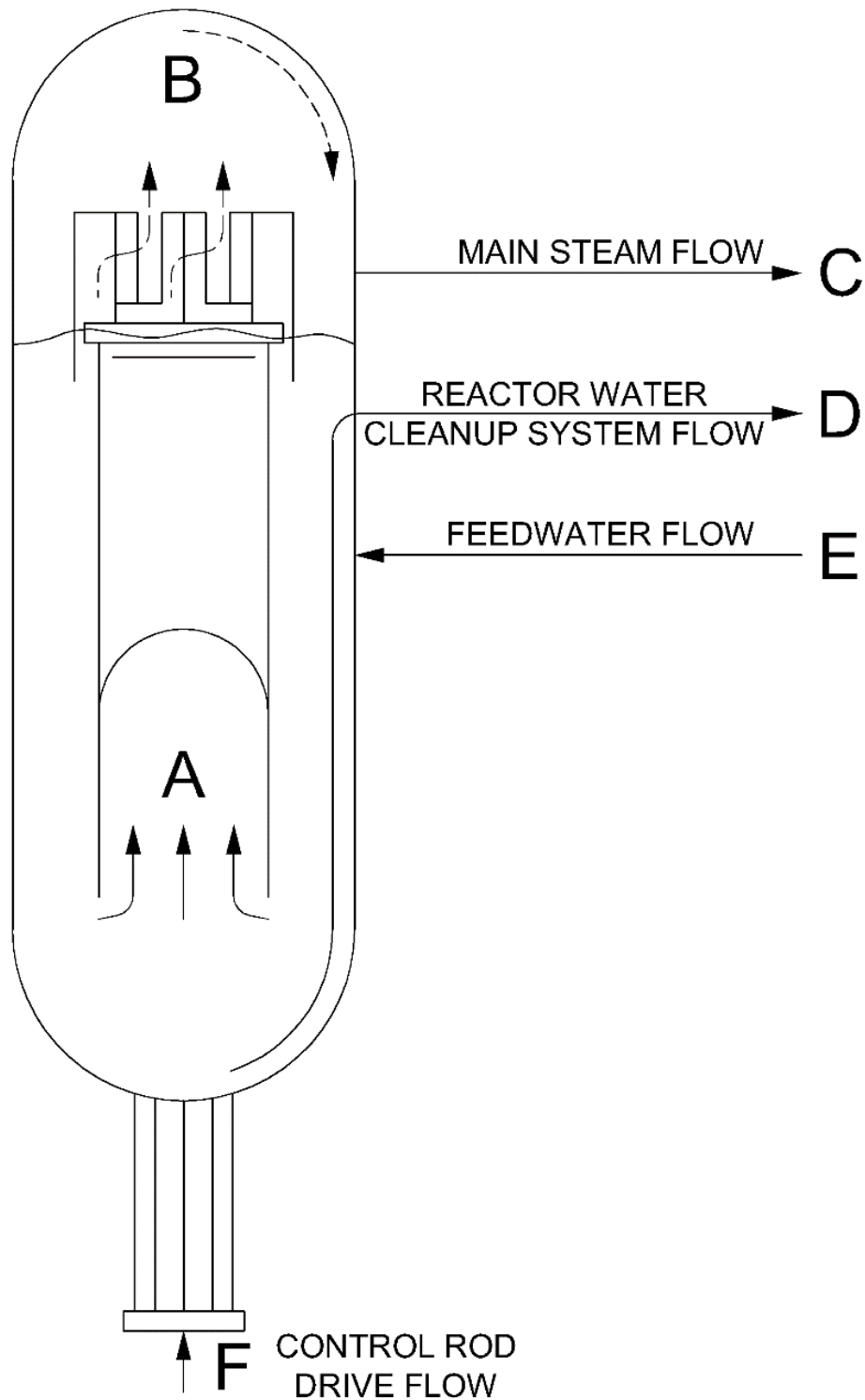
Figure 5.1-5: BWRX-300 Reactor Coolant System Schematic Flow Diagram at 100% Power
