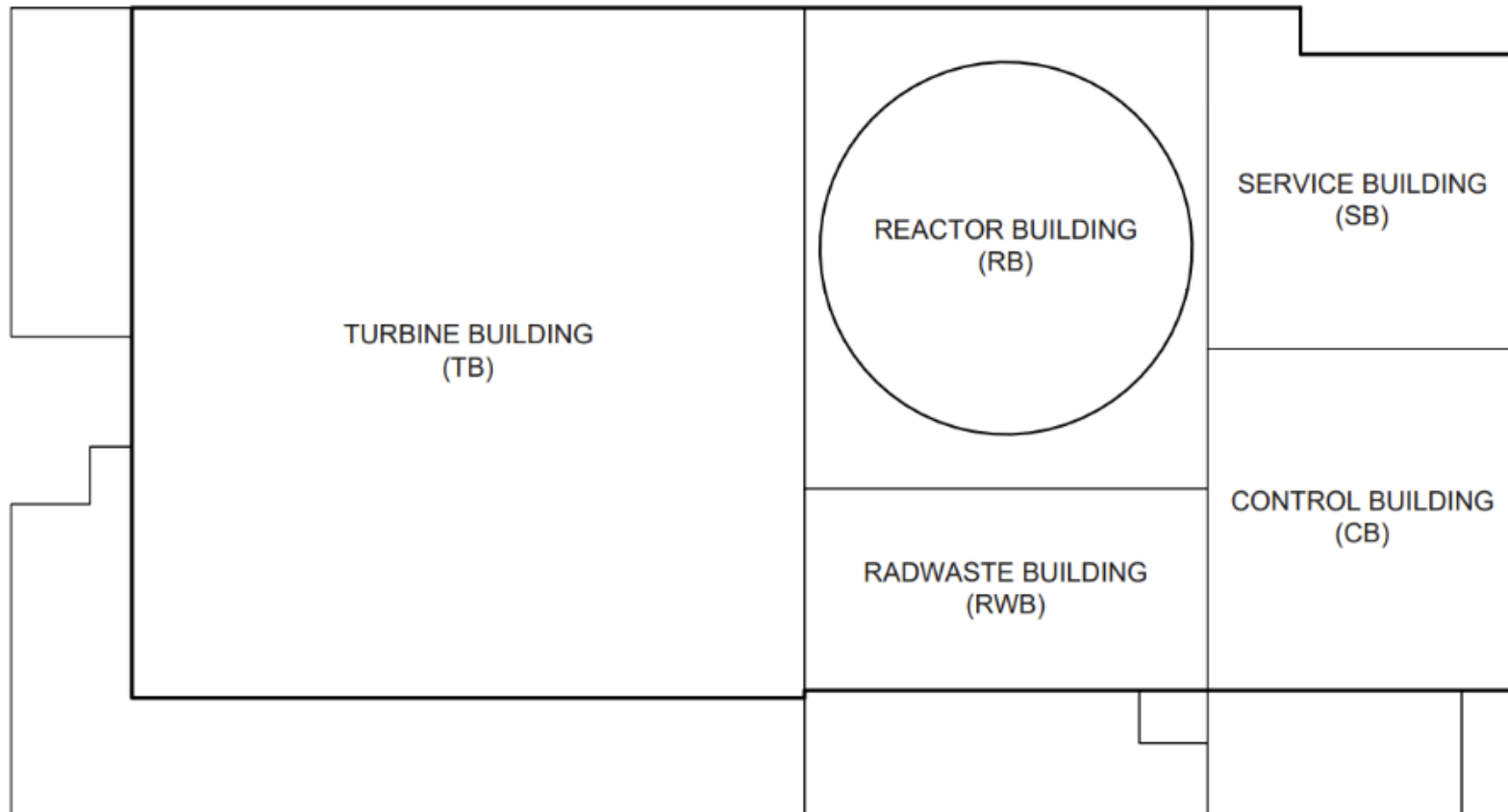
Figure 1.2-1b: BWRX-300 Power Block General Arrangement
