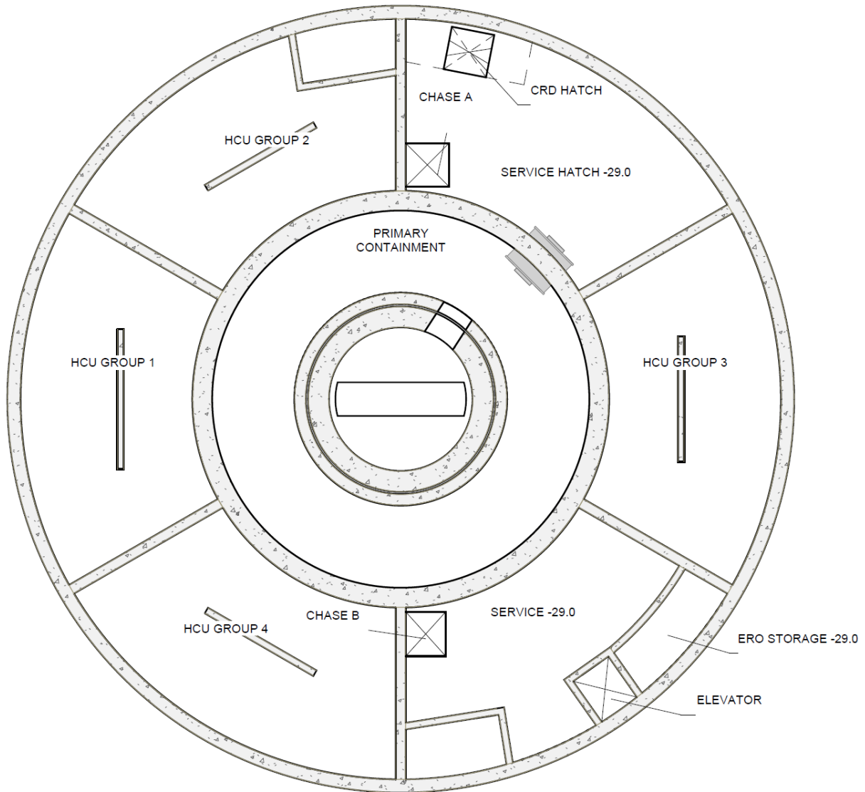
Figure 1.2-12: Reactor Building Plan View, Elevation -29.0m
