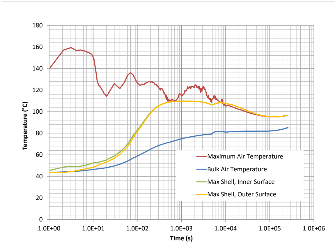
Figure 15.5-118: Containment Temperature, Small Liquid Pipe Break, Conservative Case
