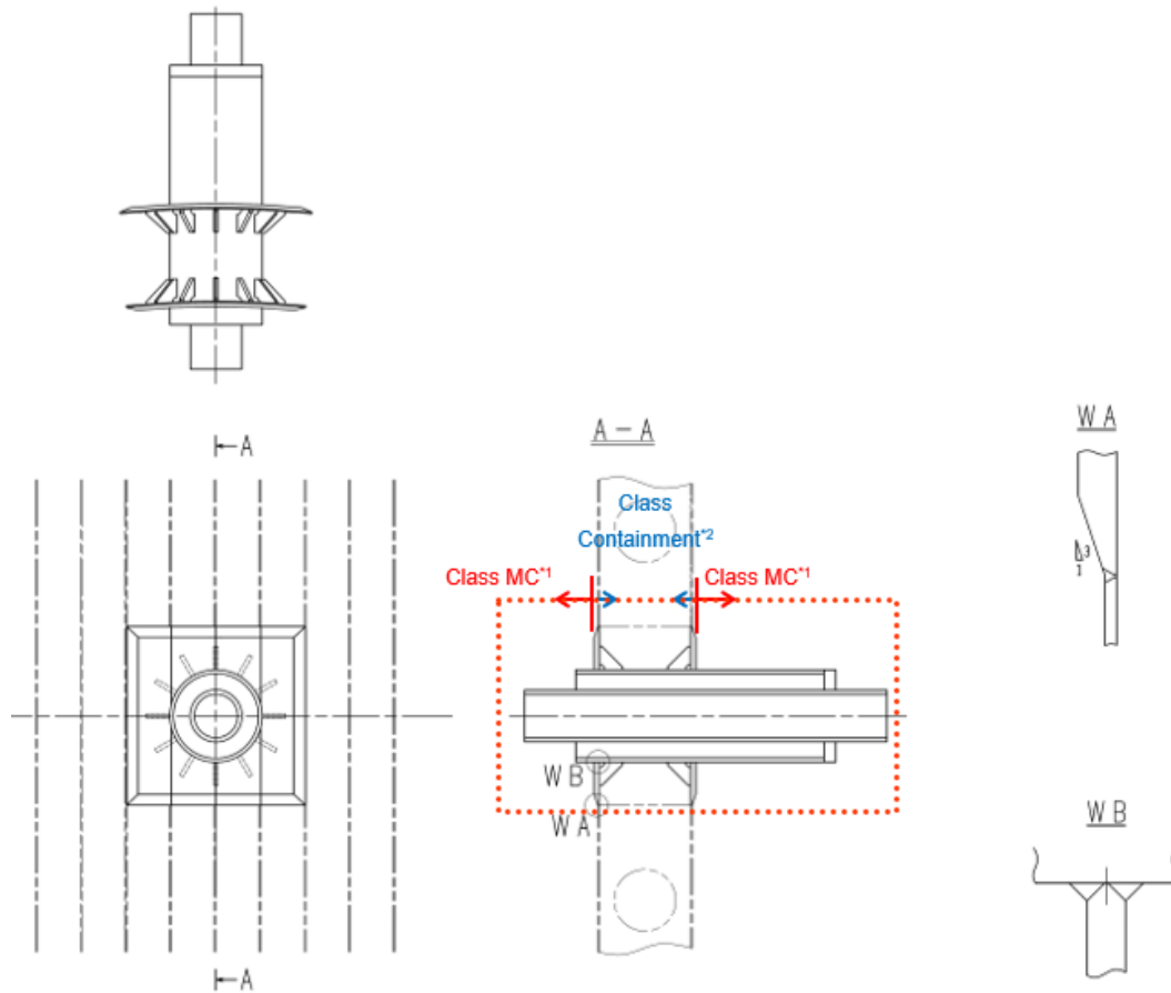
Figure 3.8-5: Penetrations Jurisdictional Boundary
