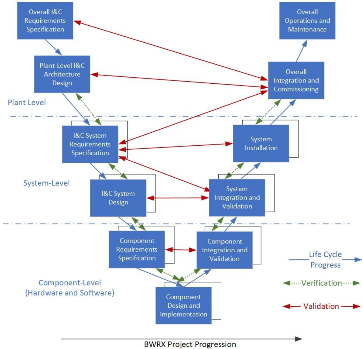
Figure 7.4-2: Overall BWRX-300 Instrumentation and Control System Life Cycle
