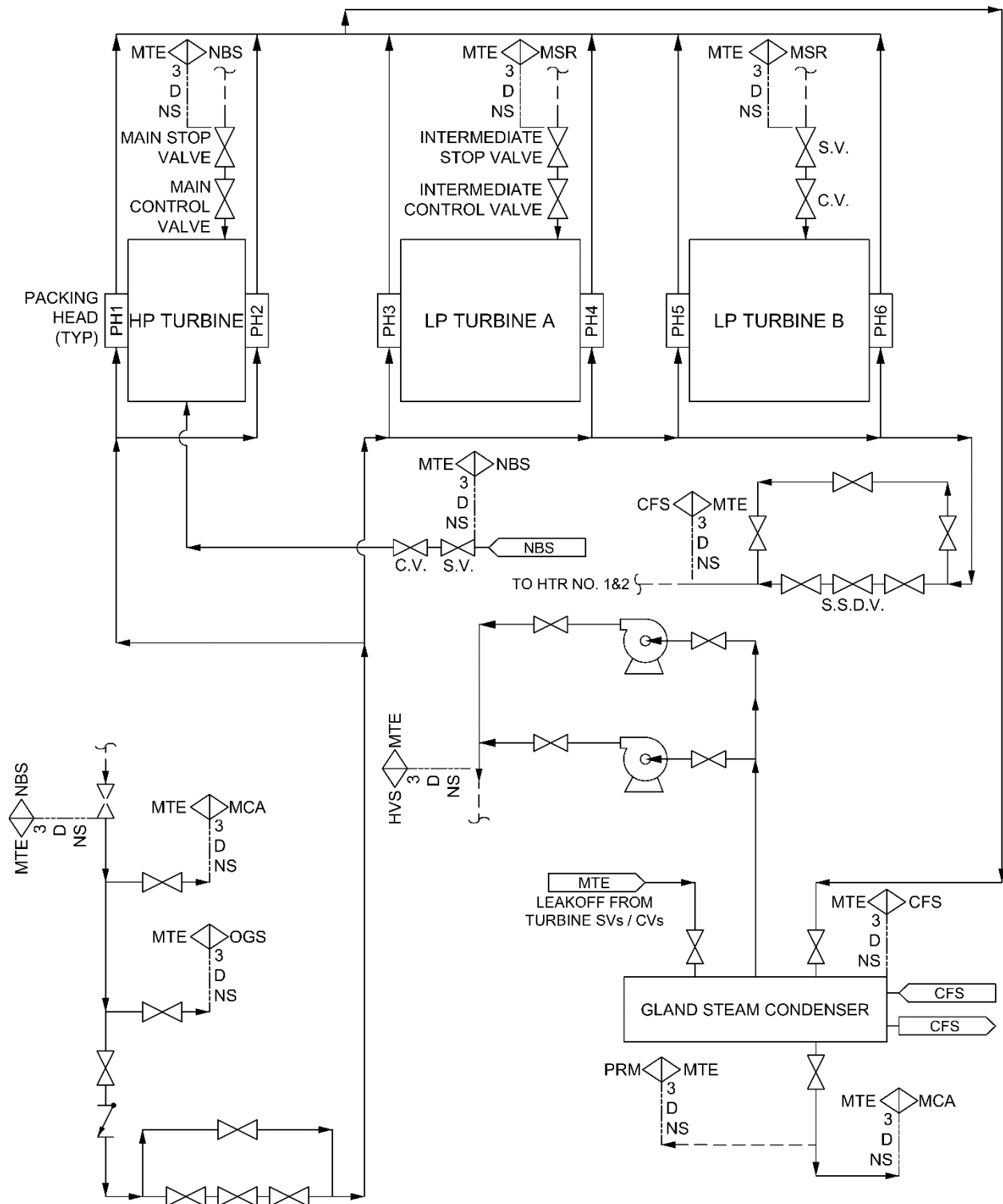
Figure 10.4-3: Turbine Gland Seal System Simplified Diagram
