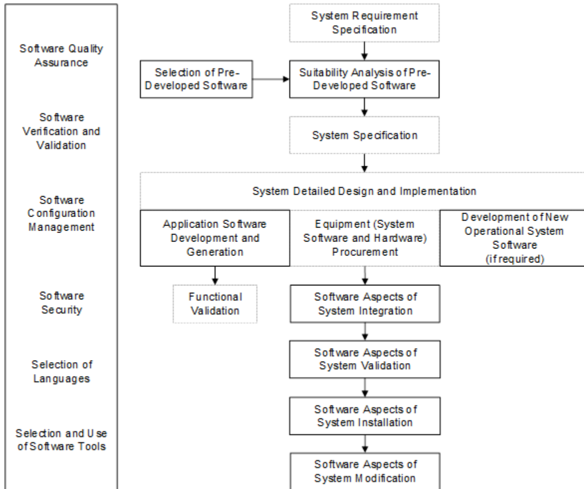
Figure 7.4-3: Software Related Activities in Instrumentation and Control System Life Cycle
