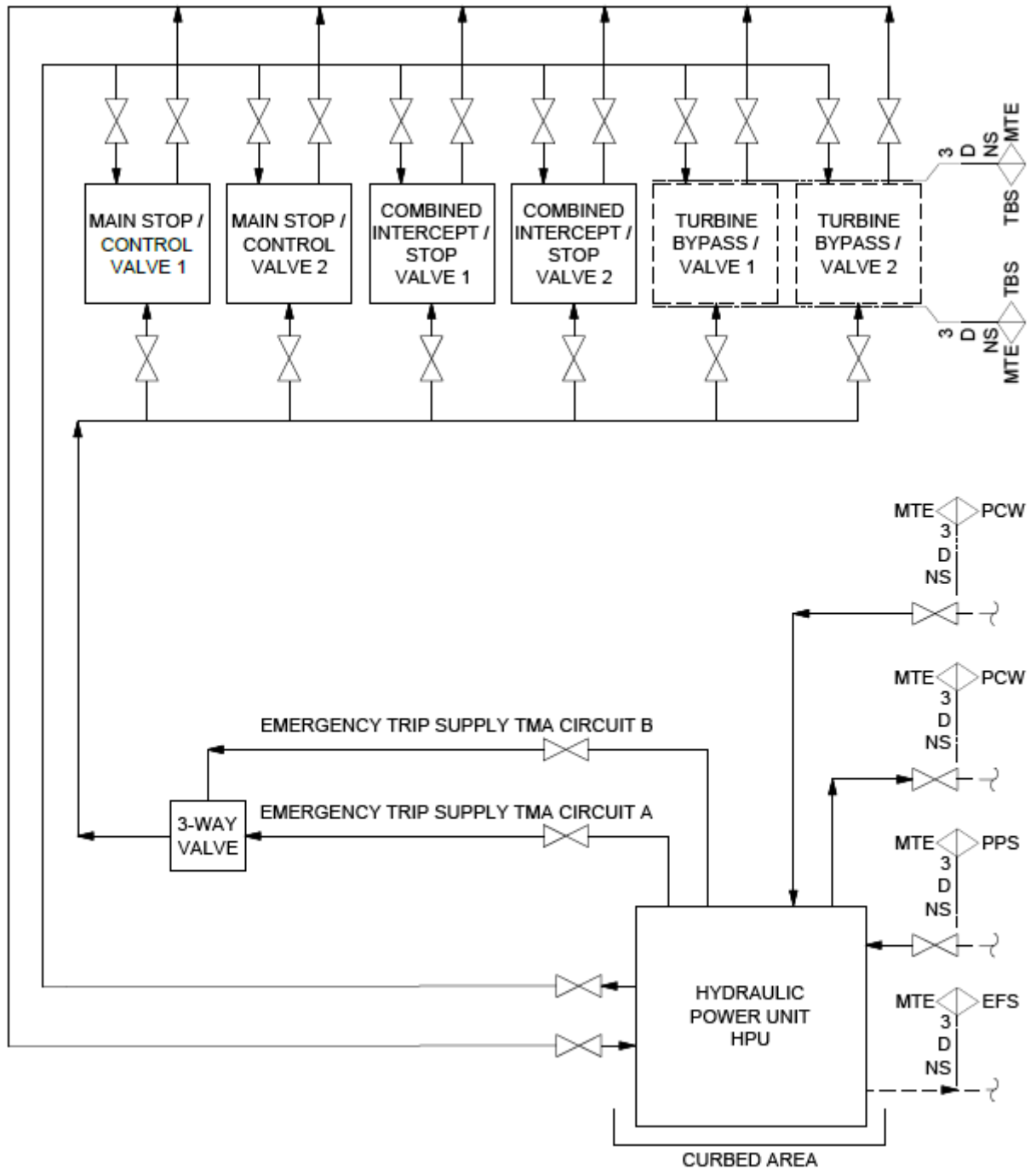
Figure 10.2-4: Electro-Hydraulic Control System Simplified Single Line Diagram
