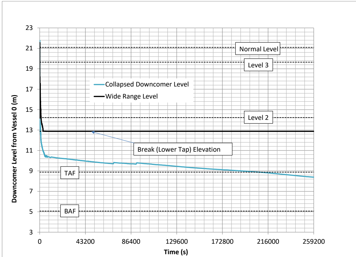
Figure 15.5-114: Reactor Water Level, Small Liquid Break, Conservative Case
