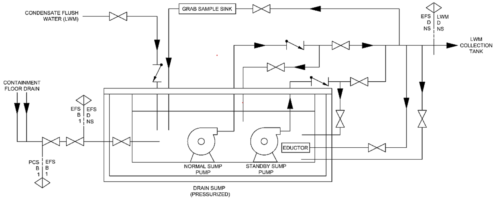
Figure 9.3-3: Pressurized Sump Simplified Diagram
