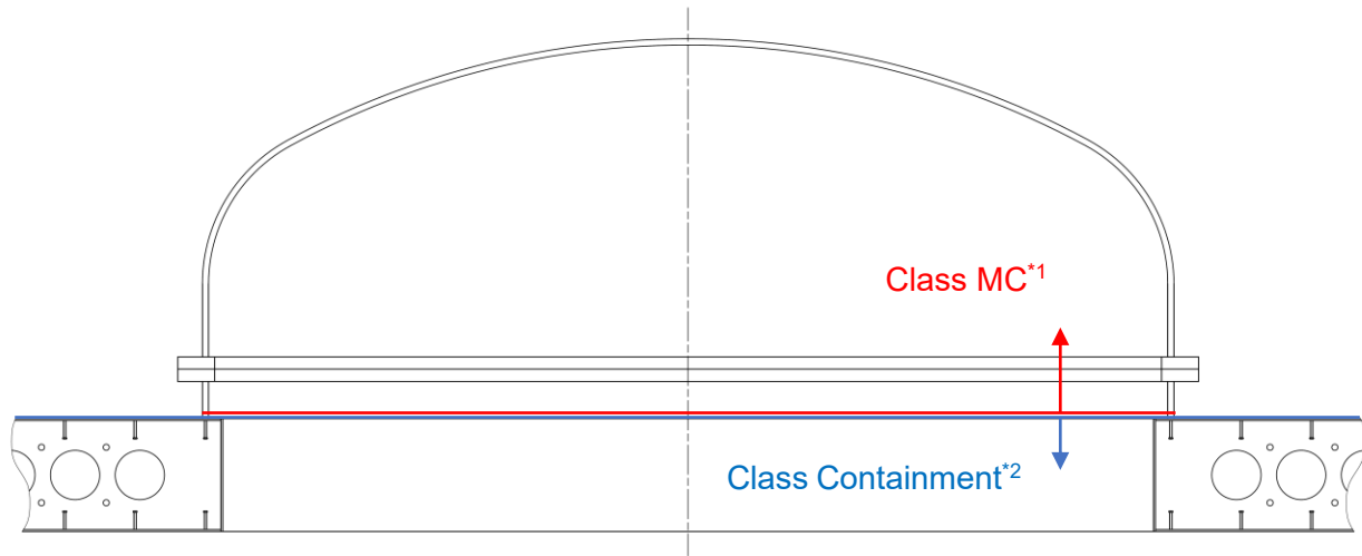
Figure 3.8-3: Containment Closure Head Structure Boundary
