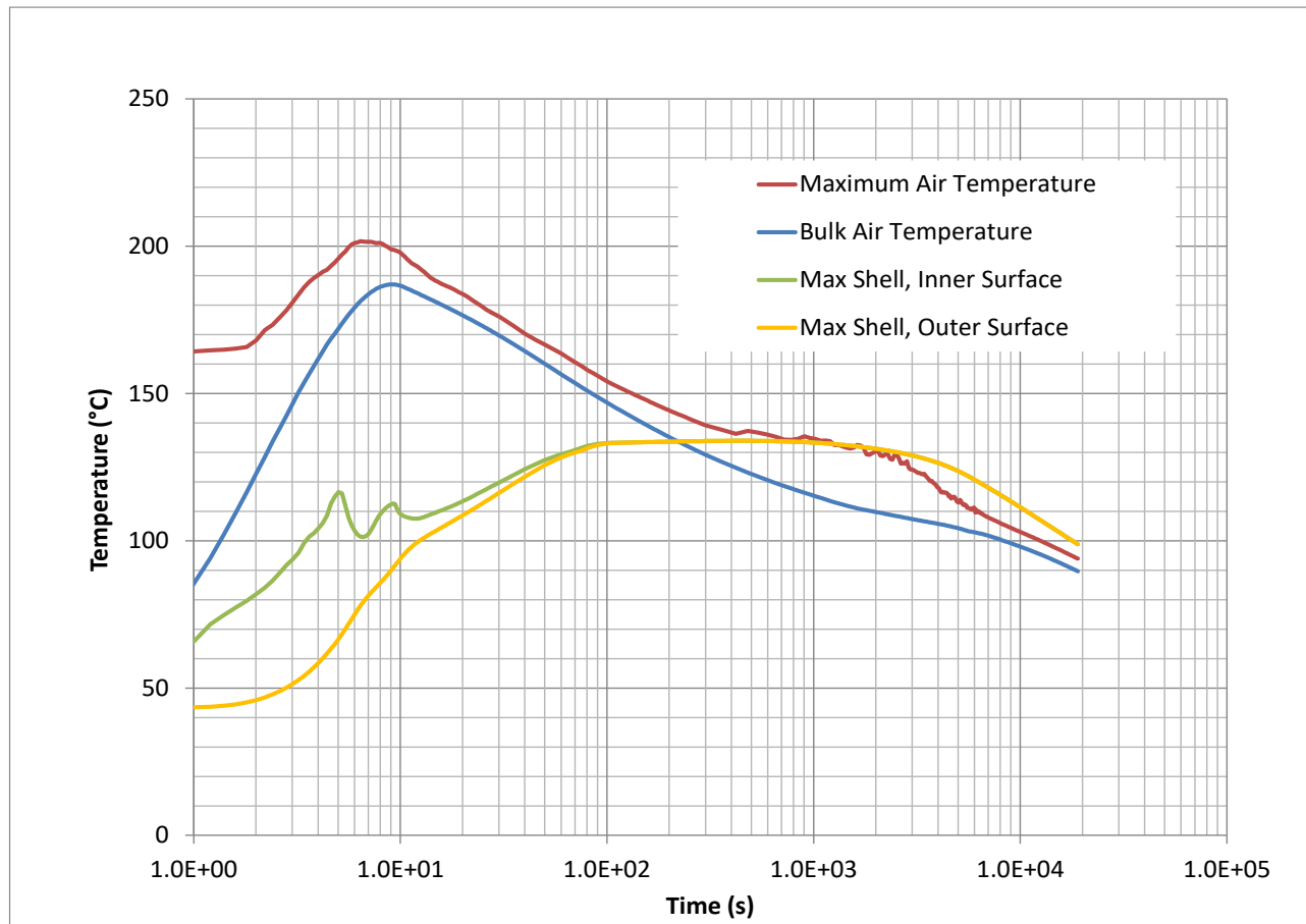
Figure 15.5-166: Containment Temperature, Large FW Pipe Break, Conservative Case
