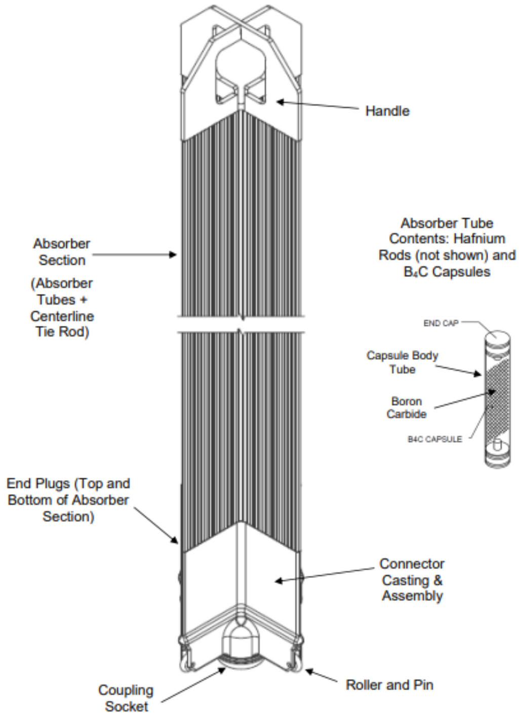
Figure 4.2-4: BWRX-300 Control Rod
