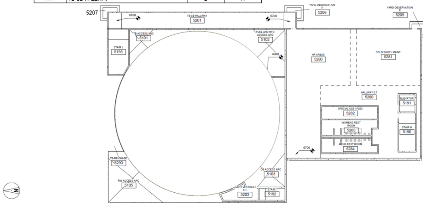
Figure 12.3-18: Service Building Level 6.1/6.7 Meters Radiation Zones
