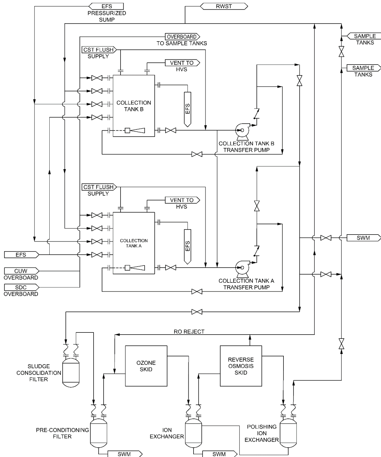
Figure 11.2-1: Waste Collection and Filtering Subsystem Simplified Diagram
