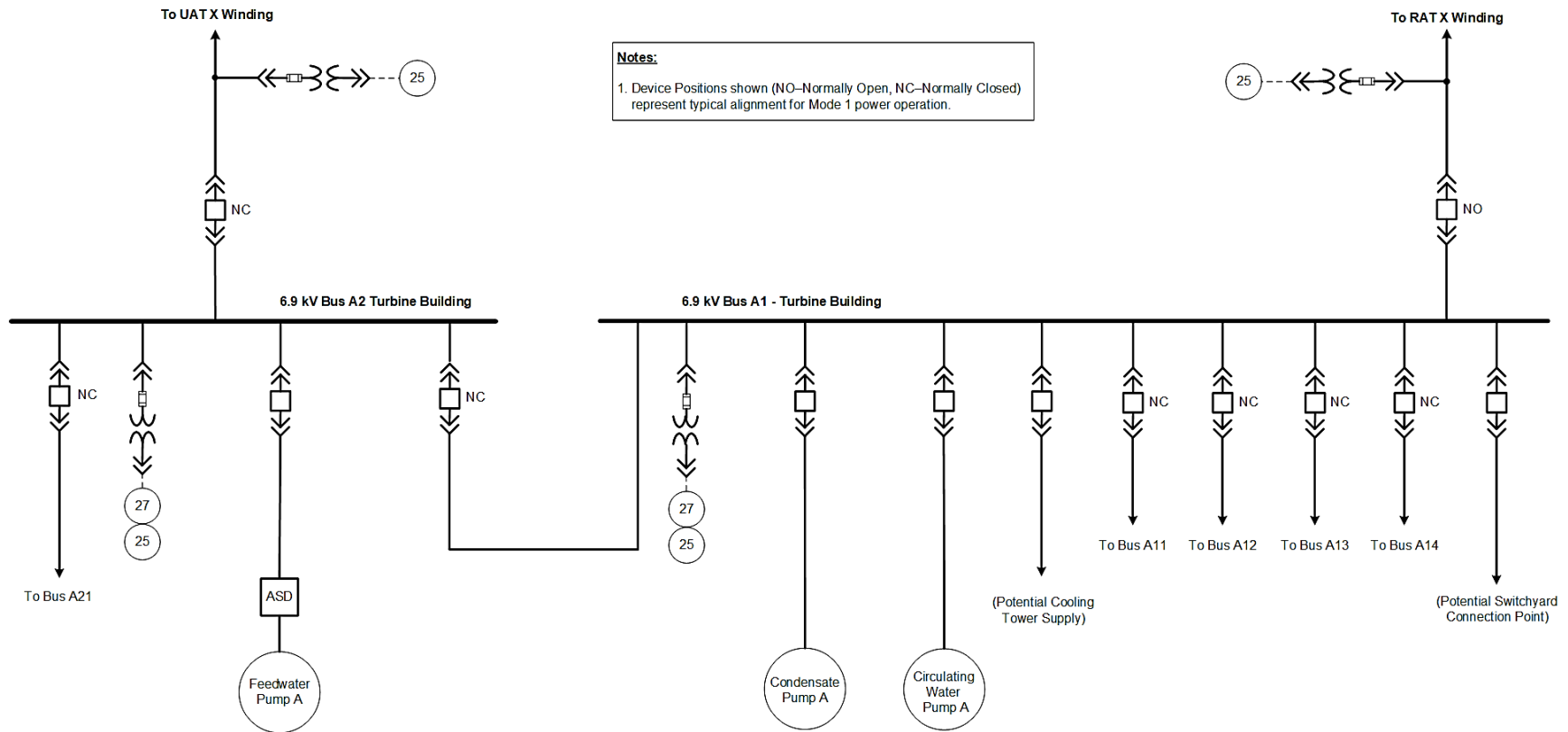
Figure 8.3-1: Preferred Power Medium Voltage Bus A Train
