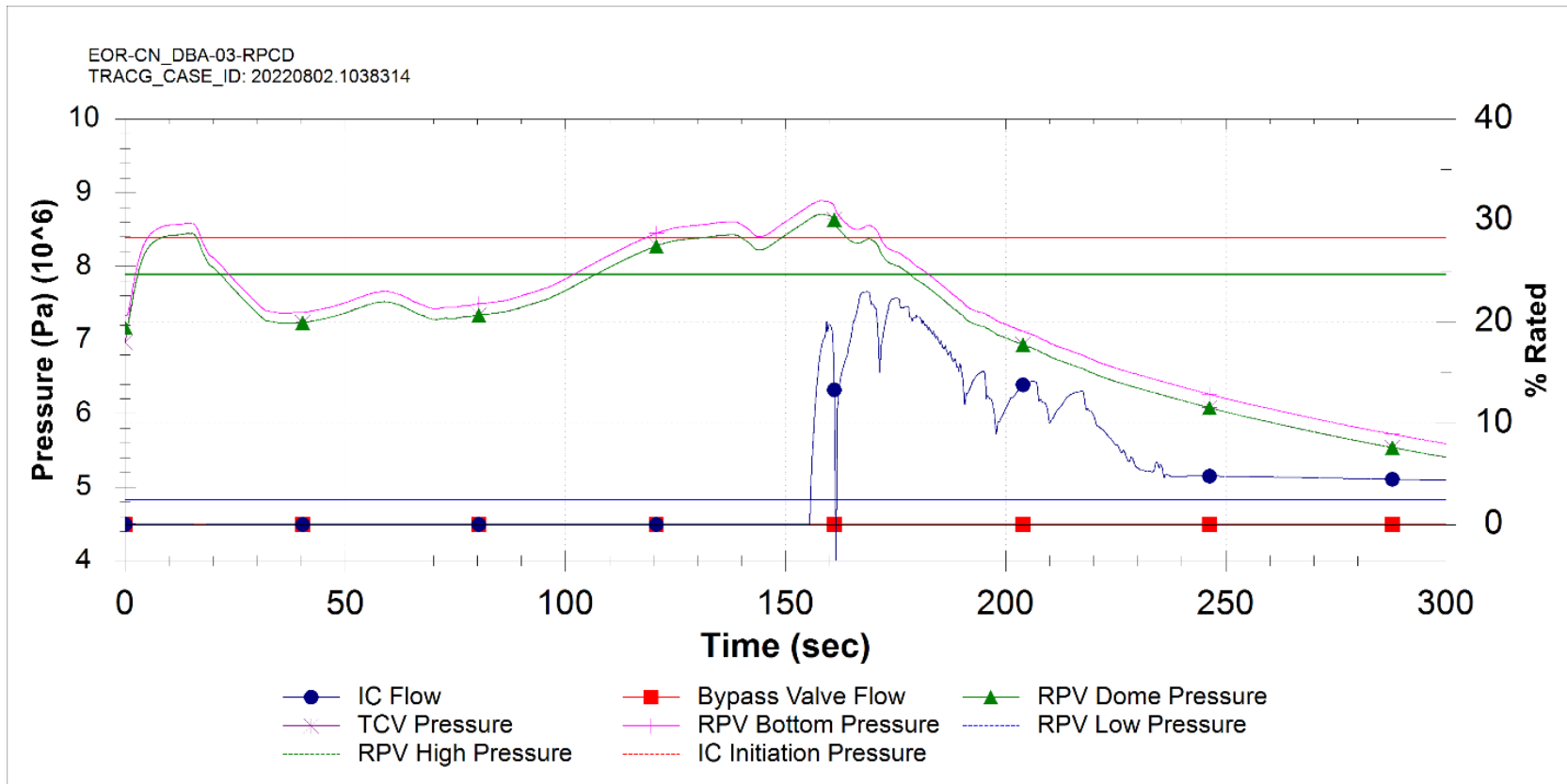
Figure 15.5-65: RPV Pressure Control Downscale (DBA)
