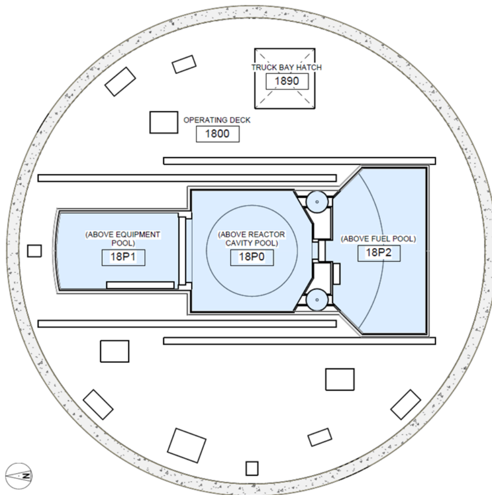
Figure 12.3-9: Reactor Building Level 13.0 Meters Radiation Zones
