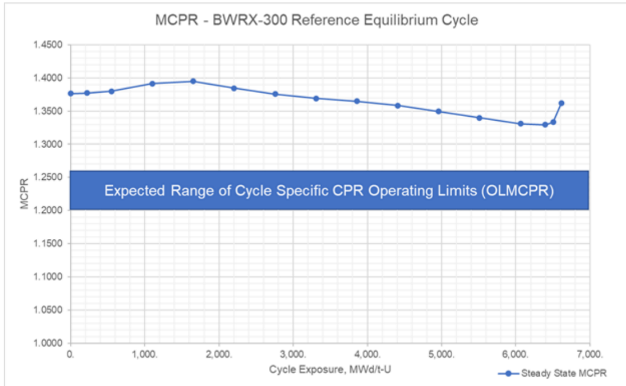
Figure 4.3-6: MCPR vs. Cycle Exposure for the Reference Equilibrium Cycle
