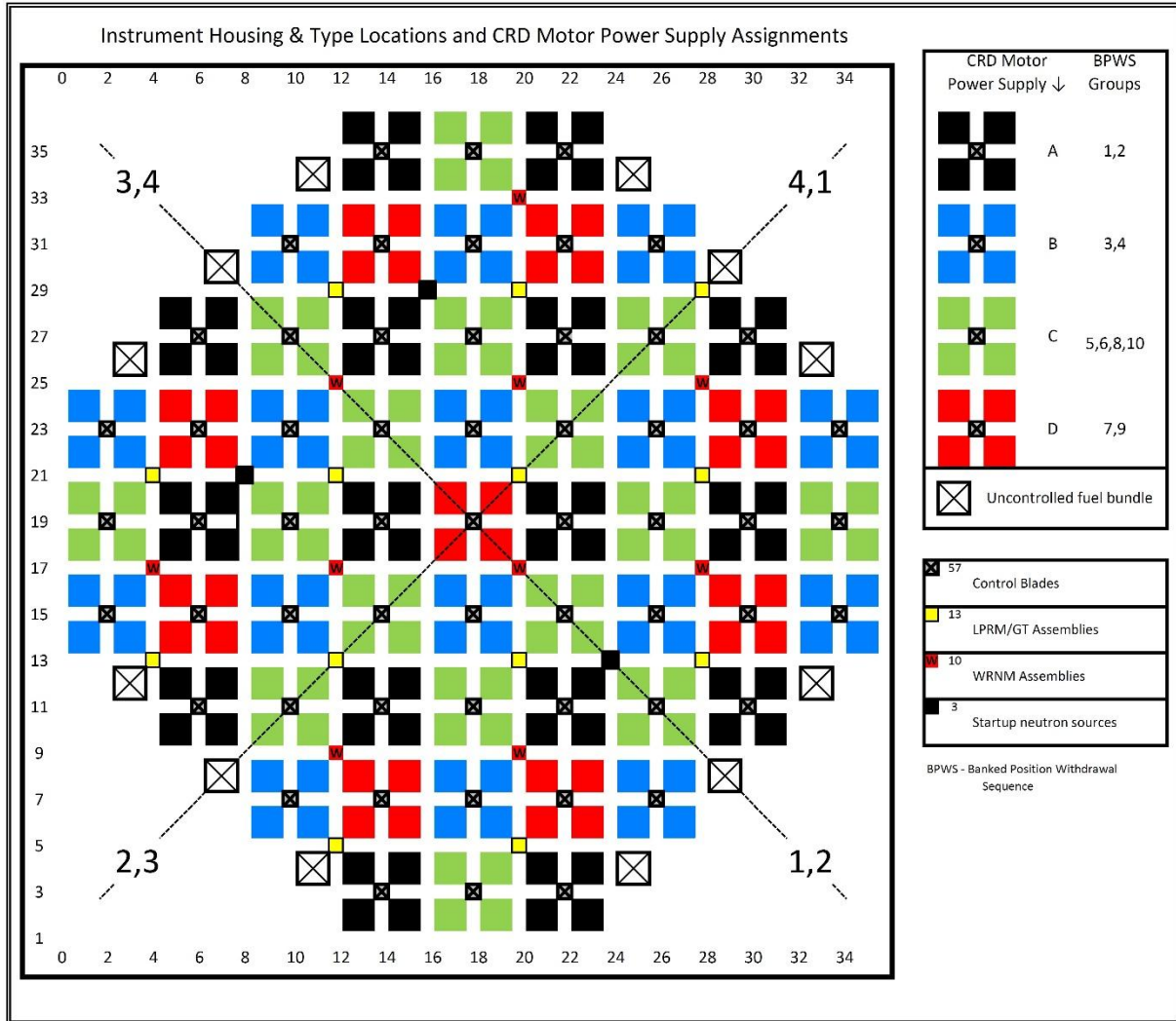
Figure 7.3-6: BWRX-300 Core Map with Monitoring Locations and Fine Motion Control Rod Drive Power Assignments
