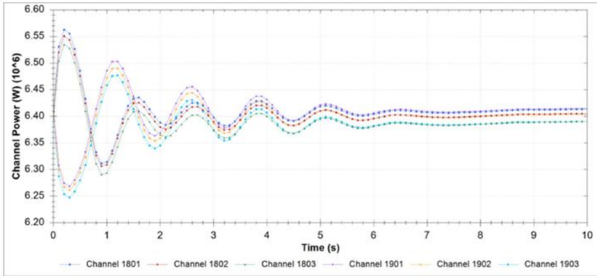
Figure 15.5-3: Regional Mode Stability Response at 115% Power
