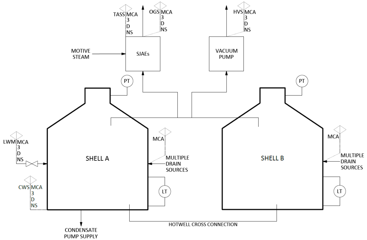
Figure 10.4-1: Main Condenser and Auxiliaries Simplified Diagram
