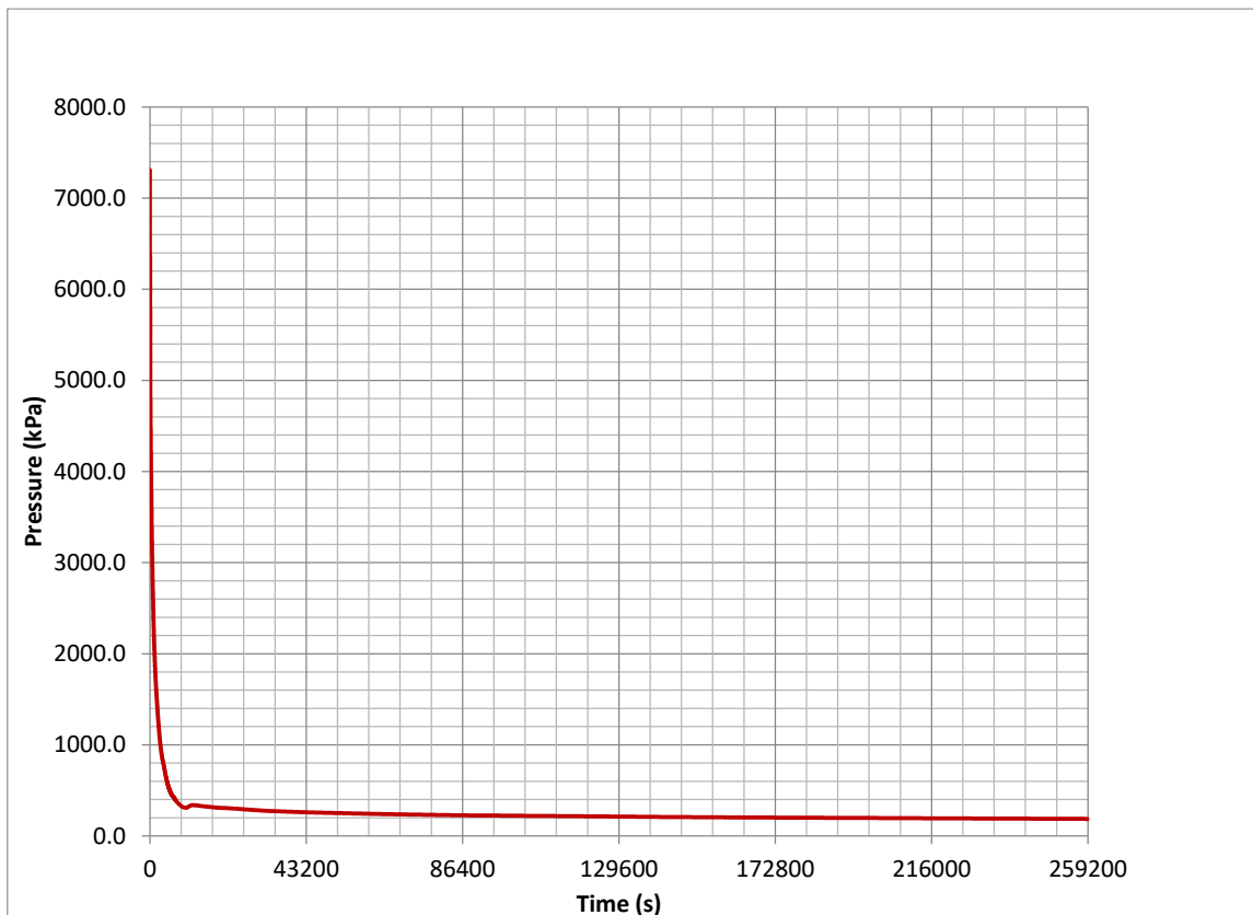
Figure 15.5-113: Reactor Pressure, Small Liquid Pipe Break, Conservative Case
