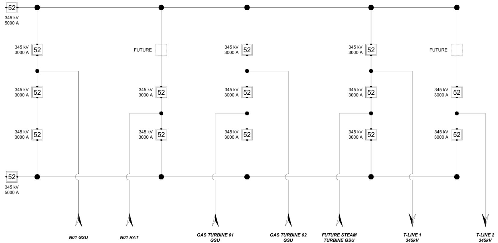
Figure 8.1-2: Preliminary BECPV-N01 Switchyard Interface
