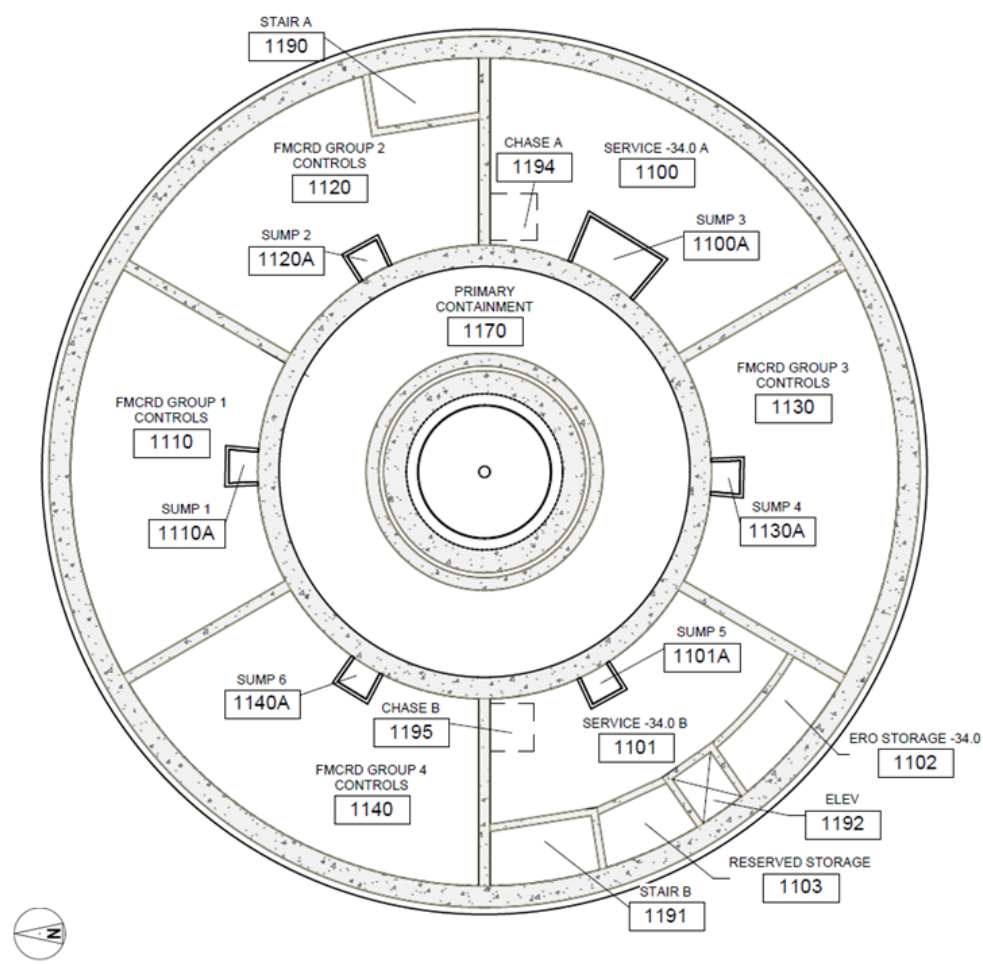
Figure 12.3-1: Reactor Building Level -34.0 Meters Radiation Zones
