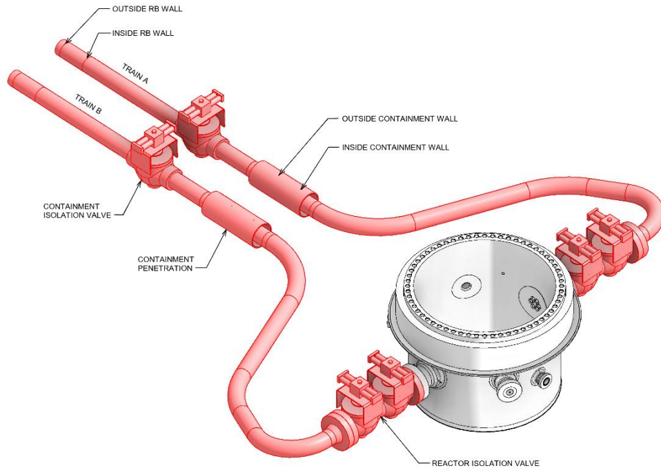
Figure 5.4-5: Main Steam System
