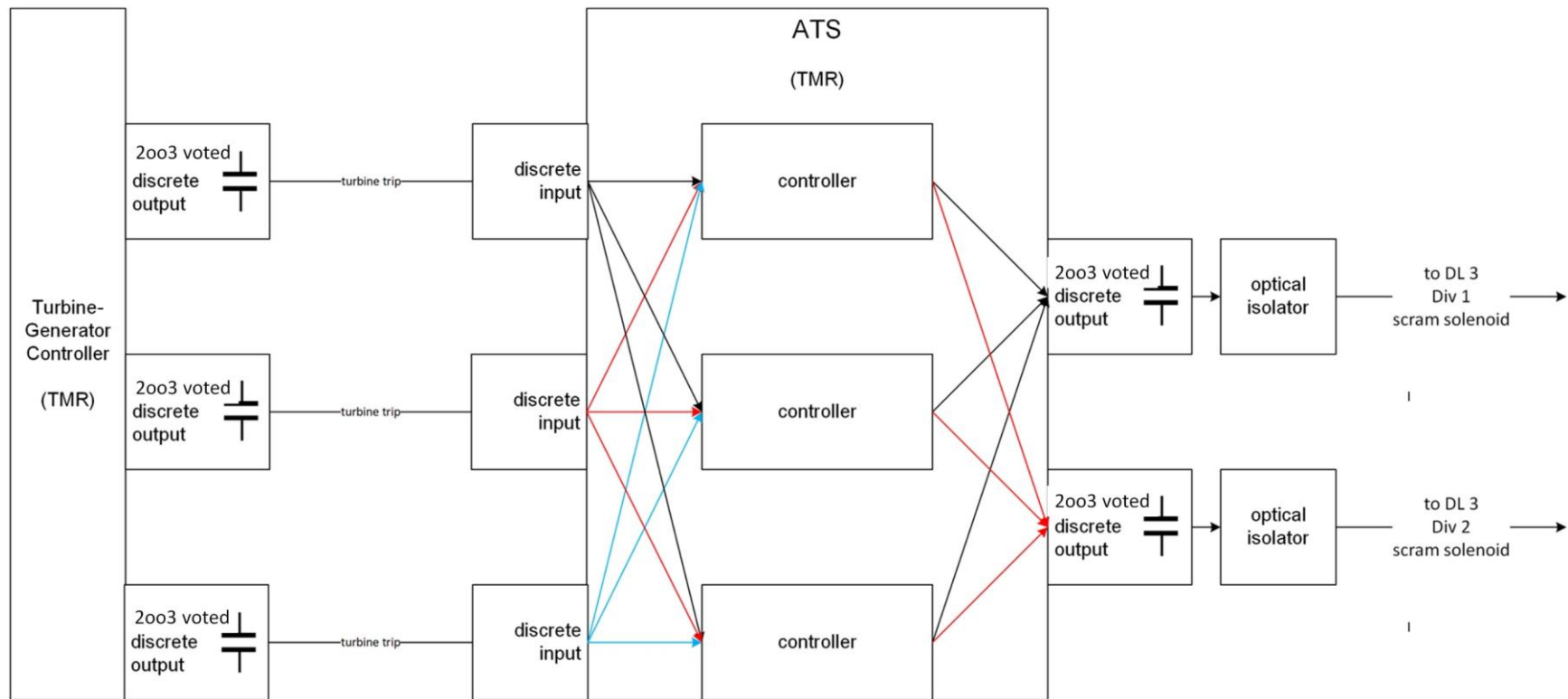
Figure 7.3-12: Representative Anticipatory Trip System Scram Block Diagram
