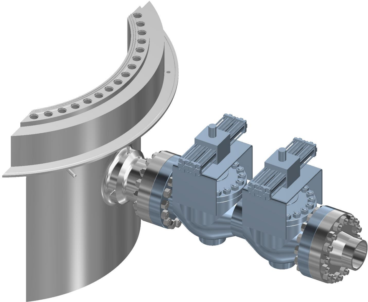
Figure 5.4-1: BWRX-300 Reactor Pressure Vessel Reactor Isolation Valve
