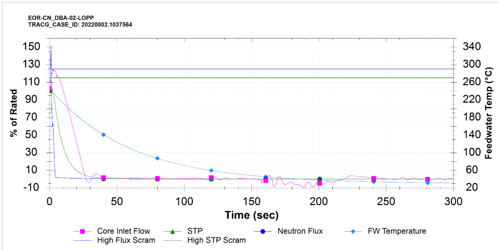
Figure 15.5-58: Loss of Preferred Power (DBA)
