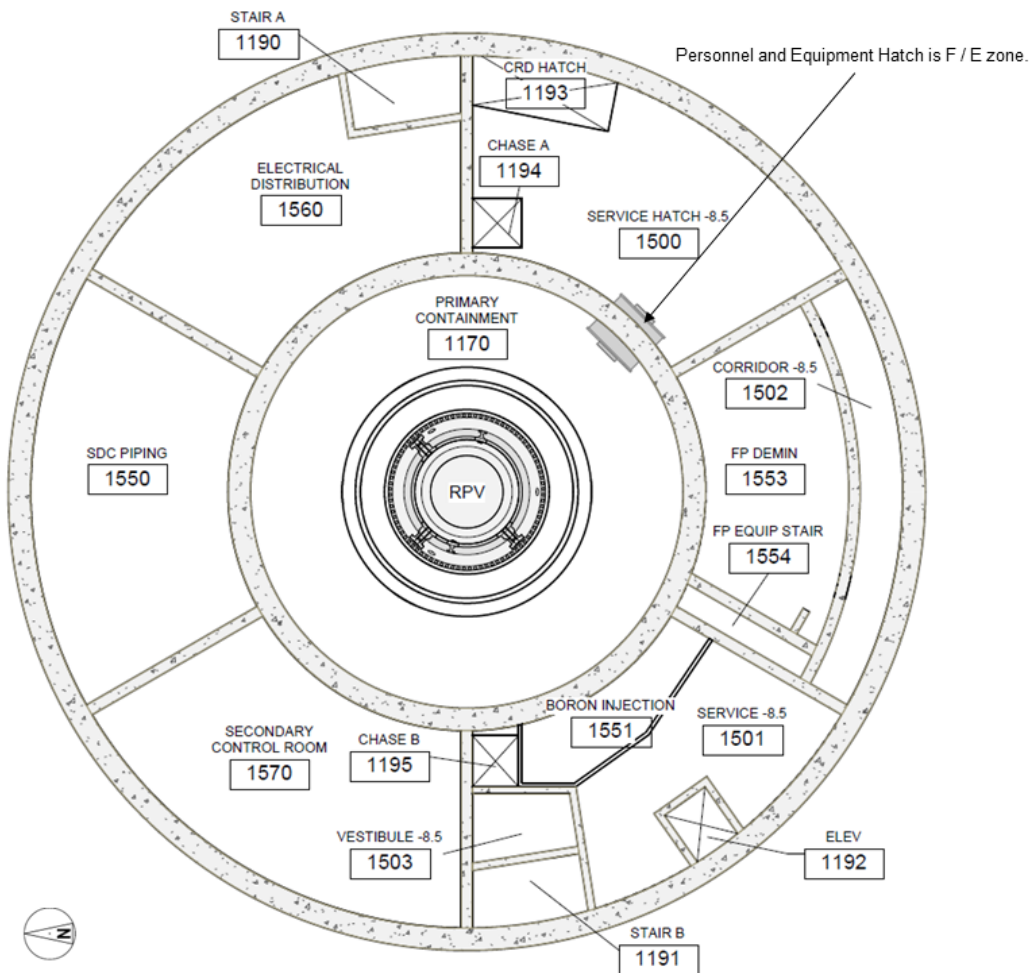
Figure 12.3-5: Reactor Building Level -8.5 Meters Radiation Zones
