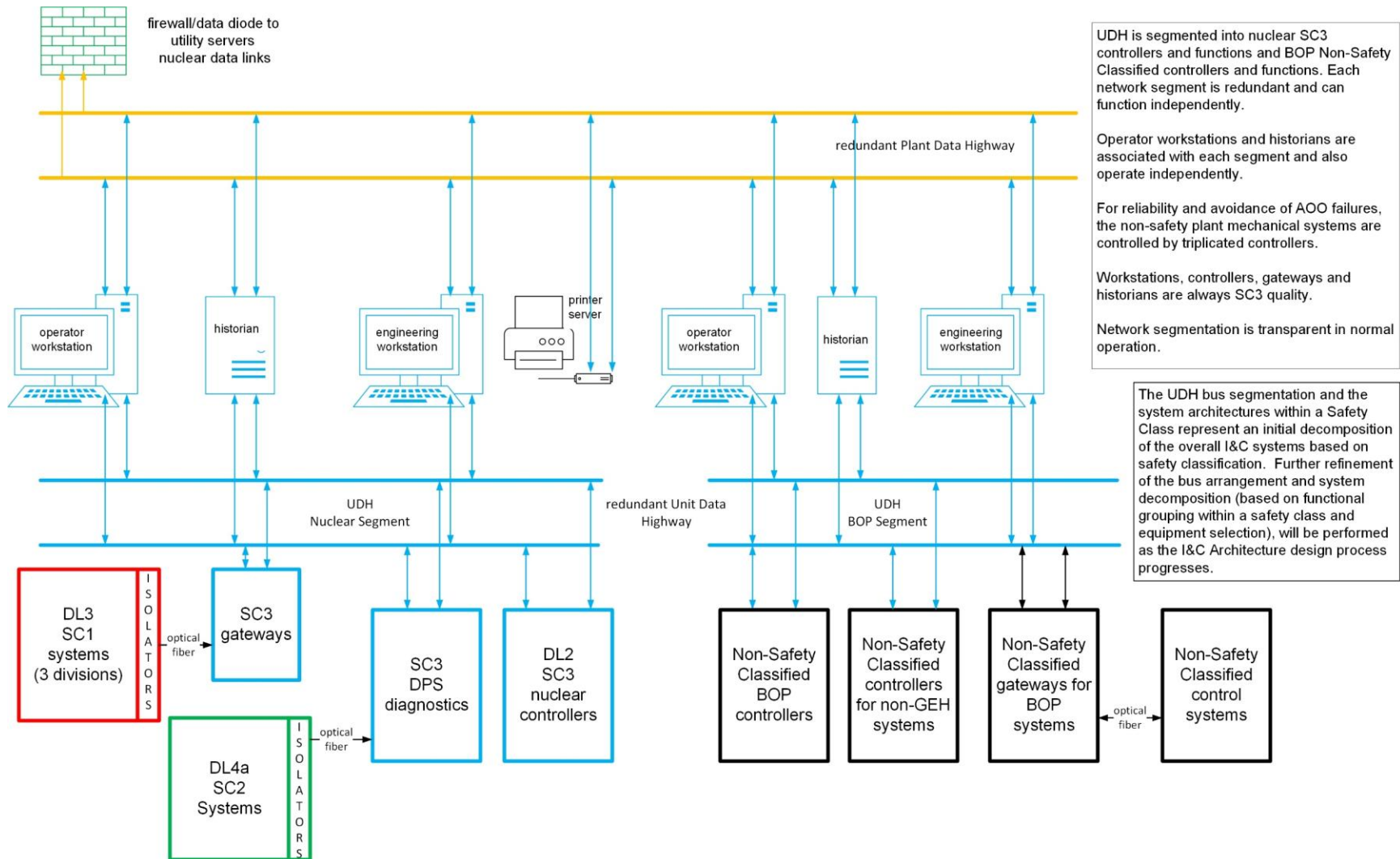
Figure 7.2-1: BWRX-300 Distributed Control and Information System Network Architecture
