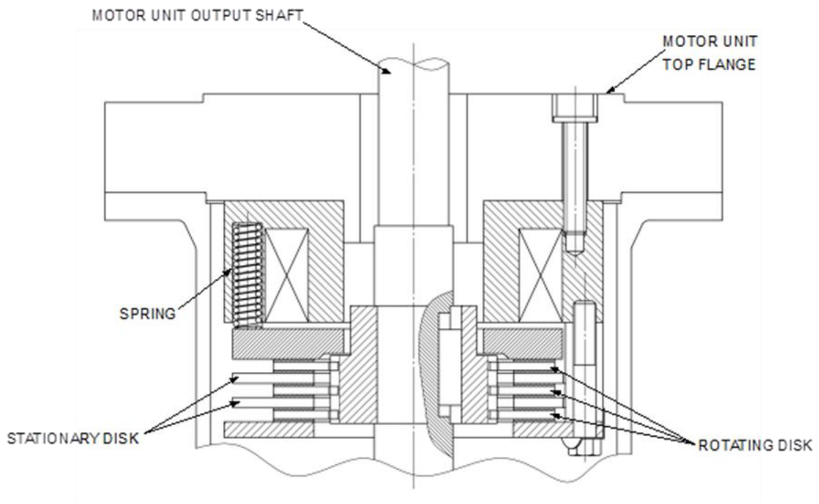
Figure 4.6-7: Representative Fine Motion Control Rod Drive Electro-Mechanical Brake
