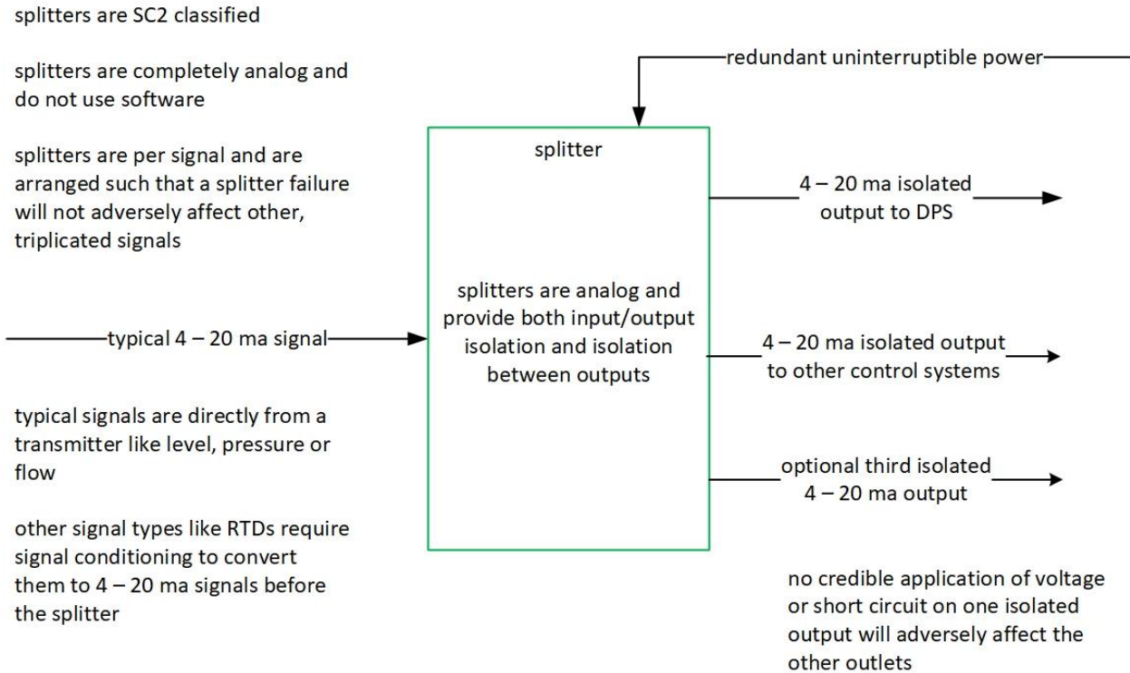
Figure 7.3-9: Safety Class 2 Analog Signal Splitters
