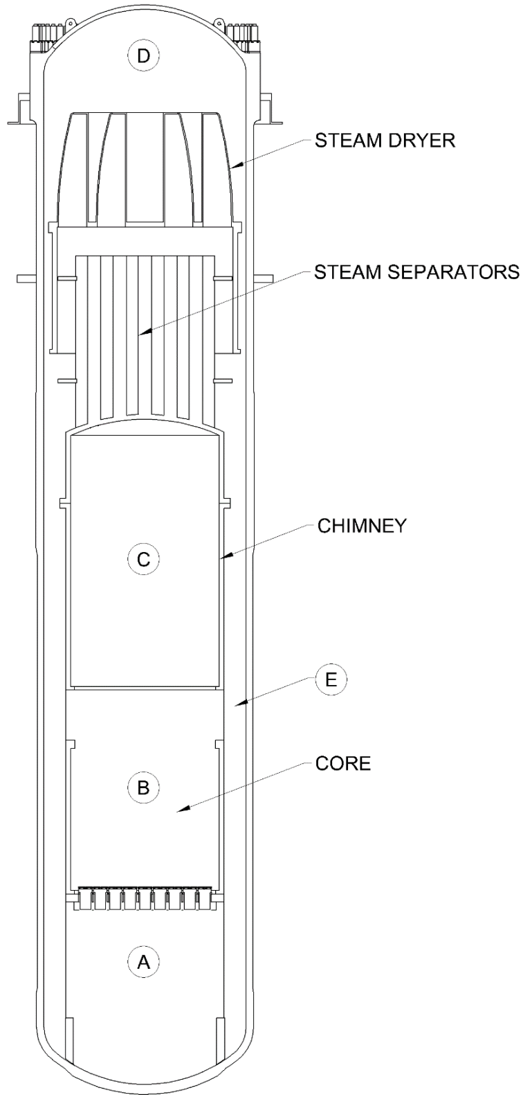
Figure 5.1-4: BWRX-300 Reactor Pressure Vessel Volumes at 100% Power
