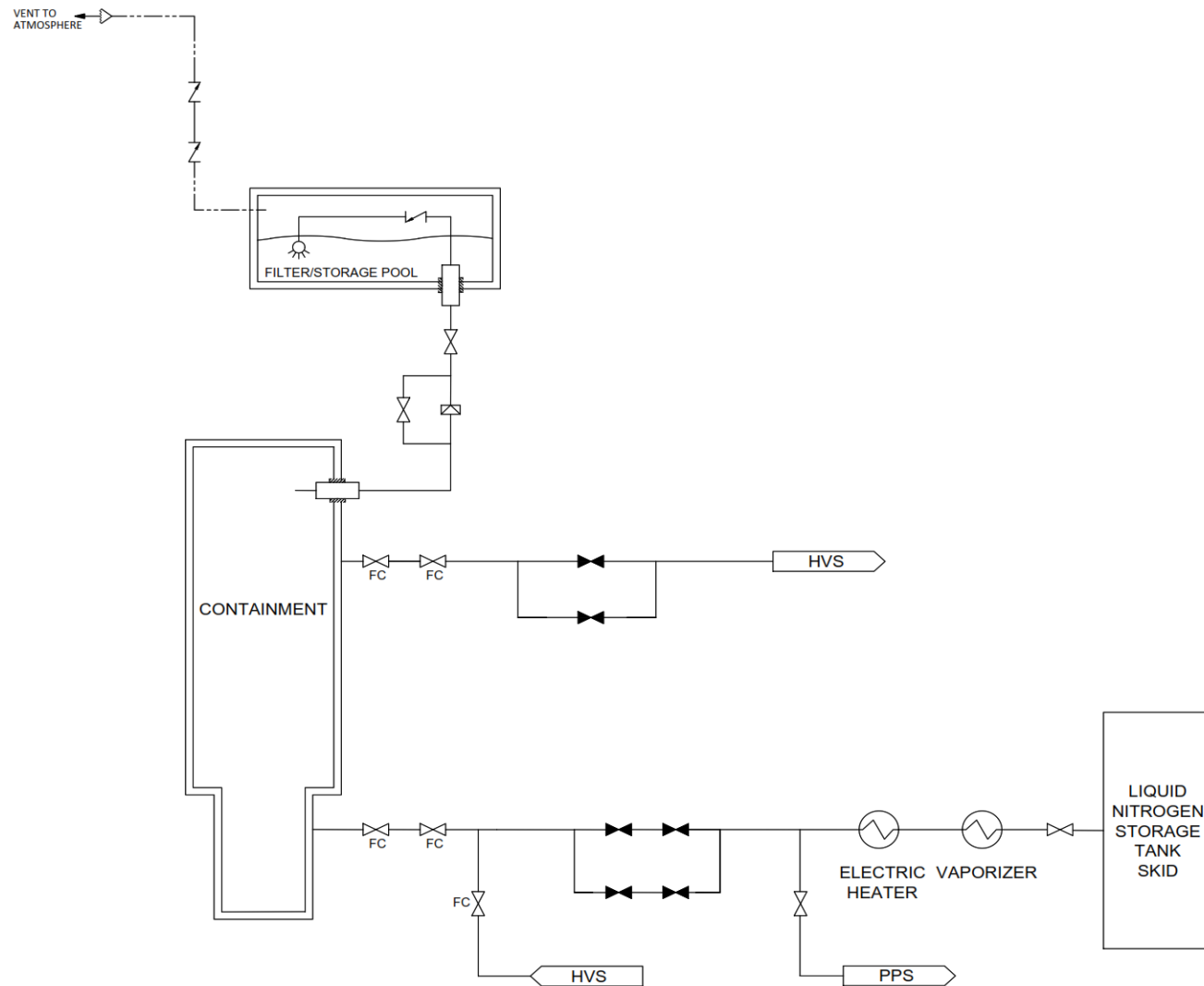
Figure 9.3-5: Containment Inerting System Simplified Diagram
