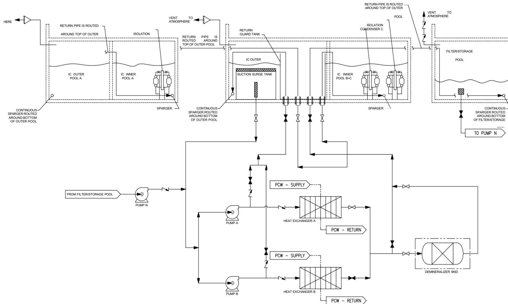
Figure 9.2-6: Isolation Condenser Pools Cooling and Cleanup System Simplified Diagram
