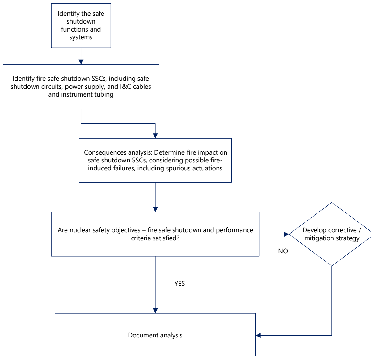
Figure 9A-1: BWRX-300 Fire Safe Shutdown Analysis Methodology
