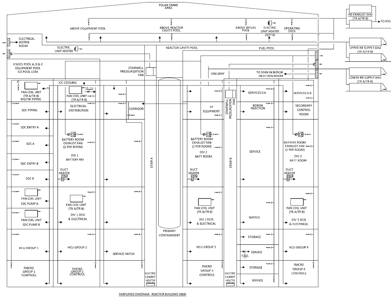
Figure 9.4-4: Reactor Building Heating, Ventilation, and Cooling Simplified Diagram
