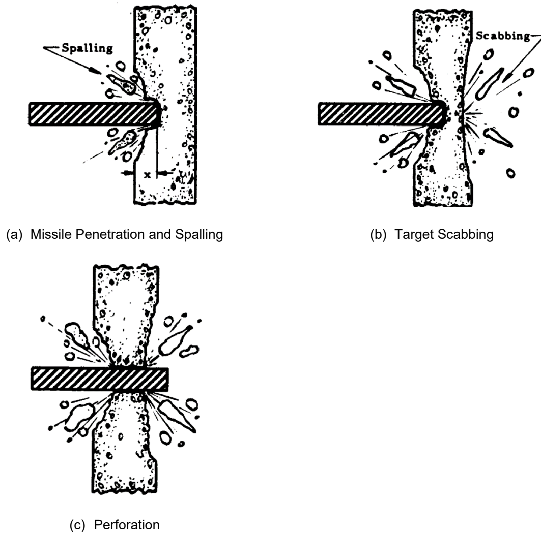
Figure 3.5-1: BWRX-300 Missile Impact Local Damage Modes for the Concrete Barrier
