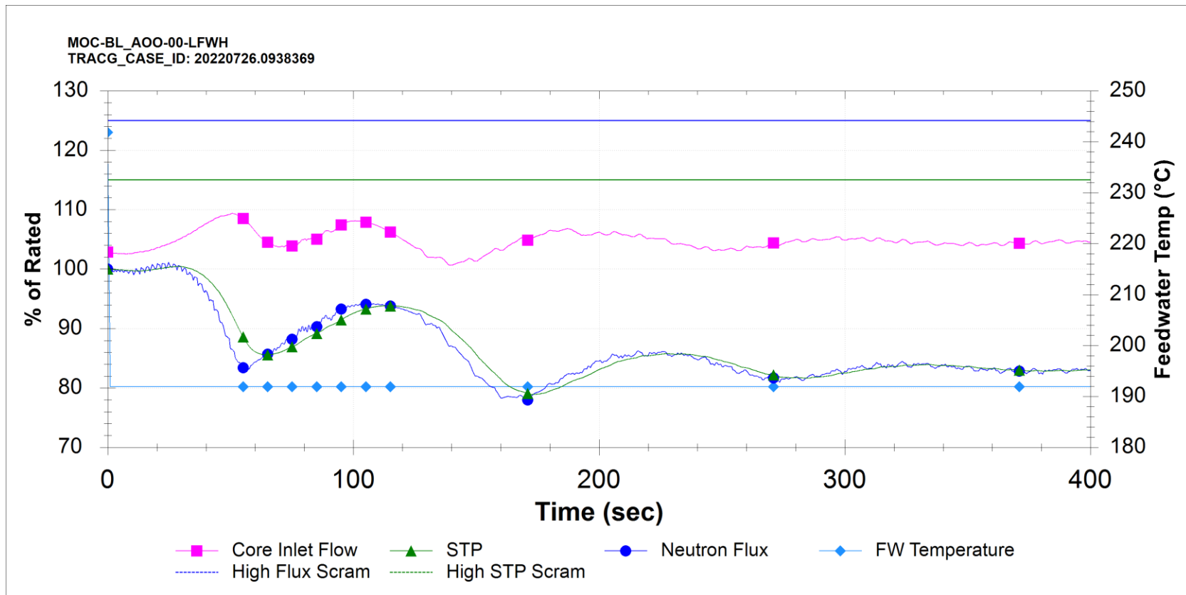
Figure 15.5-4: Loss of Feedwater Heating (AOO)
