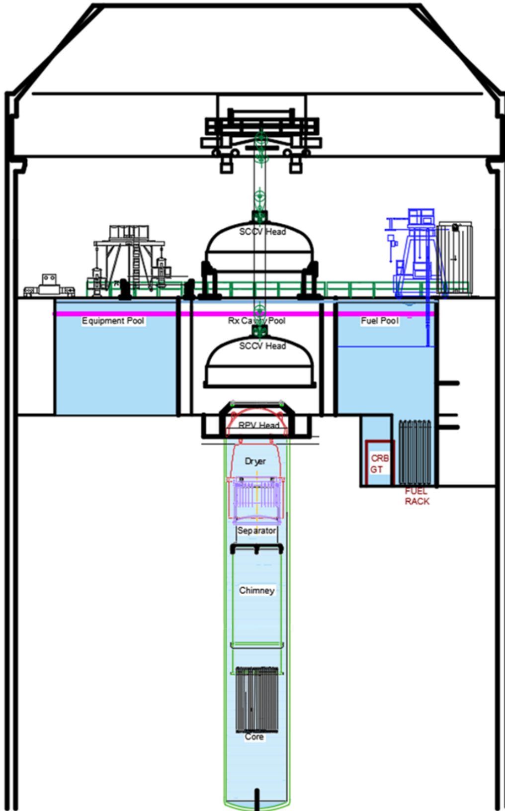
Figure 9.1-5: Containment Closure Head Removal
