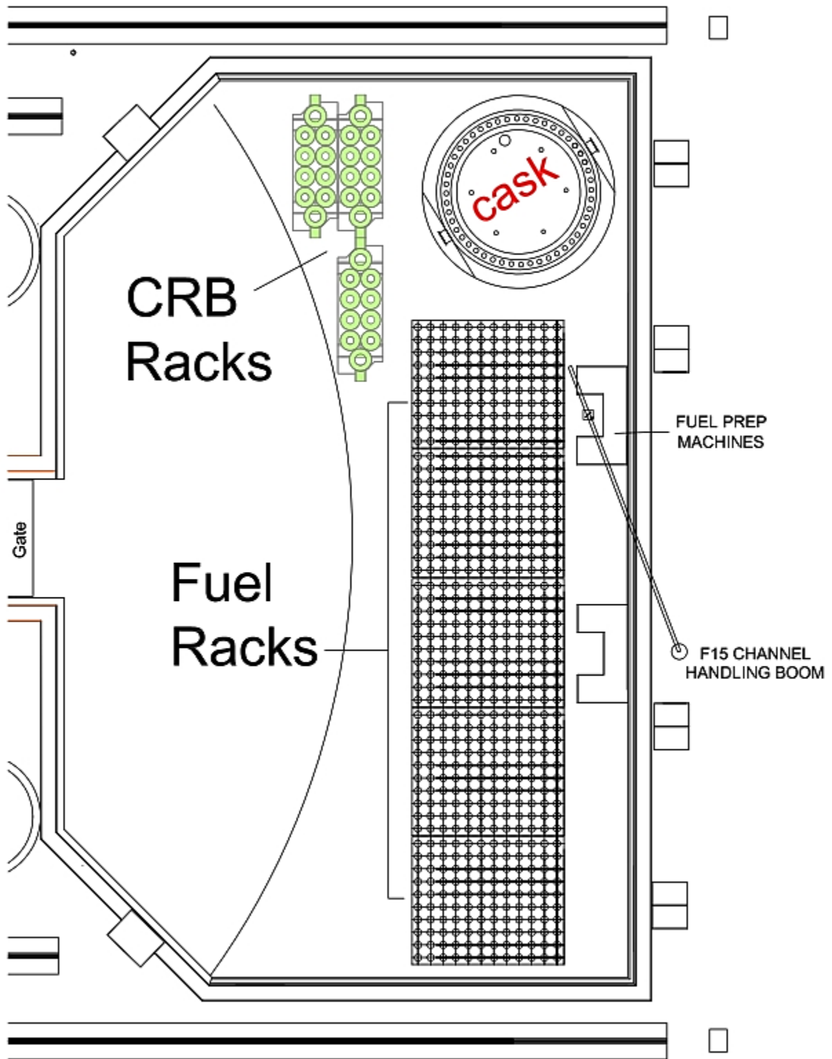
Figure 9.1-2: Fuel Pool Arrangement
