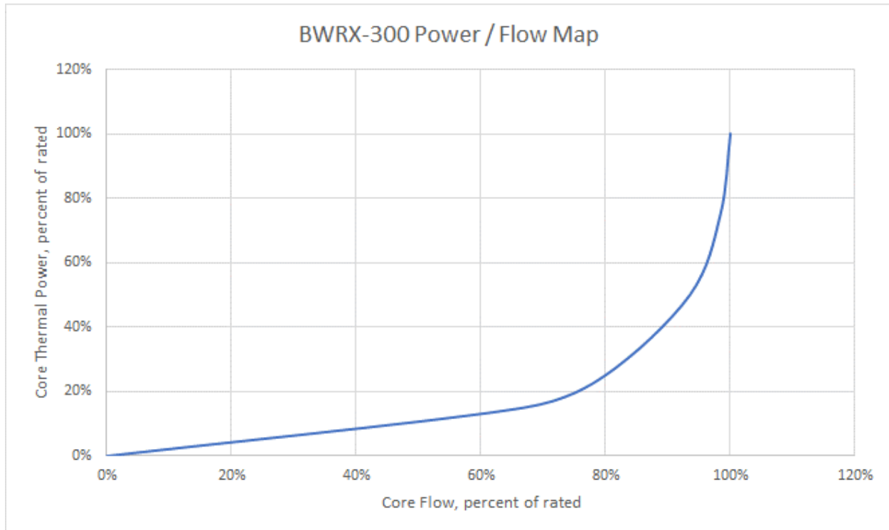
Figure 4.4-1: BWRX-300 Power / Flow Map
