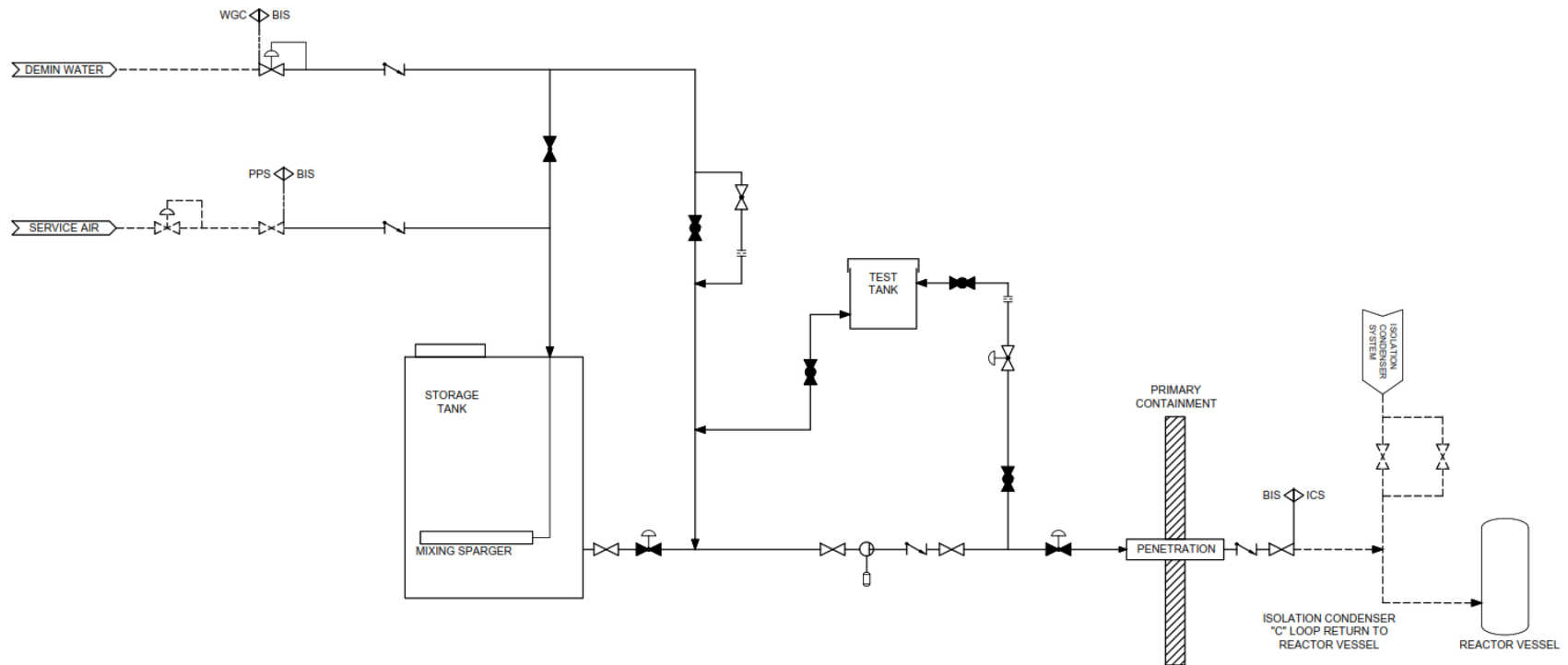
Figure 9.3-6: Boron Injection System Simplified Diagram
