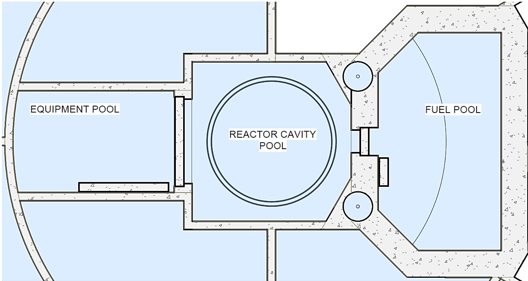
Figure 9.1-1: Arrangement of Fuel, Reactor Cavity and Equipment Pools
