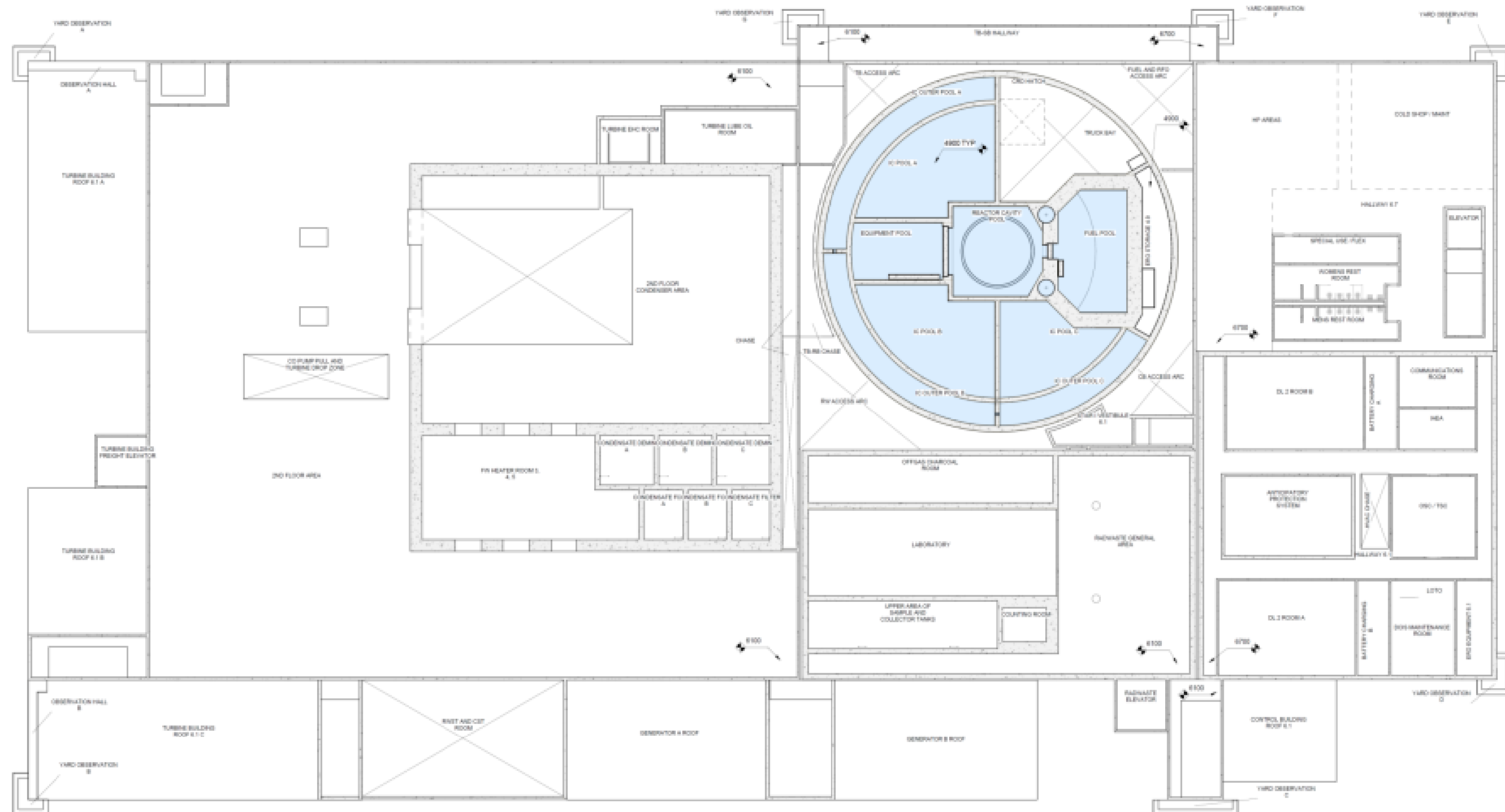
Figure 1.2-4: BWRX-300 Plan View Elevation 4.9m/6.1m/6.7m
