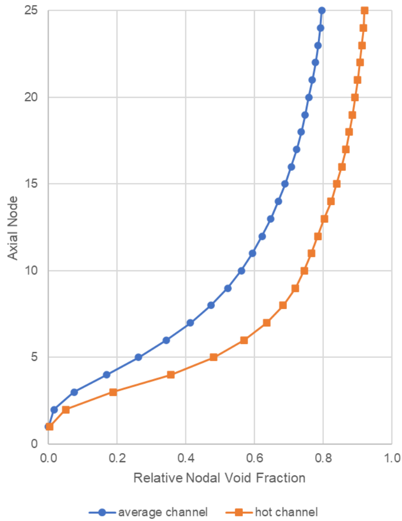
Figure 4.4-2: Relative Void Fraction for Analyzed Node (Hot Channel and Average Channel)
