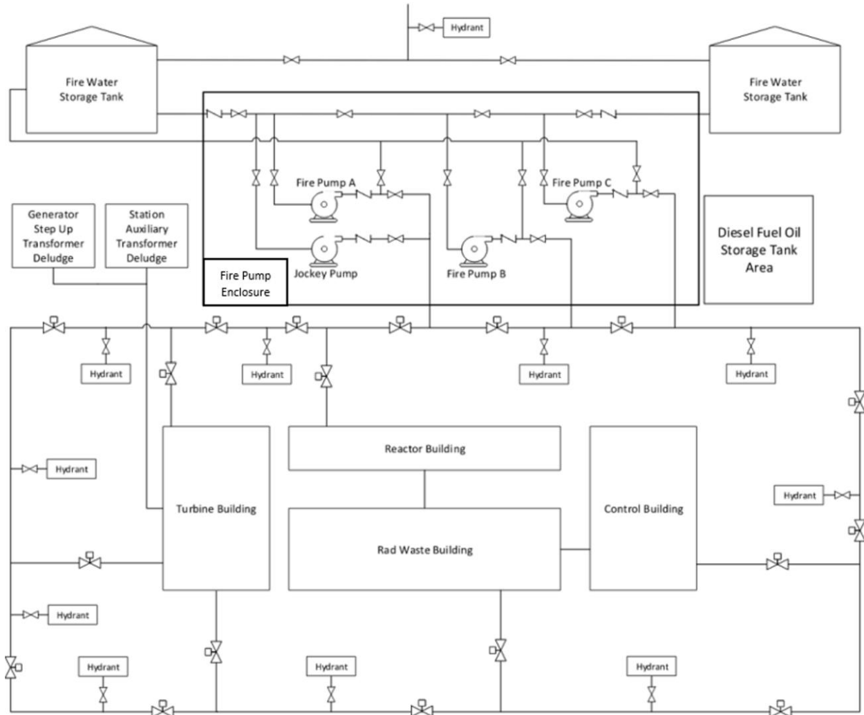
Figure 9.5-1: BWRX-300 Fire Protection System Schematic
