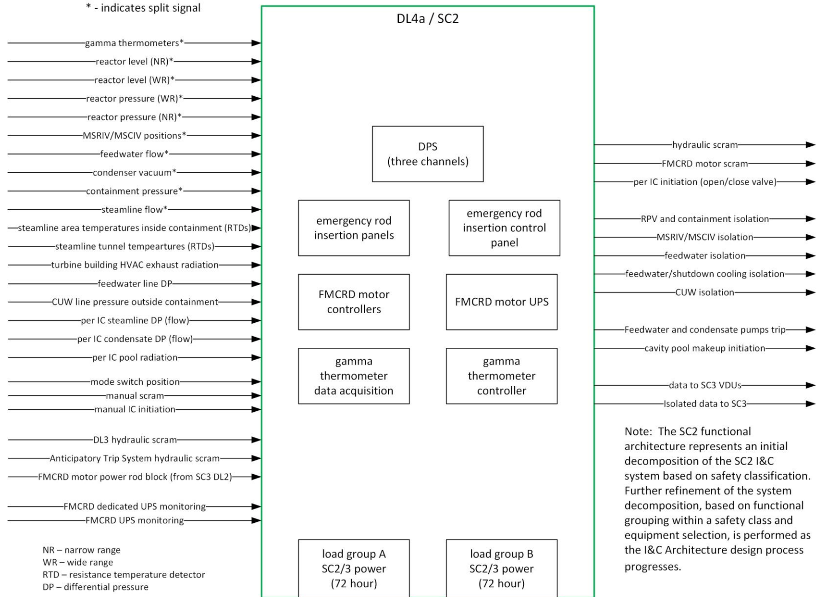
Figure 7.3-8: Safety Class 2 Functional Architecture
