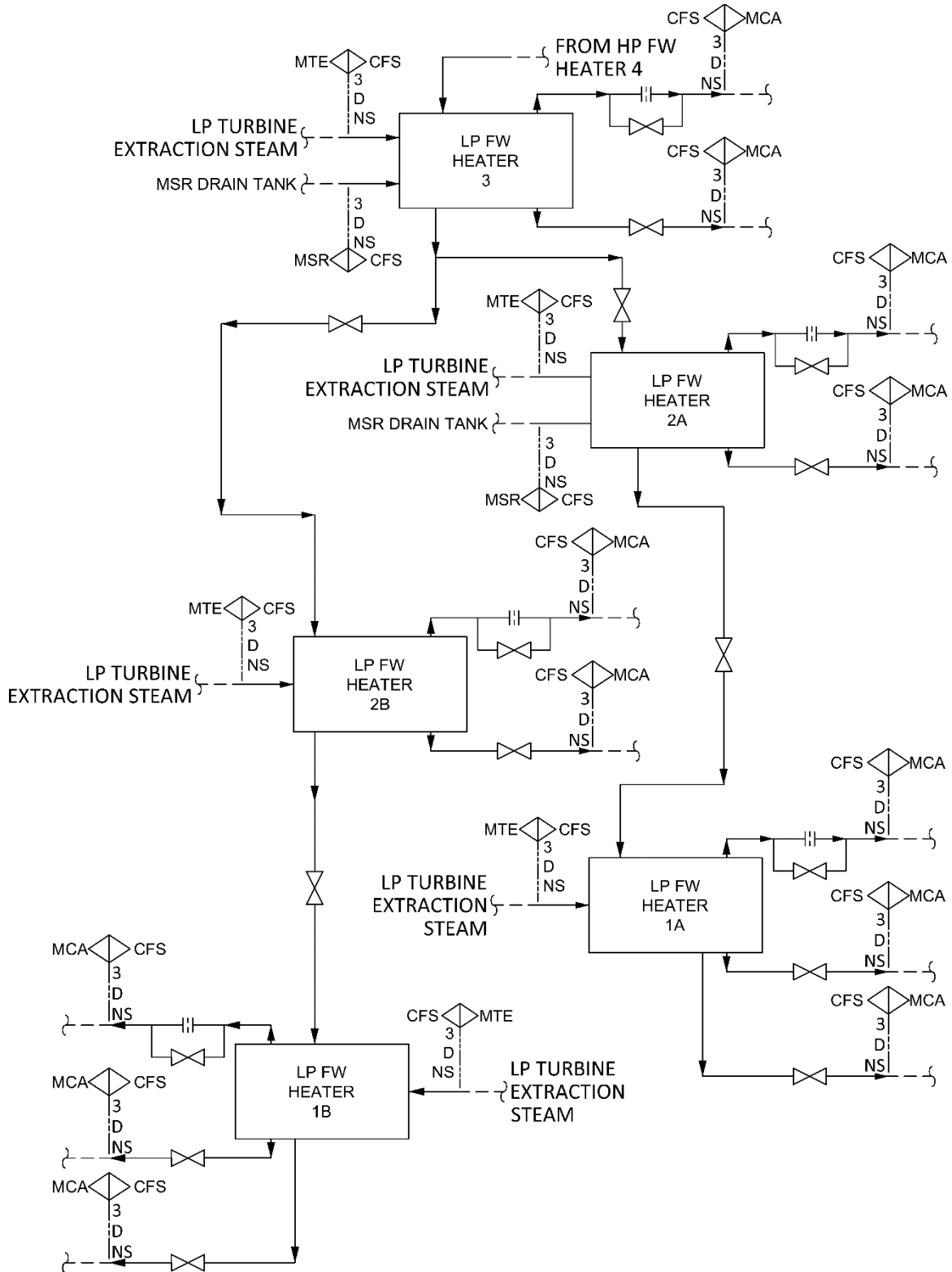
Figure 10.4-10: CFS LP Heaters and Drains Simplified Diagram
