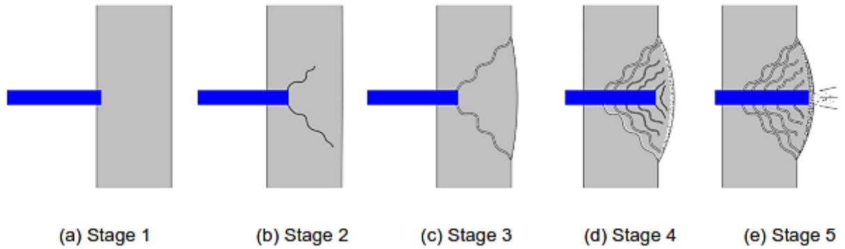
Figure 3.5-2: BWRX-300 Missile Impact Local Damage Modes for the Steel-Plate Composite Barrier
