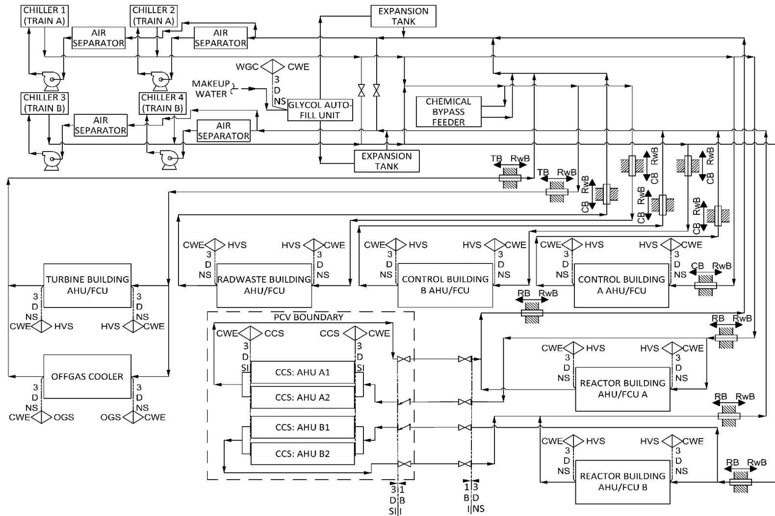
Figure 9.2-5: Chilled Water Equipment Simplified Diagram
