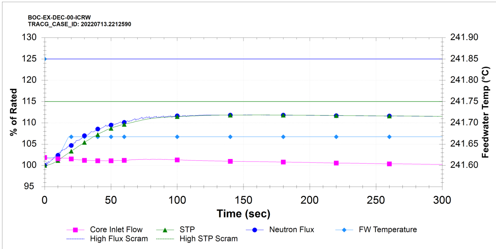
Figure 15.5-149: Inadvertent Control Rod Withdrawal at Power - Single Rod (ICRW)
