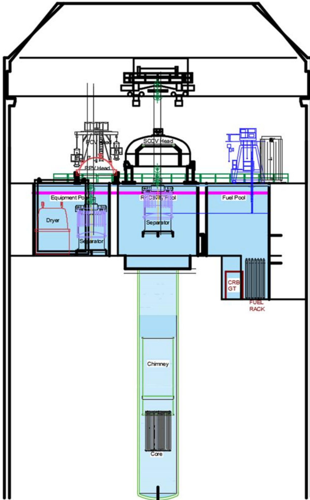
Figure 9.1-8: Chimney Head and Steam Separator Assembly Removal
