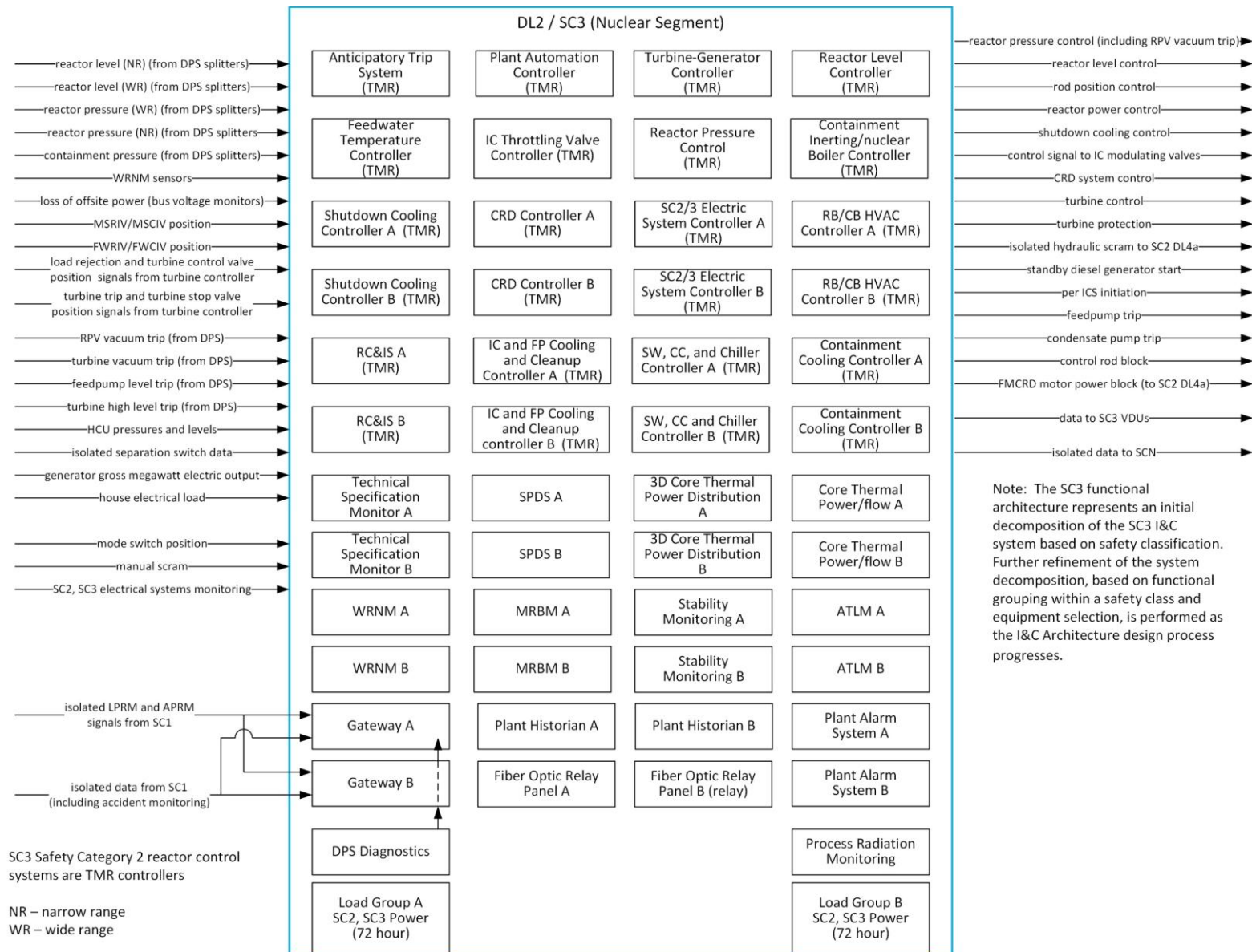
Figure 7.3-11: Safety Class 3 Nuclear Segment Functional Architecture
