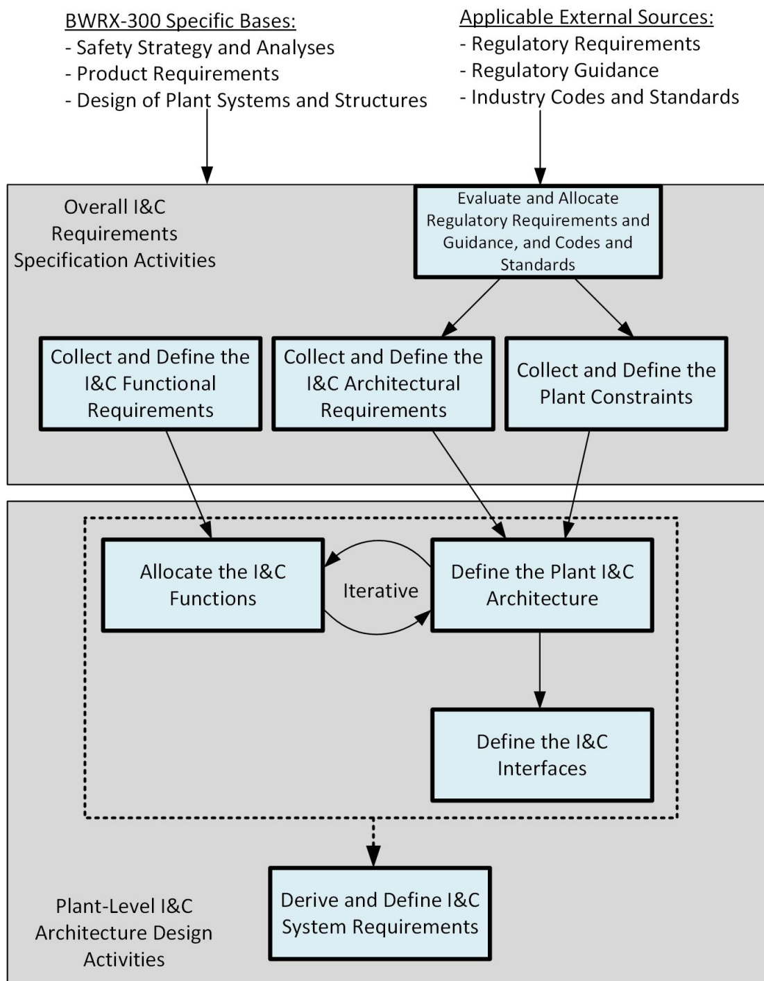
Figure 7.4-1: BWRX-300 Instrumentation and Control Architecture Design Process
