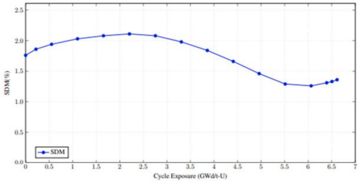
Figure 4.3-8: Shutdown Margin vs Cycle Exposure
