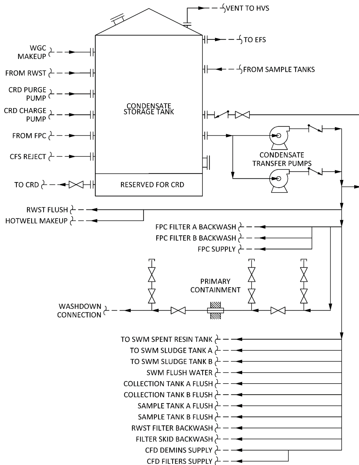
Figure 9.2-4: Condensate Storage and Transfer Subsystem Simplified Diagram
