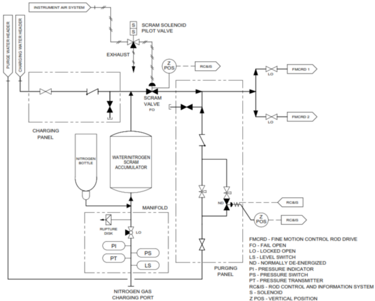
Figure 4.6-8: Hydraulic Control Unit Simplified Piping and Instrumentation Diagram
