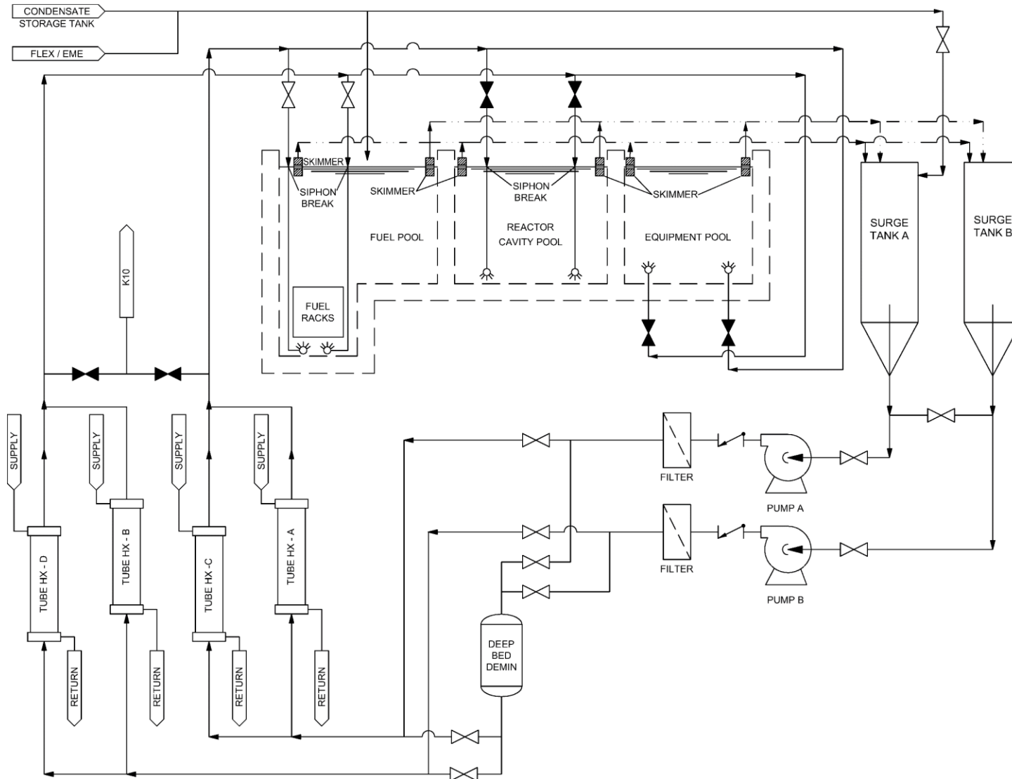
Figure 9.1-3: Fuel Pool Cooling System
