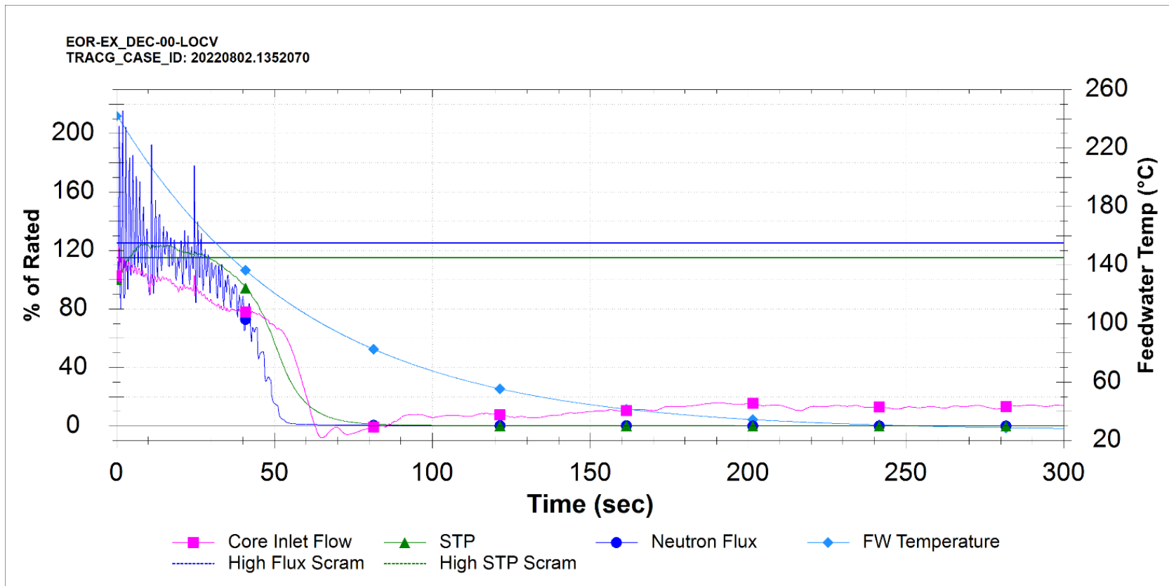
Figure 15.5-131: Loss of Condenser Vacuum (DEC)
