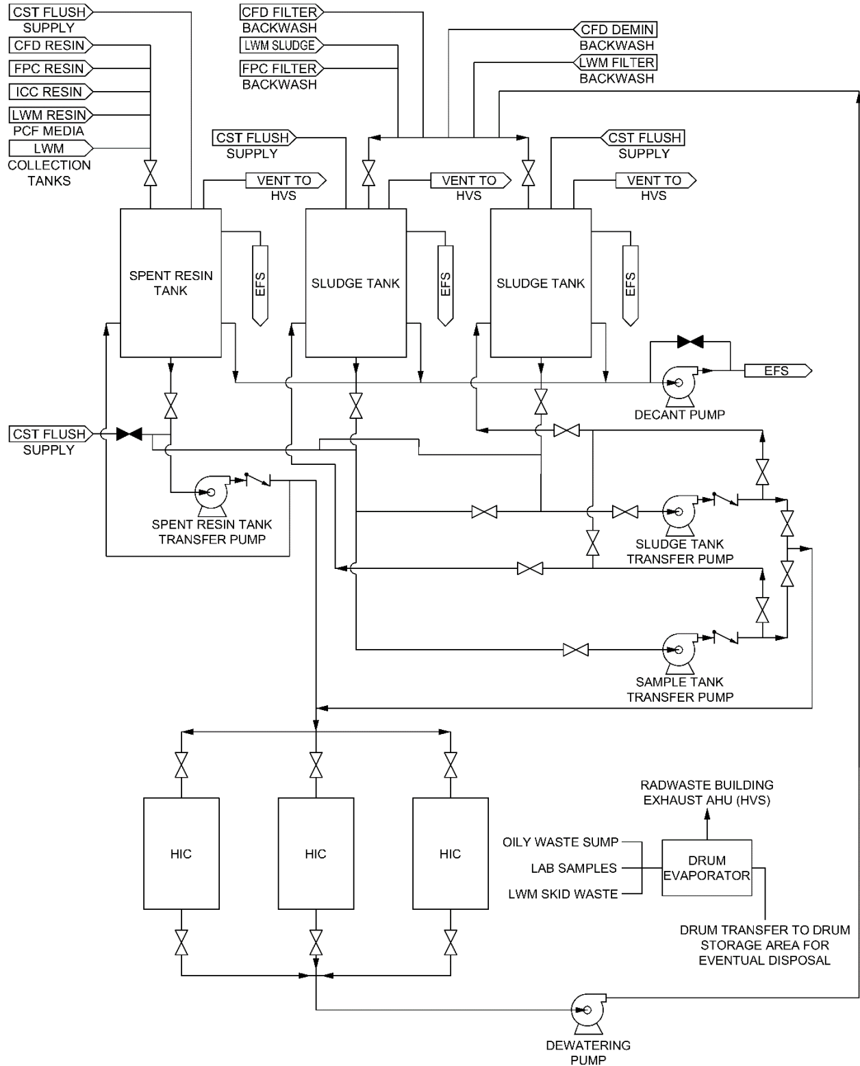
Figure 11.4-1: Solid Waste Management System Simplified Diagram
