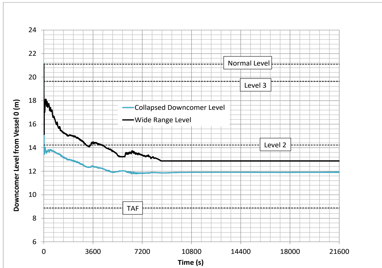
Figure 15.5-163: Reactor Water Level, Large FW Pipe Break, Conservative Case
