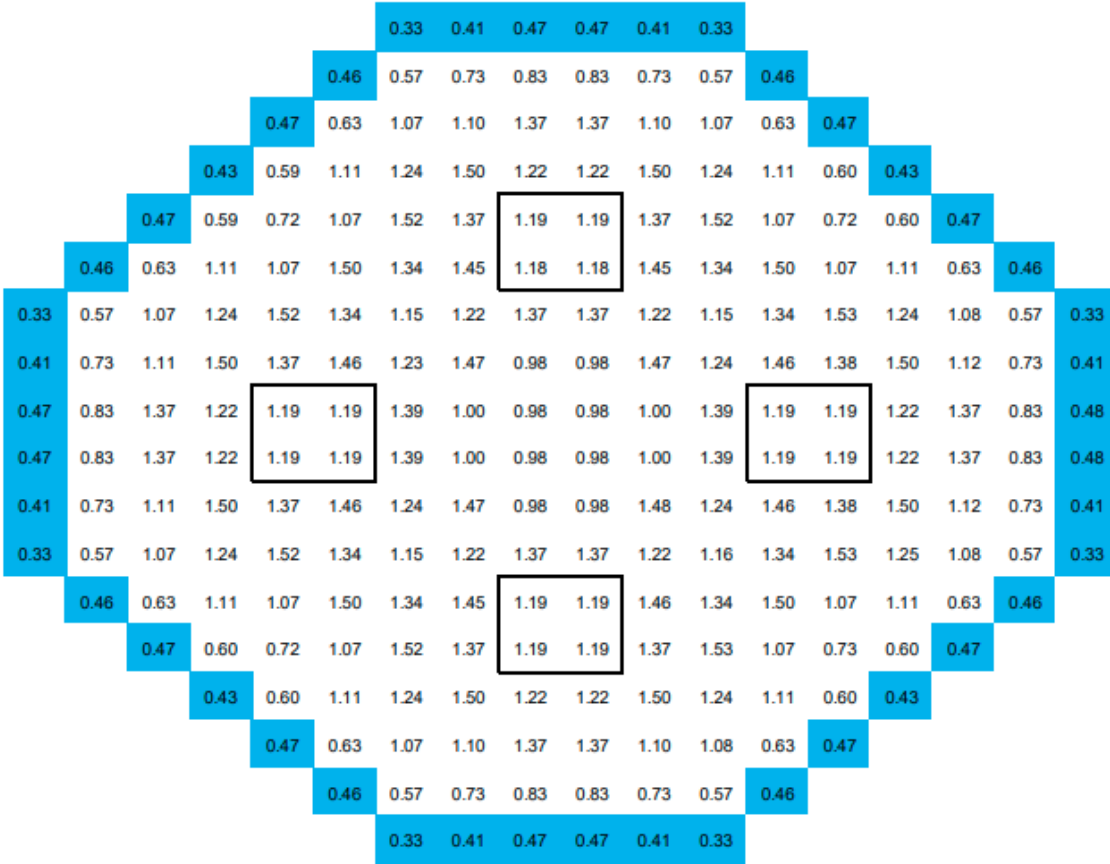
Figure 4.3-4c: Peak to Average Bundle Power Ratio at End of Cycle (Average Bundle Power – 3.625 MW th )
