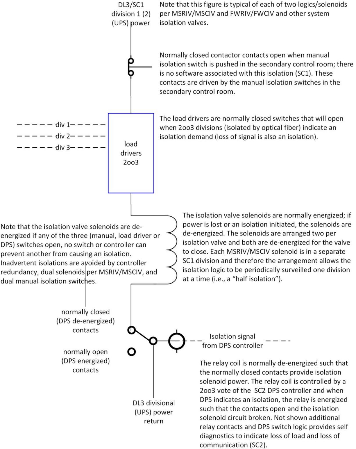
Figure 7.3-5: BWRX-300 Isolation Valve Solenoid Control and Power
