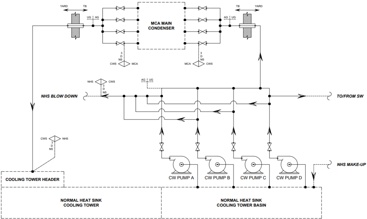
Figure 10.4-5: Circulating Water Supply Simplified Diagram
