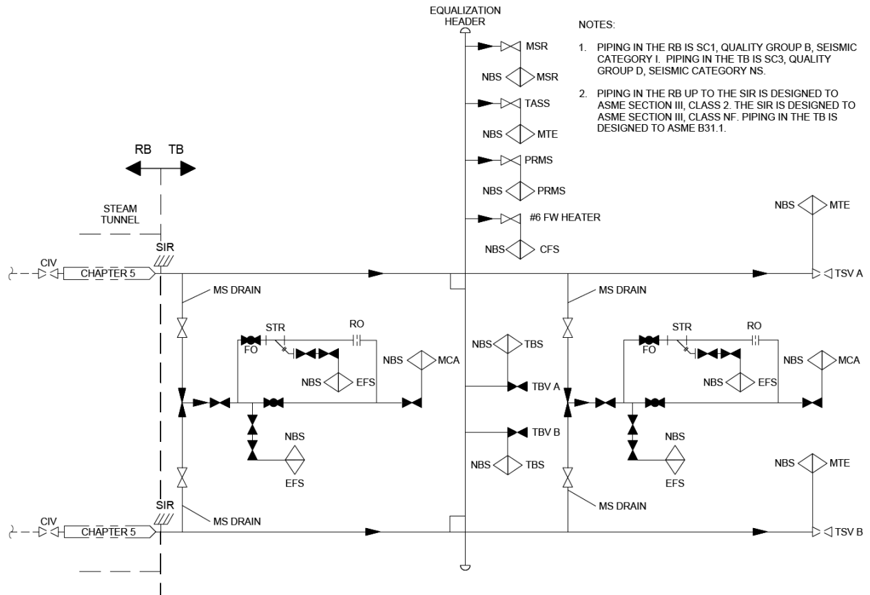
Figure 10.3-1: Main Steam Subsystem Simplified Single Line Diagram (RB & TB Portion)
