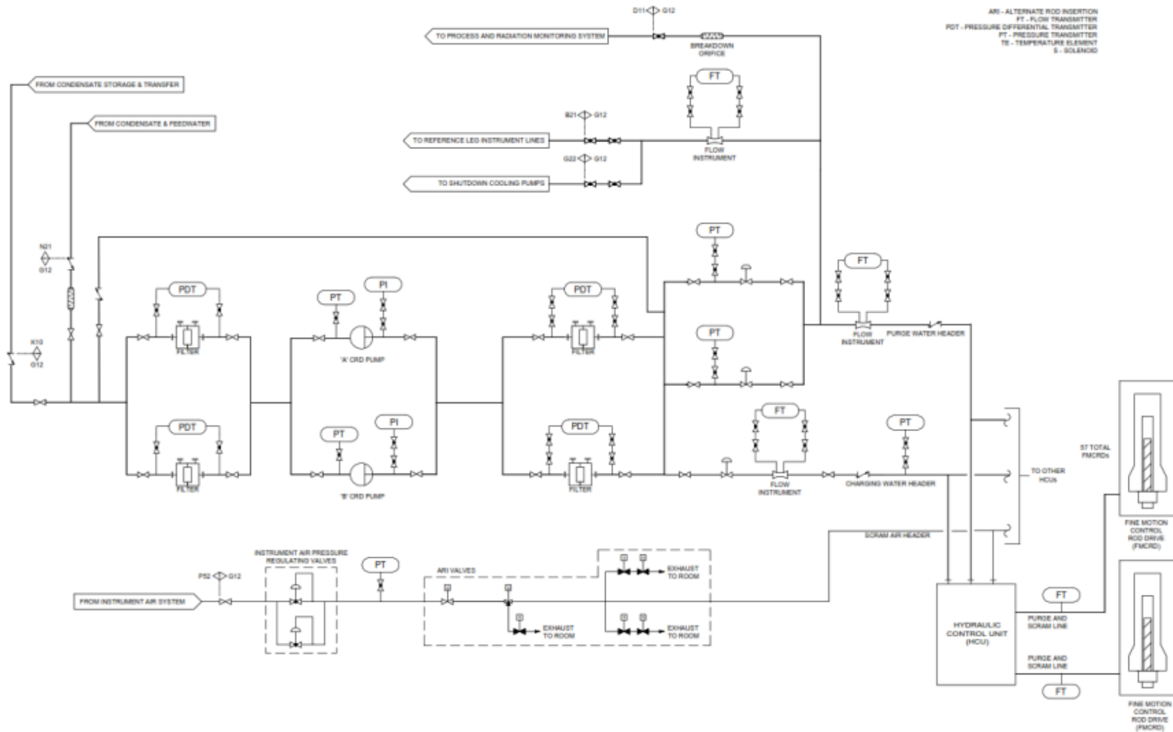
Figure 4.6-9: Control Rod Drive Hydraulic Subsystem Simplified Diagram
