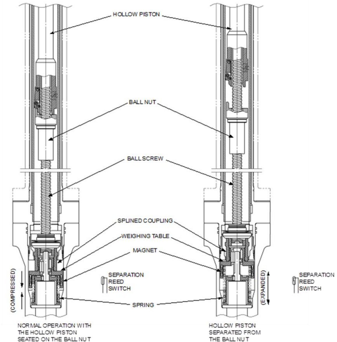
Figure 4.6-5: Representative Control Rod Separation Detection
