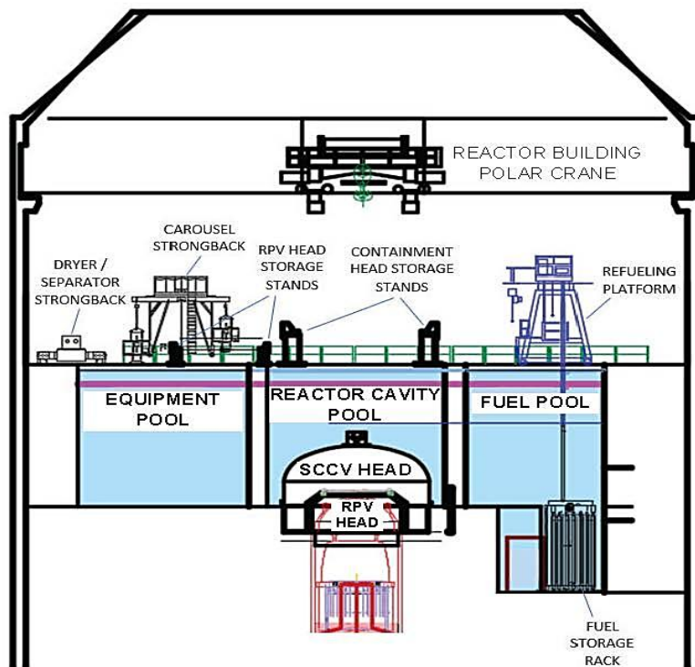
Figure 9.1-4: Location of Equipment on Refuel Floor
