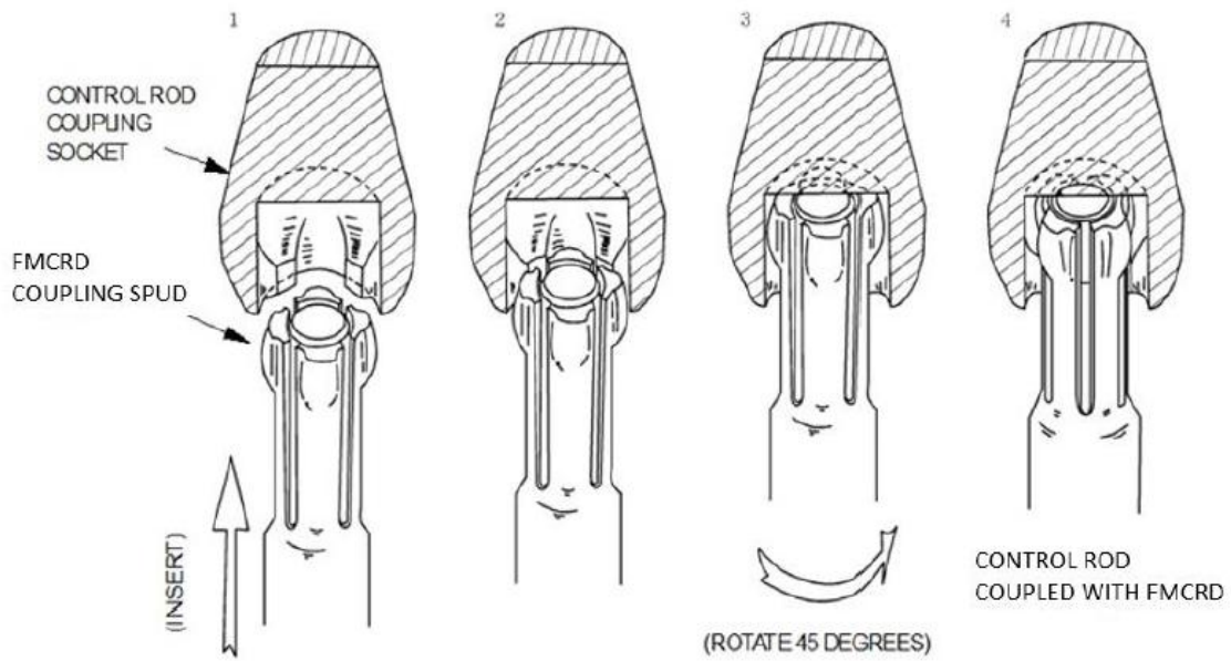
Figure 4.6-6: Representative Control Rod Coupling Socket to FMCRD Coupling Spud
