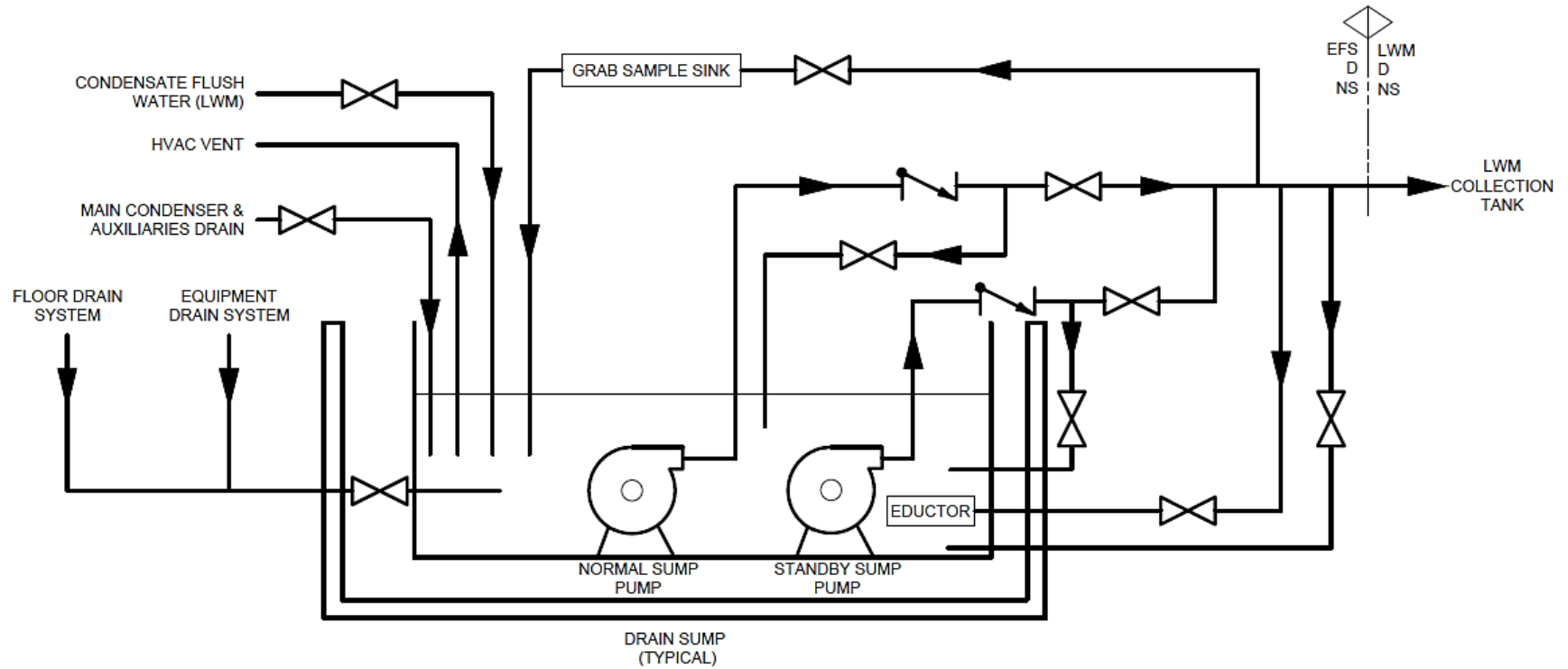
Figure 9.3-2: Normal Sump Simplified Diagram
