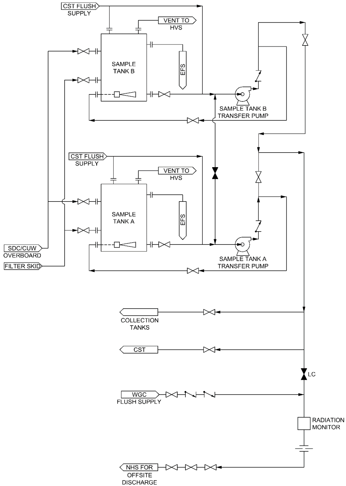
Figure 11.2-2: Waste Sampling Subsystem Simplified Diagram
