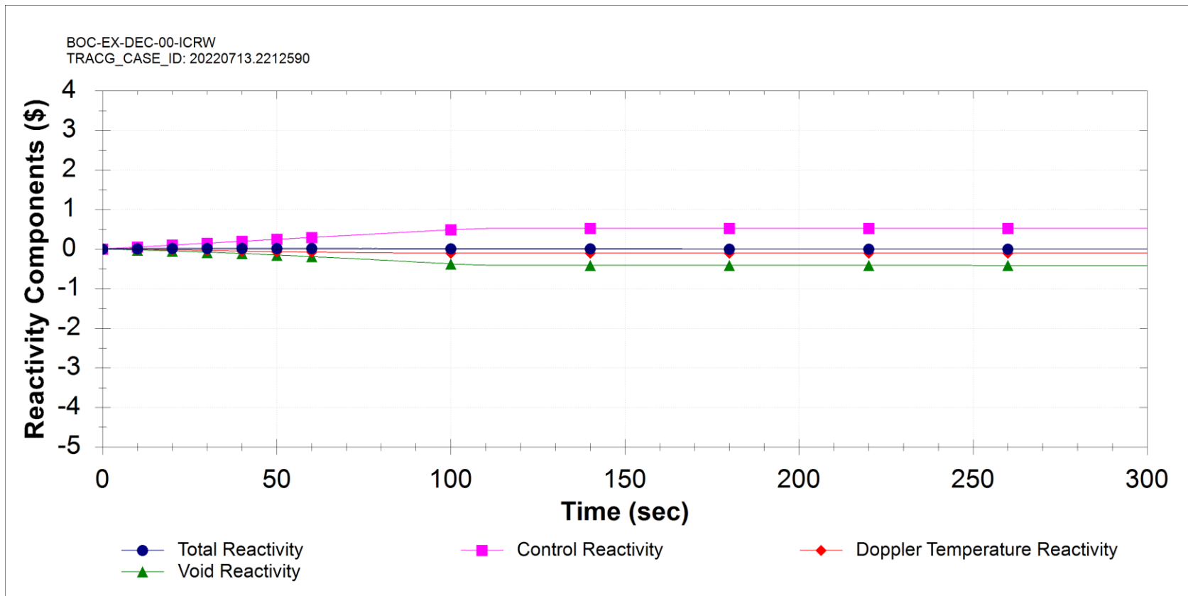
Figure 15.5-152: Inadvertent Control Rod Withdrawal at Power - Single Rod (ICRW)
