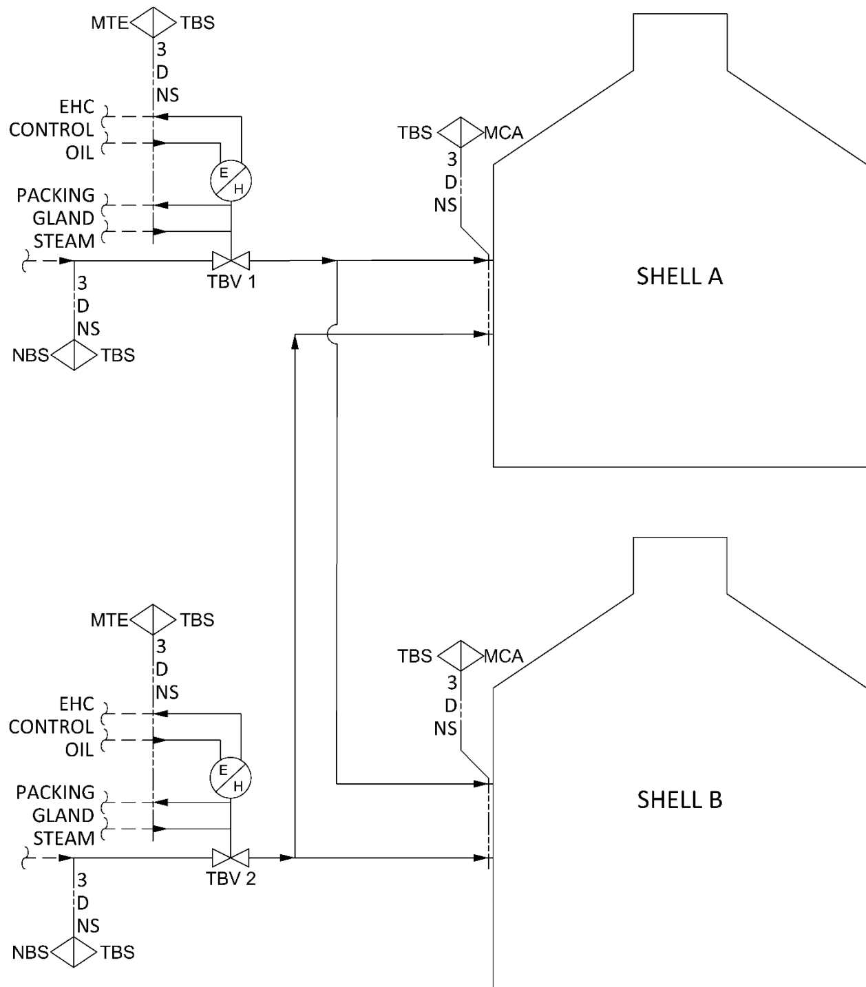
Figure 10.4-4: Turbine Bypass System Simplified Diagram
