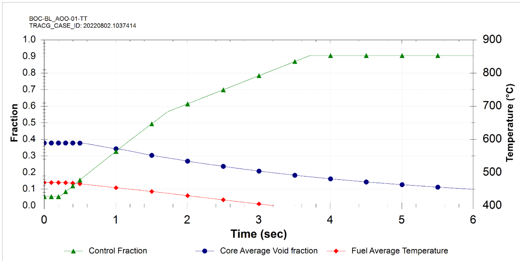
Figure 15.5-14: Turbine Trip (AOO)
