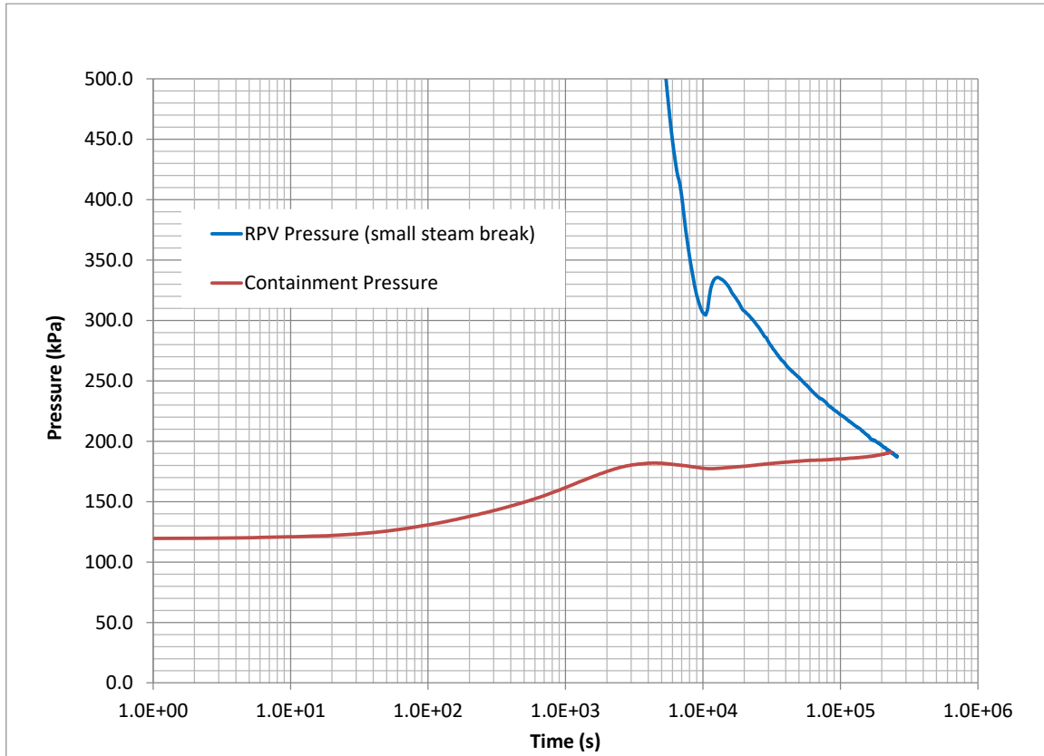
Figure 15.5-110: Containment Pressure, Small Steam Pipe Break With LOPP, Conservative Case
