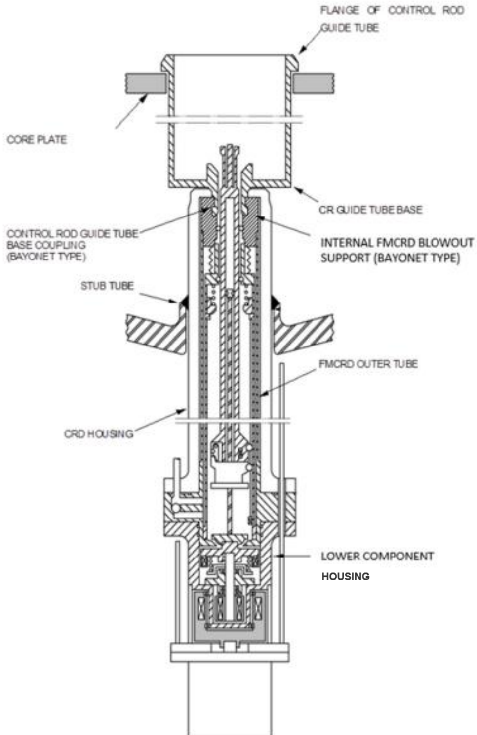
Figure 4.6-3: Representative Internal Control Rod Drive Blowout Support Schematic
