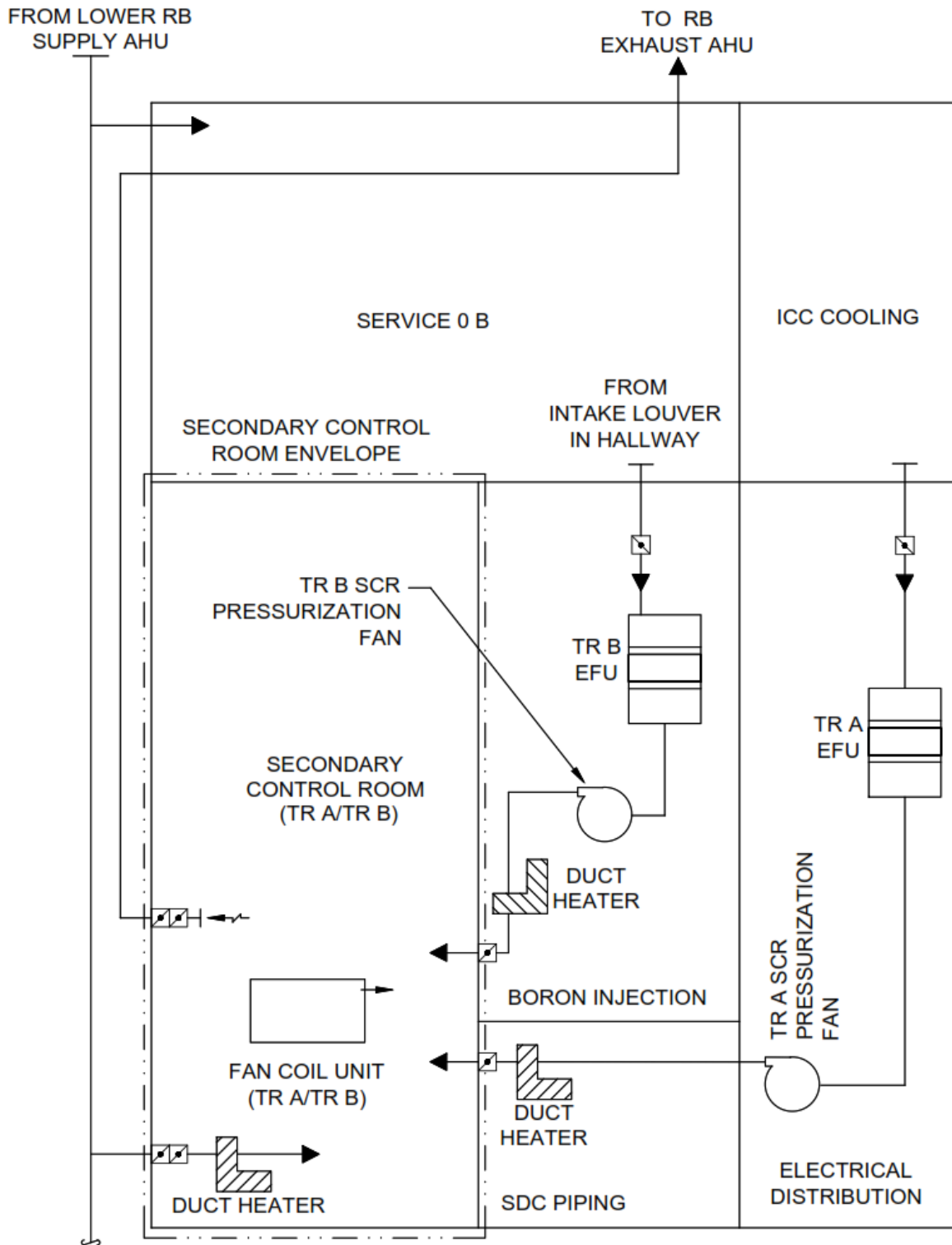
Figure 9.4-5: Secondary Control Room Heating, Ventilation, and Cooling Simplified Diagram
