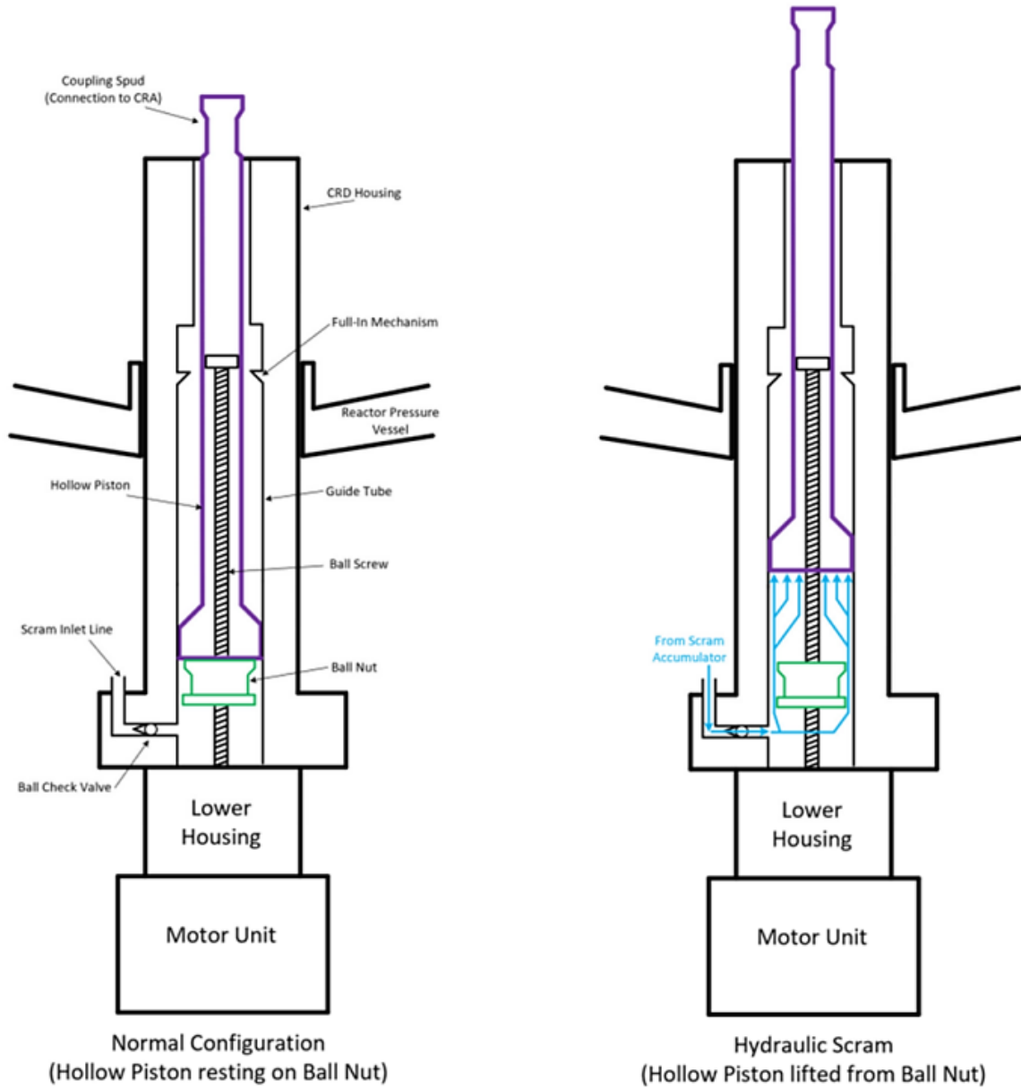
Figure 4.6-1: BWRX-300 Simplified View of FMCRD with Hydraulic Scram
