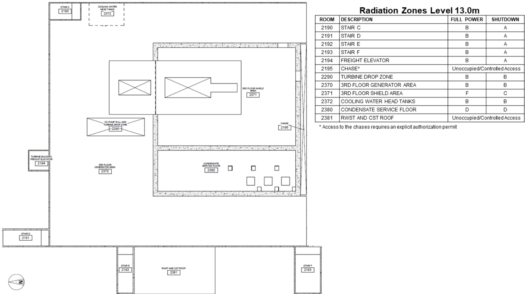
Figure 12.3-13: Turbine Building Level 13.0 Meters Radiation Zones
