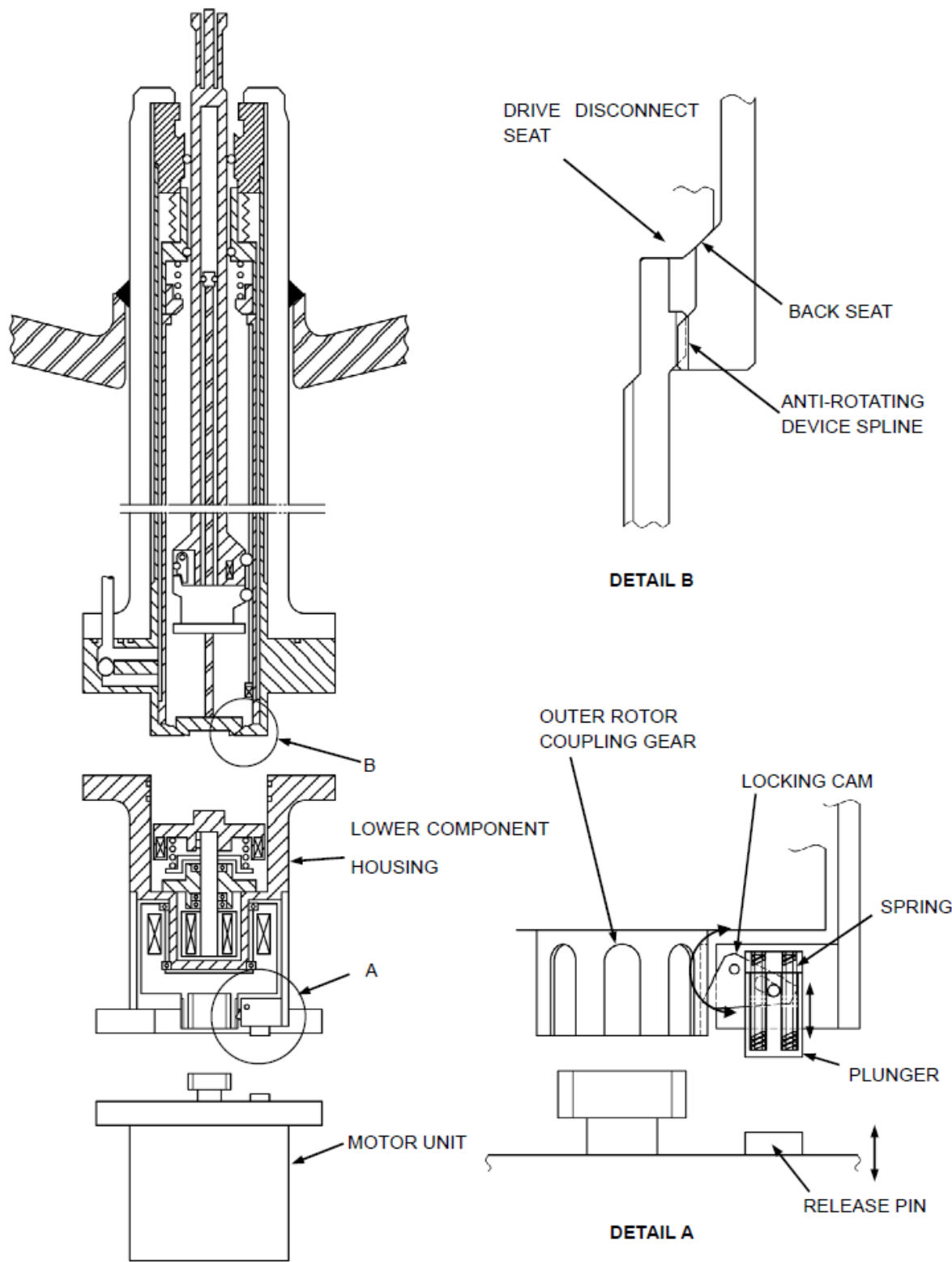
Figure 4.6-10: Representative Fine Motion Control Rod Drive Anti-Rotation Devices
