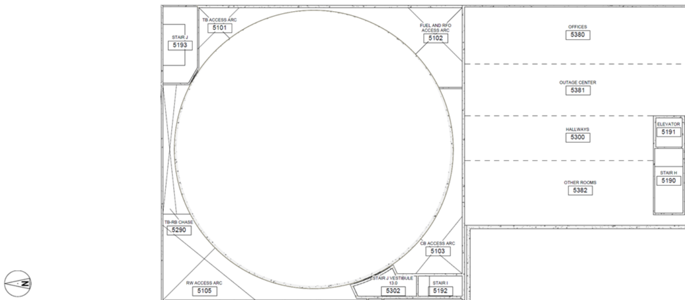
Figure 12.3-19: Service Building Level 13.0 Meters Radiation Zones
