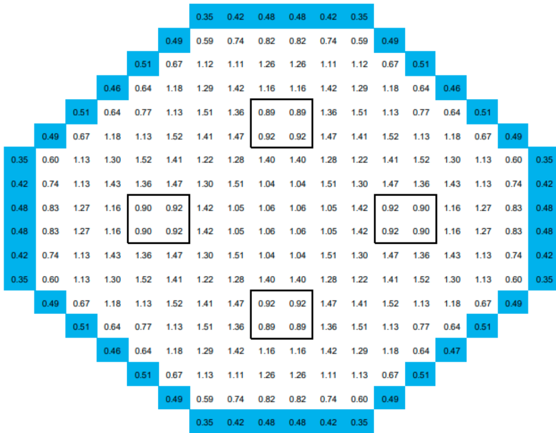
Figure 4.3-4b: Peak to Average Bundle Power Ratio at Middle of Cycle (Average Bundle Power – 3.625 MW th )
