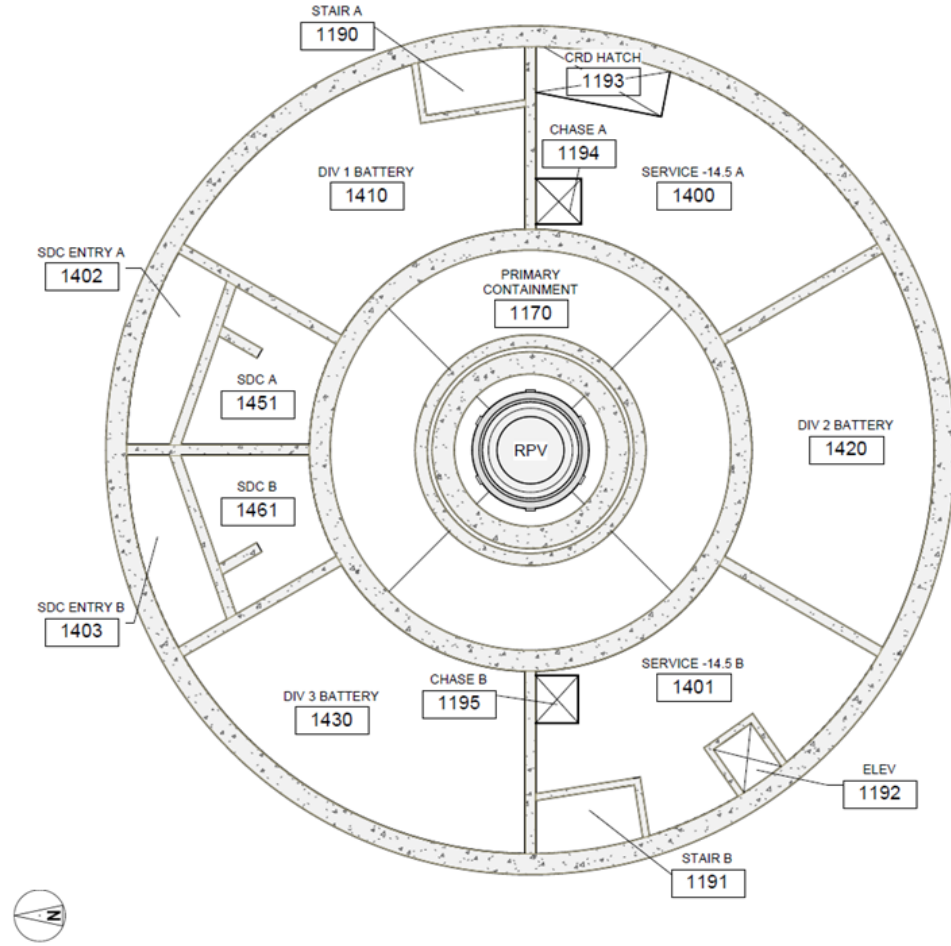
Figure 12.3-4: Reactor Building Level -14.5 Meters Radiation Zones
