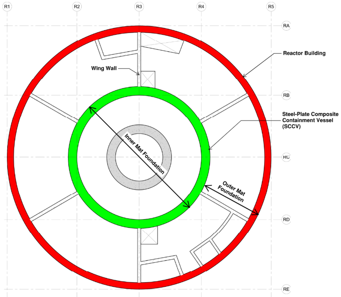
Figure 3.8-8: Plan View of BWRX-300 Mat Foundation
