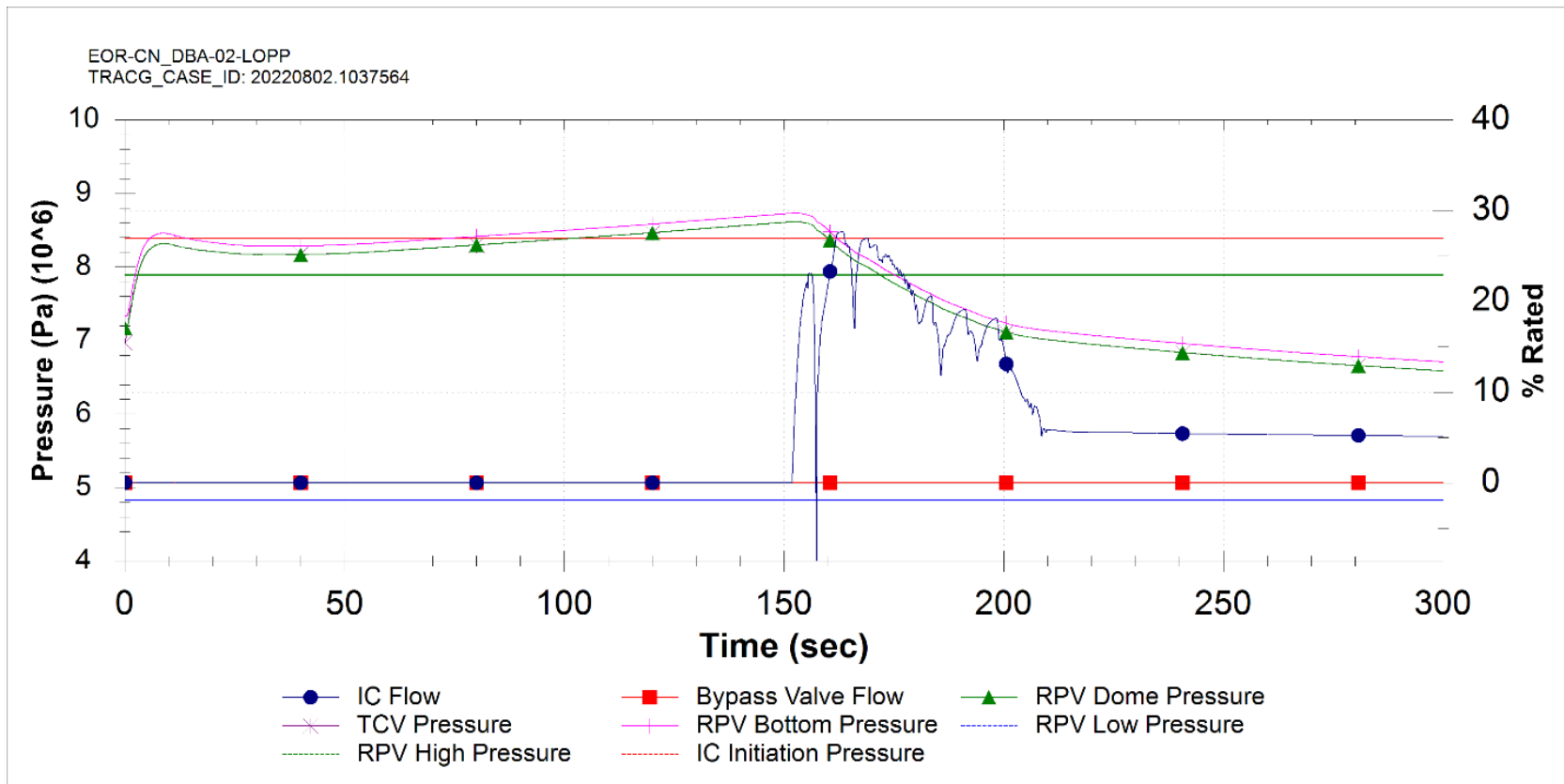
Figure 15.5-59: Loss of Preferred Power (DBA)
