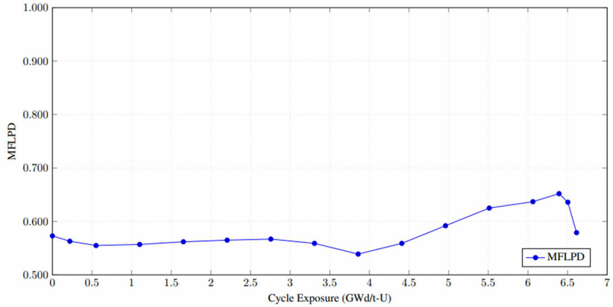
Figure 4.3-9: Maximum Fraction of Limiting Power Density (MFLPD) vs Cycle Exposure
