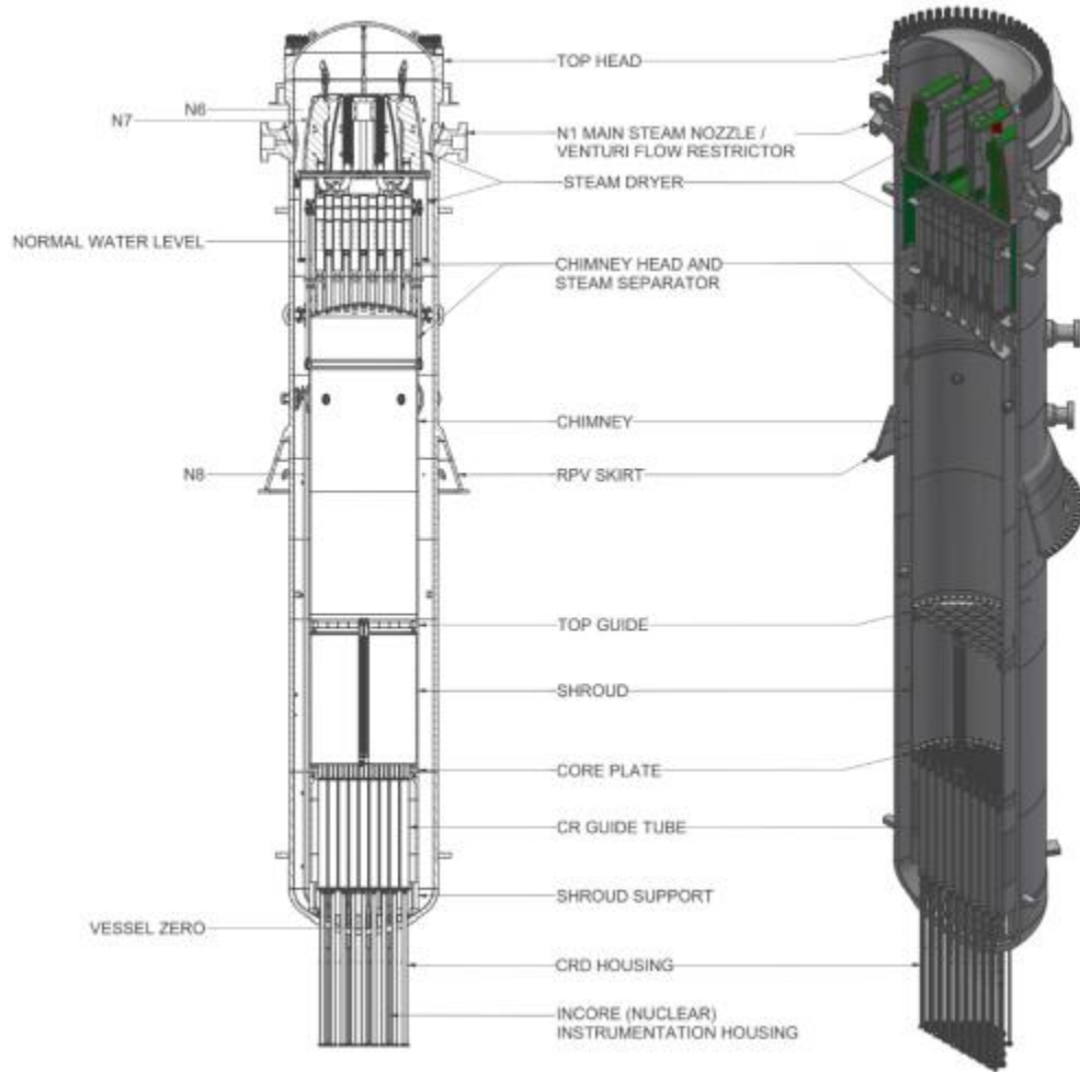
Figure 4.1-1: BWRX-300 Reactor Pressure Vessel and Internals Schematic
