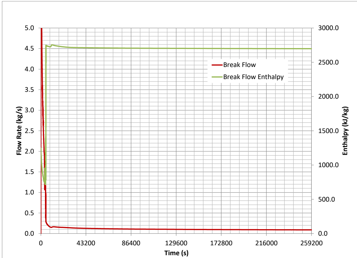
Figure 15.5-116: Break Flow Rate and Enthalpy, Small Liquid Pipe Break, Conservative Case
