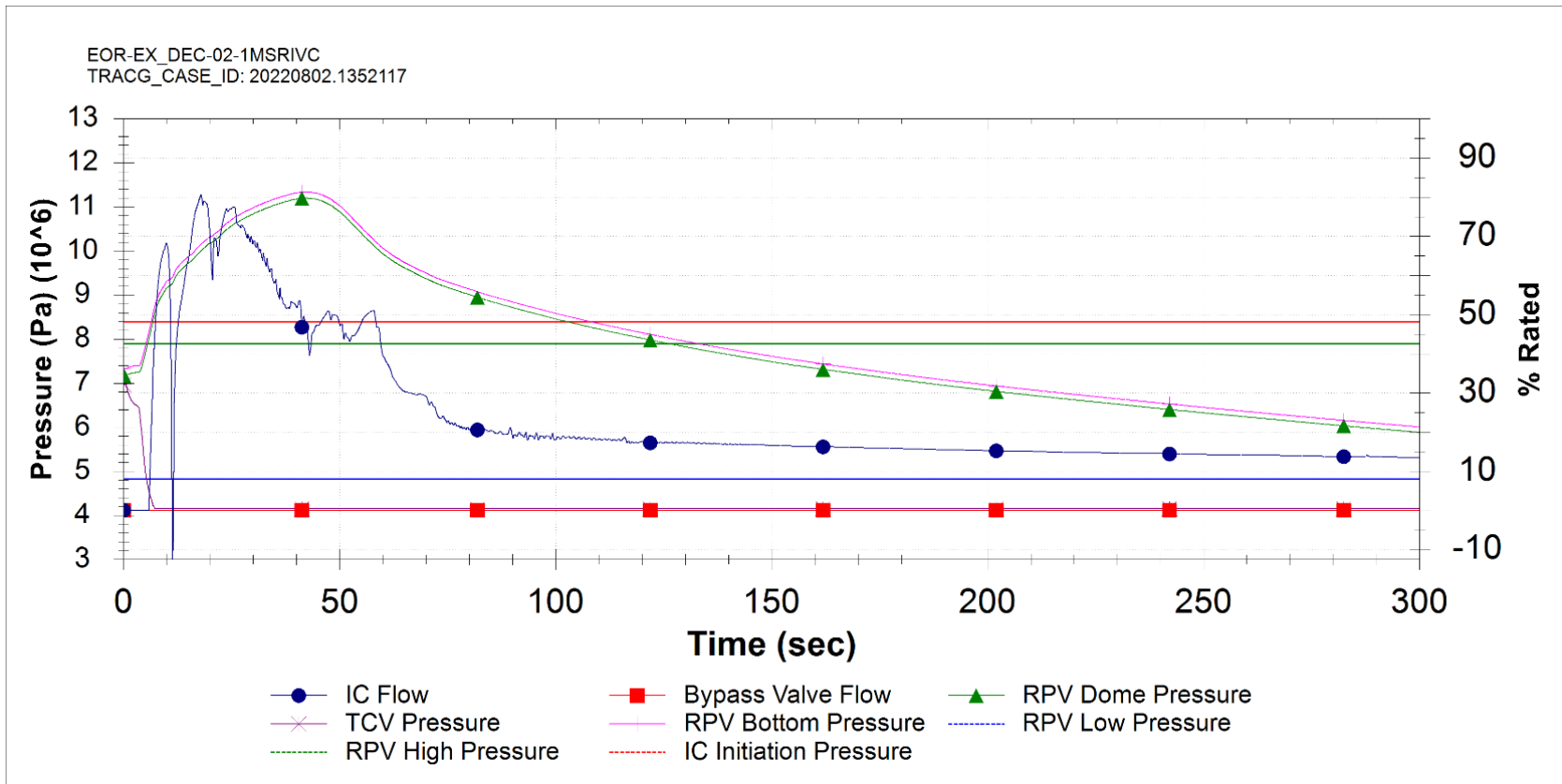
Figure 15.5-120: Closure of One Main Steam Reactor Isolation Valve with Failure to Scram (DEC)
