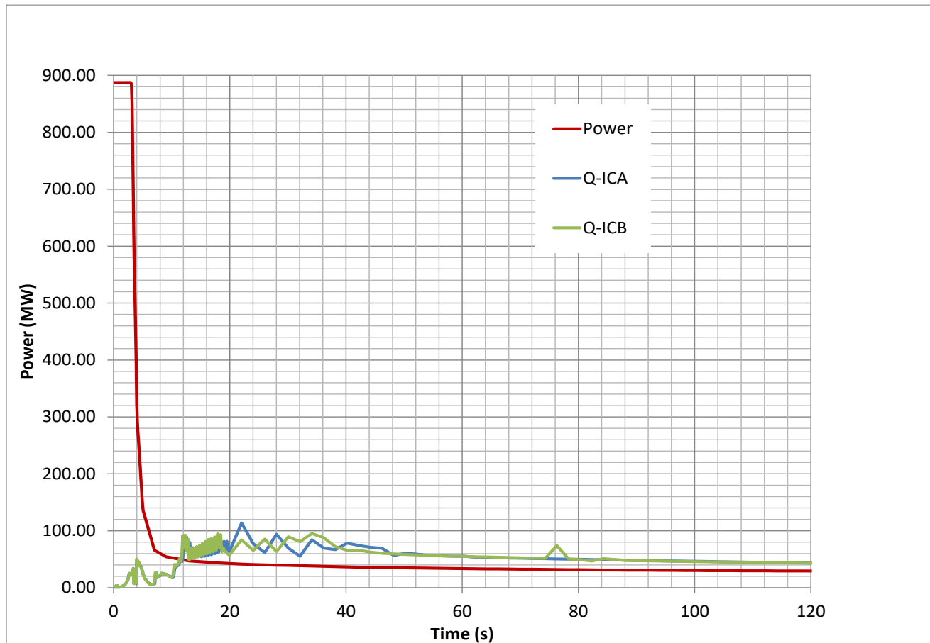
Figure 15.5-161: Reactor Power, Large FW Pipe Break, Conservative Case
