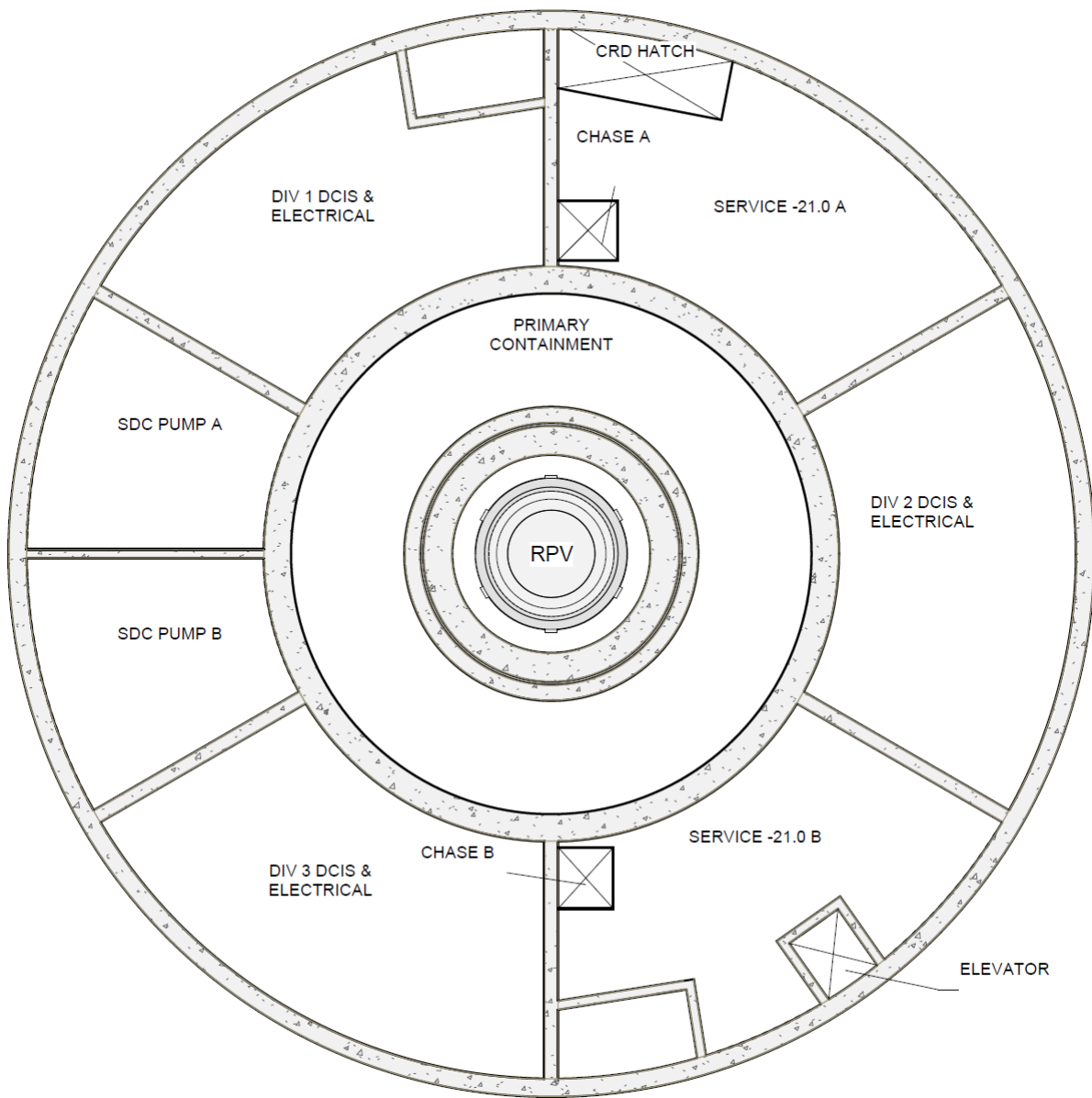
Figure 1.2-11: Reactor Building Plan View, Elevation -21.0m
