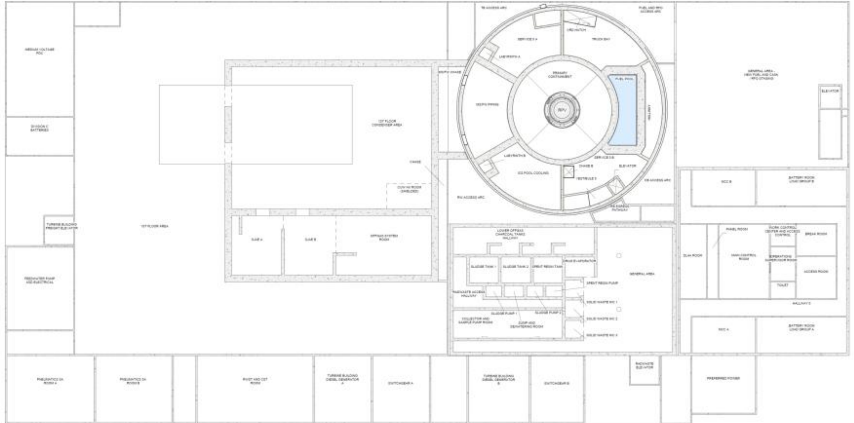
Figure 1.2-3: BWRX-300 Plan View Elevation 0m
