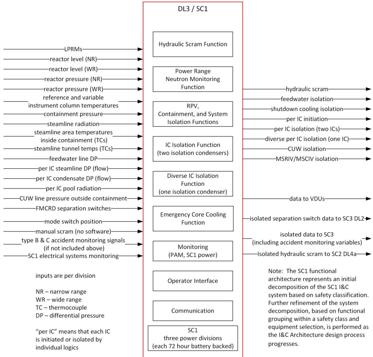
Figure 7.3-2: Safety Class 1 Functional Architecture
