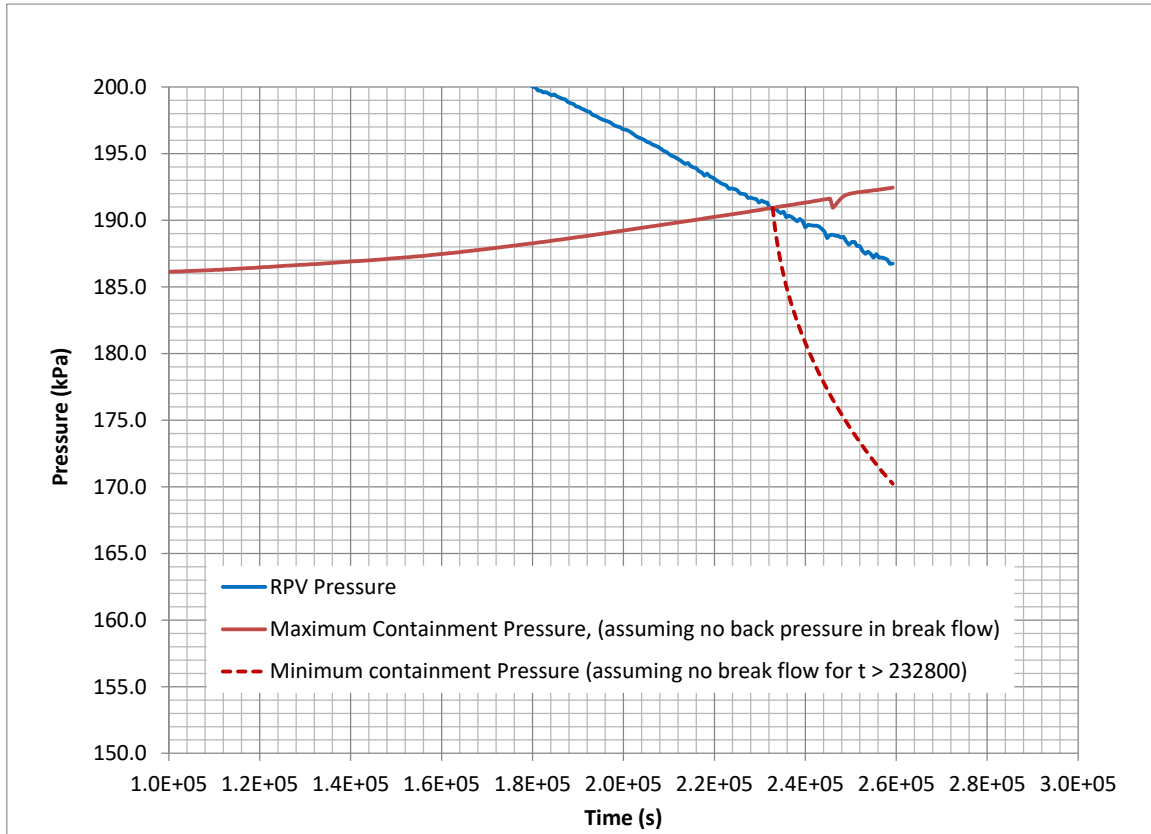
Figure 15.5-115: Containment Pressure After RPV Depressurization, Small Liquid Pipe Break, Conservative Case
