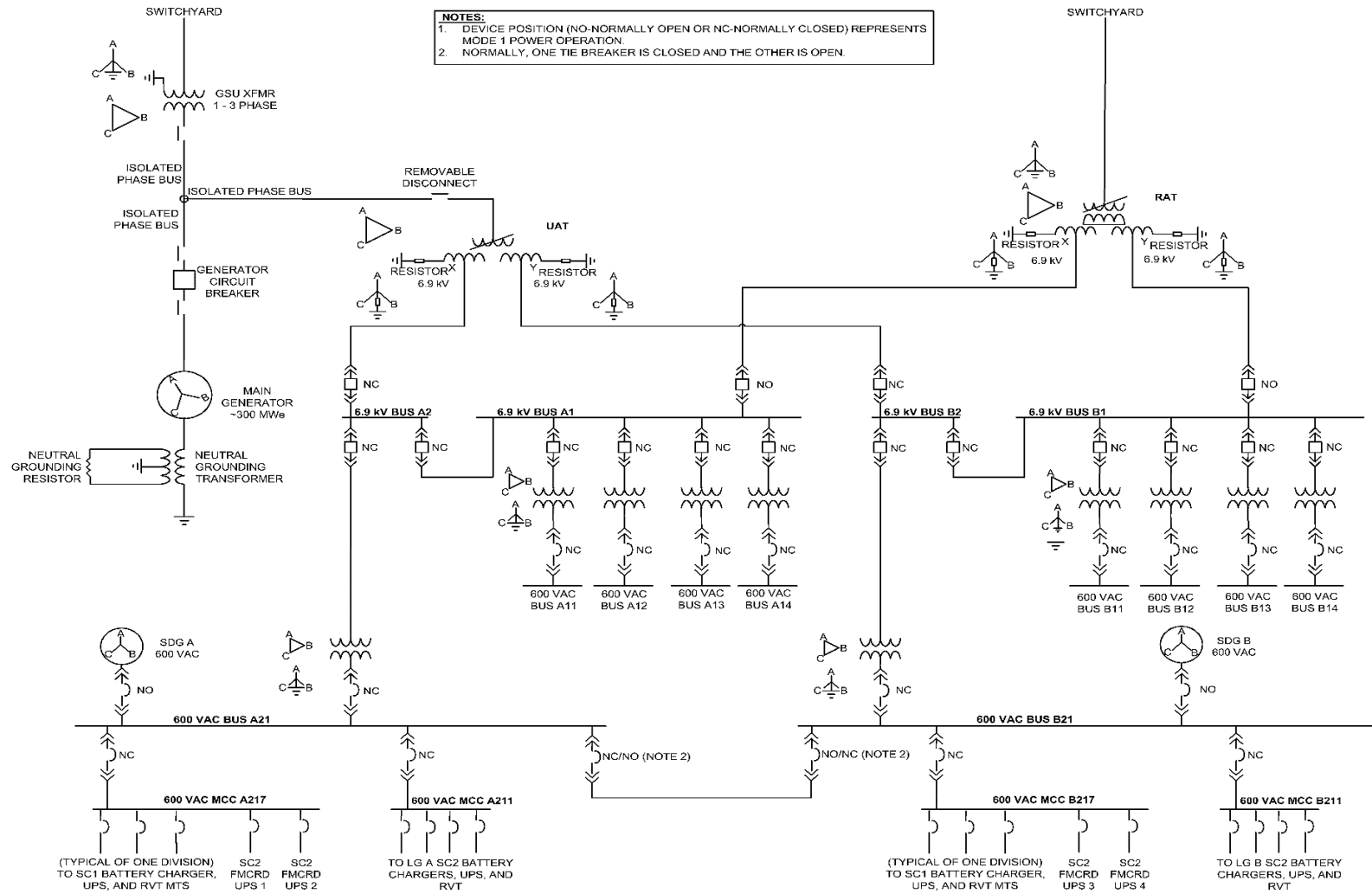
Figure 8.1-1: Main Electrical One-Line
