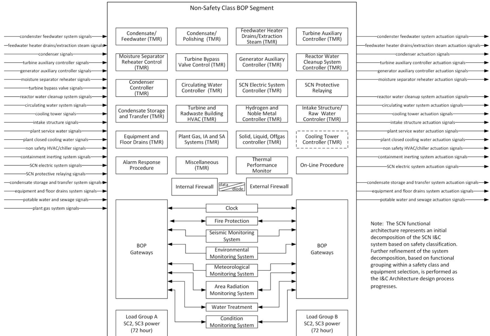
Figure 7.3-13: Non-Safety Class Balance of Plant Segment Functional Architecture
