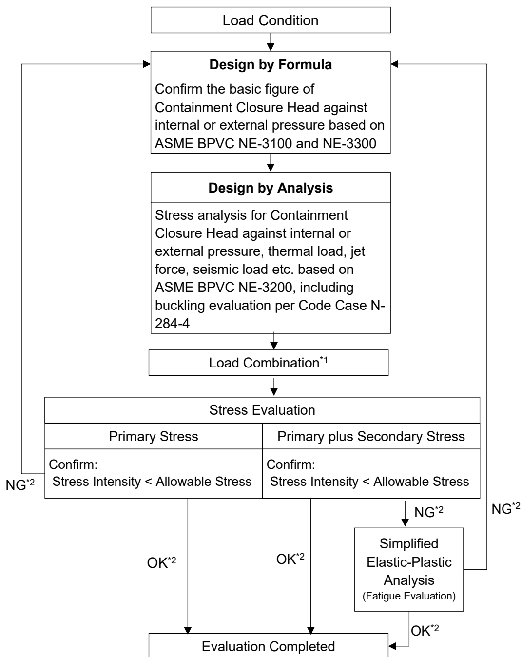
Figure 3.8-6: Design Procedures for the Containment Closure Head
