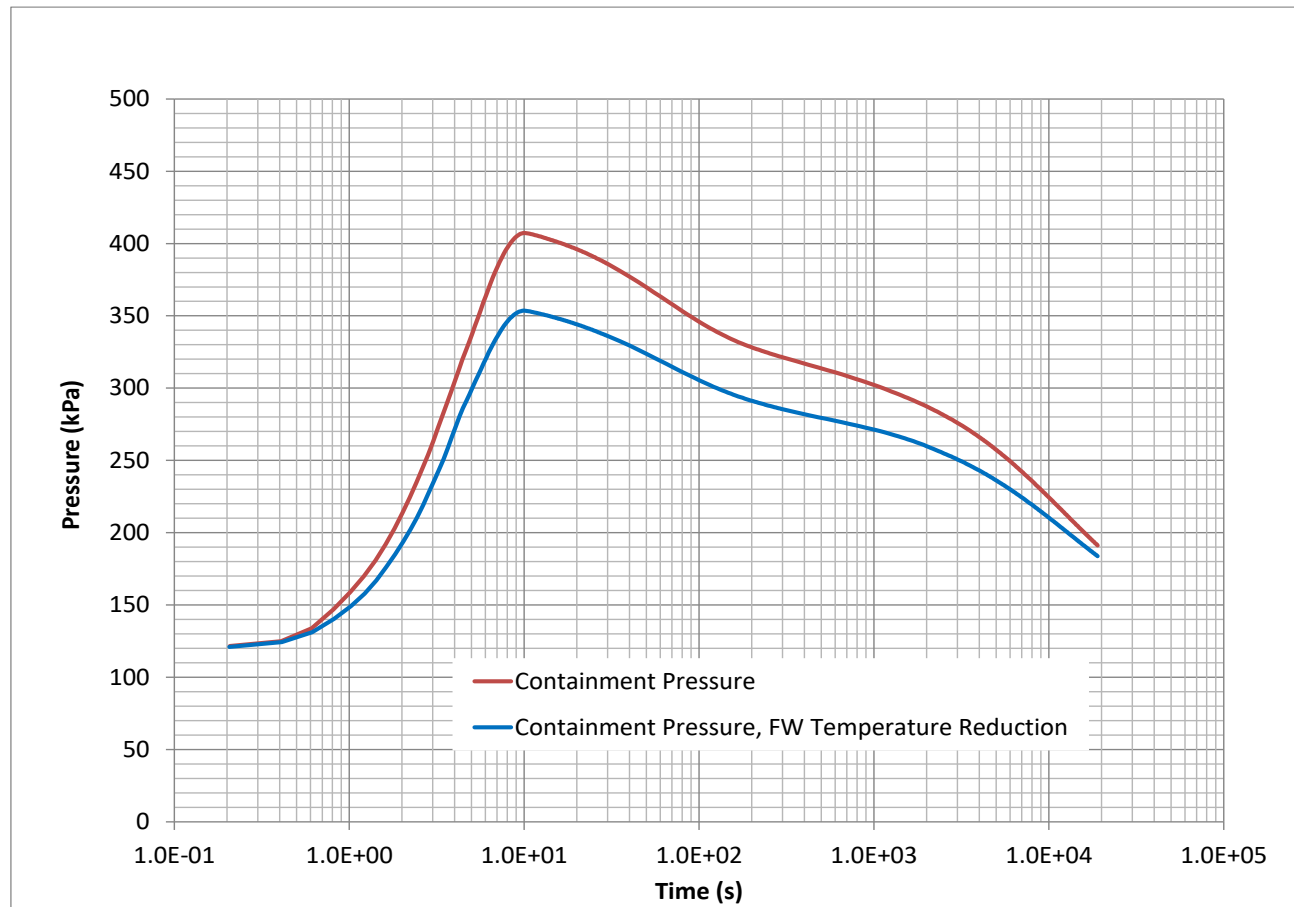
Figure 15.5-165: Containment Pressure, Large FW Pipe Break, Conservative Case
