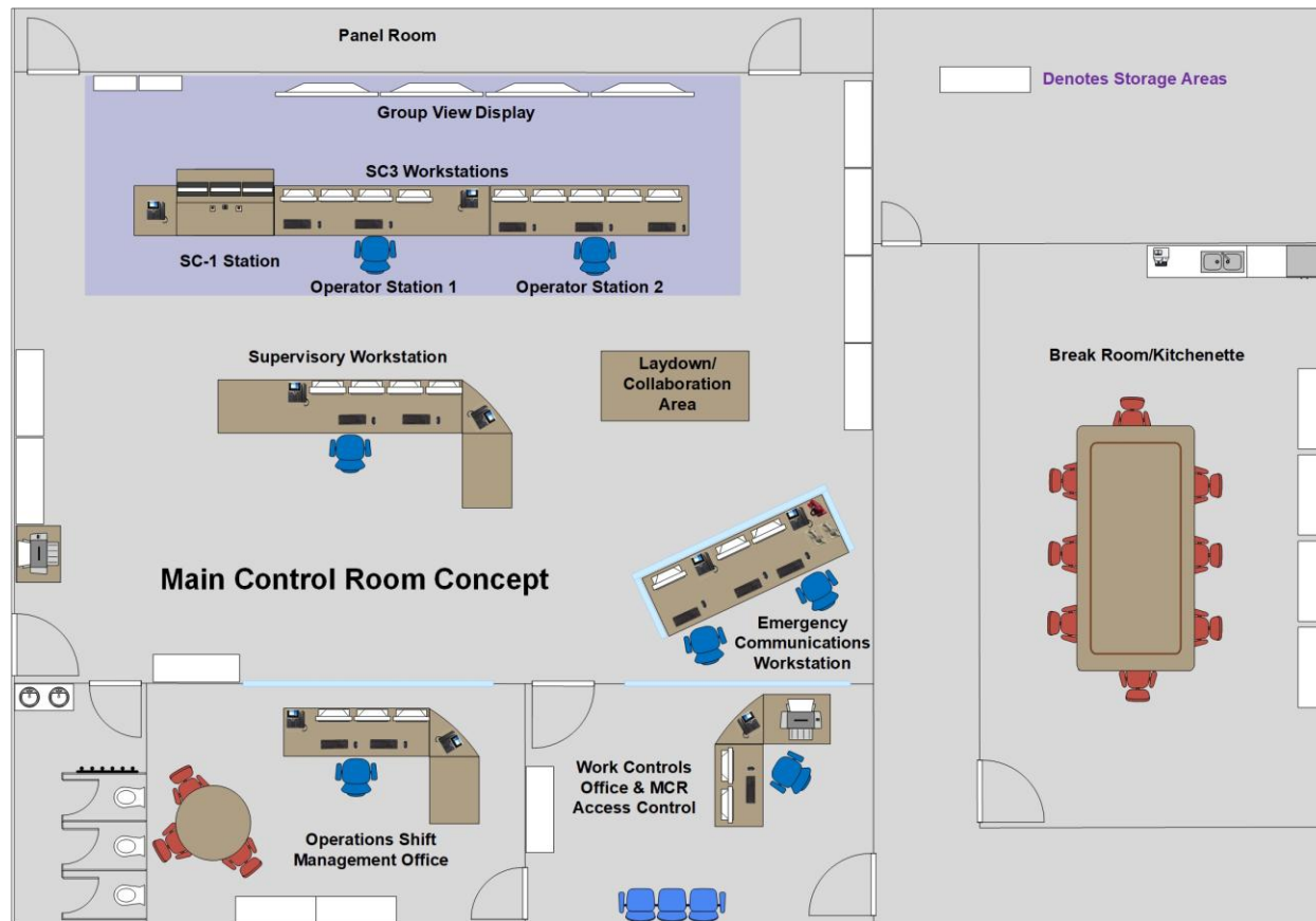
Figure 7.5-1: Main Control Room and Surrounding Areas (Top View)
