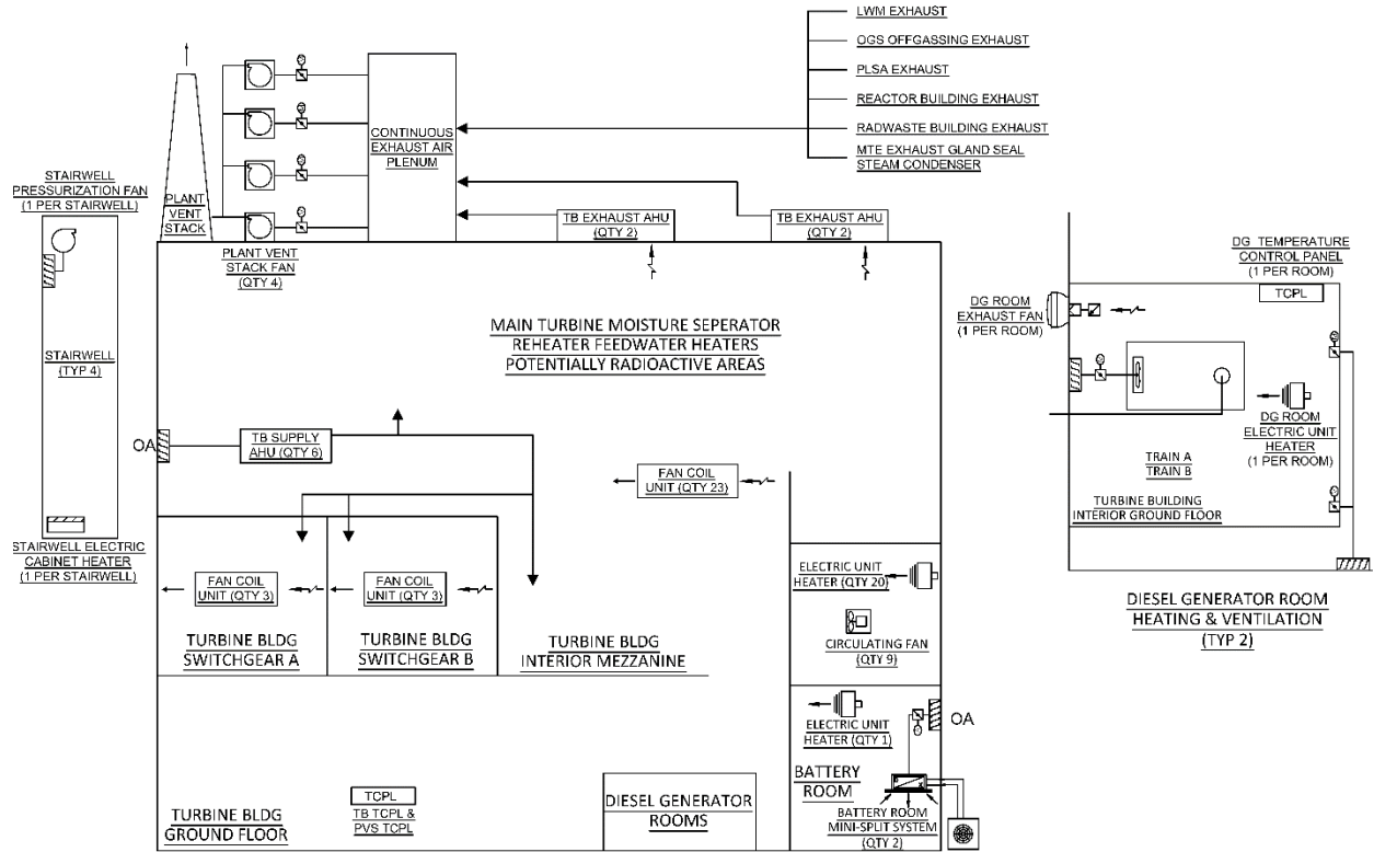
Figure 9.4-3: Turbine Building Heating Ventilation, and Cooling System and Plant Vent Stack Simplified Diagram
