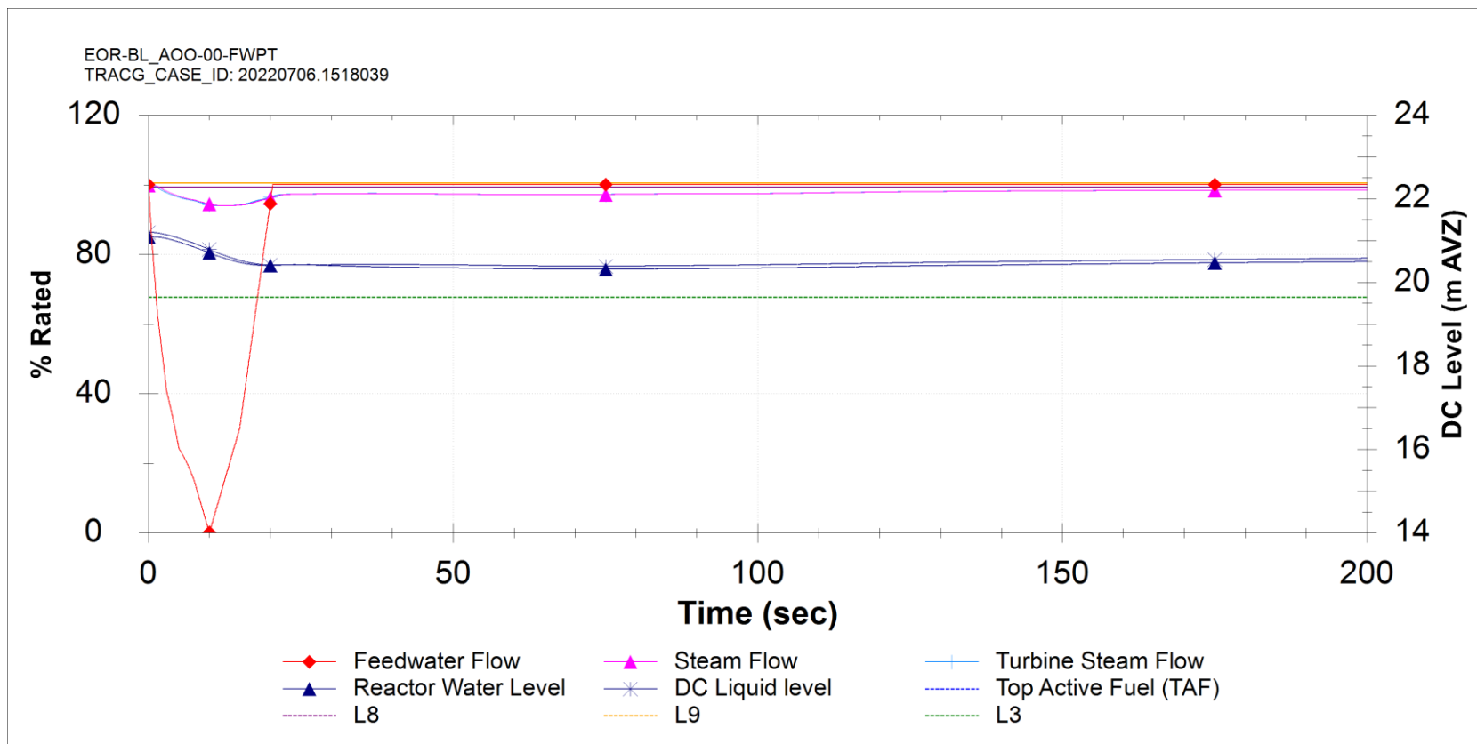
Figure 15.5-36: Feedwater Pump Trip – One Pump (AOO)
