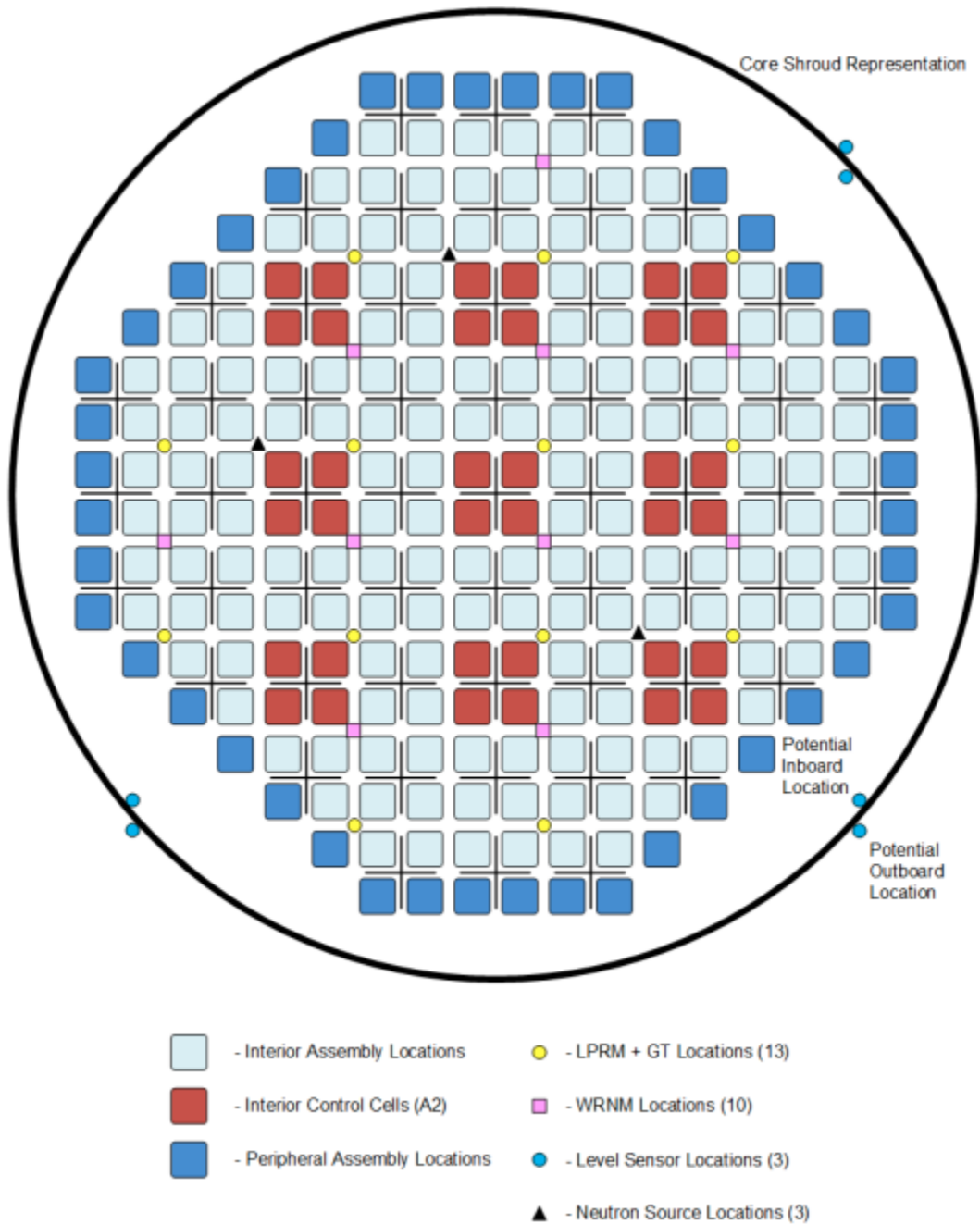
Figure 4.3-1: Core Map Instrumentation Layout
